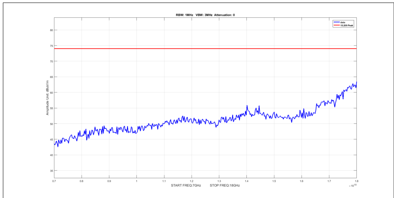
Plot 925. Undesirable Emissions, 50mni, Peak, 7-18GHz, 20M, 5490, pow11
