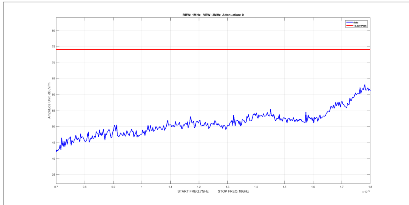
Plot 924. Undesirable Emissions, 50mni, Peak, 7-18GHz, 20M, 5330, pow12
