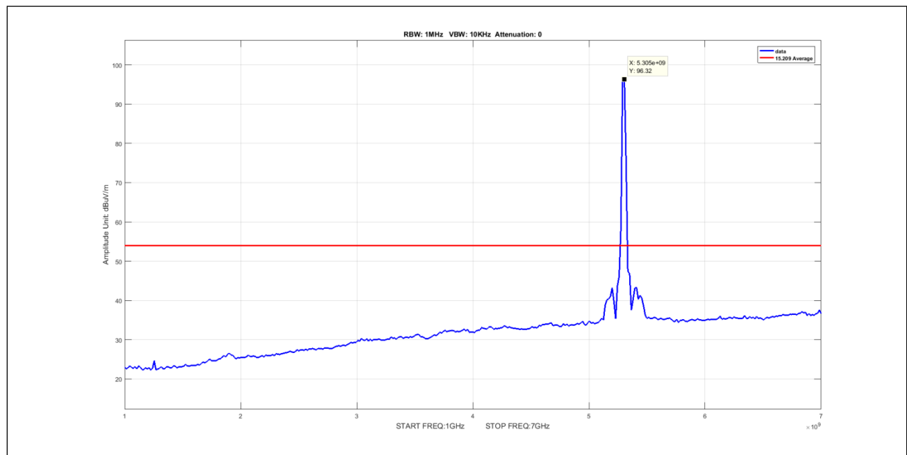
Plot 947. Undesirable Emissions, 8Omni, Average, 1-7GHz, 20M, 5300, pow12
