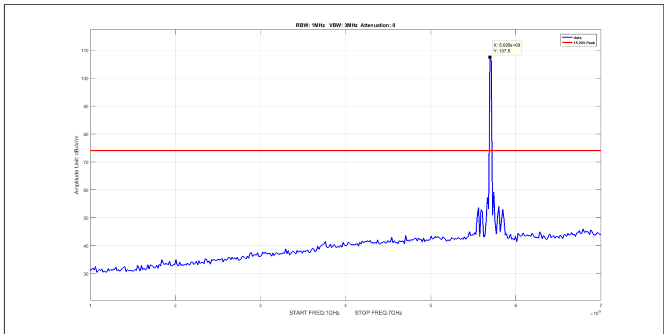
Plot 891. Undesirable Emissions, 50mni, Peak, 1-7GHz, 5M, 5700, pow8
