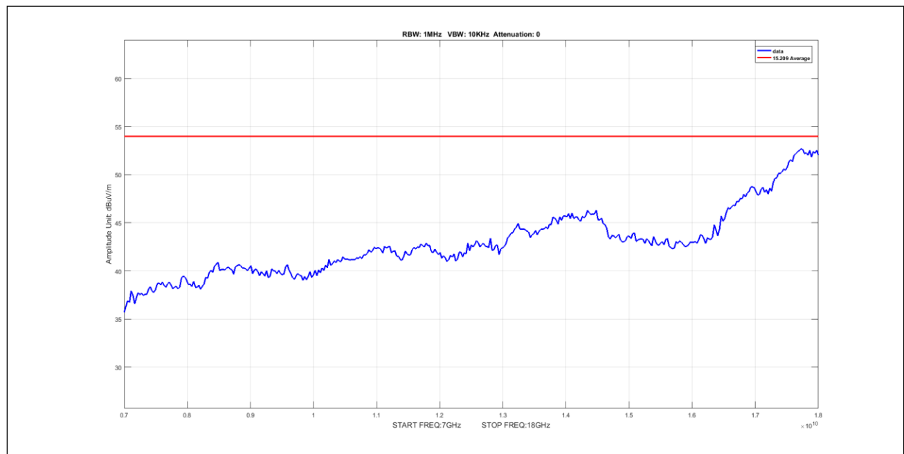
Plot 973. Undesirable Emissions, 8Omni, Average, 7-18GHz, 20M, 5490, pow9
