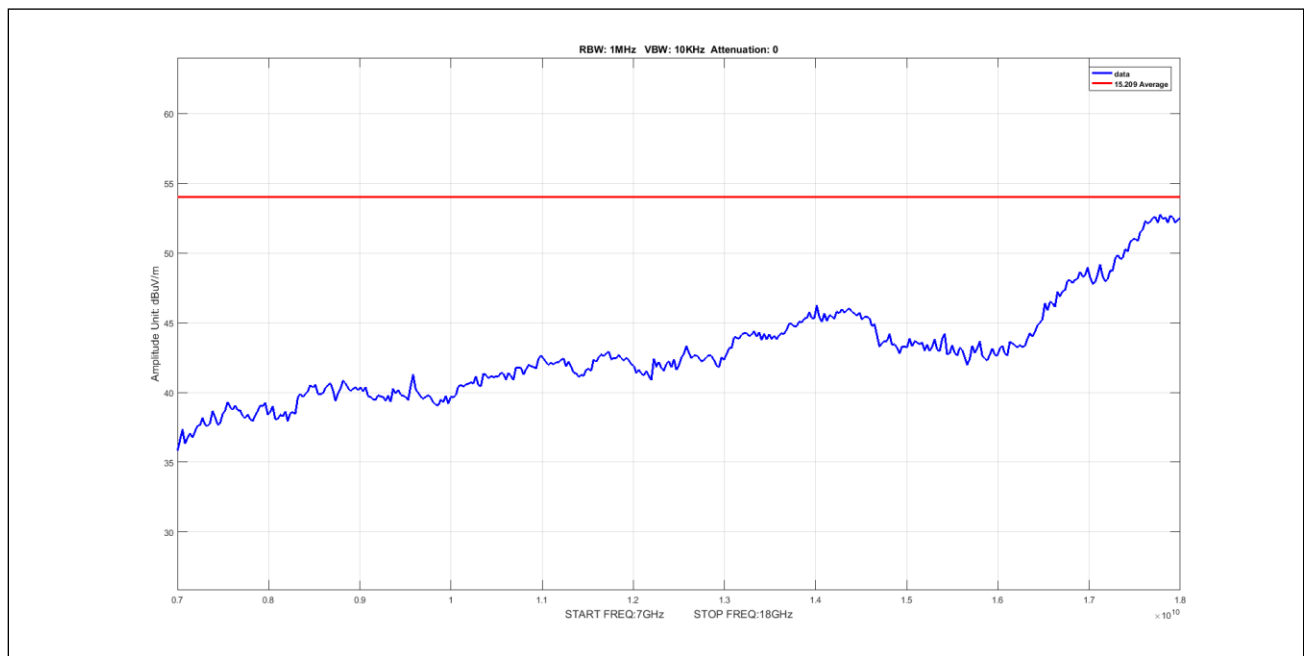
Plot 971. Undesirable Emissions, 8Omni, Average, 7-18GHz, 20M, 5300, pow12
