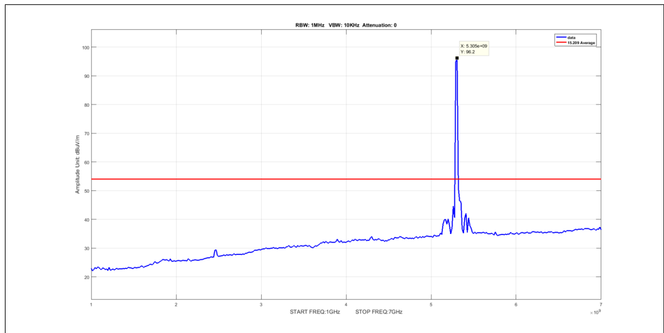
Plot 941. Undesirable Emissions, 8Omni, Average, 1-7GHz, 10M, 5300, pow9
