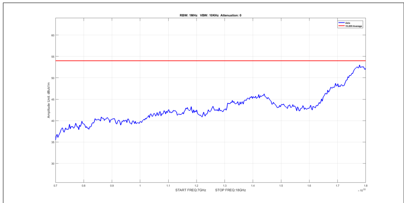
Plot 967. Undesirable Emissions, 8Omni, Average, 7-18GHz, 10M, 5490, pow10
