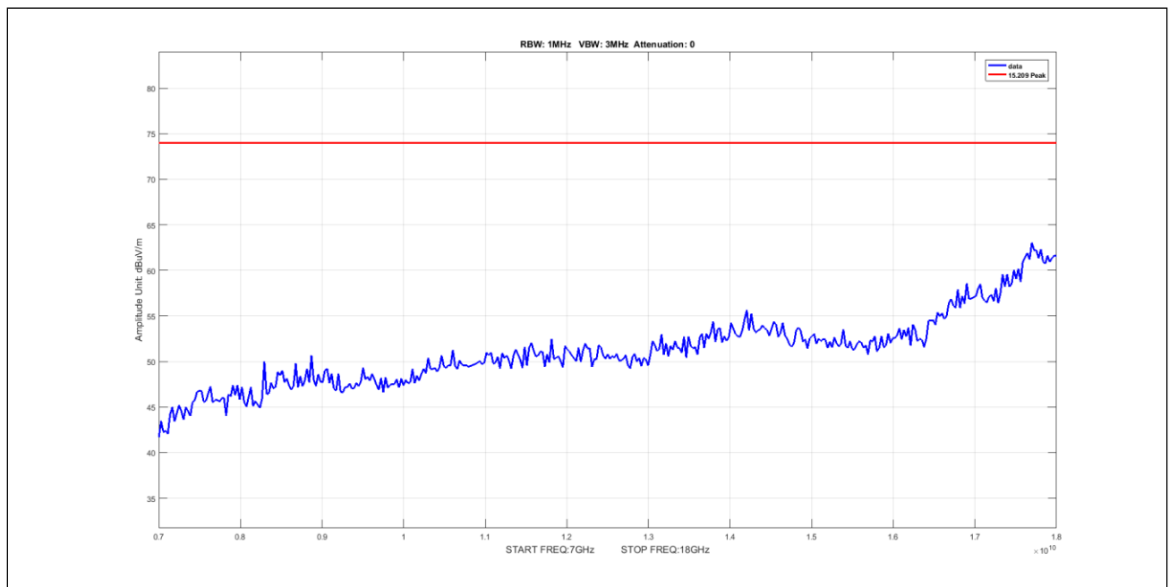
Plot 933. Undesirable Emissions, 5Omni, Peak, 7-18GHz, 40M, 5700, pow7
