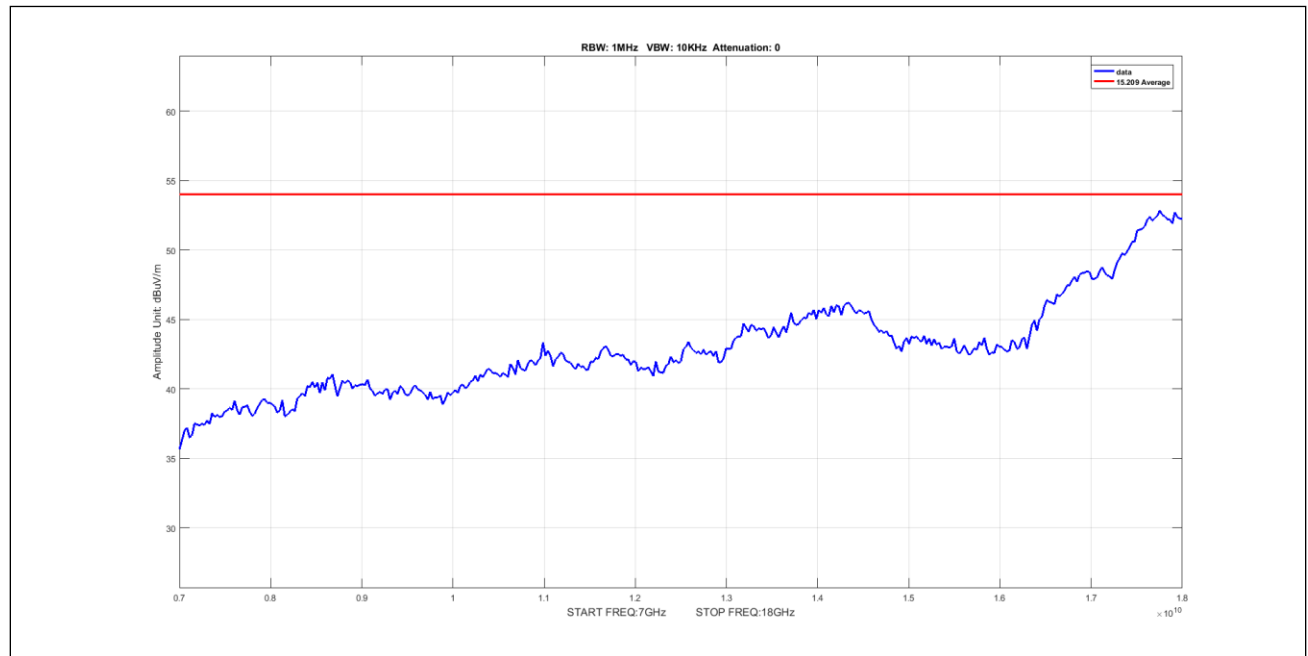
Plot 960. Undesirable Emissions, 8Omni, Average, 7-18GHz, 5M, 5330, pow6
