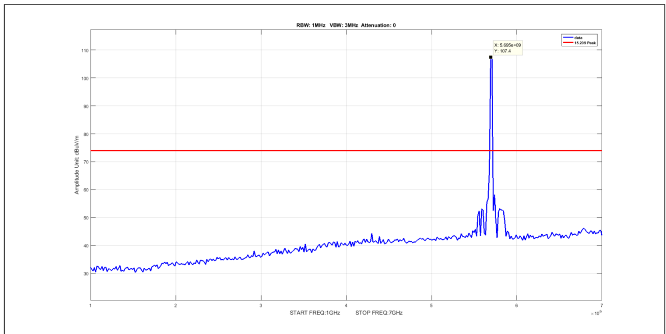
Plot 897. Undesirable Emissions, 50mni, Peak, 1-7GHz, 10M, 5700, pow11
