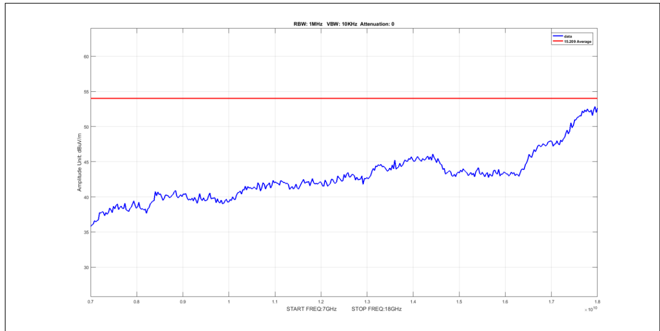
Plot 880. Undesirable Emissions, 5Omni, Average, 7-18GHz, 40M, 5270, pow19
