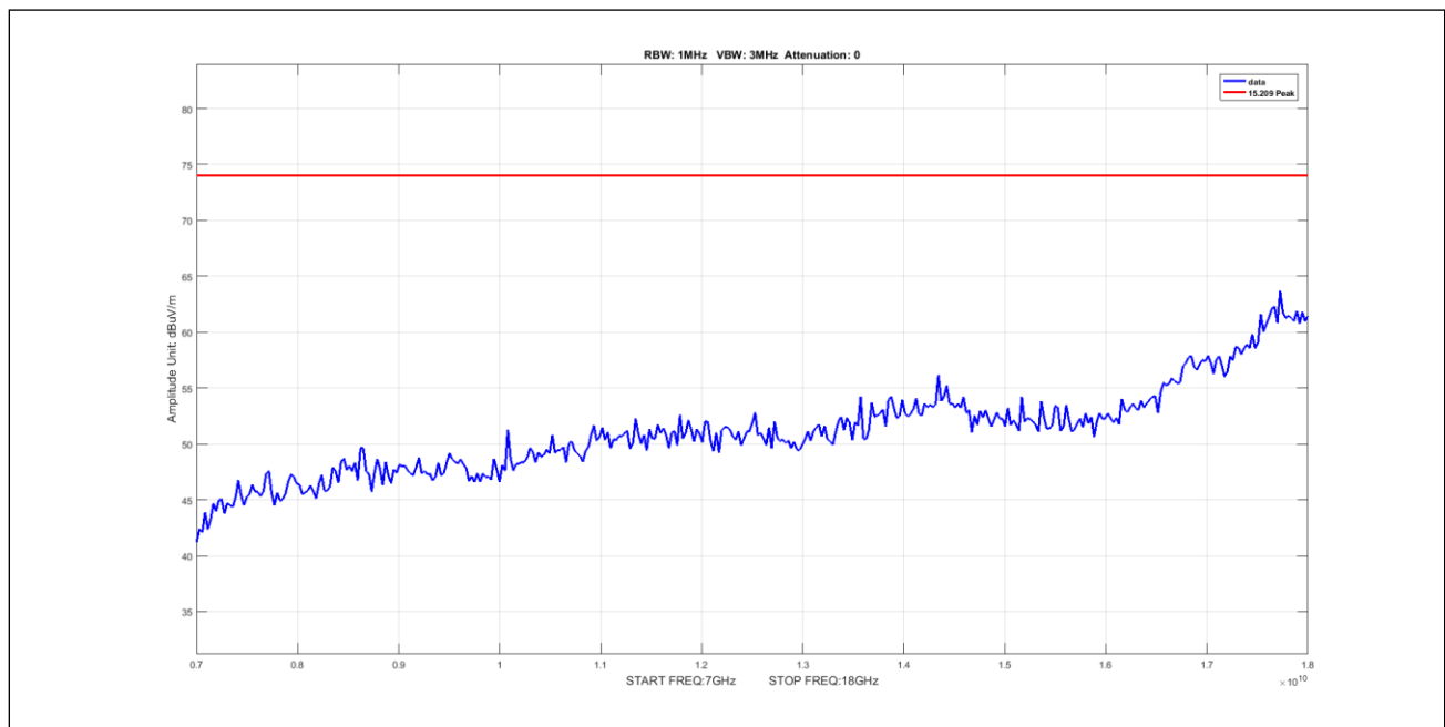
Plot 911. Undesirable Emissions, 50mni, Peak, 7-18GHz, 5M, 5300, pow8
