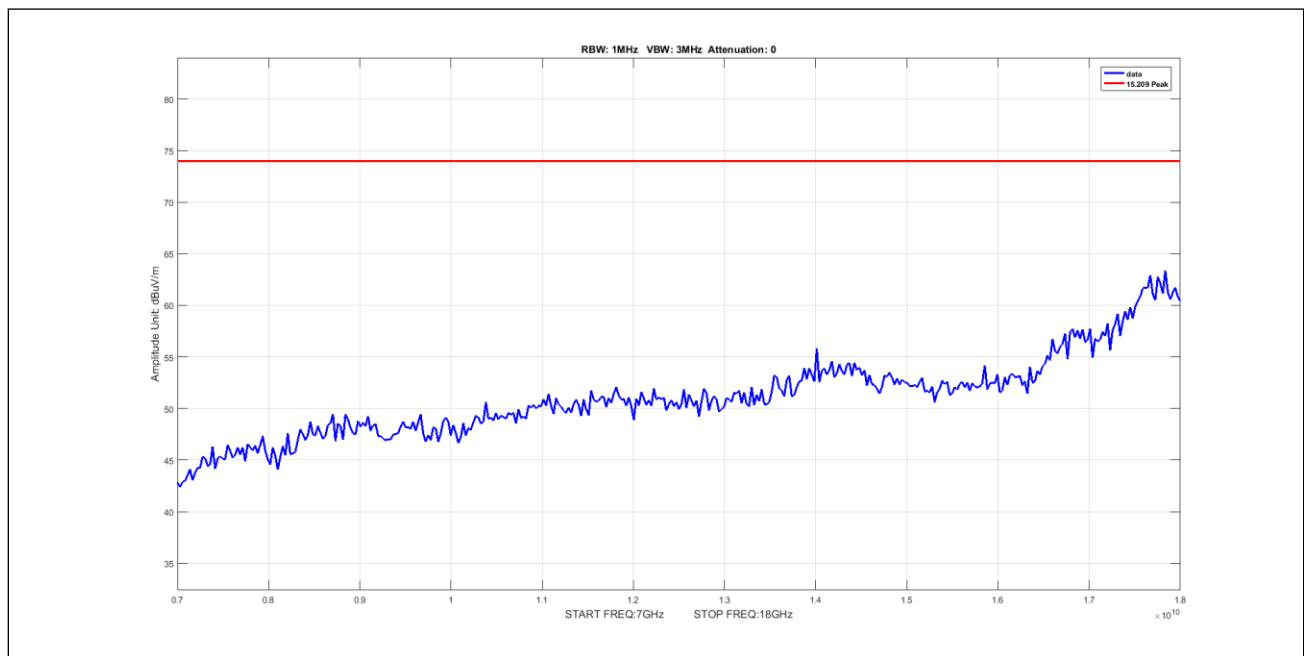
Plot 921. Undesirable Emissions, 5Omni, Peak, 7-18GHz, 10M, 5700, pow11
