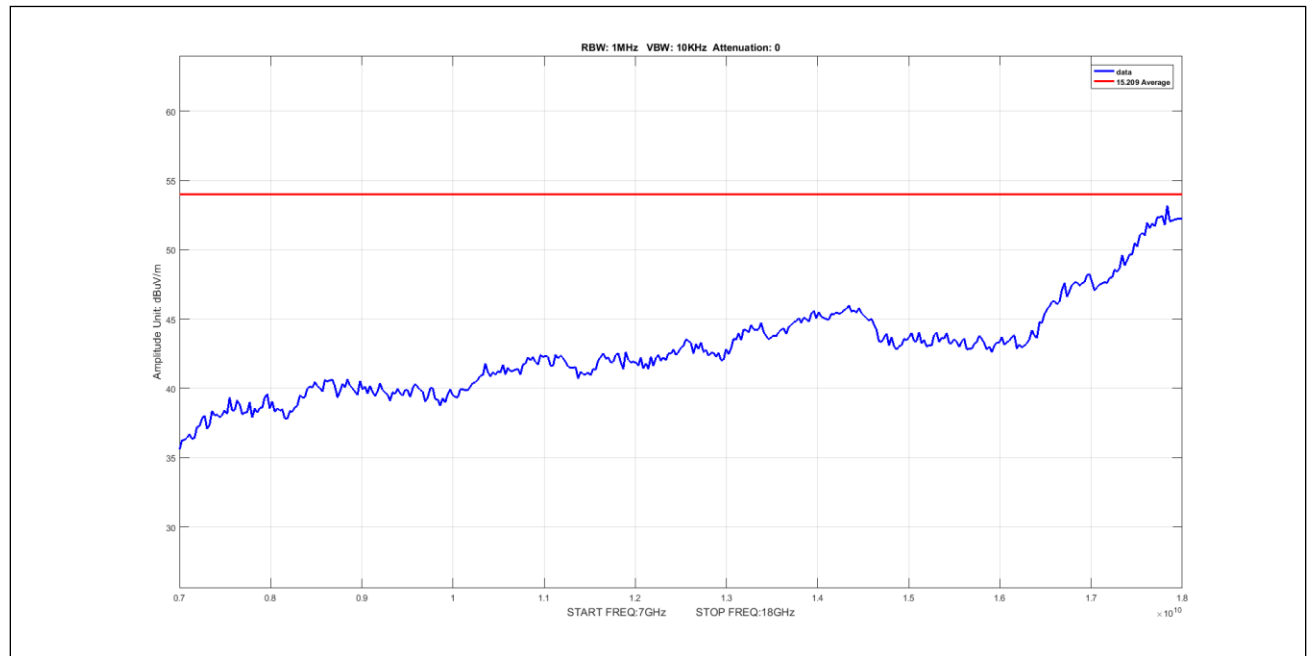
Plot 882. Undesirable Emissions, 50mni, Average, 7-18GHz, 40M, 5330, pow4
