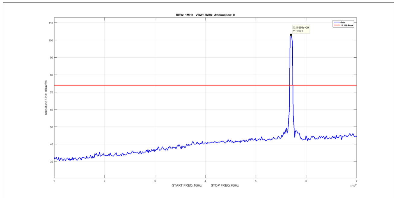
Plot 909. Undesirable Emissions, 50mni, Peak, 1-7GHz, 40M, 5700, pow7
