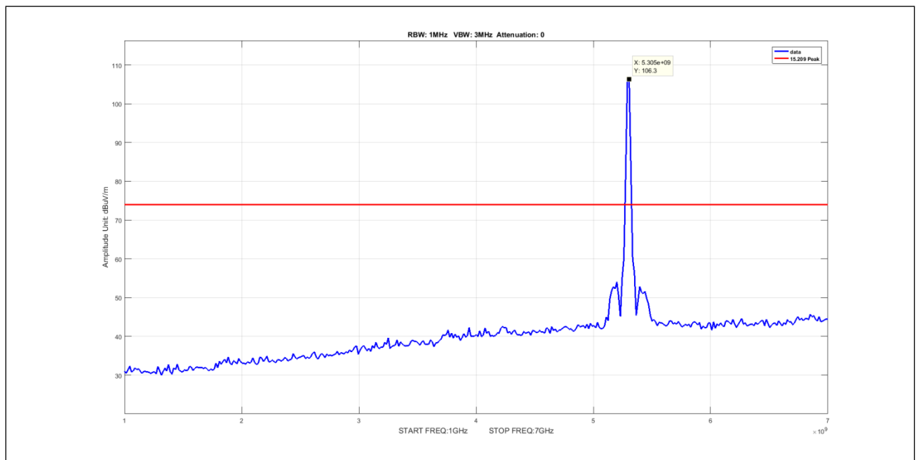
Plot 899. Undesirable Emissions, 5Omni, Peak, 1-7GHz, 20M, 5300, pow14
