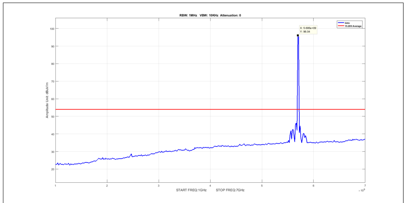
Plot 945. Undesirable Emissions, 8Omni, Average, 1-7GHz, 10M, 5700, pow8
