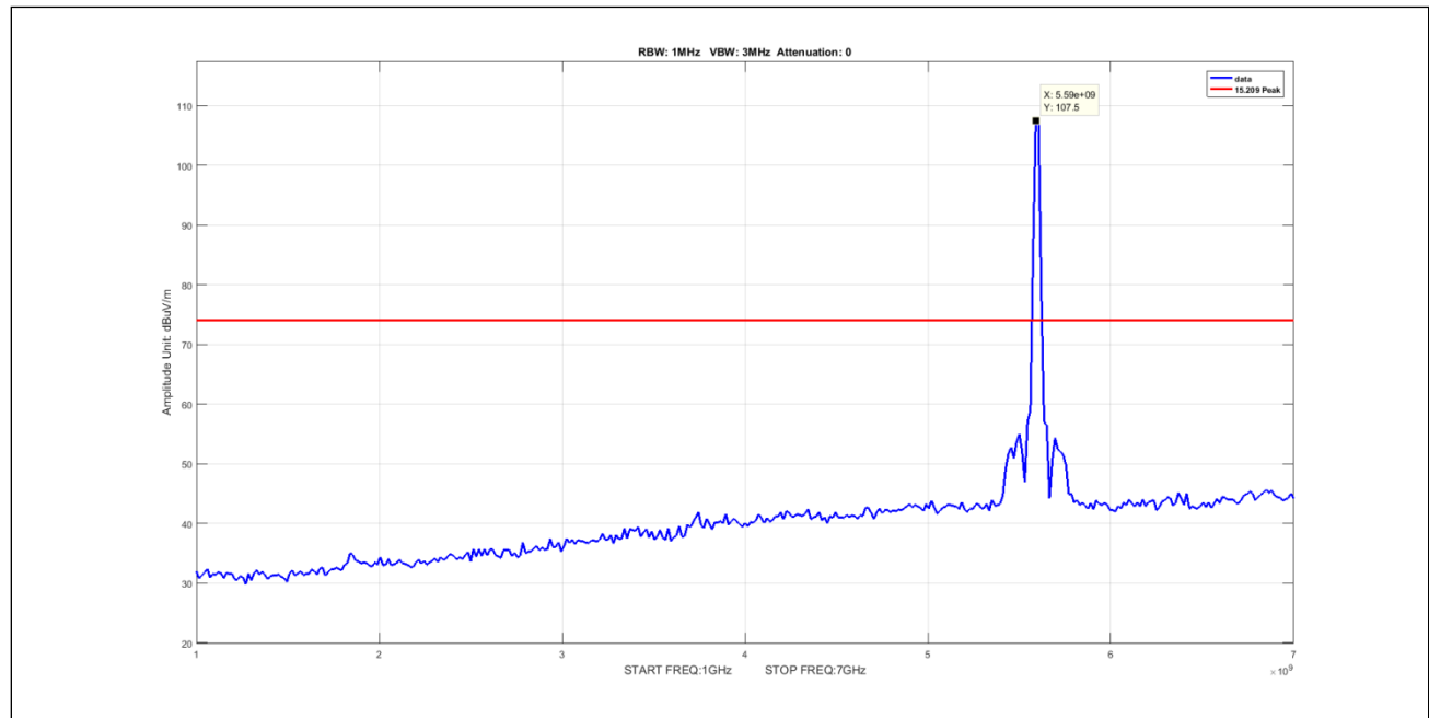
Plot 902. Undesirable Emissions, 5Omni, Peak, 1-7GHz, 20M, 5595, pow14
