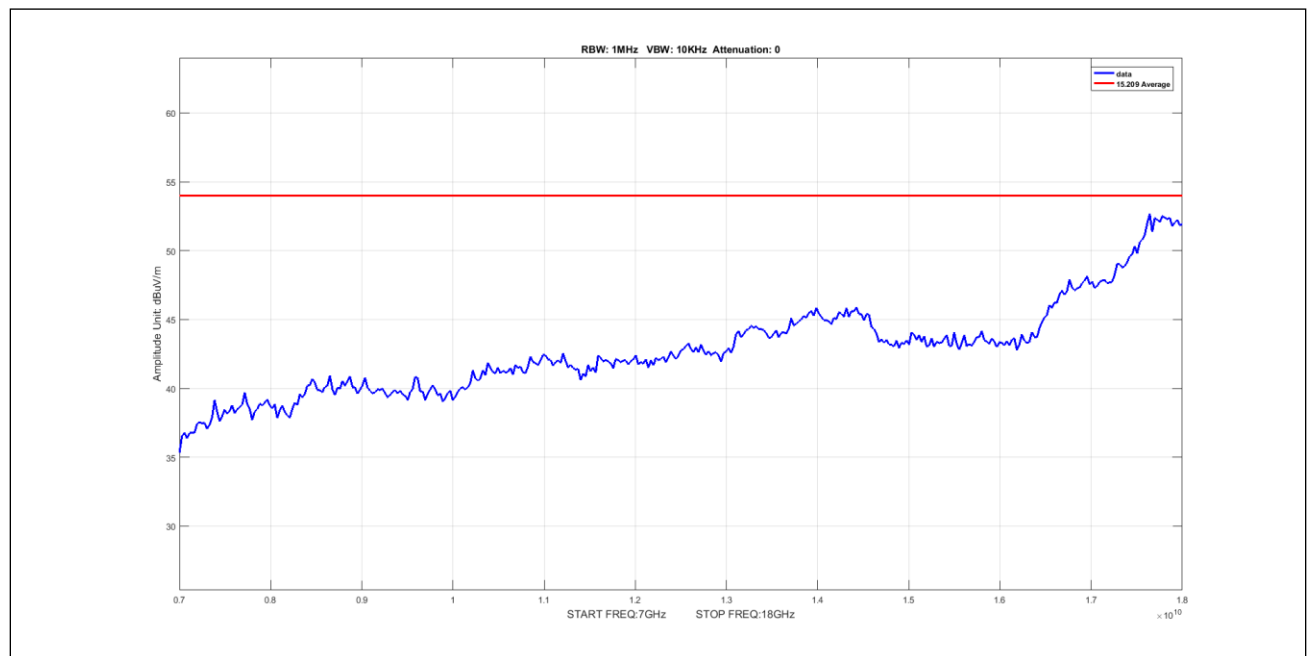
Plot 883. Undesirable Emissions, 50mni, Average, 7-18GHz, 40M, 5490, pow4
