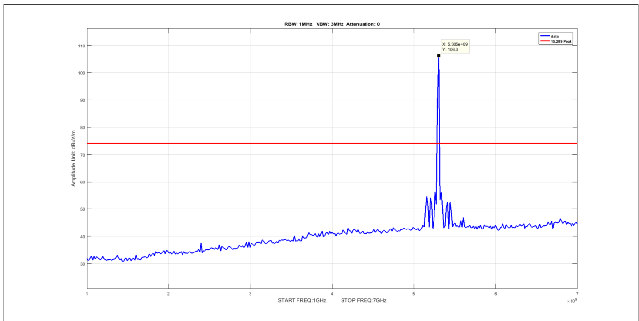
Plot 887. Undesirable Emissions, 5Omni, Peak, 1-7GHz, 5M, 5300, pow8
