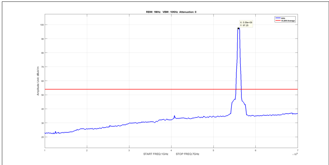
Plot 956. Undesirable Emissions, 8Omni, Average, 1-7GHz, 40M, 5595, pow17
