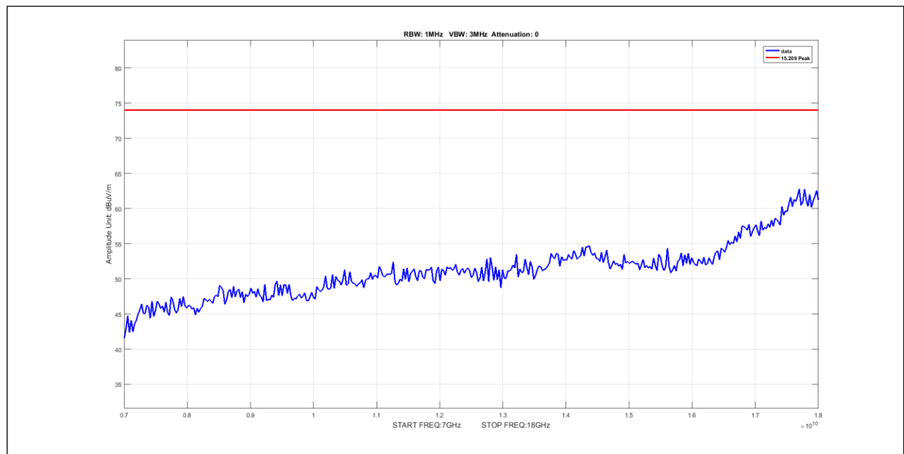
Plot 929. Undesirable Emissions, 5Omni, Peak, 7-18GHz, 40M, 5300, pow19
