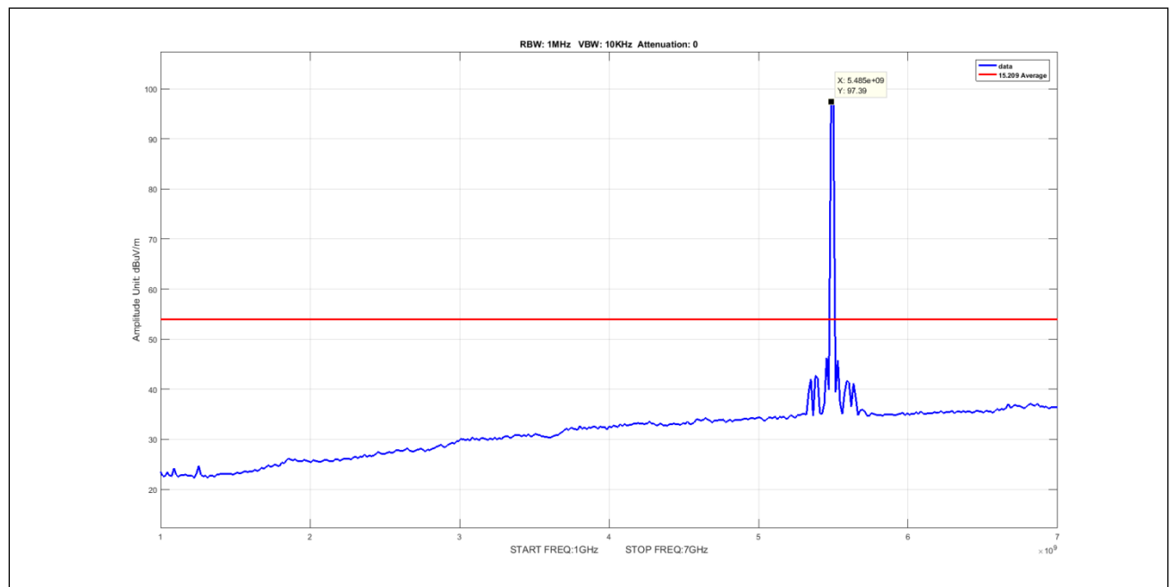
Plot 937. Undesirable Emissions, 8Omni, Average, 1-7GHz, 5M, 5490, pow6
