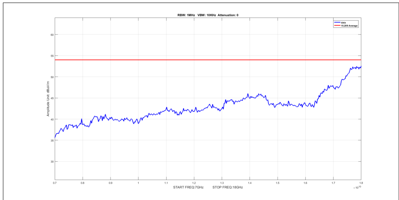
Plot 879. Undesirable Emissions, 50mni, Average, 7-18GHz, 20M, 5700, pow11
