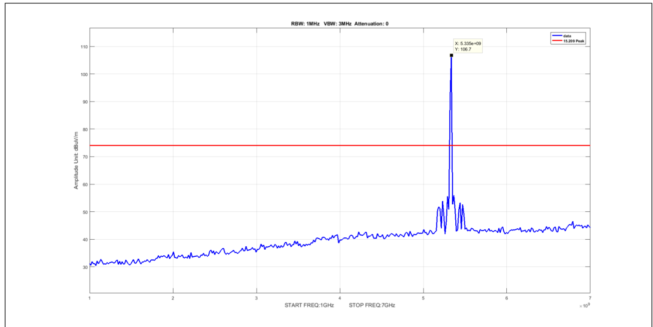
Plot 888. Undesirable Emissions, 5Omni, Peak, 1-7GHz, 5M, 5330, pow8
