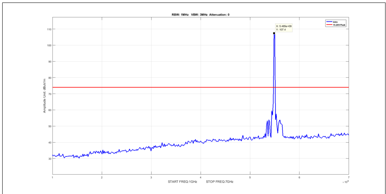
Plot 895. Undesirable Emissions, 50mni, Peak, 1-7GHz, 10M, 5490, pow12
