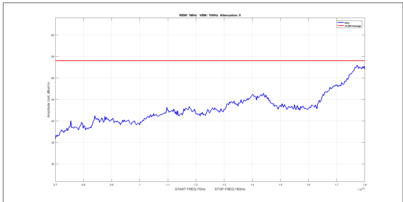
Plot 969. Undesirable Emissions, 8Omni, Average, 7-18GHz, 10M, 5700, pow8
