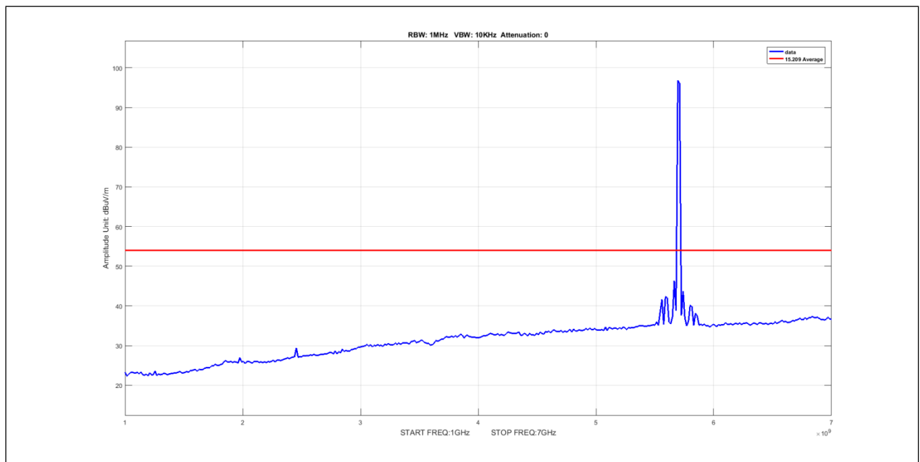
Plot 939. Undesirable Emissions, 8Omni, Average, 1-7GHz, 5M, 5700, pow6
