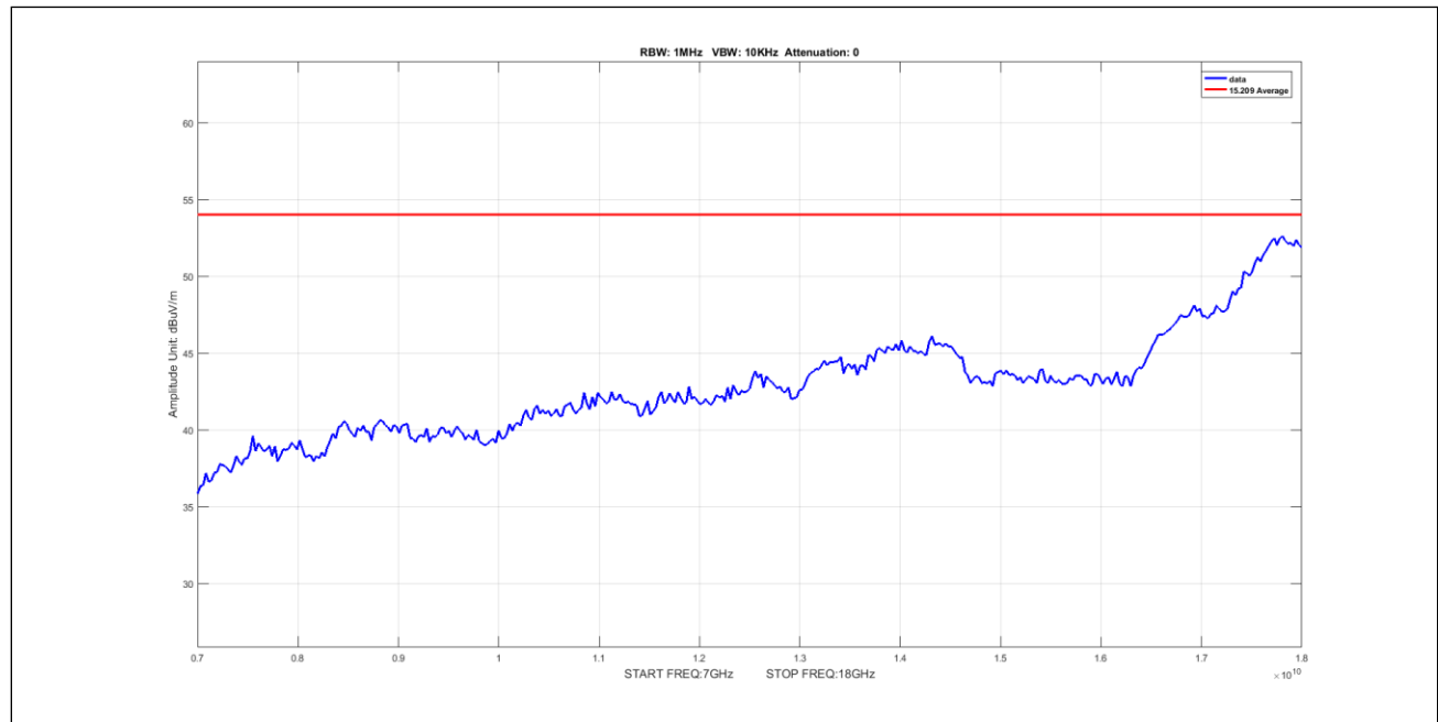
Plot 878. Undesirable Emissions, 50mni, Average, 7-18GHz, 20M, 5595, pow14
