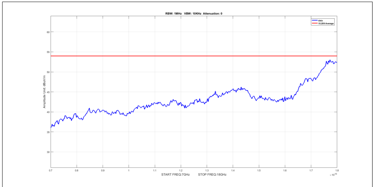
Plot 964. Undesirable Emissions, 8Omni, Average, 7-18GHz, 10M, 5255, pow9
