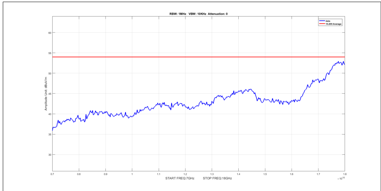
Plot 968. Undesirable Emissions, 8Omni, Average, 7-18GHz, 10M, 5595, pow9
