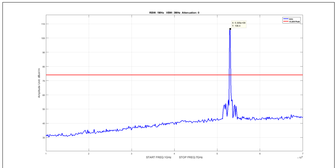
Plot 893. Undesirable Emissions, 5Omni, Peak, 1-7GHz, 10M, 5300, pow11
