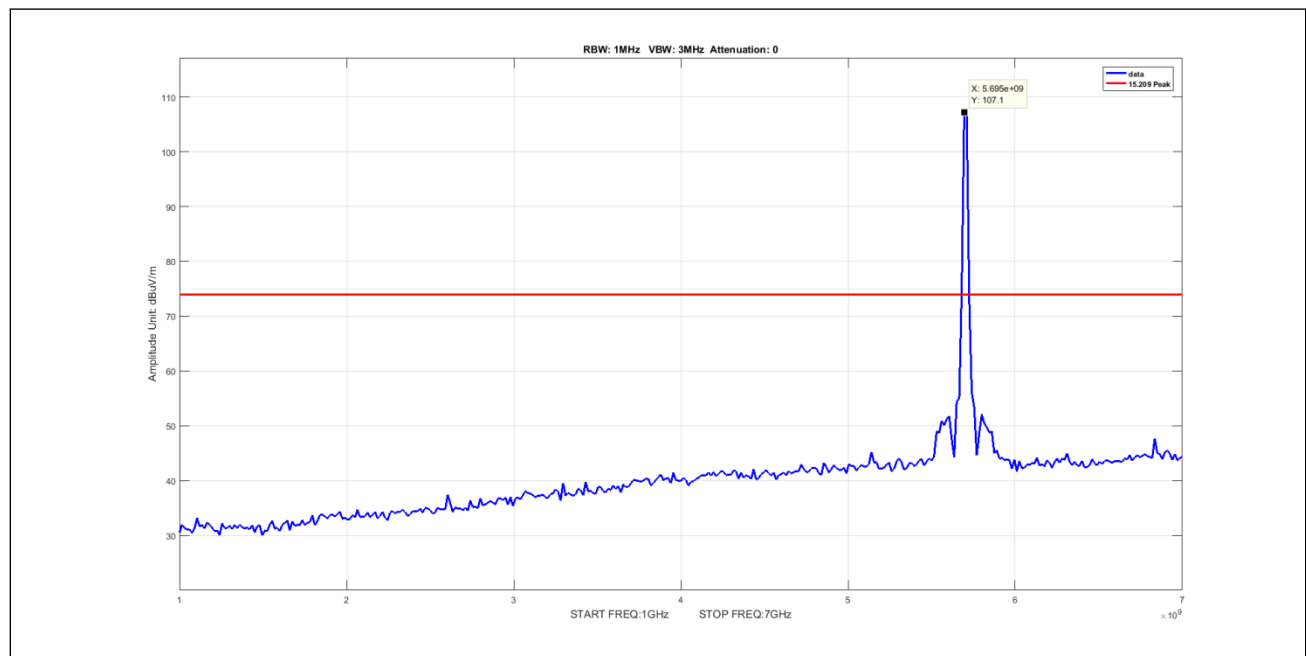
Plot 903. Undesirable Emissions, 5Omni, Peak, 1-7GHz, 20M, 5700, pow11
