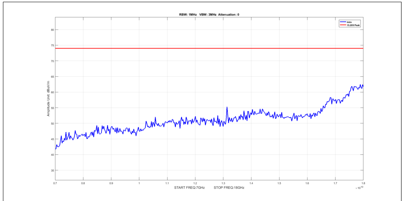
Plot 916. Undesirable Emissions, 5Omni, Peak, 7-18GHz, 10M, 5255, pow11
