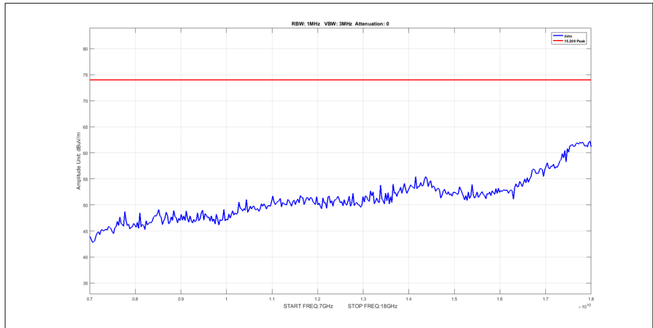
Plot 914. Undesirable Emissions, 5Omni, Peak, 7-18GHz, 5M, 5595, pow8
