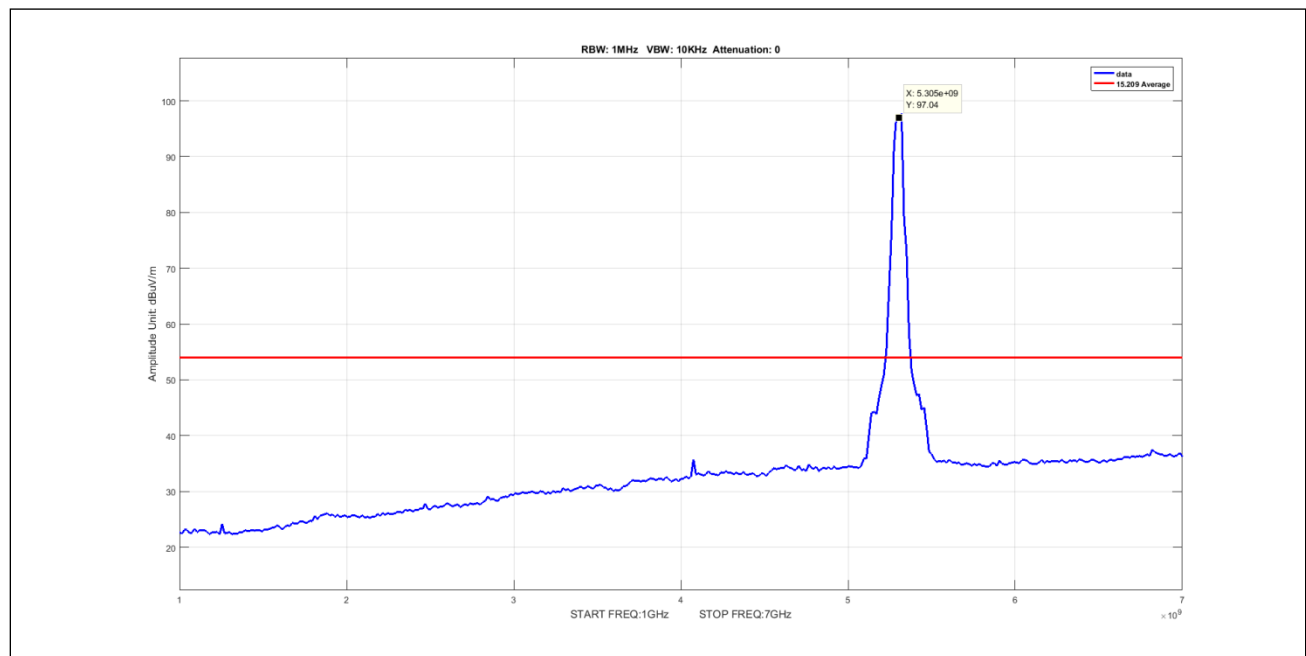
Plot 953. Undesirable Emissions, 8Omni, Average, 1-7GHz, 40M, 5300, pow18
