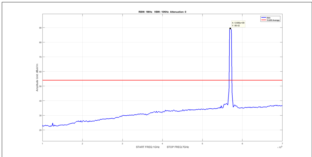
Plot 957. Undesirable Emissions, 8Omni, Average, 1-7GHz, 40M, 5700, pow6
