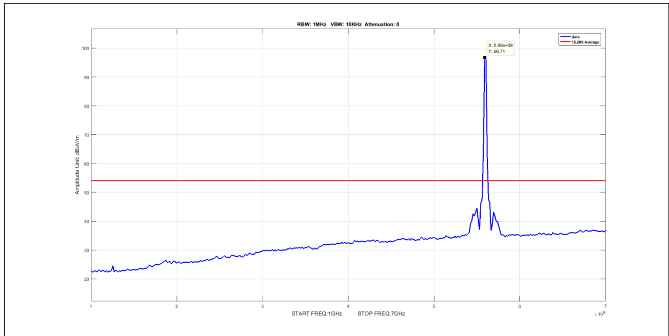
Plot 950. Undesirable Emissions, 8Omni, Average, 1-7GHz, 20M, 5595, pow12
