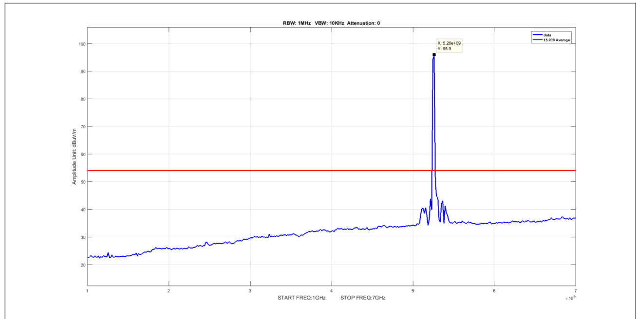
Plot 940. Undesirable Emissions, 8Omni, Average, 1-7GHz, 10M, 5255, pow9
