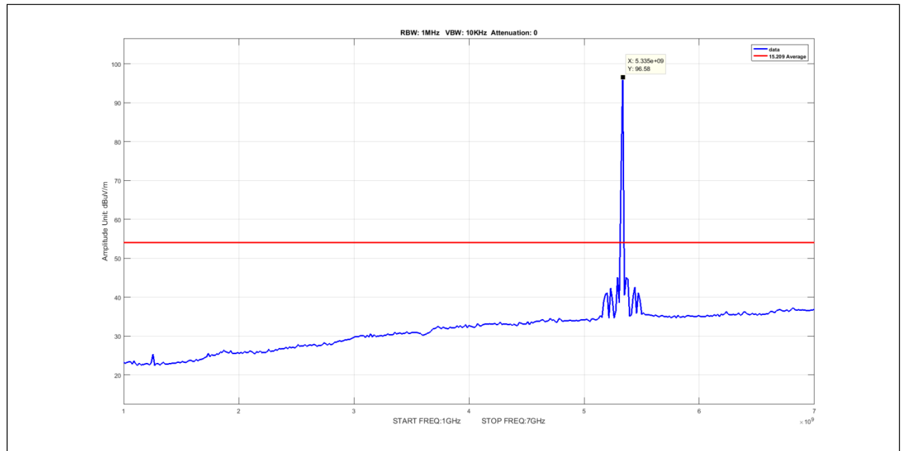
Plot 936. Undesirable Emissions, 8Omni, Average, 1-7GHz, 5M, 5330, pow6
