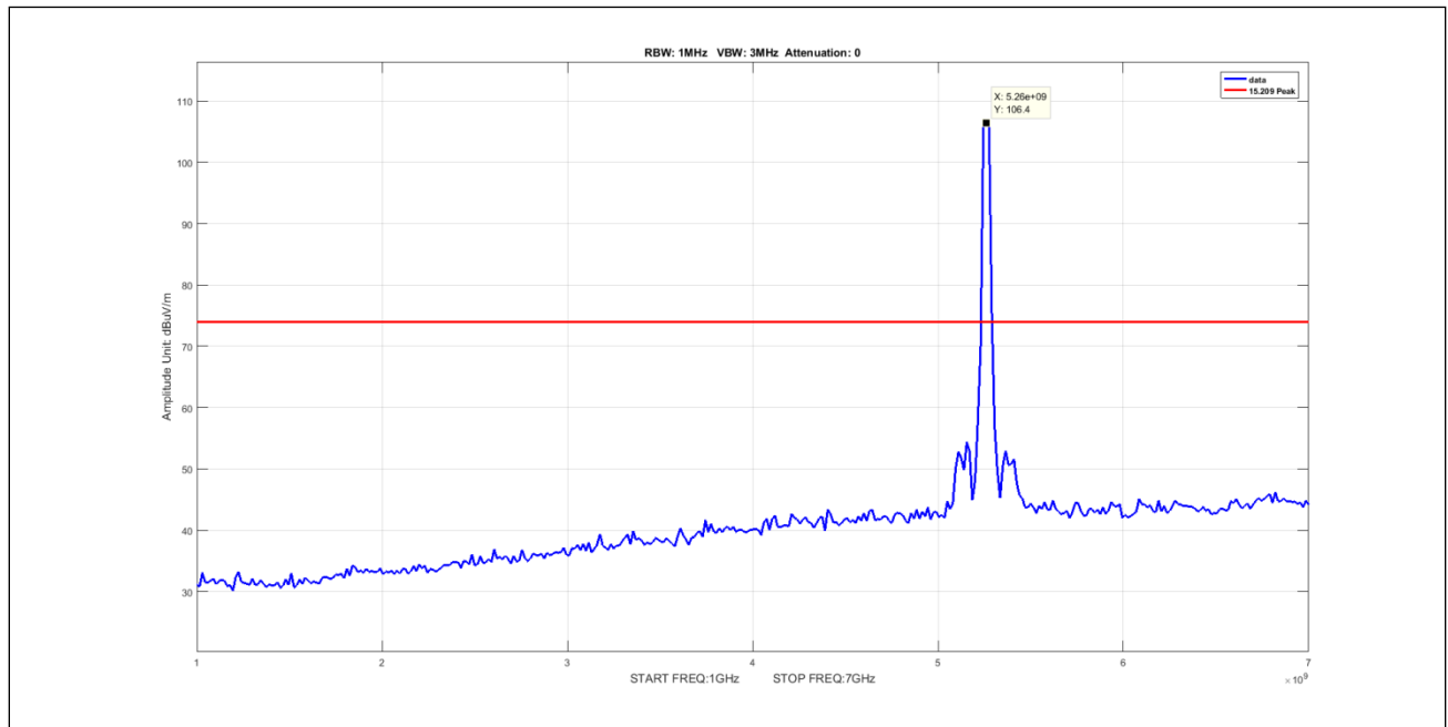
Plot 898. Undesirable Emissions, 5Omni, Peak, 1-7GHz, 20M, 5260, pow14
