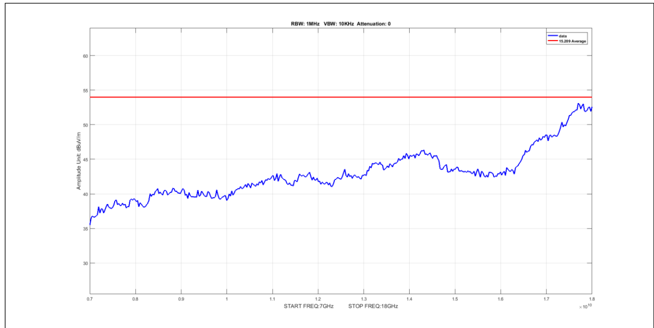
Plot 962. Undesirable Emissions, 8Omni, Average, 7-18GHz, 5M, 5595, pow6
