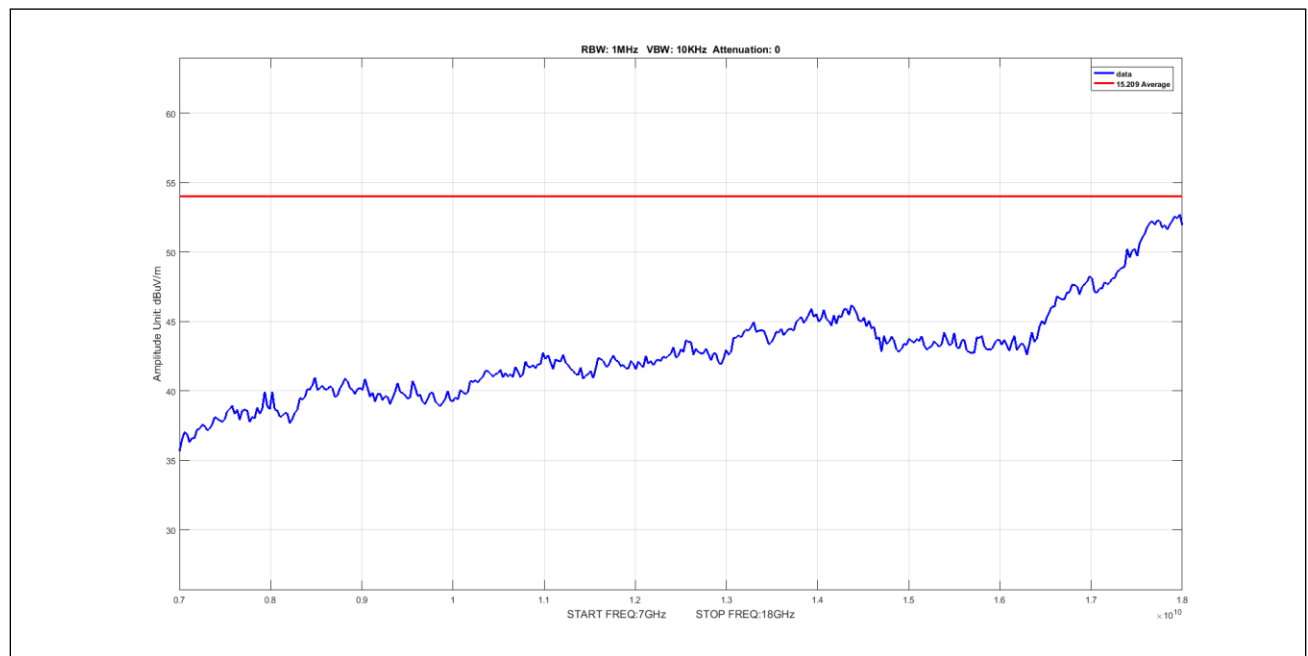
Plot 885. Undesirable Emissions, 50mni, Average, 7-18GHz, 40M, 5700, pow7
