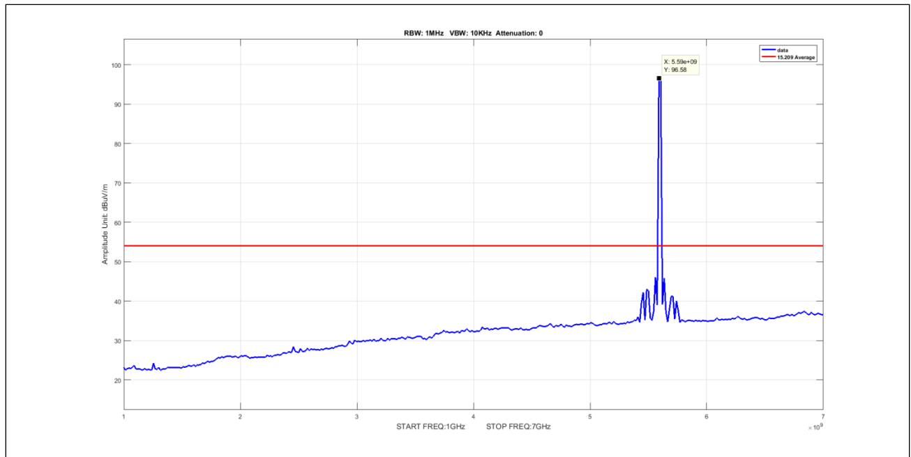
Plot 938. Undesirable Emissions, 8Omni, Average, 1-7GHz, 5M, 5595, pow6
