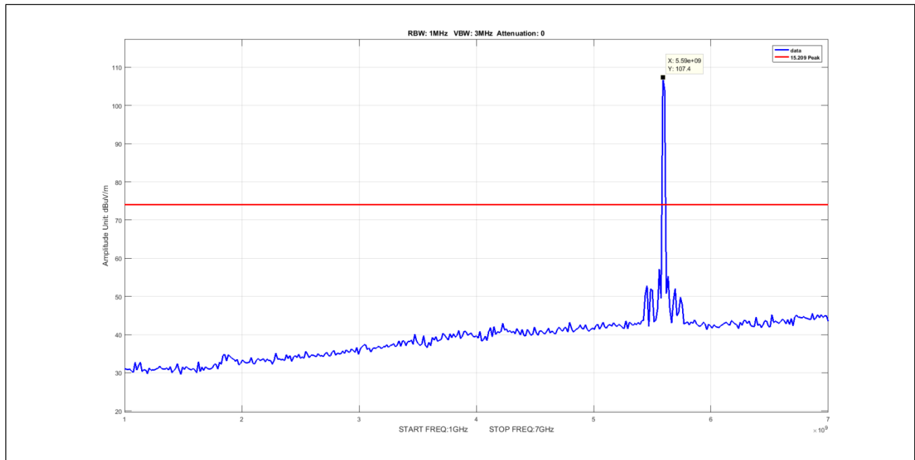
Plot 890. Undesirable Emissions, 50mni, Peak, 1-7GHz, 5M, 5595, pow8
