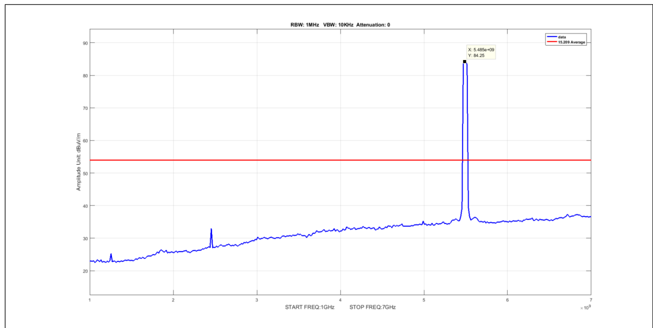
Plot 955. Undesirable Emissions, 8Omni, Average, 1-7GHz, 40M, 5490, pow1
