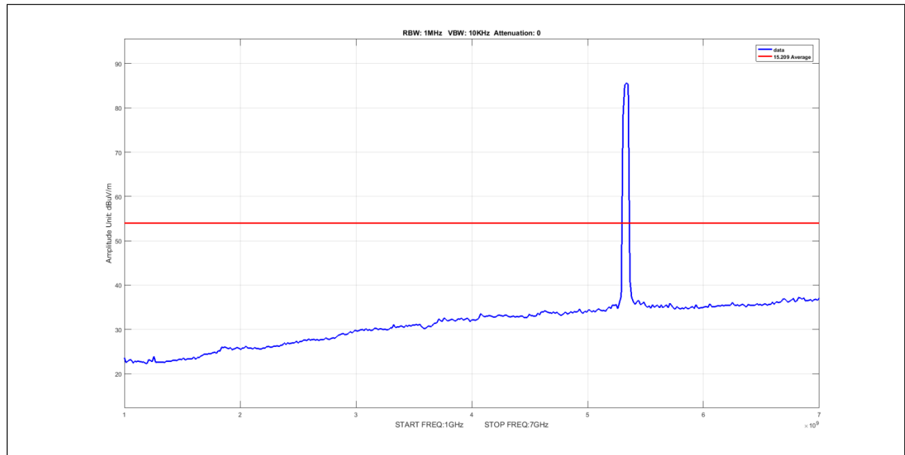
Plot 954. Undesirable Emissions, 8Omni, Average, 1-7GHz, 40M, 5330, pow1
