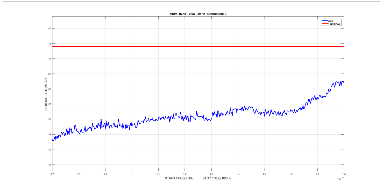
Plot 926. Undesirable Emissions, 5Omni, Peak, 7-18GHz, 20M, 5595, pow14
