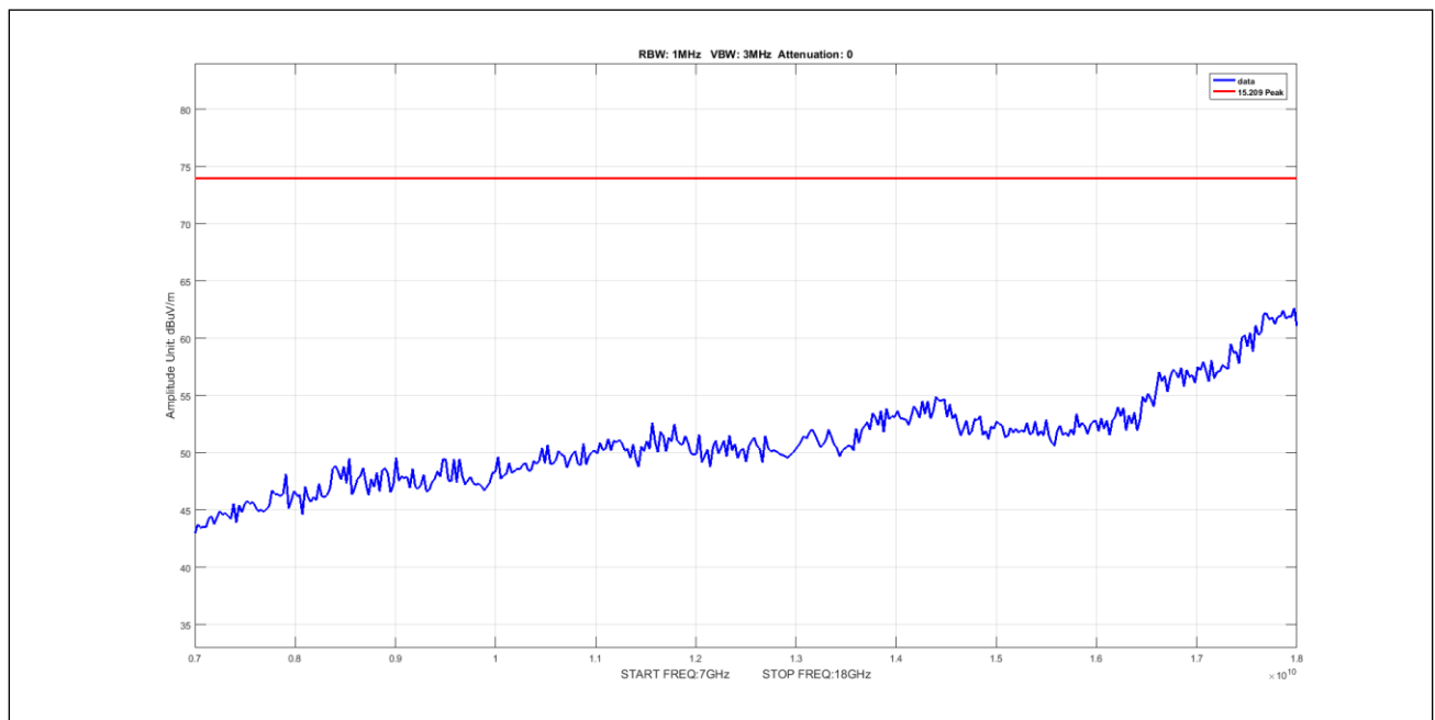
Plot 919. Undesirable Emissions, 5Omni, Peak, 7-18GHz, 10M, 5490, pow12
