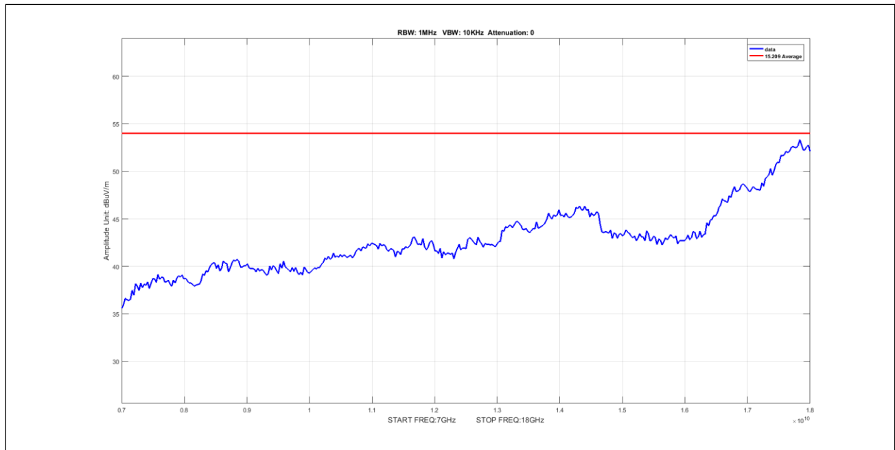
Plot 970. Undesirable Emissions, 8Omni, Average, 7-18GHz, 20M, 5260, pow12
