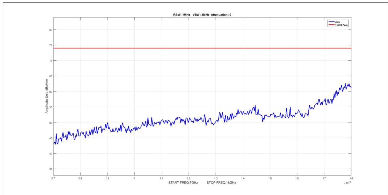
Plot 915. Undesirable Emissions, 5Omni, Peak, 7-18GHz, 5M, 5700, pow8
