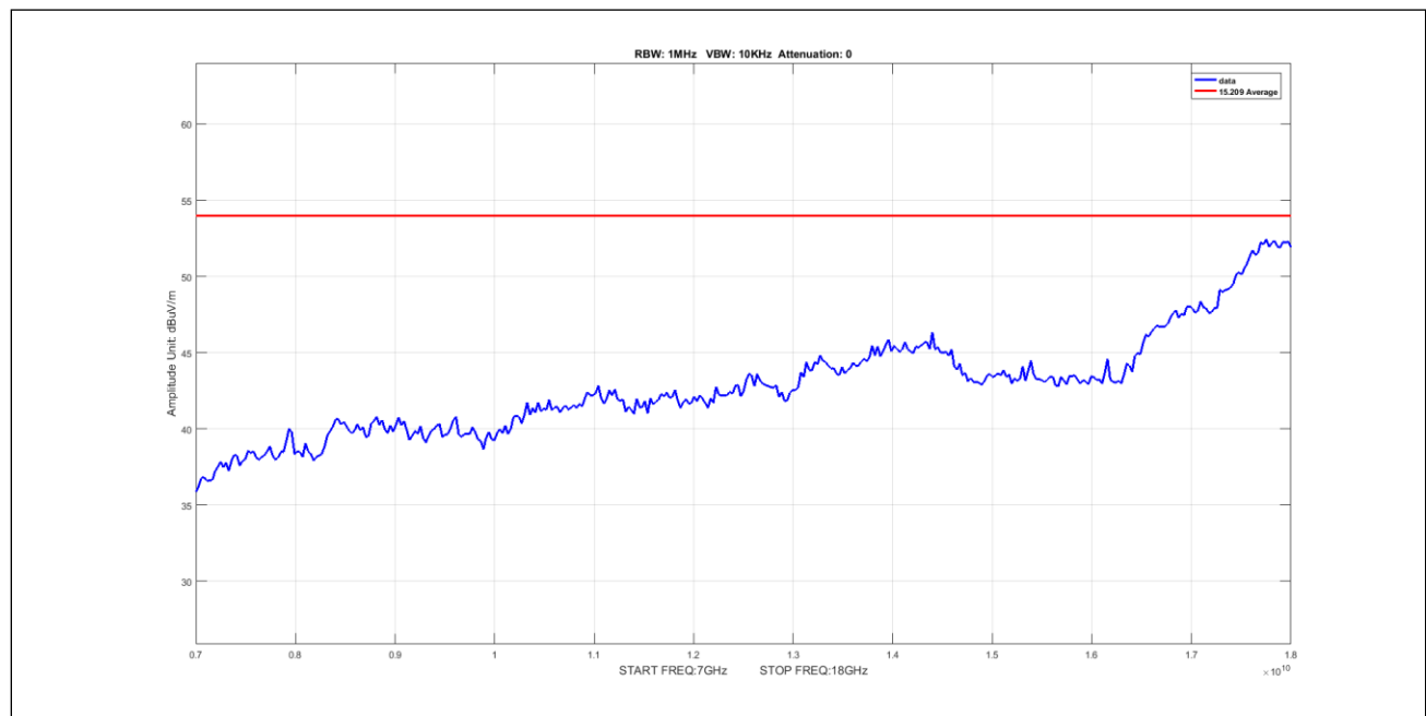
Plot 881. Undesirable Emissions, 5Omni, Average, 7-18GHz, 40M, 5300, pow19
