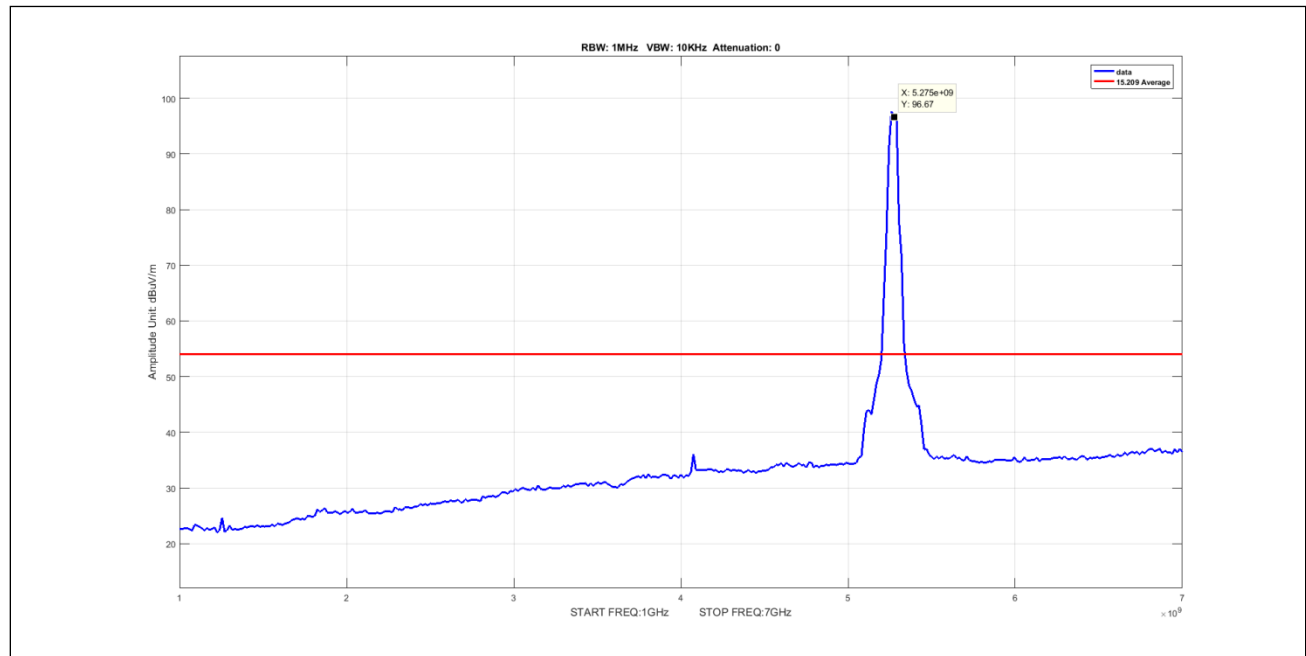
Plot 952. Undesirable Emissions, 8Omni, Average, 1-7GHz, 40M, 5270, pow18
