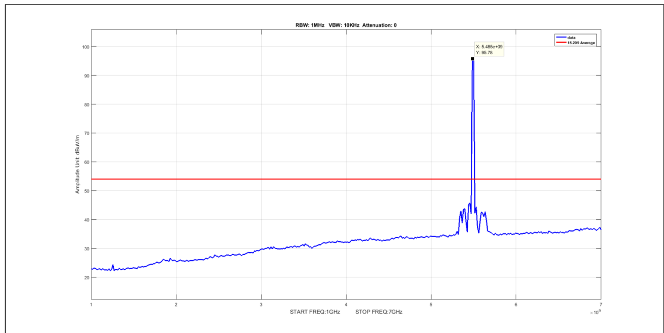
Plot 943. Undesirable Emissions, 8Omni, Average, 1-7GHz, 10M, 5490, pow10
