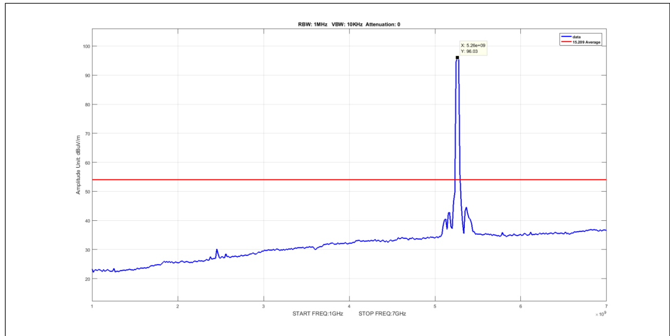
Plot 946. Undesirable Emissions, 8Omni, Average, 1-7GHz, 20M, 5260, pow12
