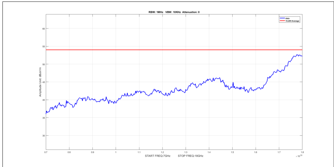
Plot 972. Undesirable Emissions, 8Omni, Average, 7-18GHz, 20M, 5330, pow10
