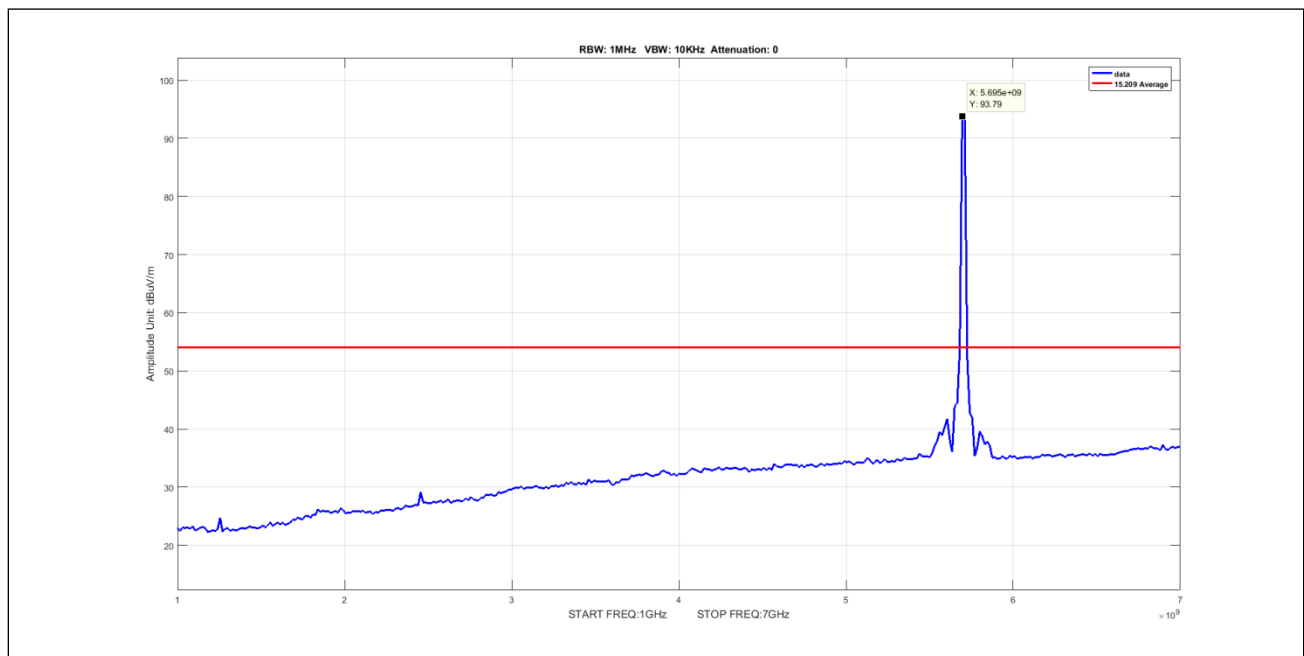
Plot 951. Undesirable Emissions, 8Omni, Average, 1-7GHz, 20M, 5700, pow8
