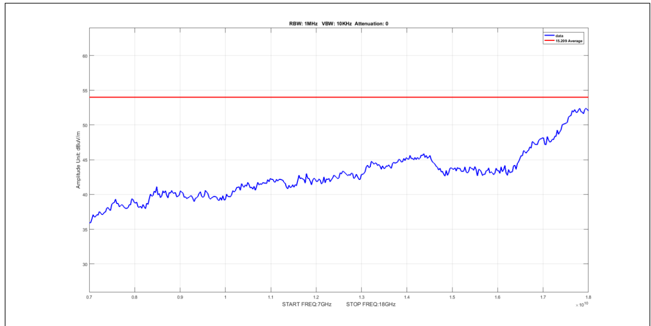
Plot 884. Undesirable Emissions, 50mni, Average, 7-18GHz, 40M, 5595, pow19
