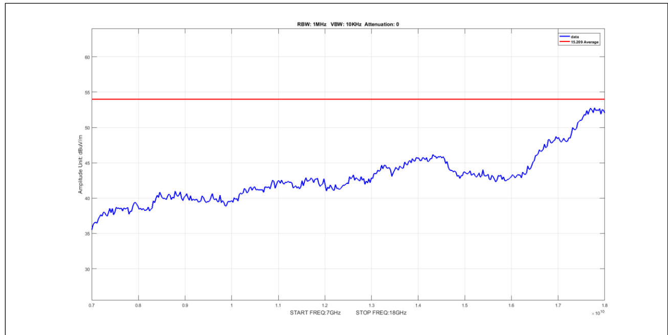
Plot 966. Undesirable Emissions, 8Omni, Average, 7-18GHz, 10M, 5330, pow9
