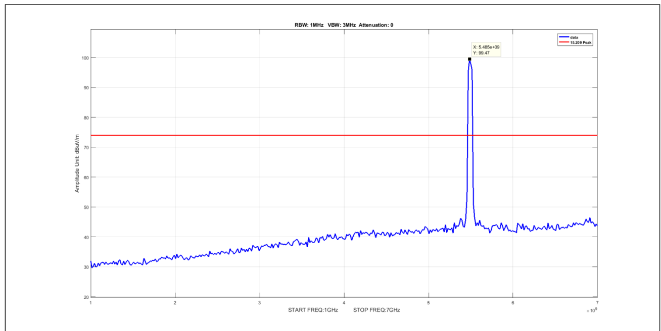
Plot 907. Undesirable Emissions, 50mni, Peak, 1-7GHz, 40M, 5490, pow4
