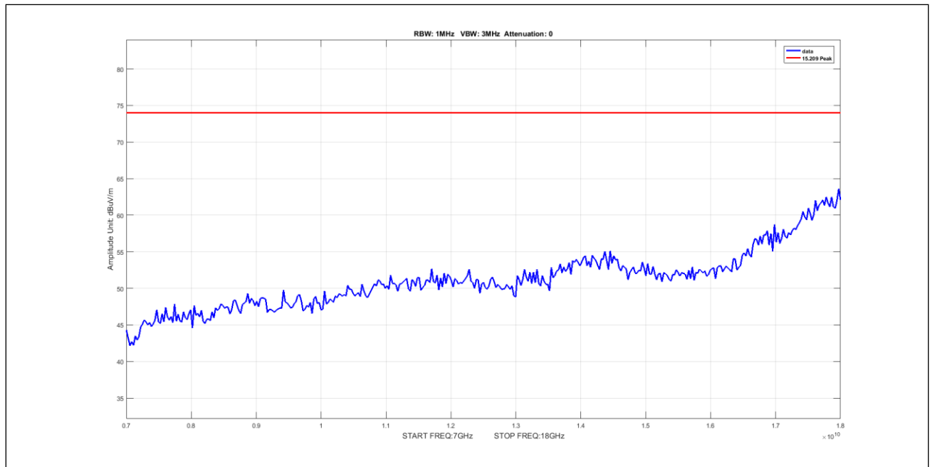
Plot 932. Undesirable Emissions, 5Omni, Peak, 7-18GHz, 40M, 5595, pow19
