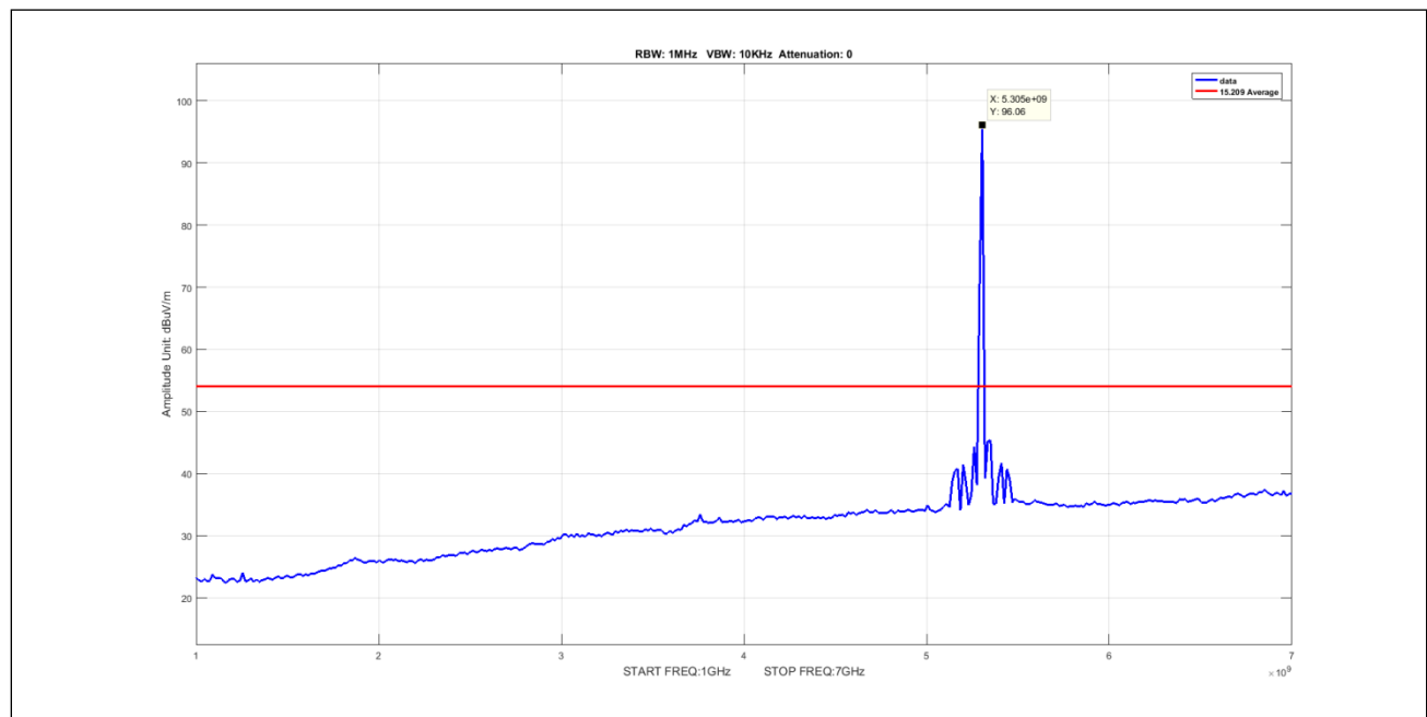
Plot 935. Undesirable Emissions, 8Omni, Average, 1-7GHz, 5M, 5300, pow6
