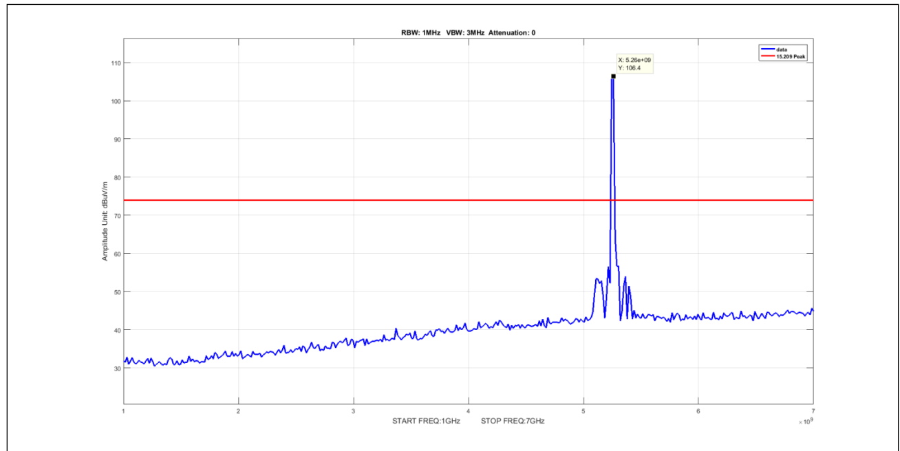
Plot 892. Undesirable Emissions, 5Omni, Peak, 1-7GHz, 10M, 5255, pow11
