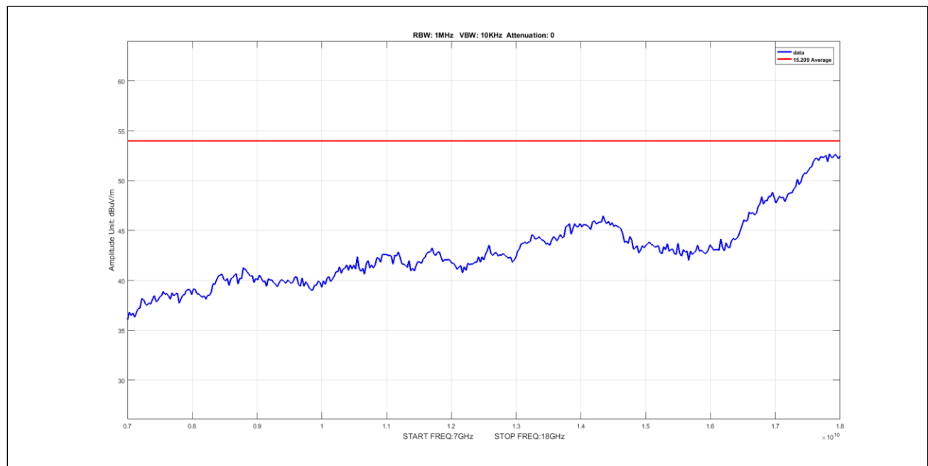
Plot 963. Undesirable Emissions, 8Omni, Average, 7-18GHz, 5M, 5700, pow6
