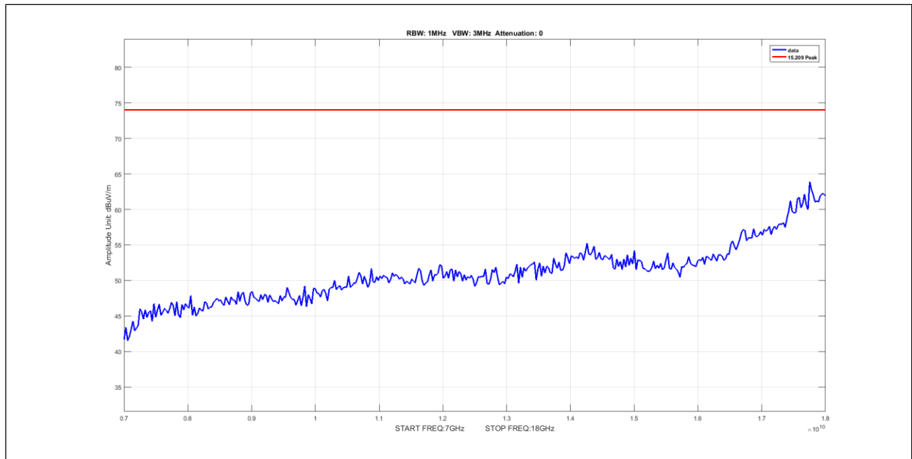
Plot 910. Undesirable Emissions, 50mni, Peak, 7-18GHz, 5M, 5252.5, pow8
