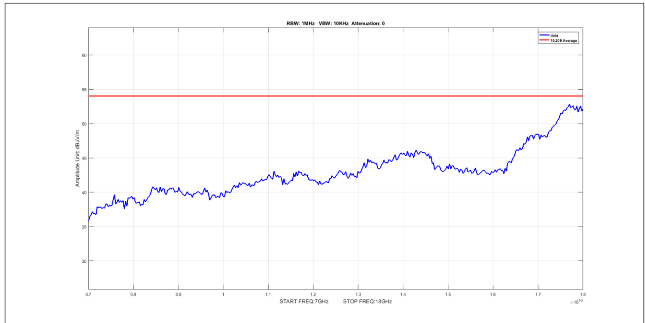
Plot 958. Undesirable Emissions, 8Omni, Average, 7-18GHz, 5M, 5252.5, pow6
