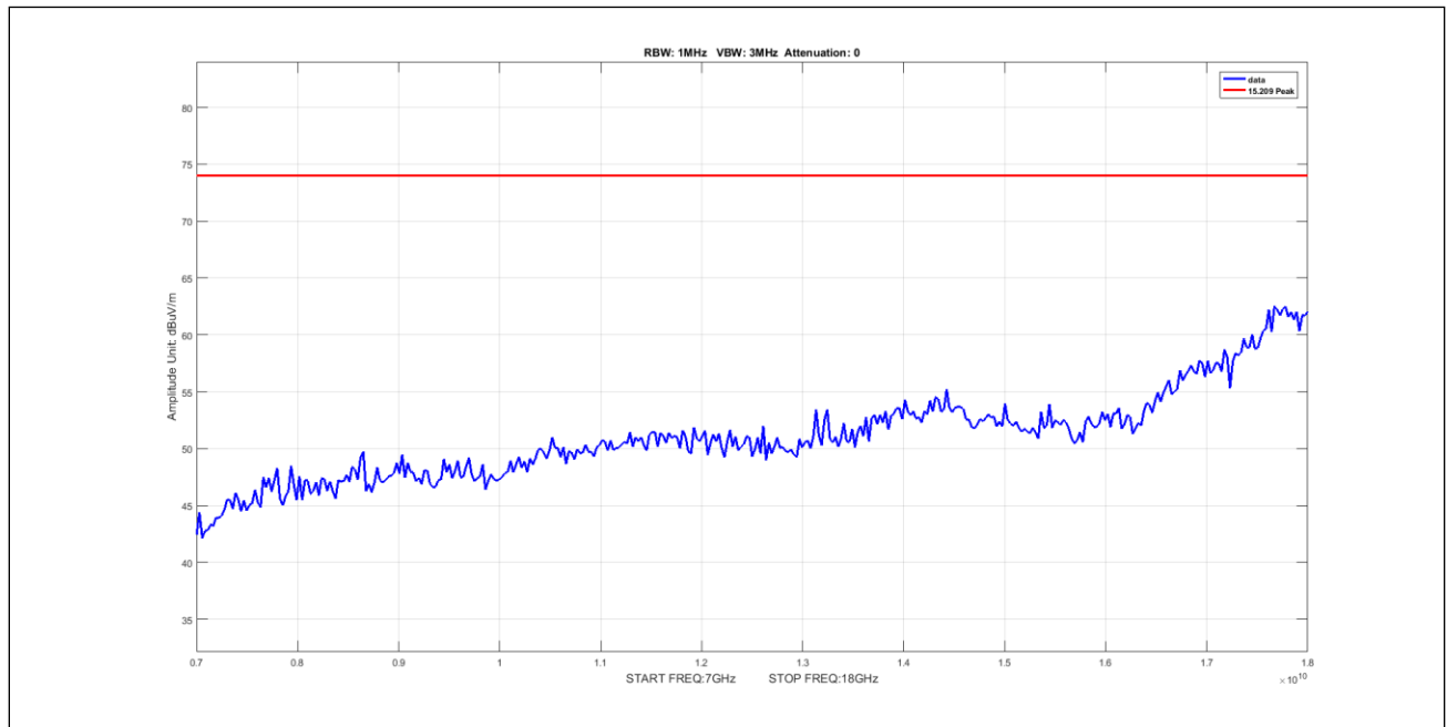
Plot 922. Undesirable Emissions, 5Omni, Peak, 7-18GHz, 20M, 5260, pow14
