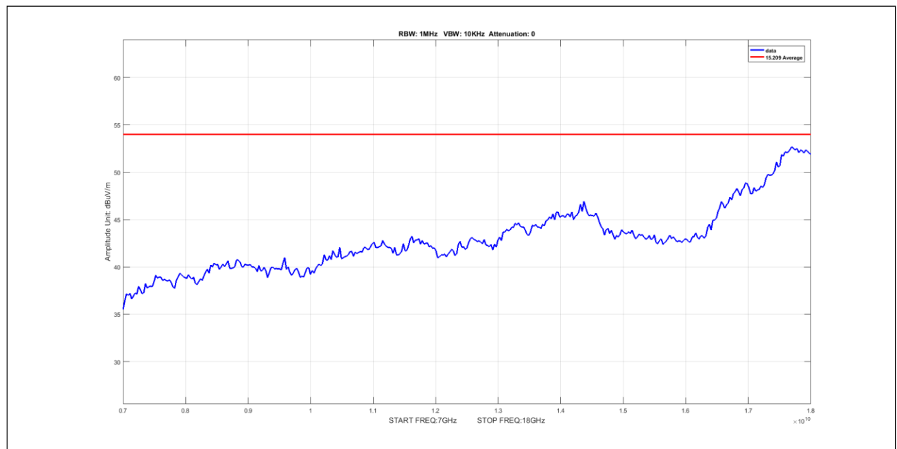
Plot 959. Undesirable Emissions, 8Omni, Average, 7-18GHz, 5M, 5300, pow6
