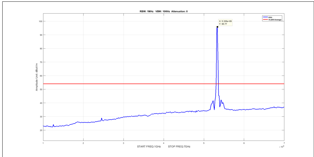
Plot 948. Undesirable Emissions, 8Omni, Average, 1-7GHz, 20M, 5330, pow10
