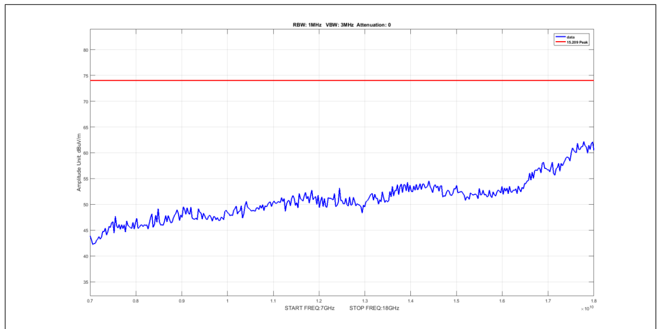
Plot 917. Undesirable Emissions, 5Omni, Peak, 7-18GHz, 10M, 5300, pow11
