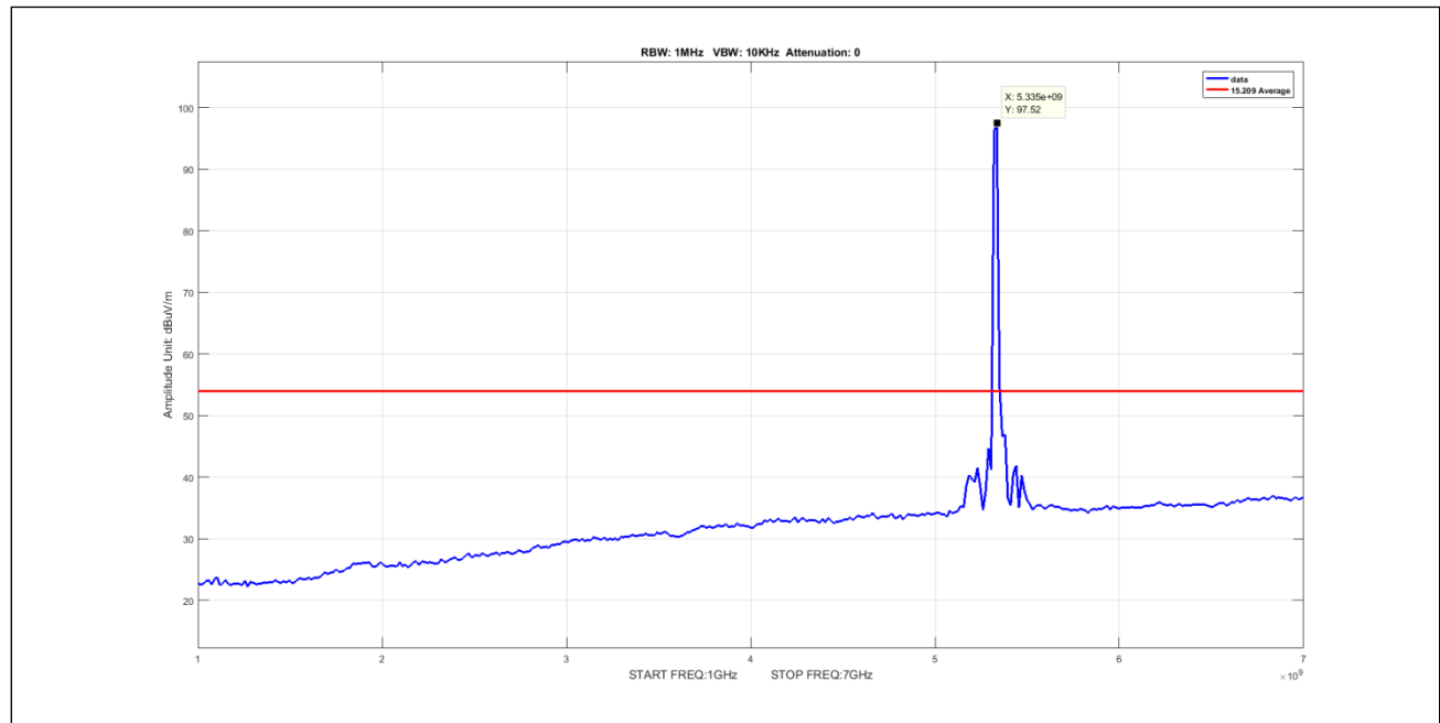
Plot 942. Undesirable Emissions, 8Omni, Average, 1-7GHz, 10M, 5330, pow9
