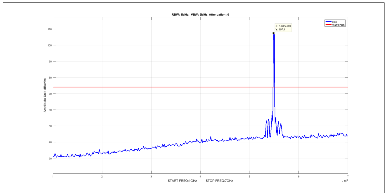
Plot 889. Undesirable Emissions, 5Omni, Peak, 1-7GHz, 5M, 5490, pow9
