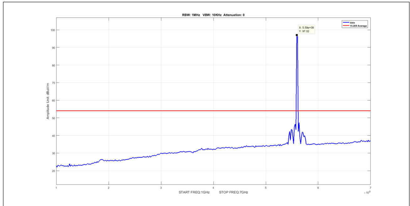
Plot 944. Undesirable Emissions, 8Omni, Average, 1-7GHz, 10M, 5595, pow9
