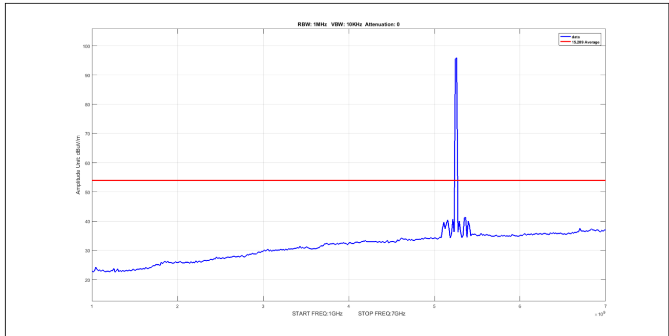
Plot 934. Undesirable Emissions, 8Omni, Average, 1-7GHz, 5M, 5252.5, pow6
