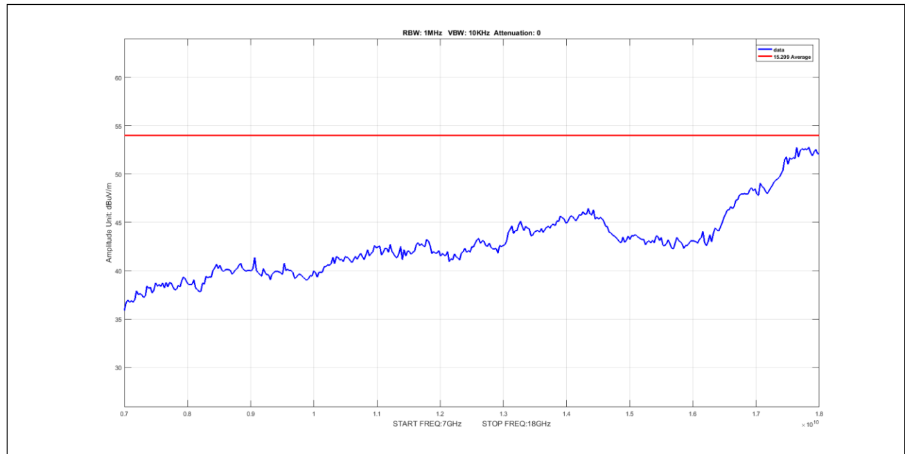
Plot 974. Undesirable Emissions, 8Omni, Average, 7-18GHz, 20M, 5595, pow12
