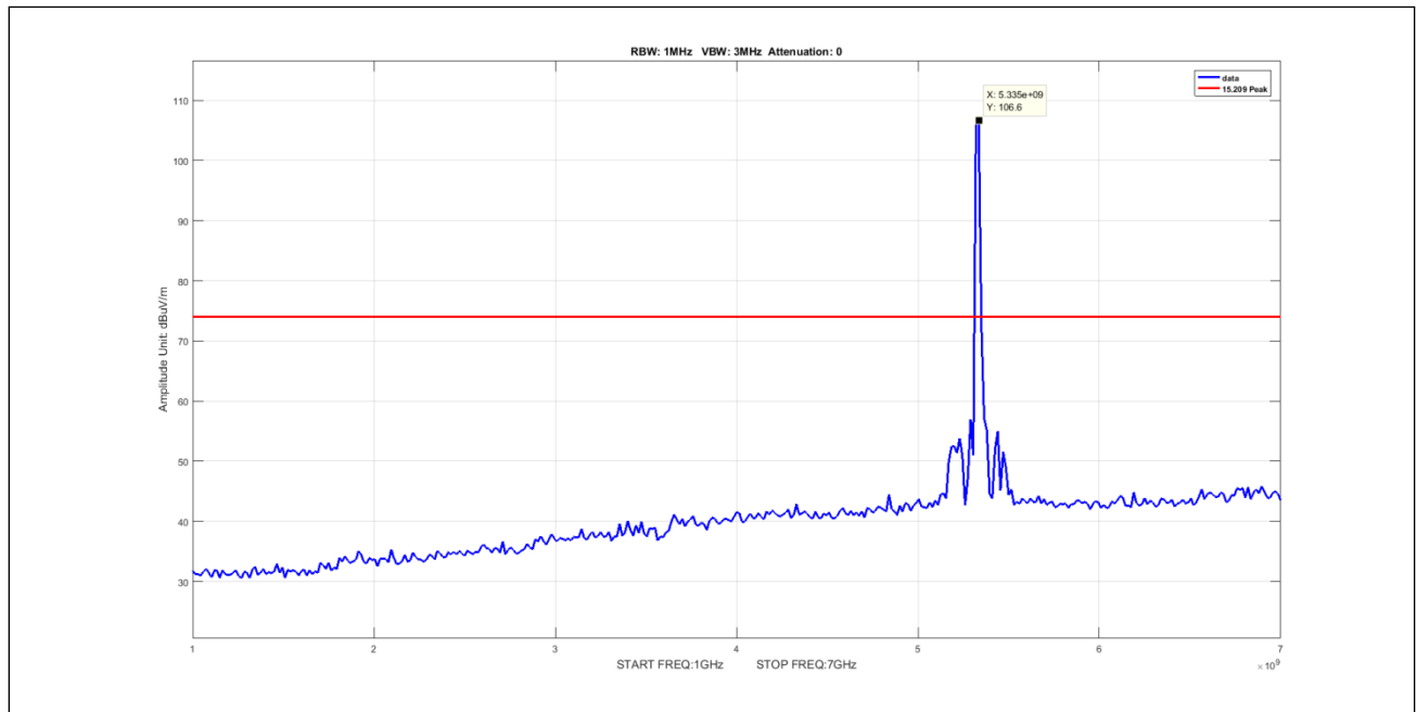
Plot 894. Undesirable Emissions, 50mni, Peak, 1-7GHz, 10M, 5330, pow11
