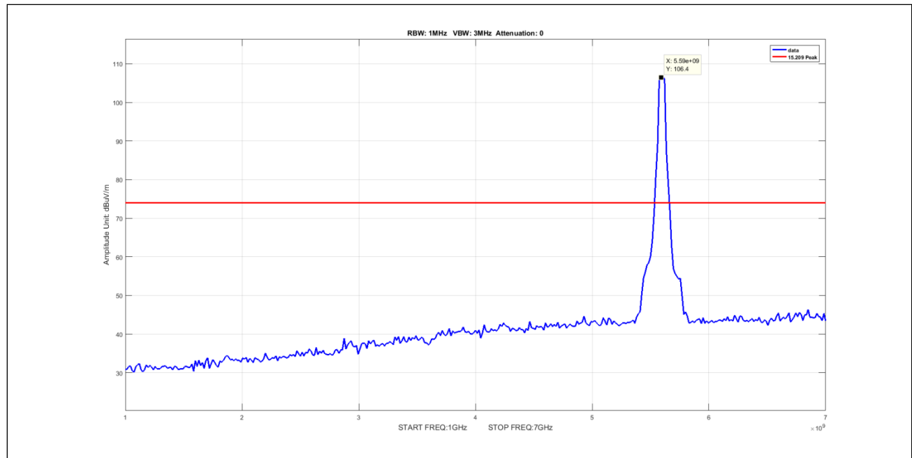
Plot 908. Undesirable Emissions, 50mni, Peak, 1-7GHz, 40M, 5595, pow19
