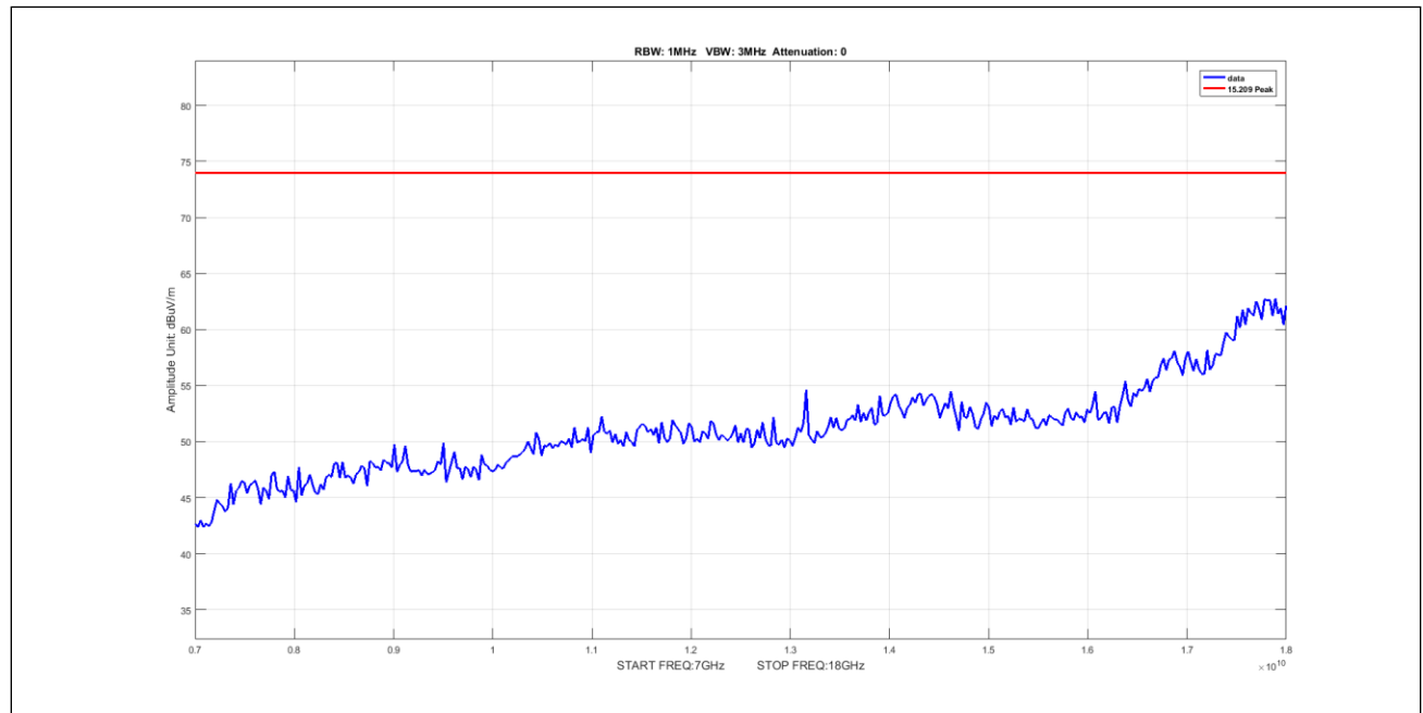
Plot 930. Undesirable Emissions, 5Omni, Peak, 7-18GHz, 40M, 5330, pow4
