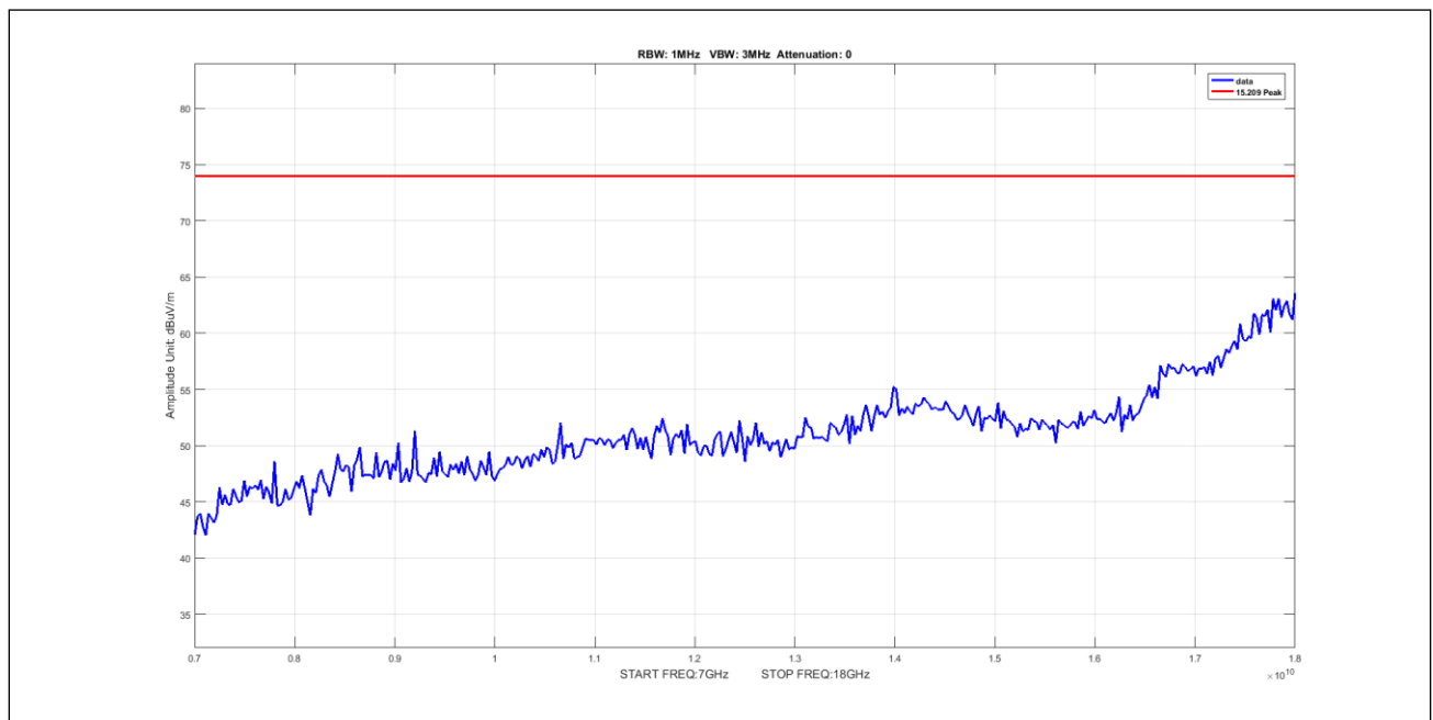
Plot 913. Undesirable Emissions, 5Omni, Peak, 7-18GHz, 5M, 5490, pow9
