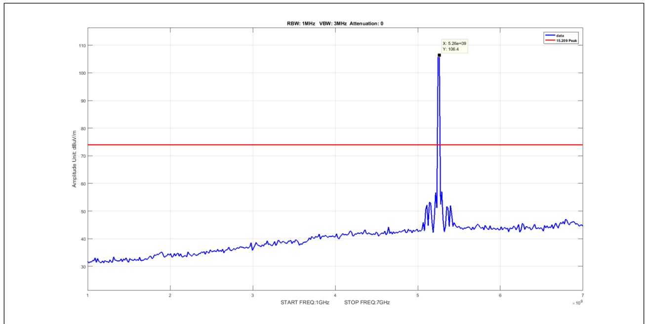
Plot 886. Undesirable Emissions, 5Omni, Peak, 1-7GHz, 5M, 5252.5, pow8
