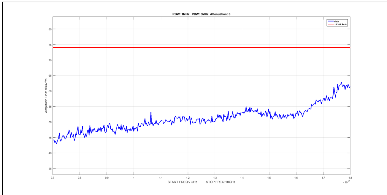
Plot 920. Undesirable Emissions, 5Omni, Peak, 7-18GHz, 10M, 5595, pow11
