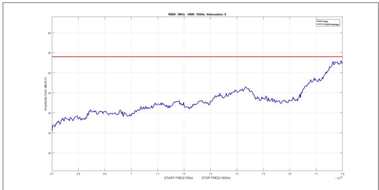
Plot 961. Undesirable Emissions, 8Omni, Average, 7-18GHz, 5M, 5490, pow6
