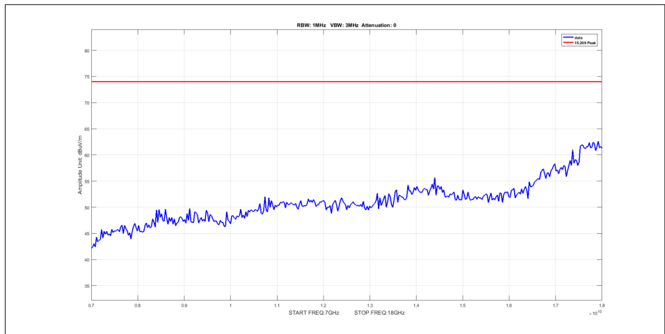
Plot 927. Undesirable Emissions, 5Omni, Peak, 7-18GHz, 20M, 5700, pow11
