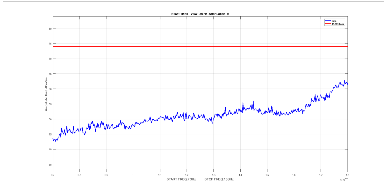
Plot 928. Undesirable Emissions, 5Omni, Peak, 7-18GHz, 40M, 5270, pow19
