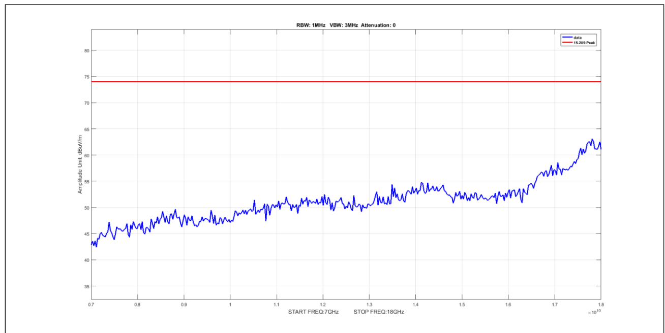
Plot 931. Undesirable Emissions, 5Omni, Peak, 7-18GHz, 40M, 5490, pow4
