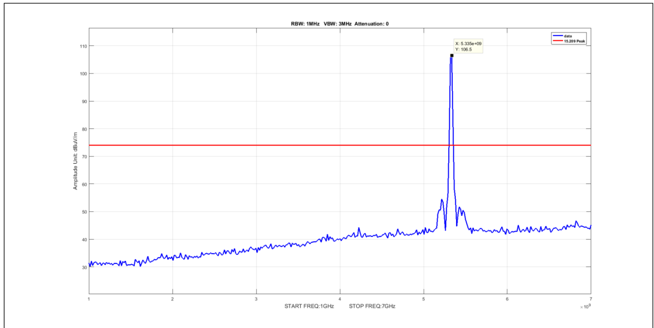
Plot 900. Undesirable Emissions, 5Omni, Peak, 1-7GHz, 20M, 5330, pow12
