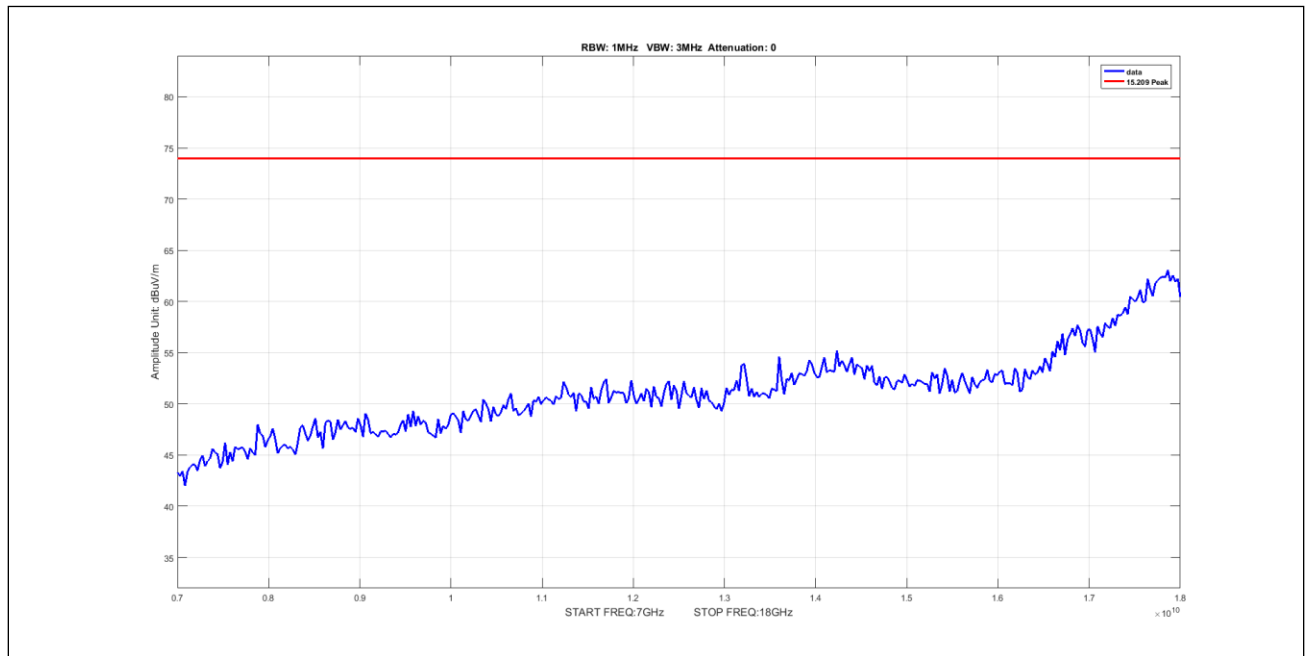
Plot 918. Undesirable Emissions, 5Omni, Peak, 7-18GHz, 10M, 5330, pow11
