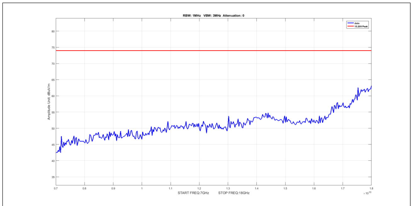
Plot 923. Undesirable Emissions, 5Omni, Peak, 7-18GHz, 20M, 5300, pow14
