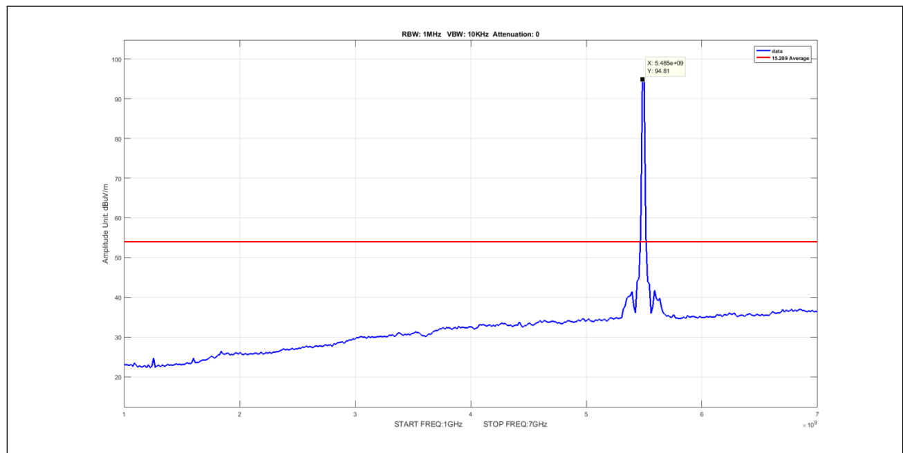
Plot 949. Undesirable Emissions, 8Omni, Average, 1-7GHz, 20M, 5490, pow9
