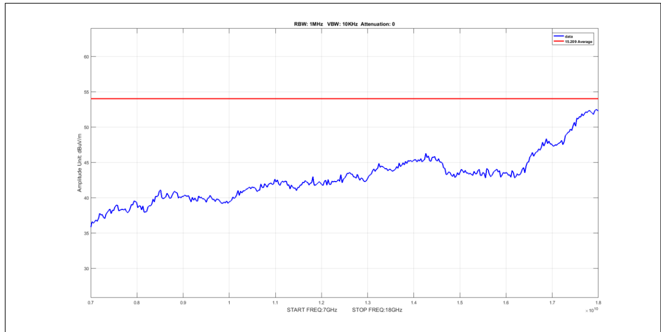
Plot 864. Undesirable Emissions, 5Omni, Average, 7-18GHz, 5M, 5330, pow8
