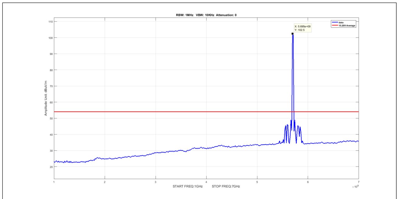
Plot 843. Undesirable Emissions, 5Omni, Average, 1-7GHz, 5M, 5700, pow8
