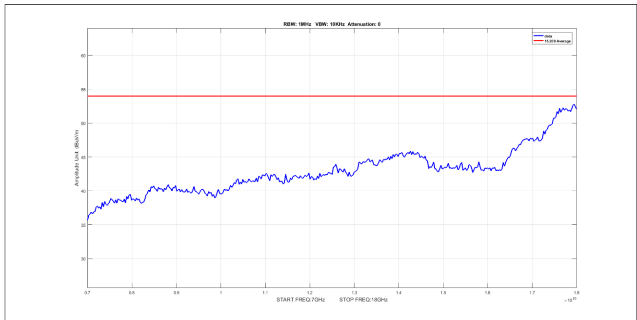
Plot 865. Undesirable Emissions, 5Omni, Average, 7-18GHz, 5M, 5490, pow9
