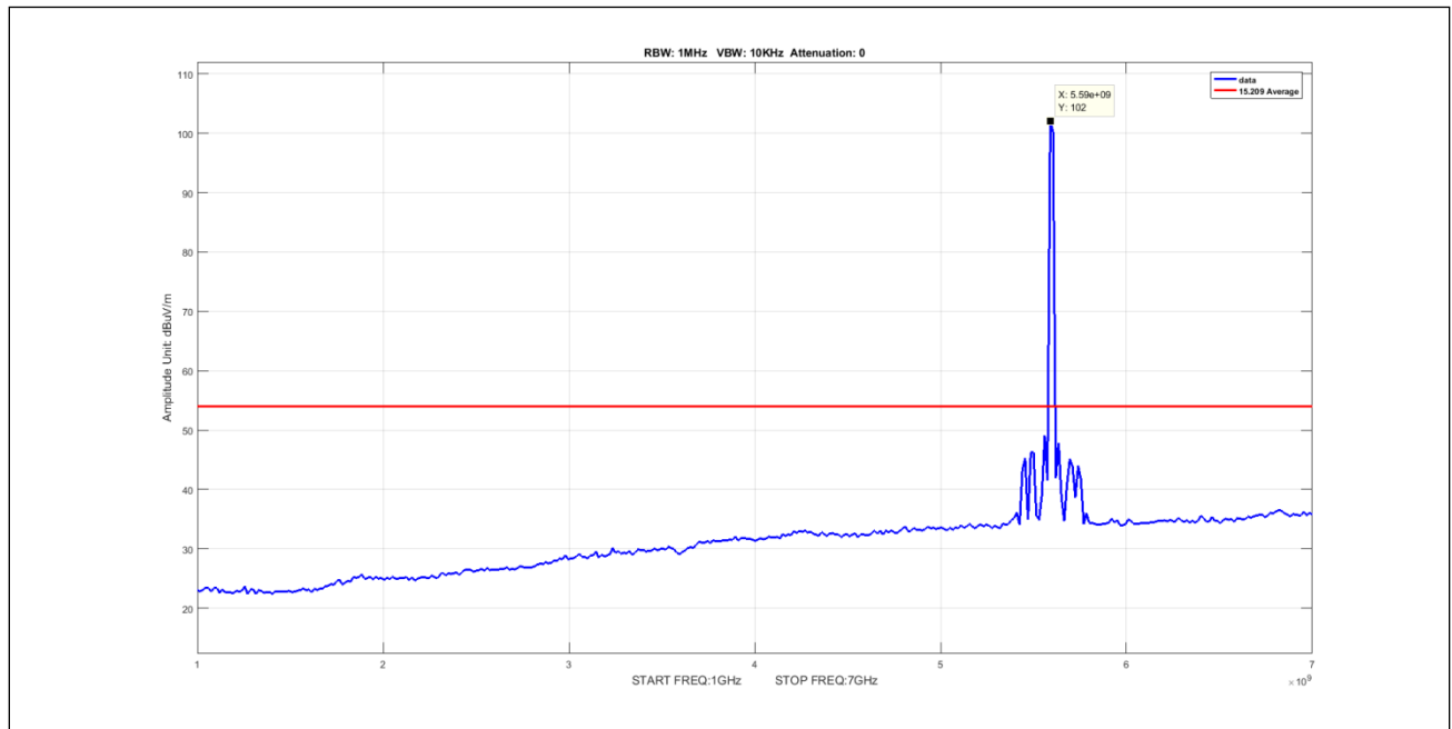
Plot 842. Undesirable Emissions, 5Omni, Average, 1-7GHz, 5M, 5595, pow8
