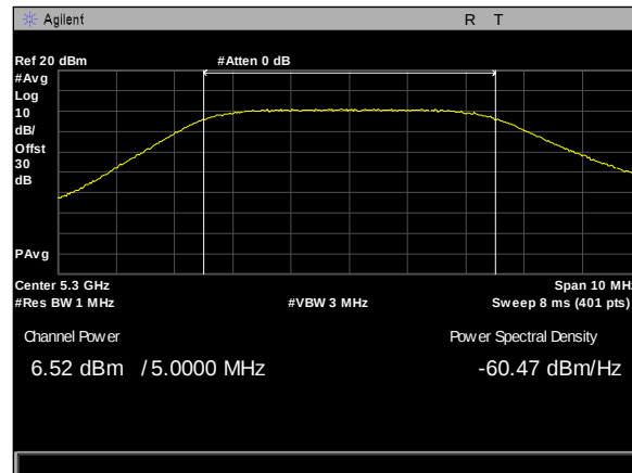
Plot 236. Maximum Conducted Output Power, 80Omni, 5M, 5300M, rf2
