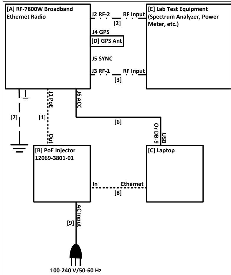
Figure 1. Block Diagram of Test Configuration
