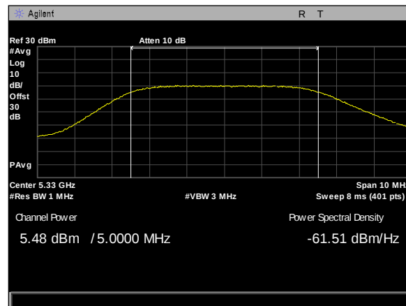
Plot 237. Maximum Conducted Output Power, 80Omni, 5M, 5330M, rf1
