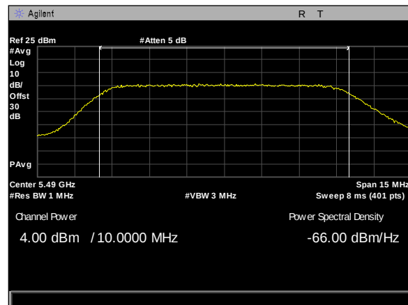
Plot 300. Maximum Conducted Output Power, 90Sector, 10M, 5490M, rf1
