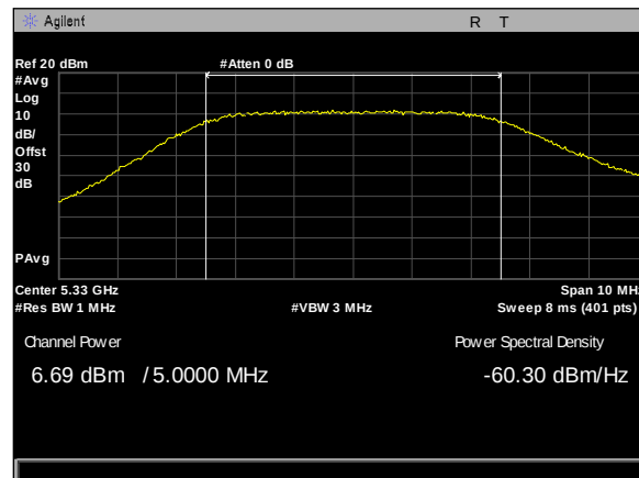
Plot 238. Maximum Conducted Output Power, 80Omni, 5M, 5330M, rf2
