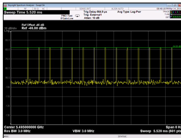
Plot 12. Radar Waveform Calibration, 5495 MHz, 10 MHz, Channel Radar Type 4
