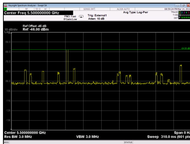
Plot 21. Radar Waveform Calibration, 5500 MHz, 20 MHz, Channel Radar Type 6
