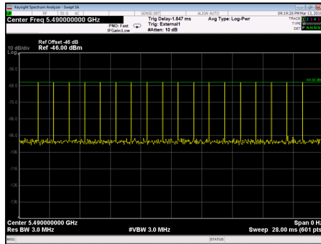
Plot 1. Radar Waveform Calibration, 5490 MHz, 5 MHz, Channel Radar Type 0
