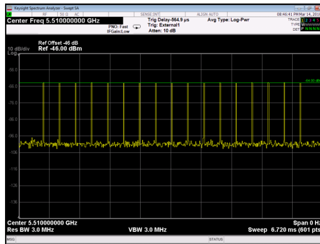
Plot 25. Radar Waveform Calibration, 5510 MHz, 40 MHz, Channel Radar Type 3
