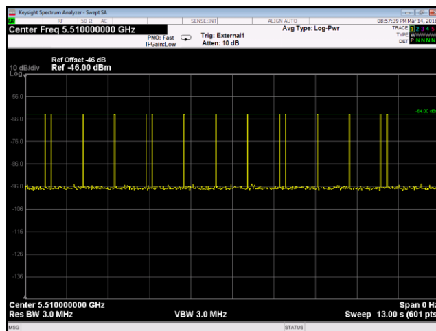
Plot 27. Radar Waveform Calibration, 5510 MHz, 40 MHz, Channel Radar Type 5
