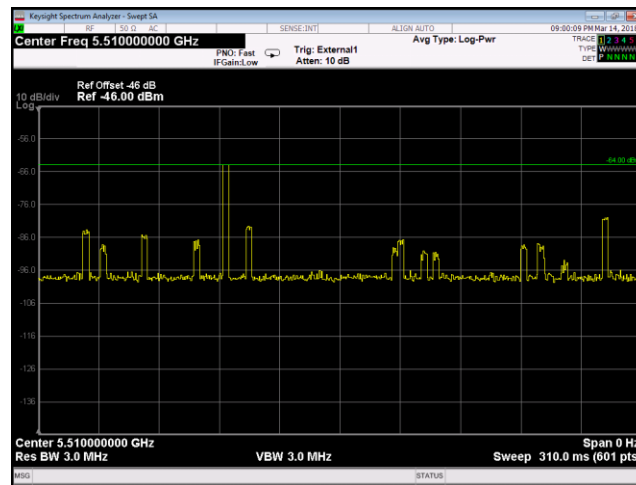
Plot 28. Radar Waveform Calibration, 5510 MHz, 40 MHz, Channel Radar Type 6
