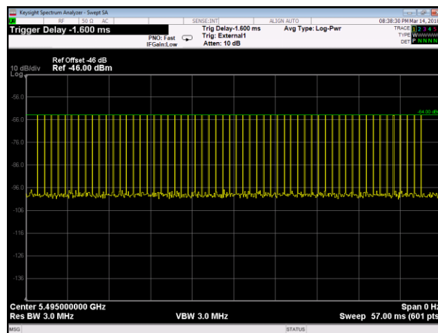
Plot 9. Radar Waveform Calibration, 5495 MHz, 10 MHz, Channel Radar Type 1
