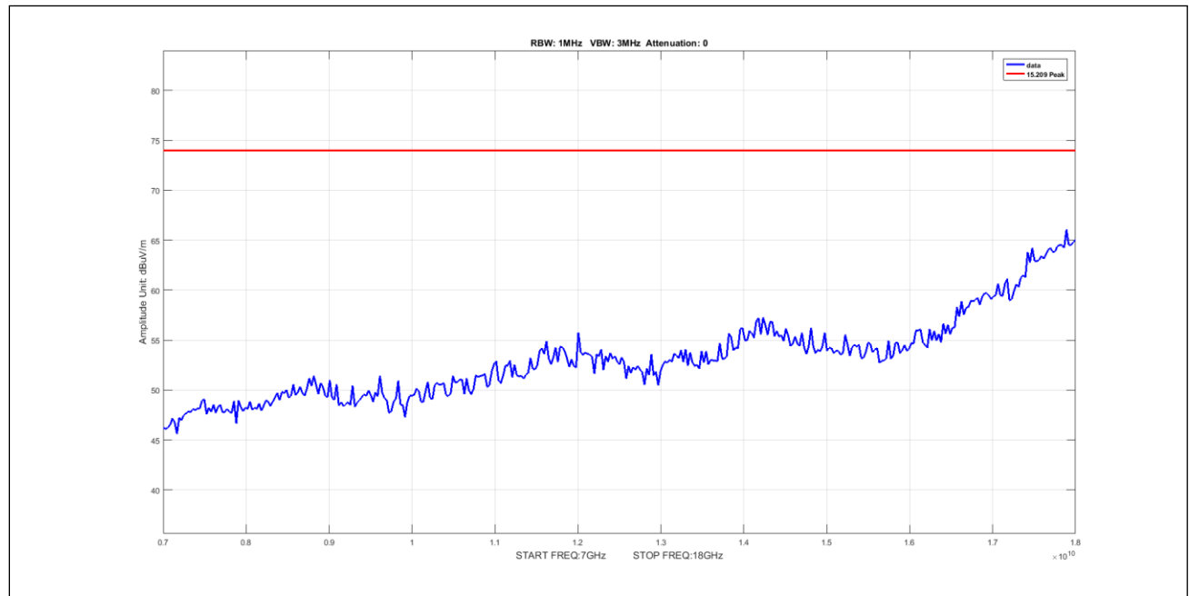
Plot 597. Undesirable Emissions, 8Omni Peak 7-18GHz 5M 5170 pow12
