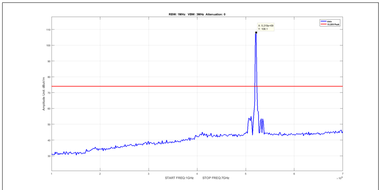
Plot 638. Undesirable Emissions, 90Sector Peak 1-7GHz 10M 5210 pow9
