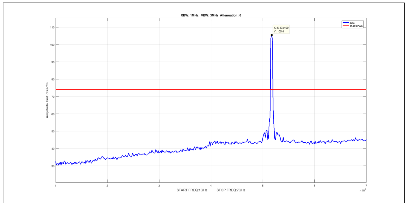
Plot 640. Undesirable Emissions, 90Sector Peak 1-7GHz 20M 5170 pow6
