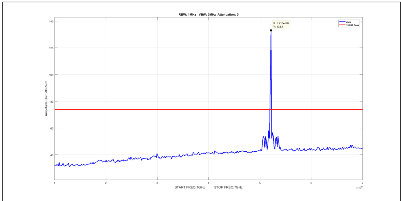
Plot 585. Undesirable Emissions, 8Omni Peak 1-7GHz 5M 5210 pow11
