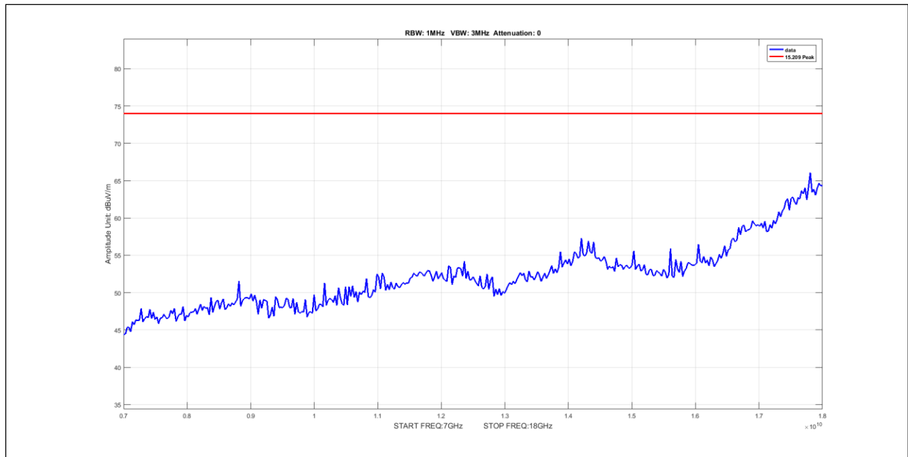
Plot 605. Undesirable Emissions, 8Omni Peak 7-18GHz 20M 5240 pow18
