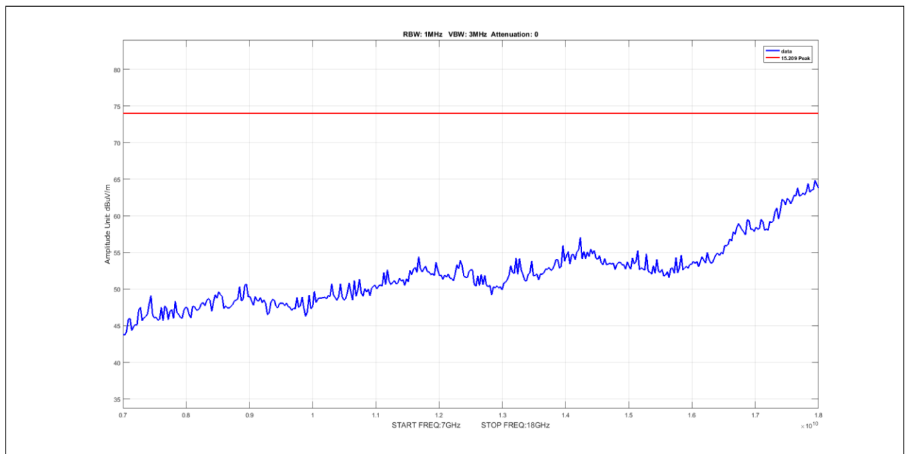
Plot 600. Undesirable Emissions, 8Omni Peak 7-18GHz 10M 5170 pow15
