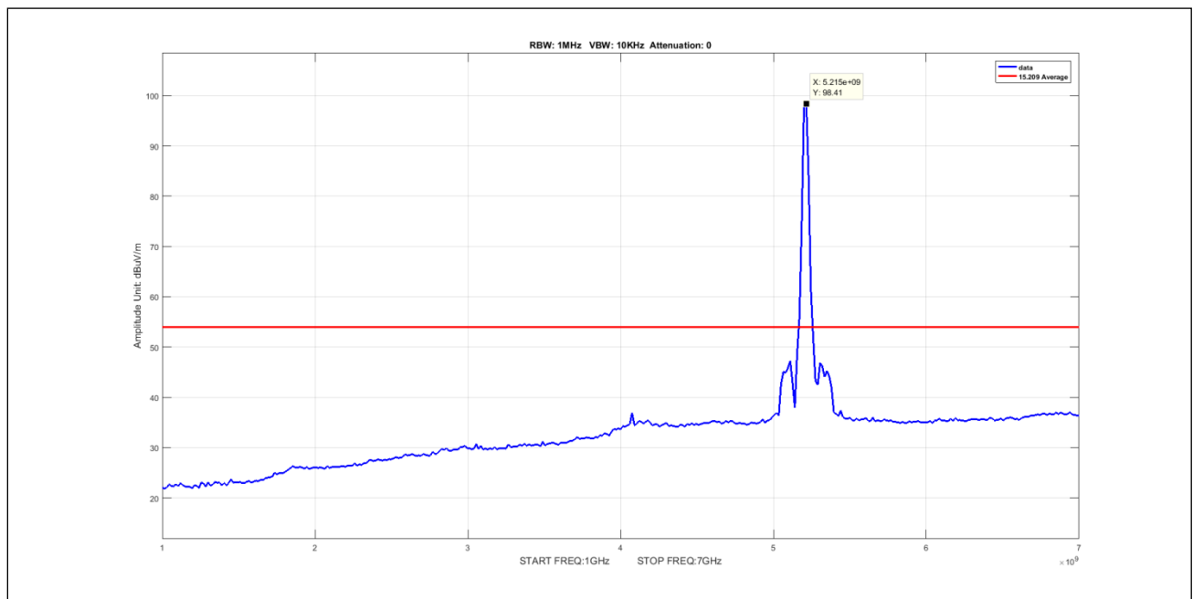
Plot 616. Undesirable Emissions, 90Sector Avg 1-7GHz 20M 5210 pow12
