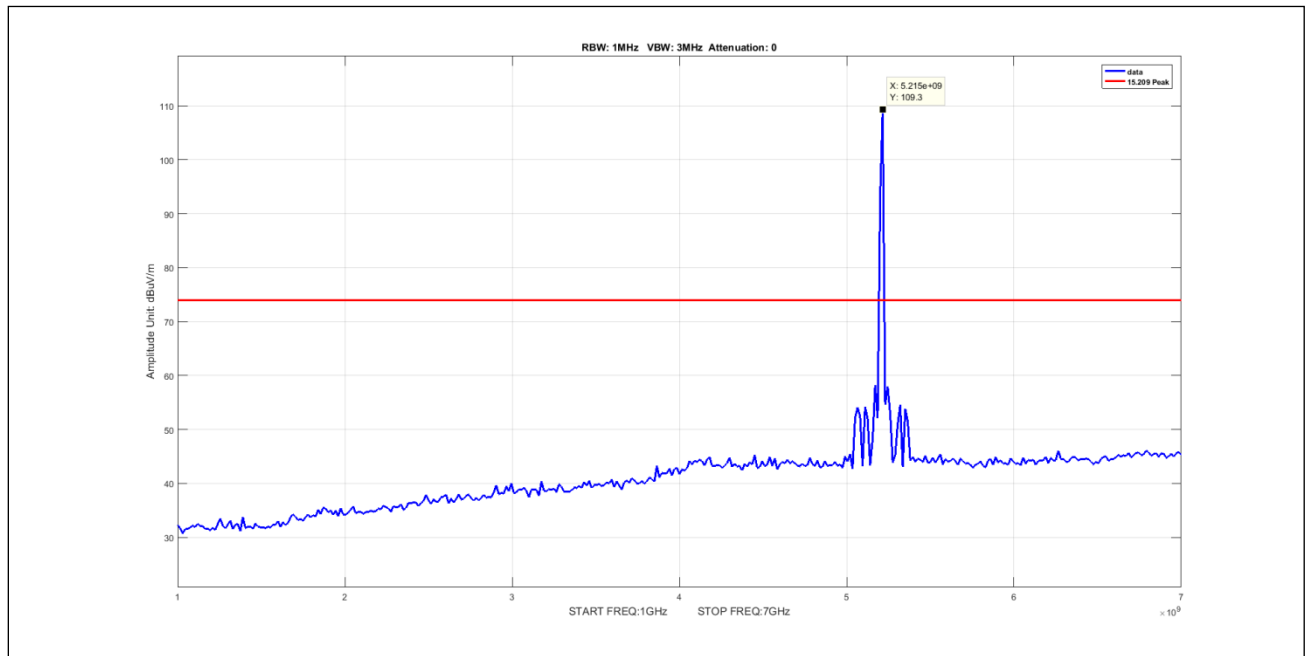
Plot 635. Undesirable Emissions, 90Sector Peak 1-7GHz 5M 5210 pow6
