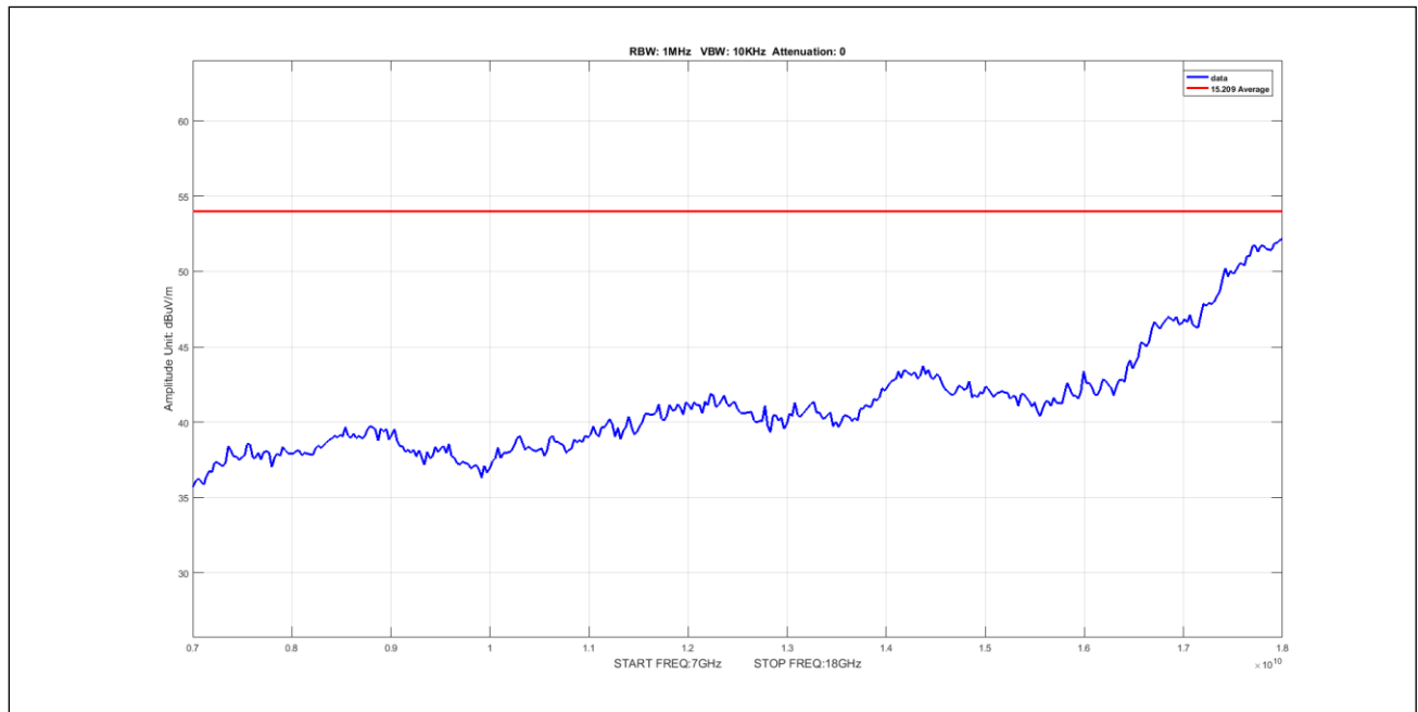
Plot 579. Undesirable Emissions, 8Omni Avg 7-18GHz 20M 5210 pow18
