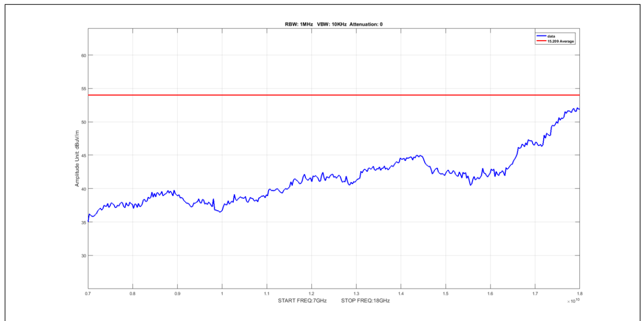
Plot 626. Undesirable Emissions, 90Sector Avg 7-18GHz 10M 5210 pow9
