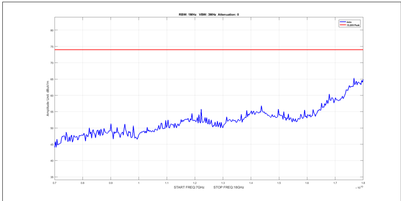
Plot 603. Undesirable Emissions, 8Omni Peak 7-18GHz 20M 5170 pow9
