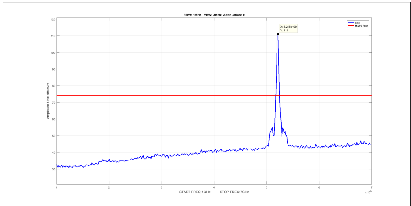
Plot 591. Undesirable Emissions, 8Omni Peak 1-7GHz 20M 5210 pow18
