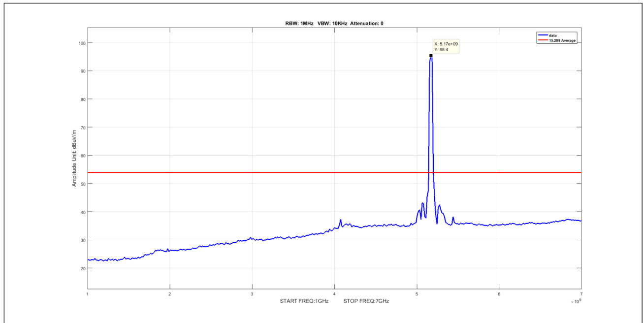
Plot 615. Undesirable Emissions, 90Sector Avg 1-7GHz 20M 5170 pow6
