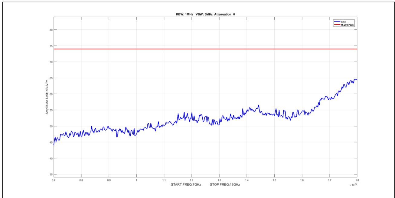
Plot 607. Undesirable Emissions, 8Omni Peak 7-18GHz 40M 5210 pow22
