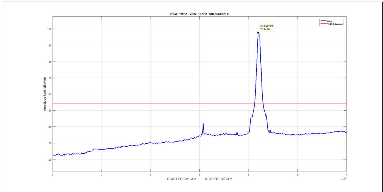
Plot 619. Undesirable Emissions, 90Sector Avg 1-7GHz 40M 5210 pow16
