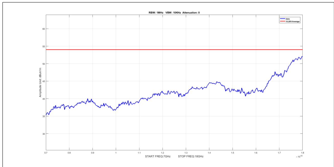
Plot 622. Undesirable Emissions, 90Sector Avg 7-18GHz 5M 5170 pow7
