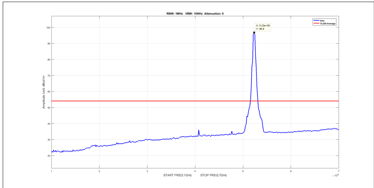
Plot 571. Undesirable Emissions, 8Omni Avg 1-7GHz 40M 5230 pow22
