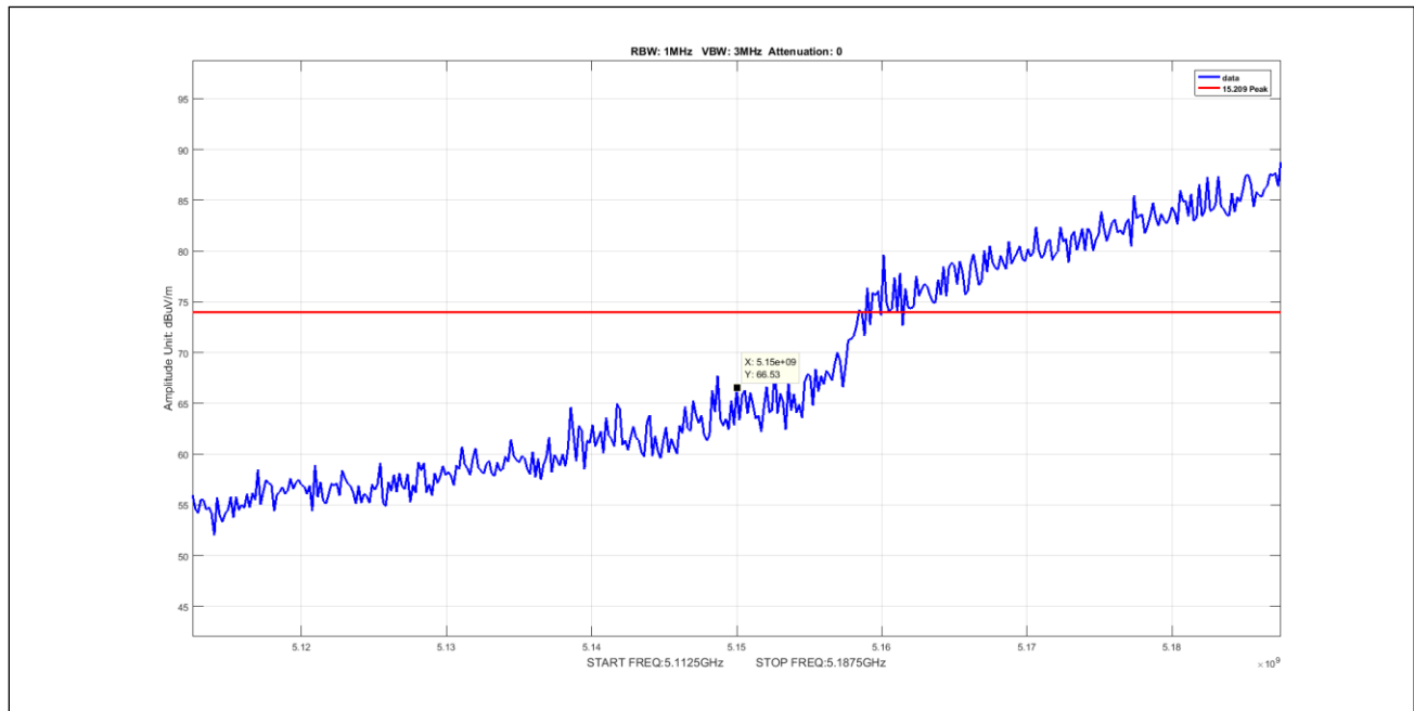
Plot 595. Undesirable Emissions, 8Omni Peak 1-7GHz 40M 5210 pow22 zoom
