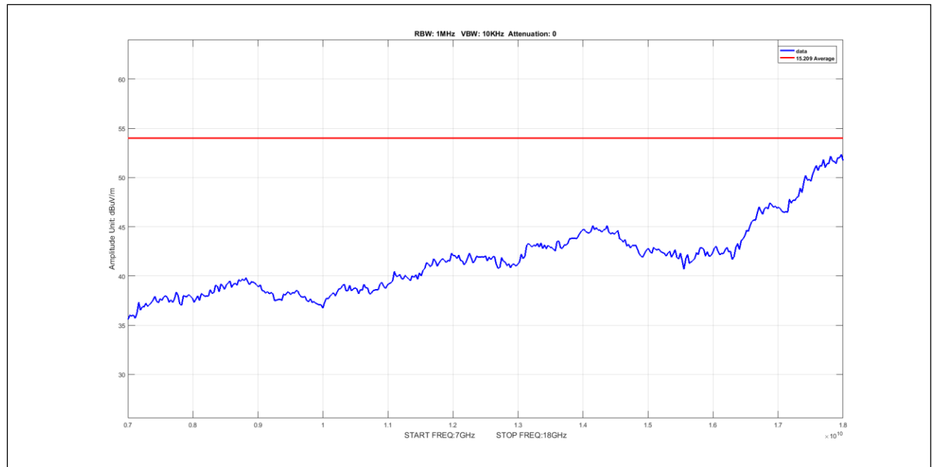
Plot 625. Undesirable Emissions, 90Sector Avg 7-18GHz 10M 5170 pow10
