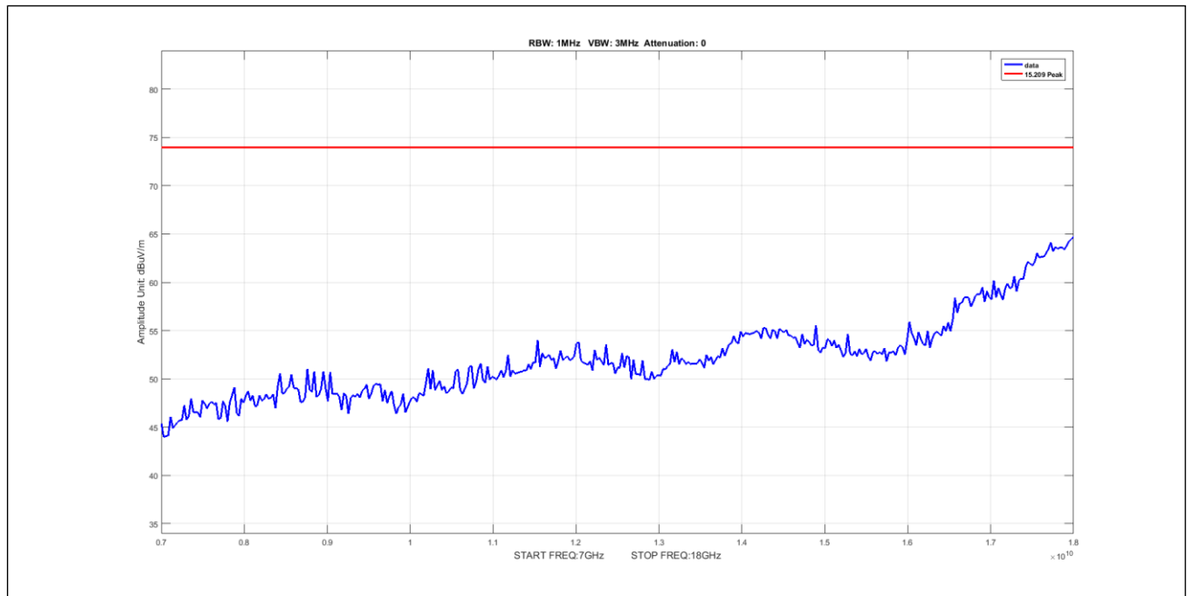
Plot 601. Undesirable Emissions, 8Omni Peak 7-18GHz 10M 5210 pow15
