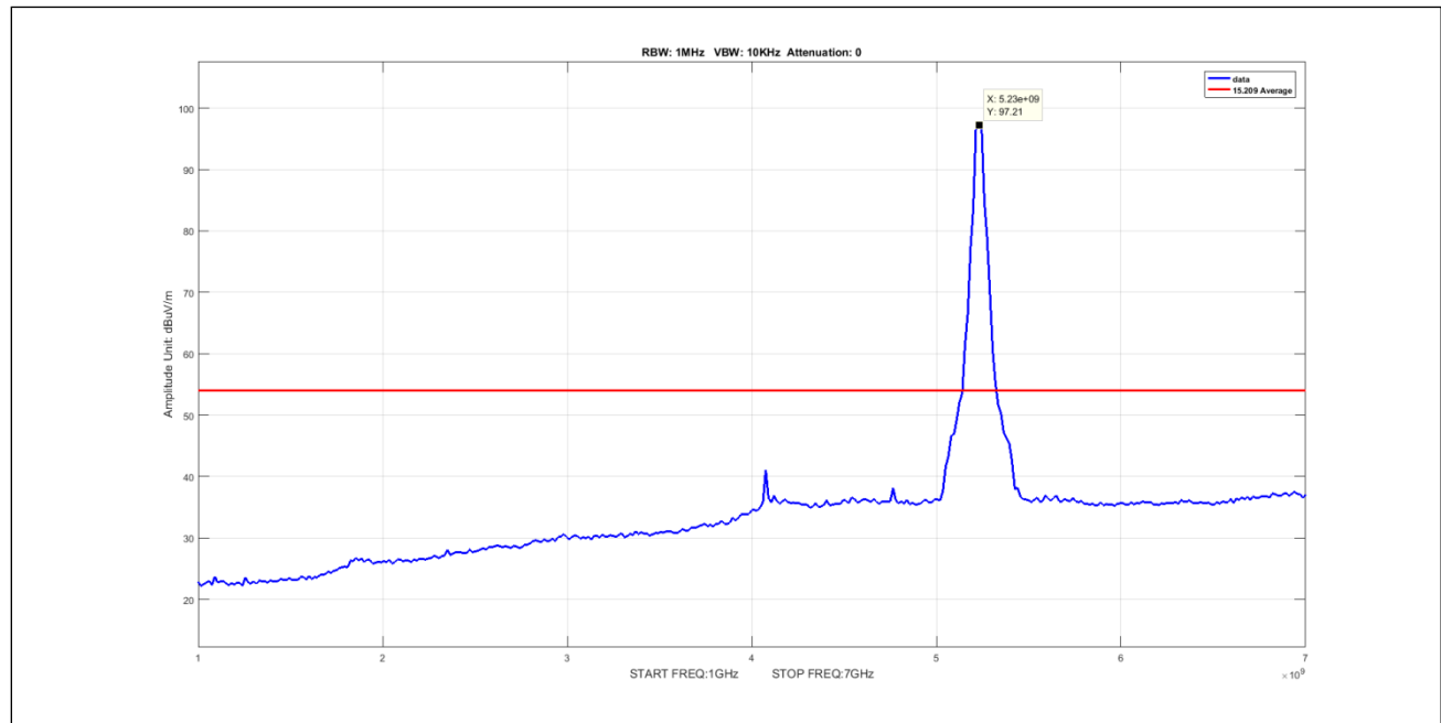
Plot 621. Undesirable Emissions, 90Sector Avg 1-7GHz 40M 5230 pow16
