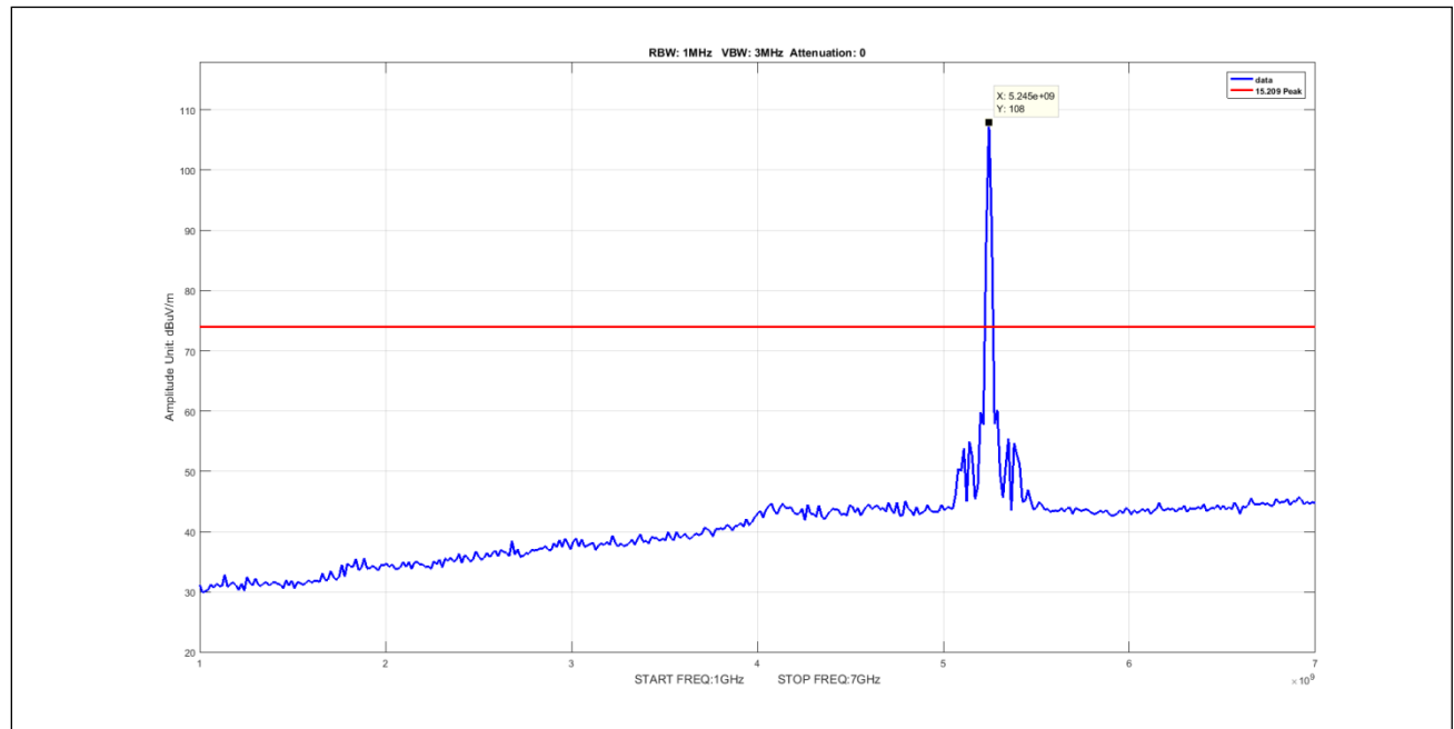
Plot 639. Undesirable Emissions, 90Sector Peak 1-7GHz 10M 5245 pow9
