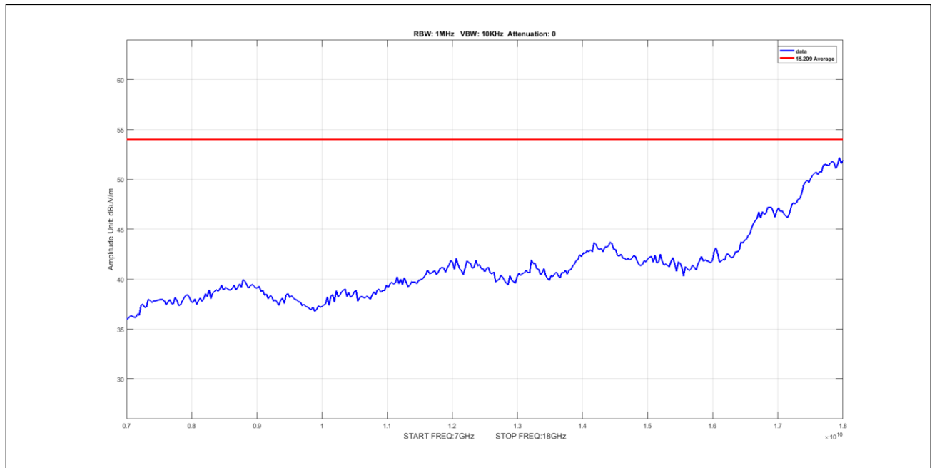
Plot 581. Undesirable Emissions, 80mni Avg 7-18GHz 40M 5170 pow4
