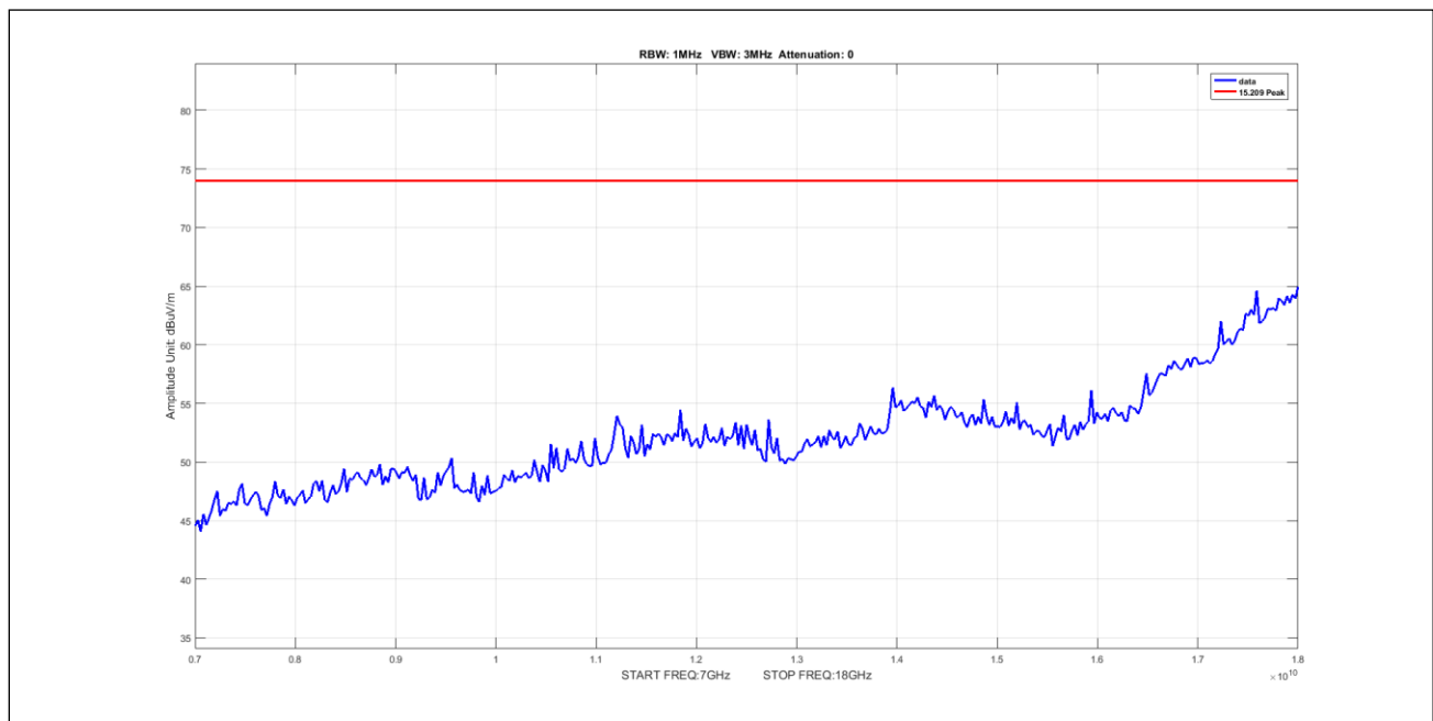
Plot 604. Undesirable Emissions, 8Omni Peak 7-18GHz 20M 5210 pow18
