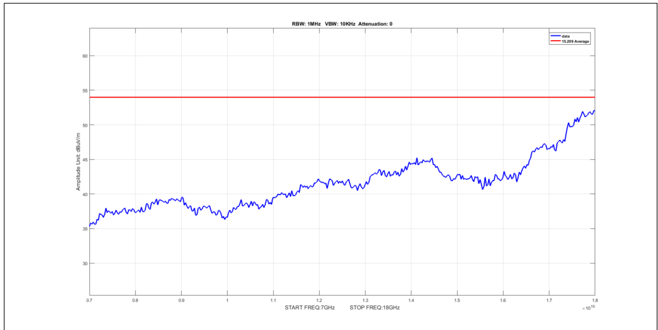
Plot 623. Undesirable Emissions, 90Sector Avg 7-18GHz 5M 5210 pow6
