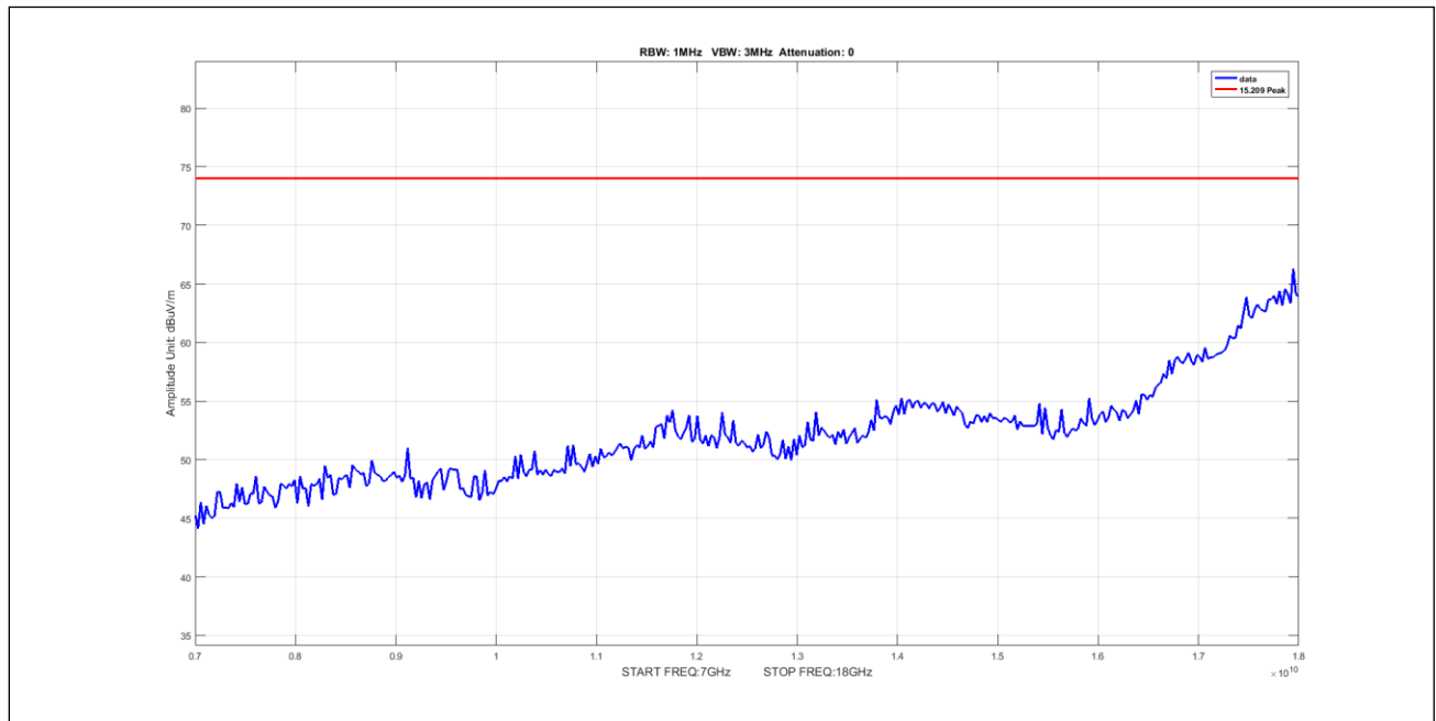
Plot 599. Undesirable Emissions, 8Omni Peak 7-18GHz 5M 5247.5 pow11
