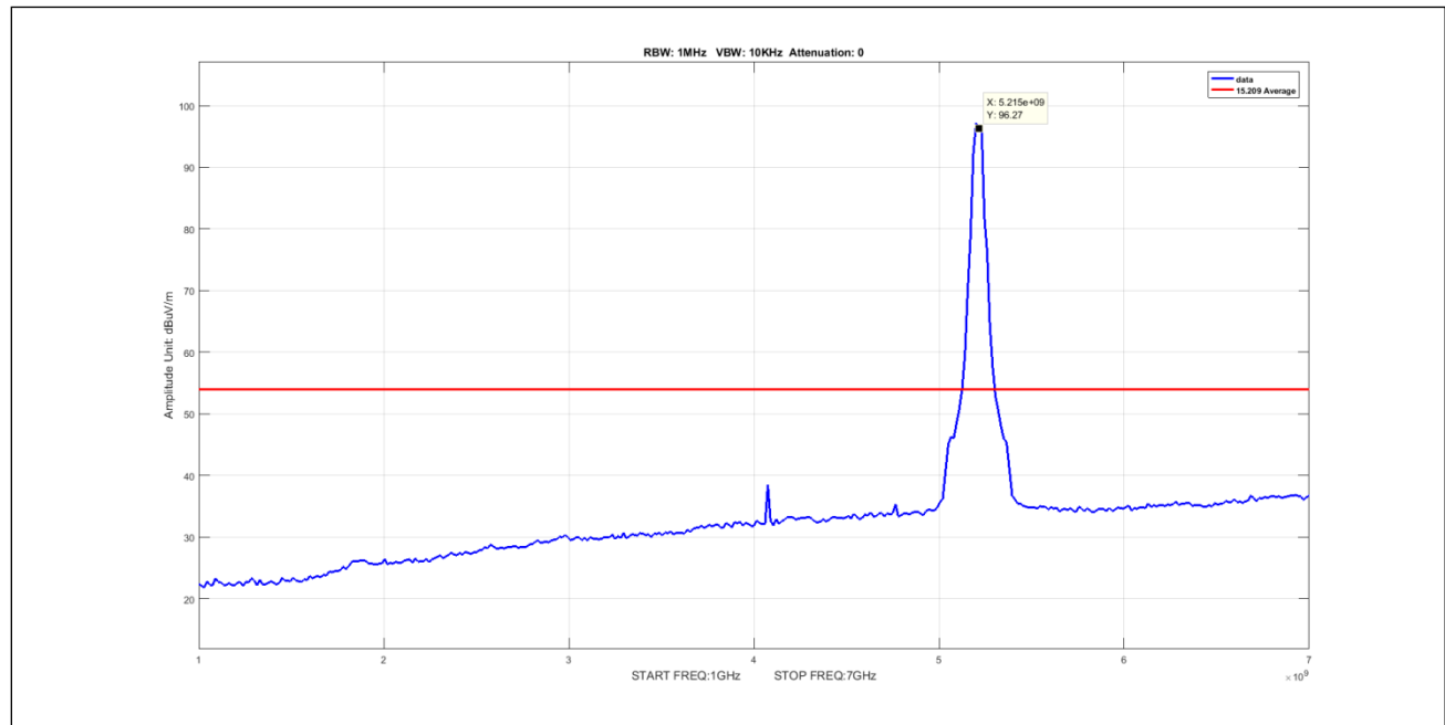
Plot 569. Undesirable Emissions, 8Omni Avg 1-7GHz 40M 5210 pow22
