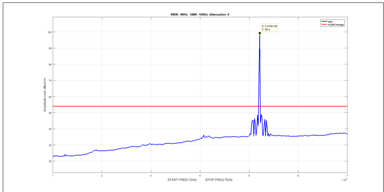
Plot 610. Undesirable Emissions, 90Sector Avg 1-7GHz 5M 5210 pow6
