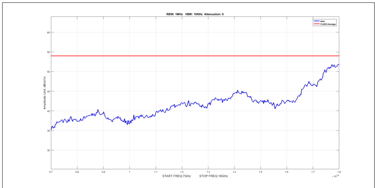
Plot 632. Undesirable Emissions, 90Sector Avg 7-18GHz 40M 5210 pow16
