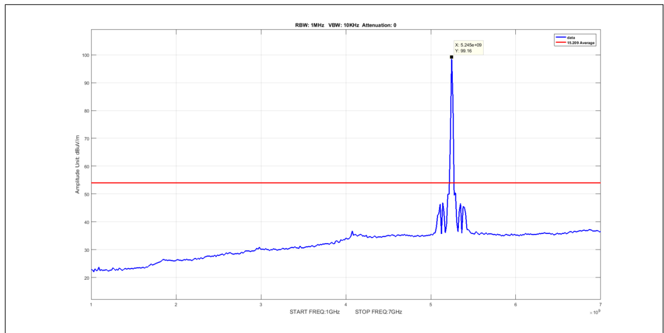
Plot 614. Undesirable Emissions, 90Sector Avg 1-7GHz 10M 5245 pow9
