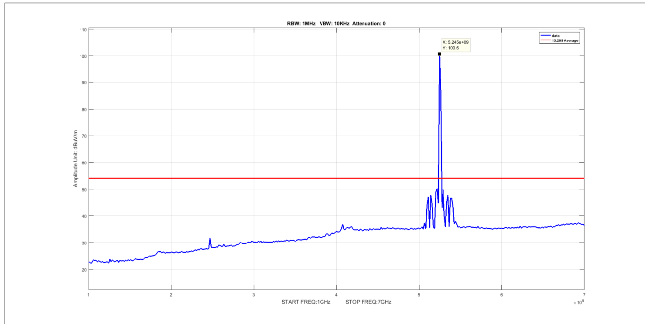
Plot 611. Undesirable Emissions, 90Sector Avg 1-7GHz 5M 5247.5 pow7
