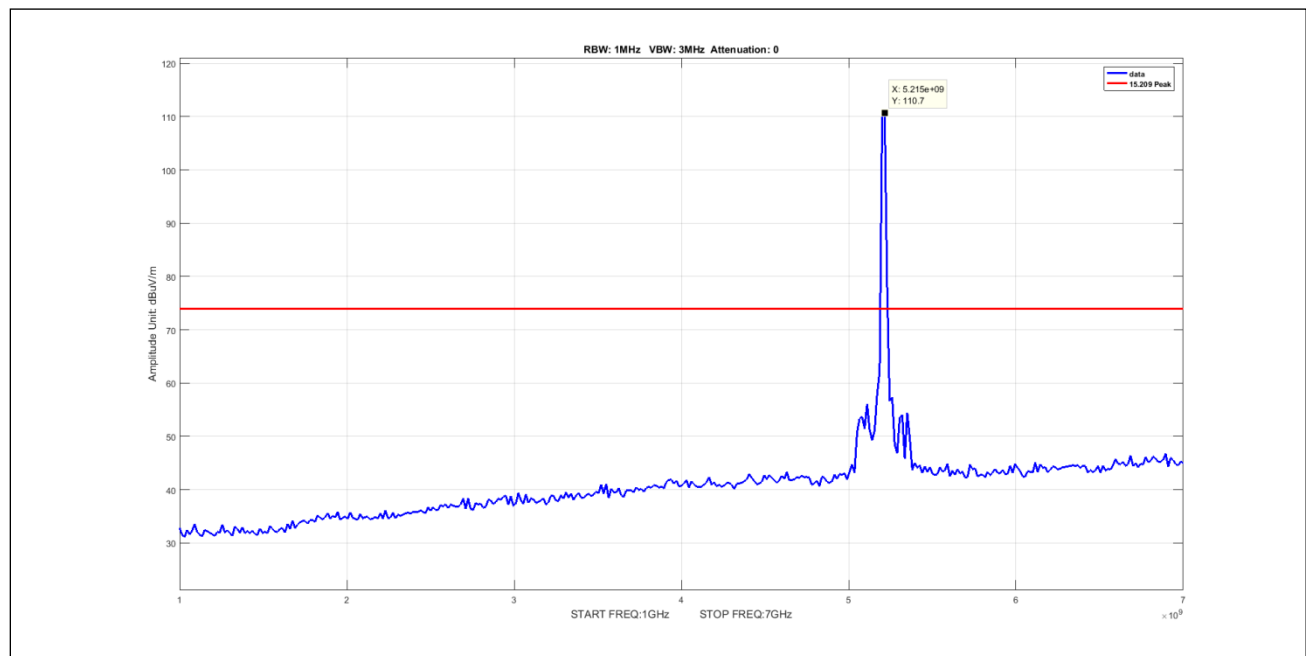
Plot 588. Undesirable Emissions, 8Omni Peak 1-7GHz 10M 5210 pow15
