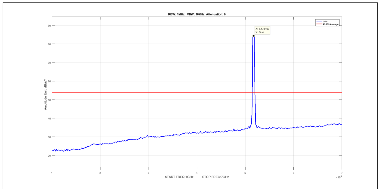
Plot 568. Undesirable Emissions, 8Omni Avg 1-7GHz 40M 5170 pow4
