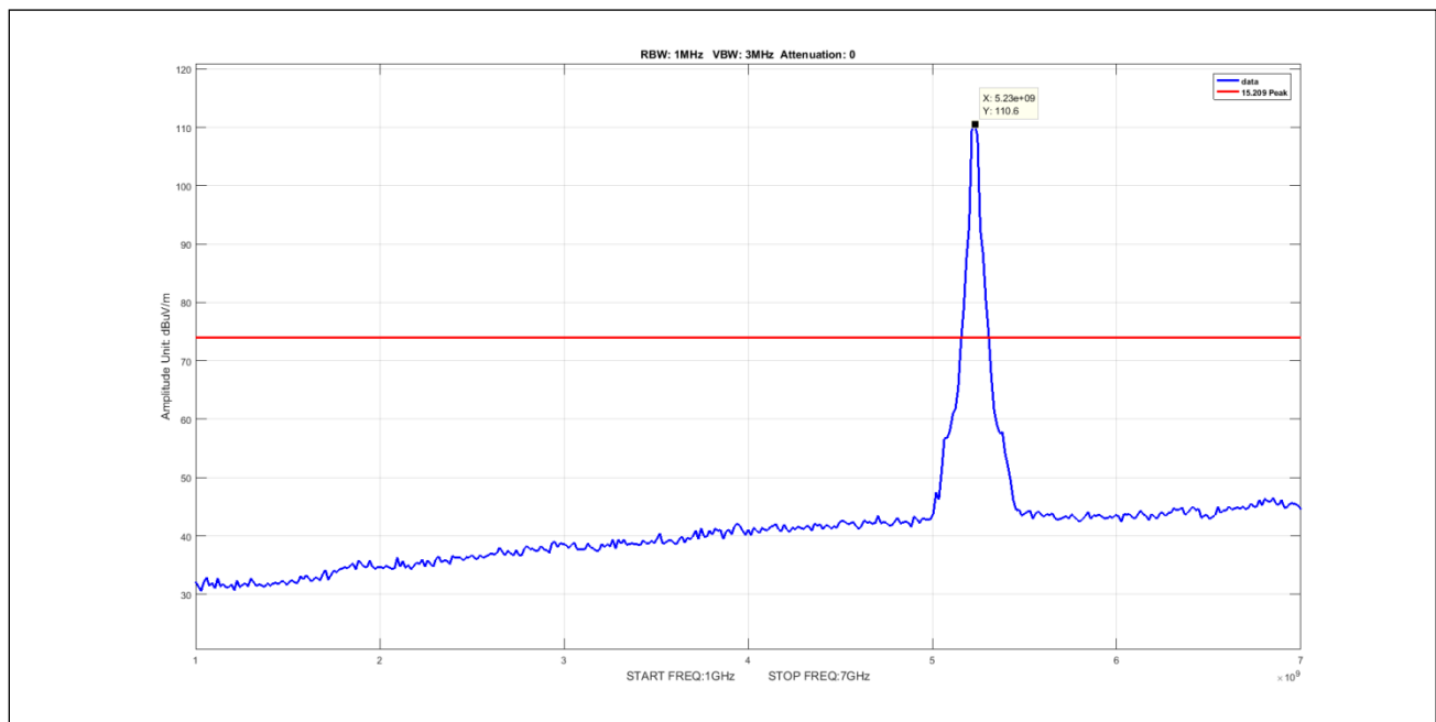
Plot 596. Undesirable Emissions, 8Omni Peak 1-7GHz 40M 5230 pow22
