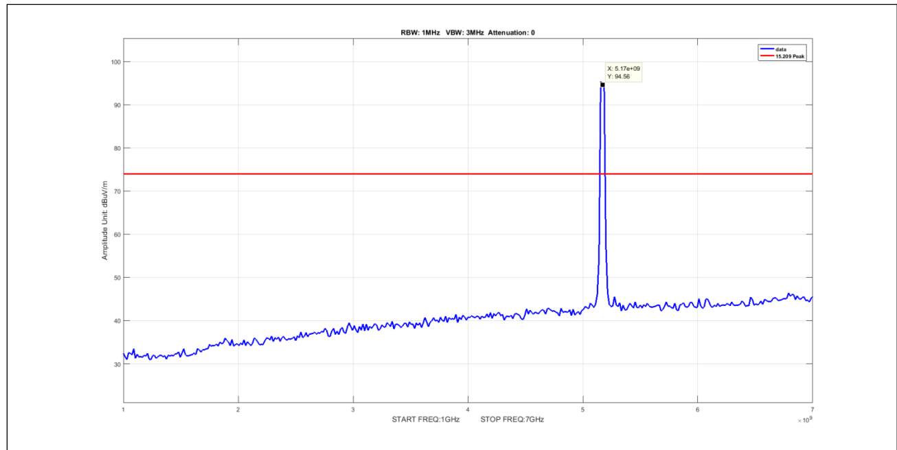
Plot 593. Undesirable Emissions, 8Omni Peak 1-7GHz 40M 5170 pow4
