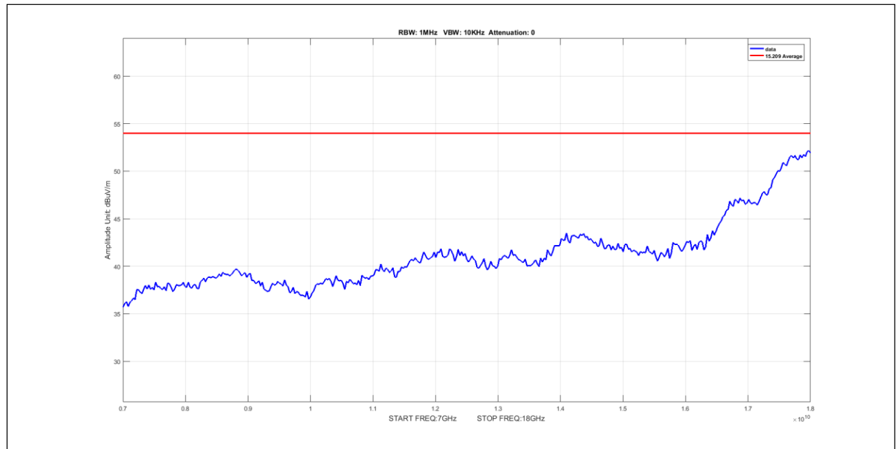
Plot 573. Undesirable Emissions, 8Omni Avg 7-18GHz 5M 5210 pow11
