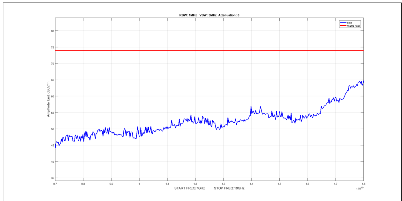
Plot 598. Undesirable Emissions, 8Omni Peak 7-18GHz 5M 5210 pow11
