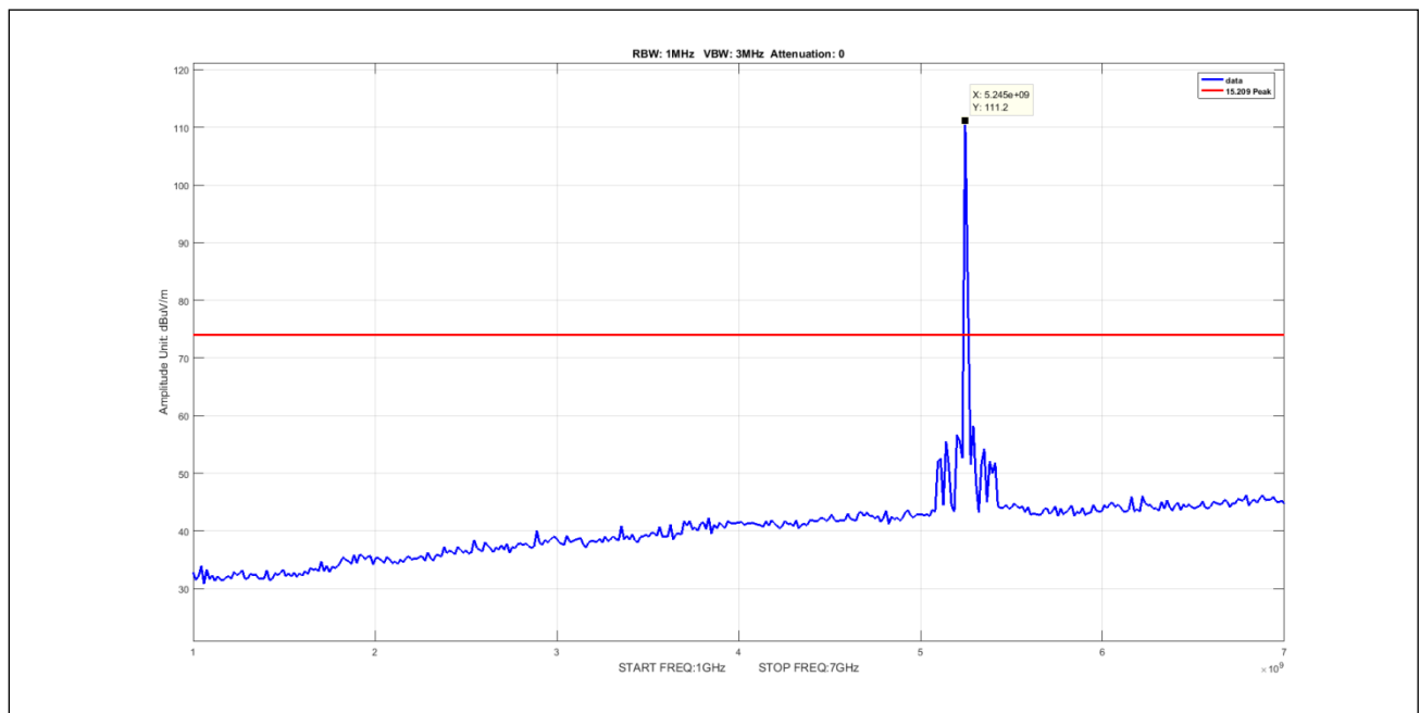
Plot 586. Undesirable Emissions, 8Omni Peak 1-7GHz 5M 5247.5 pow11
