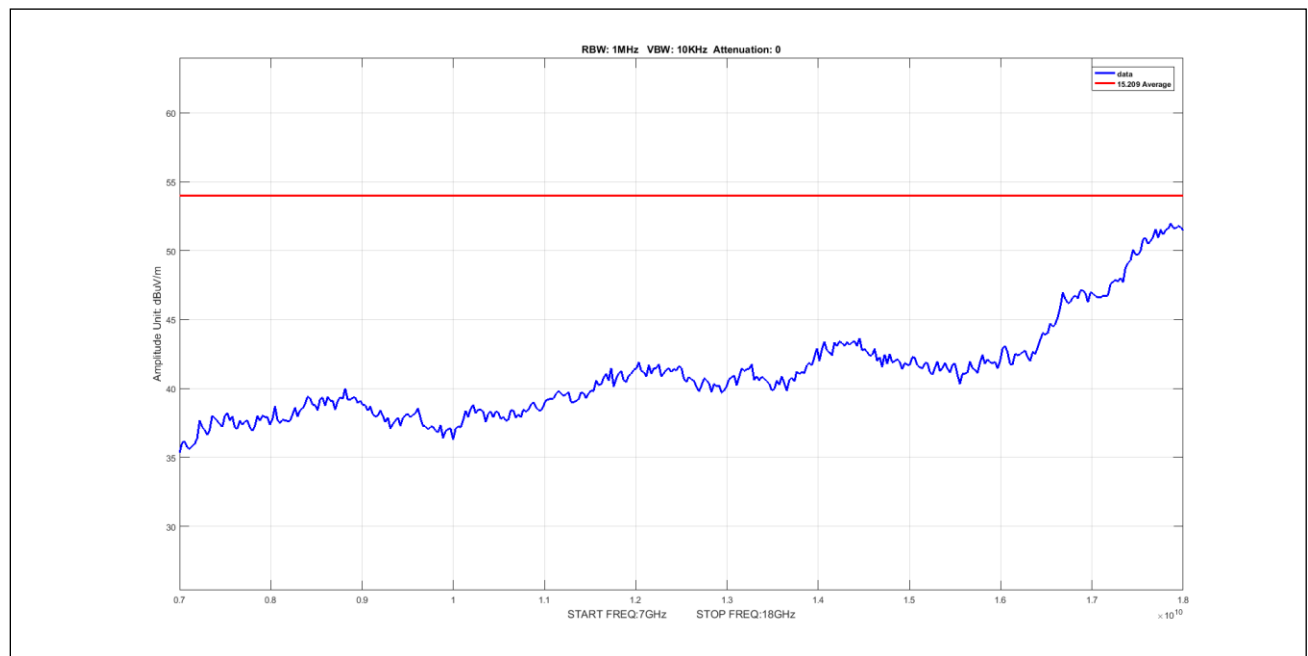
Plot 574. Undesirable Emissions, 8Omni Avg 7-18GHz 5M 5247.5 pow11
