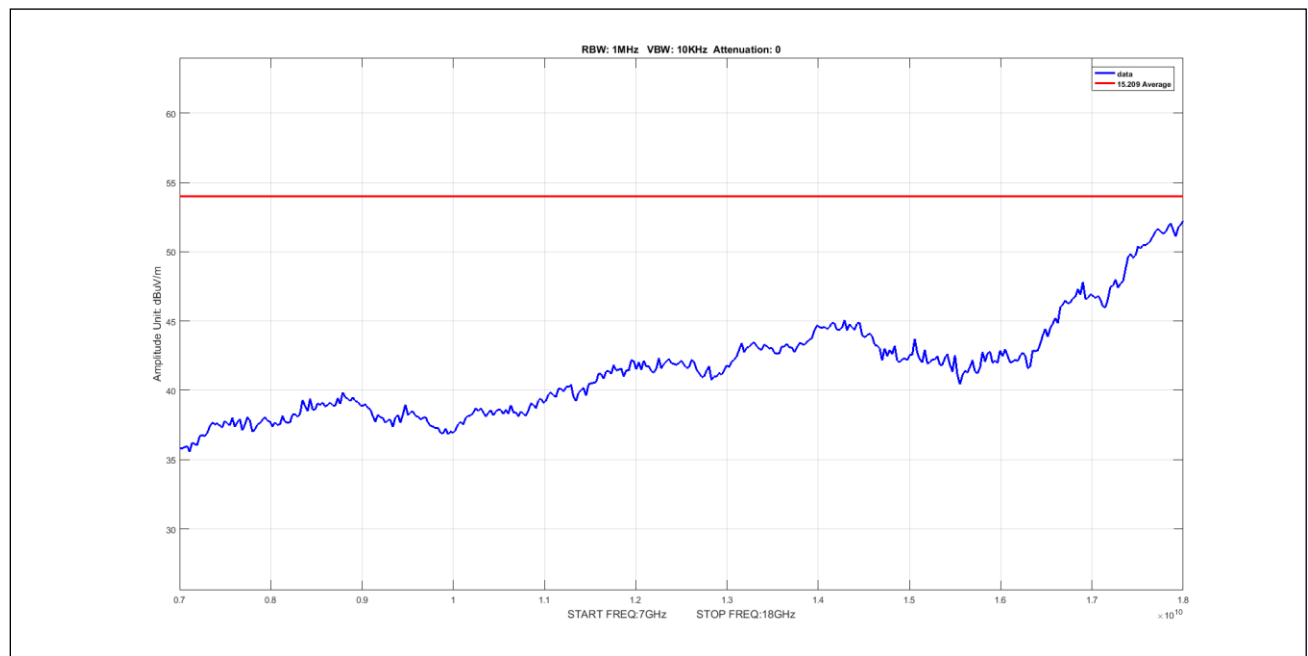
Plot 630. Undesirable Emissions, 90Sector Avg 7-18GHz 20M 5240 pow12
