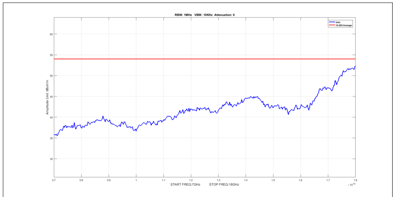
Plot 628. Undesirable Emissions, 90Sector Avg 7-18GHz 20M 5170 pow6
