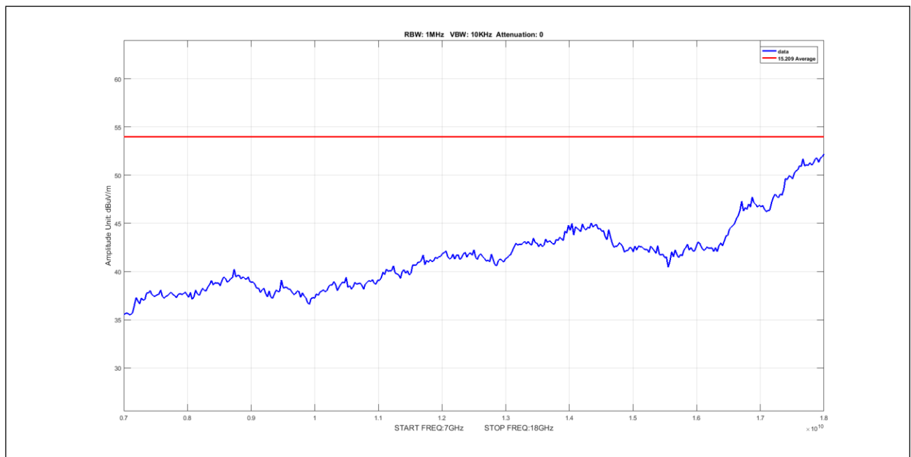
Plot 624. Undesirable Emissions, 90Sector Avg 7-18GHz 5M 5247.5 pow7
