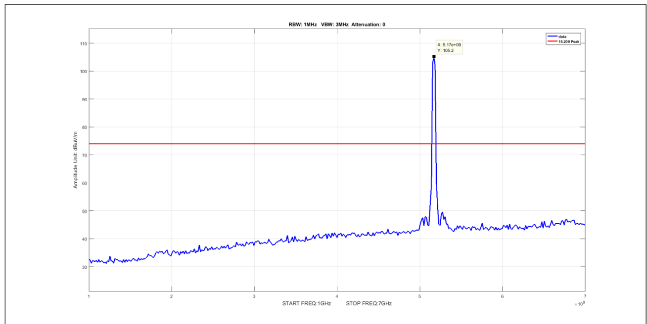
Plot 590. Undesirable Emissions, 8Omni Peak 1-7GHz 20M 5170 pow9
