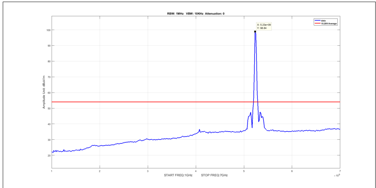
Plot 617. Undesirable Emissions, 90Sector Avg 1-7GHz 20M 5240 pow12
