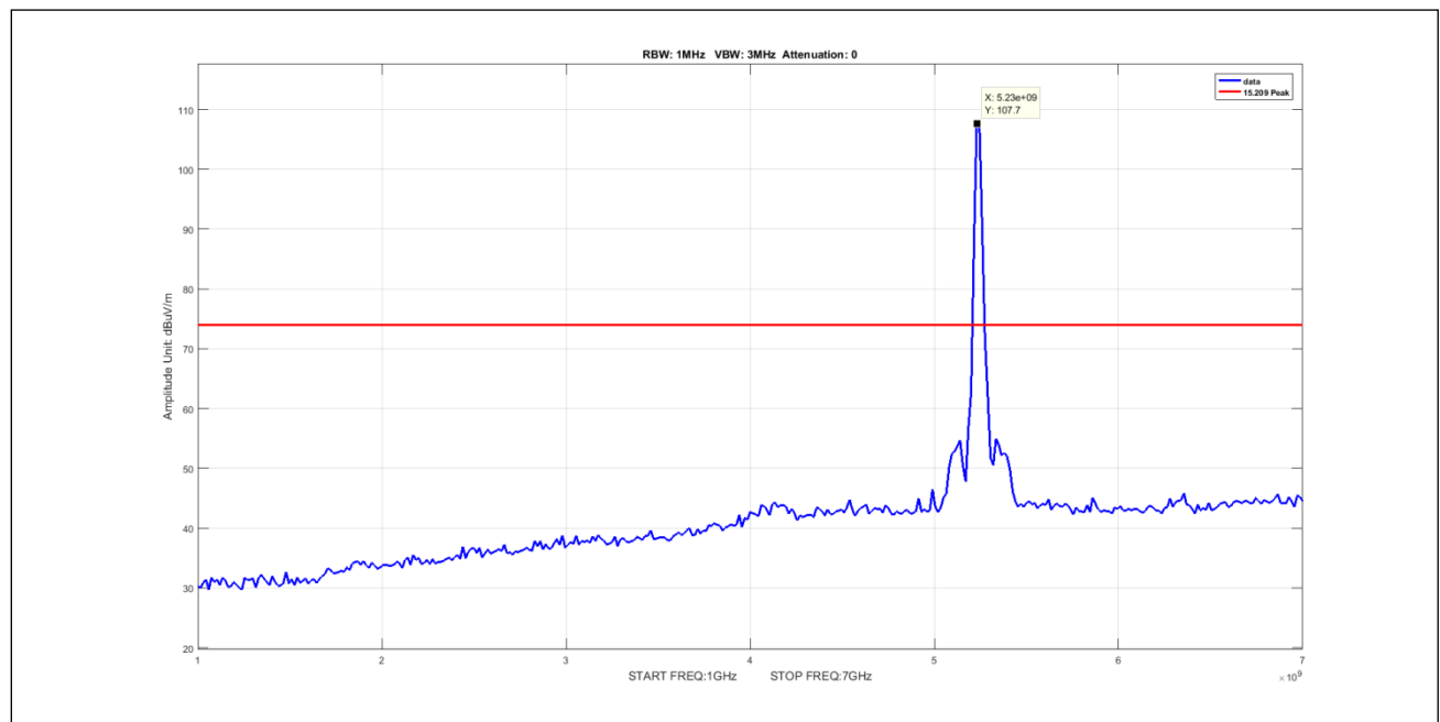
Plot 642. Undesirable Emissions, 90Sector Peak 1-7GHz 20M 5230 pow12
