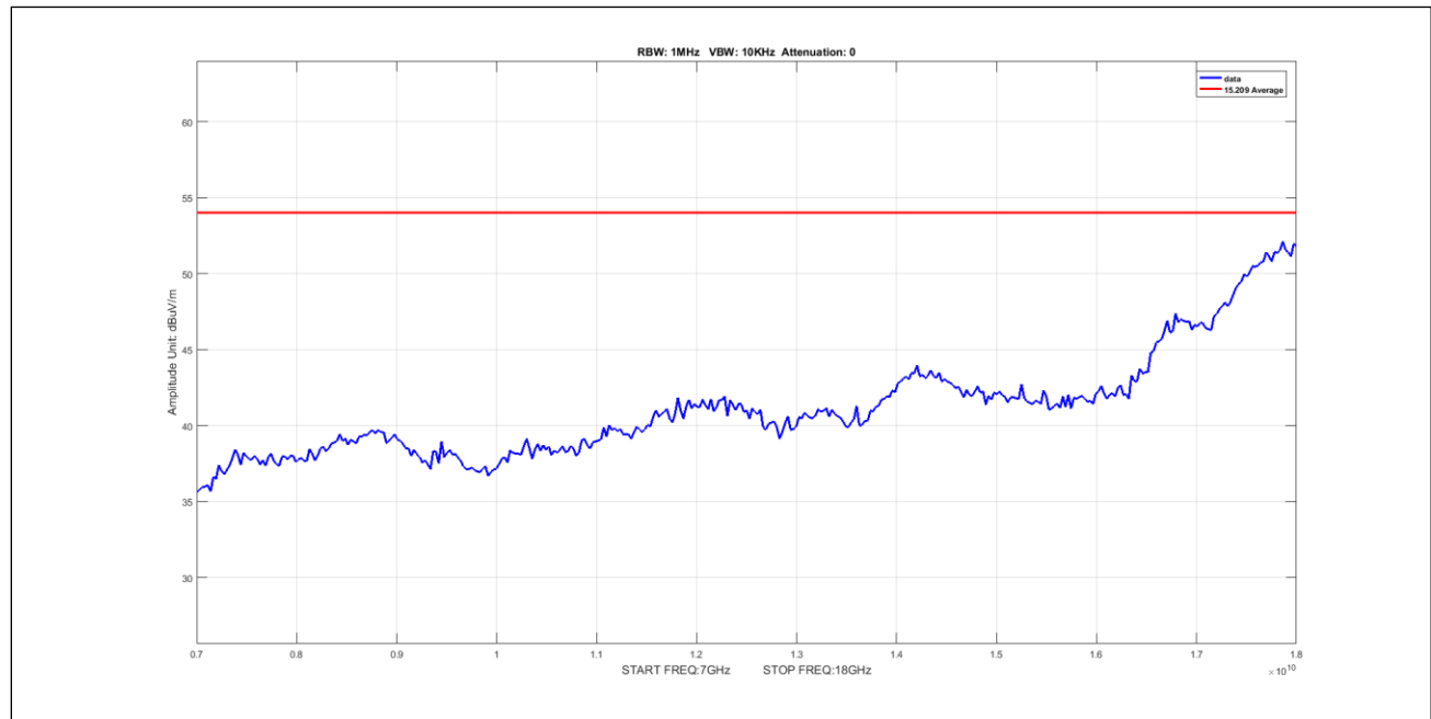
Plot 583. Undesirable Emissions, 8Omni Avg 7-18GHz 40M 5230 pow22
