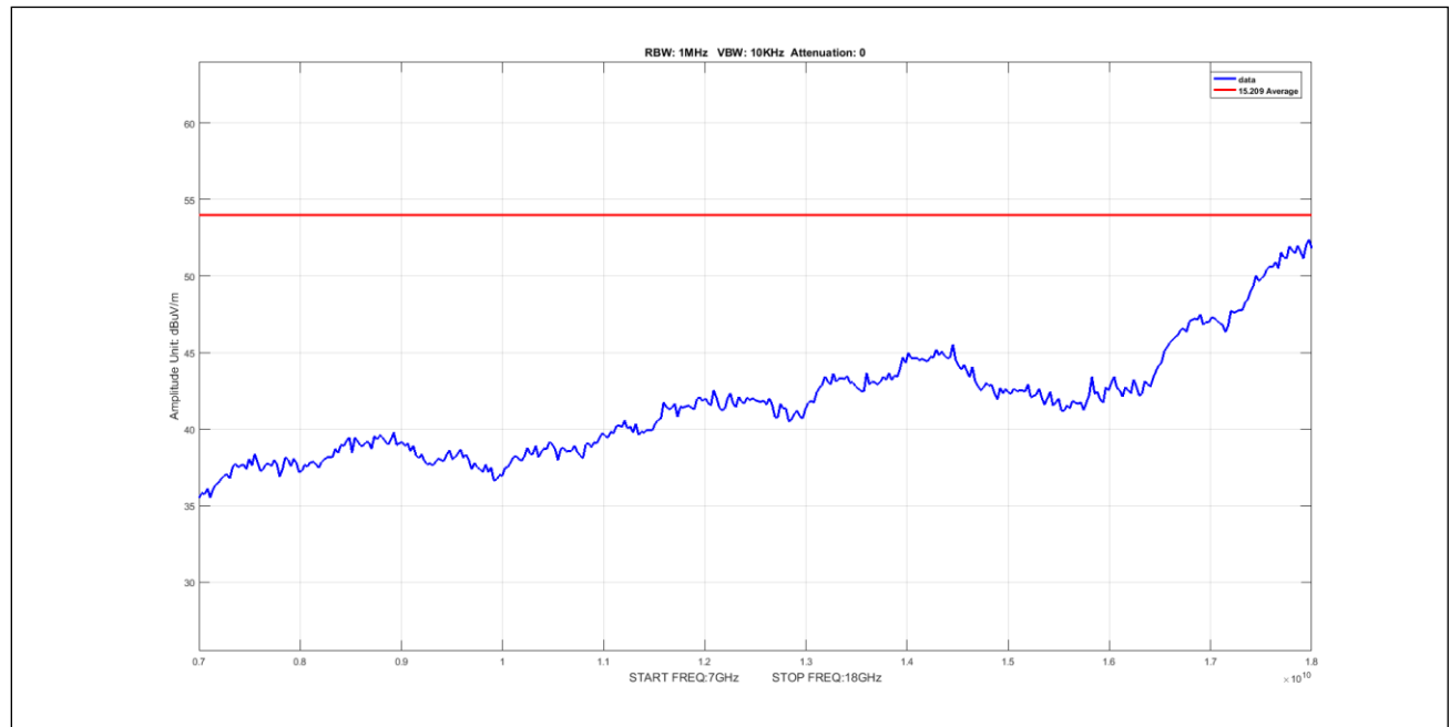
Plot 627. Undesirable Emissions, 90Sector Avg 7-18GHz 10M 5245 pow9
