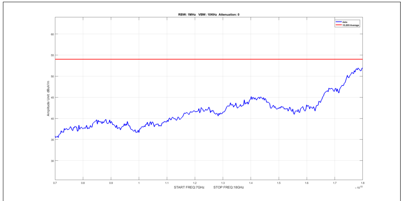
Plot 629. Undesirable Emissions, 90Sector Avg 7-18GHz 20M 5210 pow12
