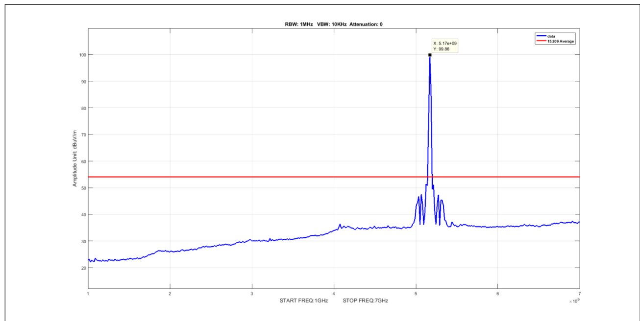
Plot 612. Undesirable Emissions, 90Sector Avg 1-7GHz 10M 5170 pow10
