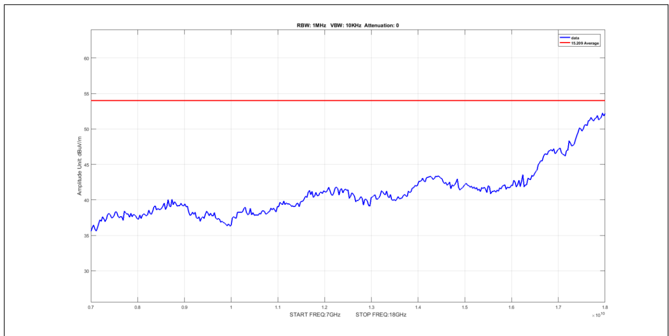
Plot 580. Undesirable Emissions, 8Omni Avg 7-18GHz 20M 5240 pow18
