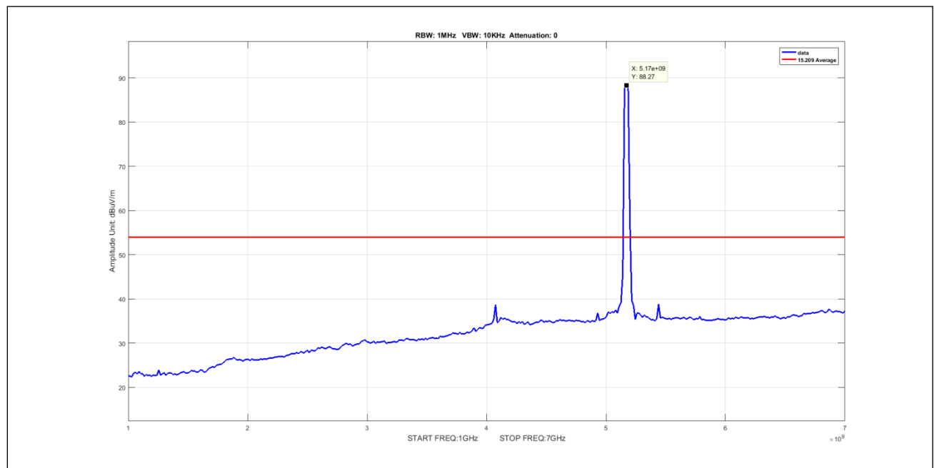
Plot 618. Undesirable Emissions, 90Sector Avg 1-7GHz 40M 5170 pow0
