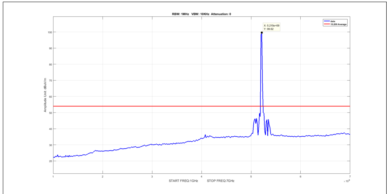
Plot 613. Undesirable Emissions, 90Sector Avg 1-7GHz 10M 5210 pow9
