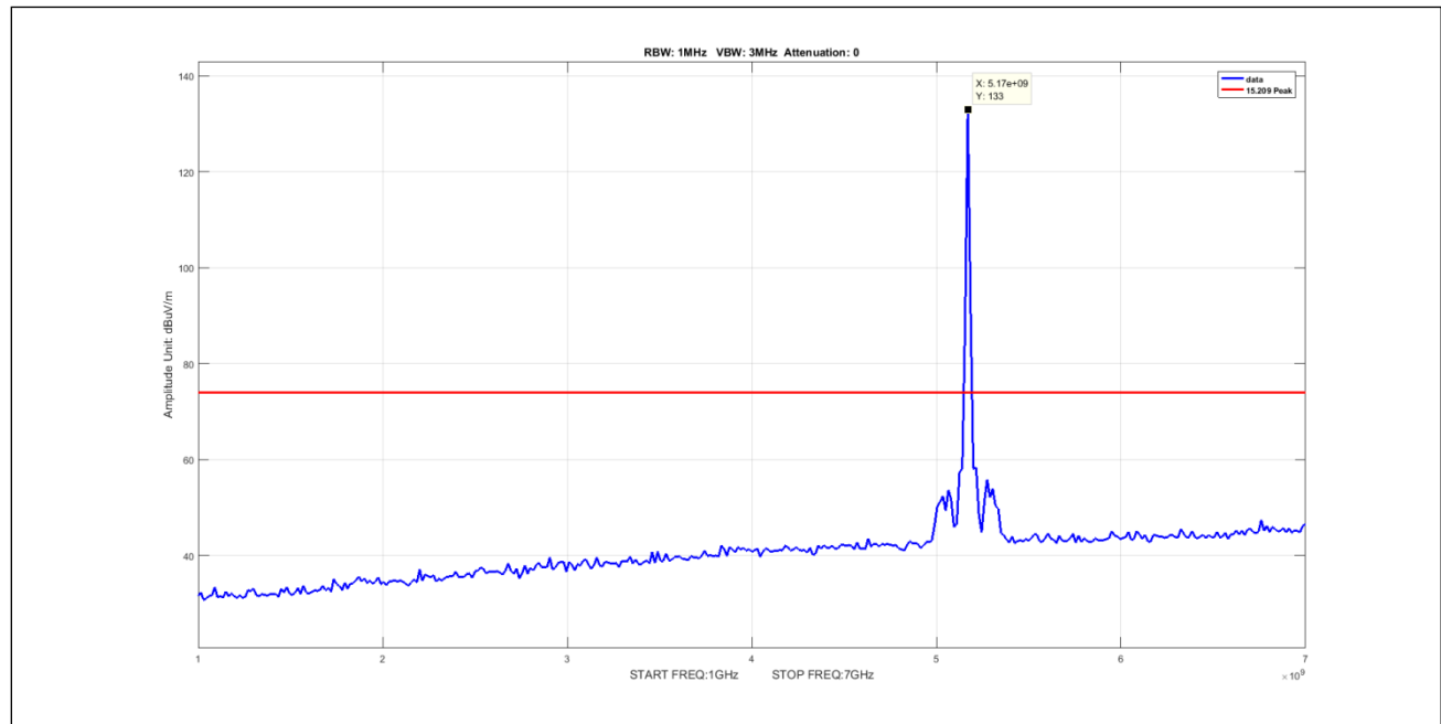
Plot 587. Undesirable Emissions, 8Omni Peak 1-7GHz 10M 5170 pow15
