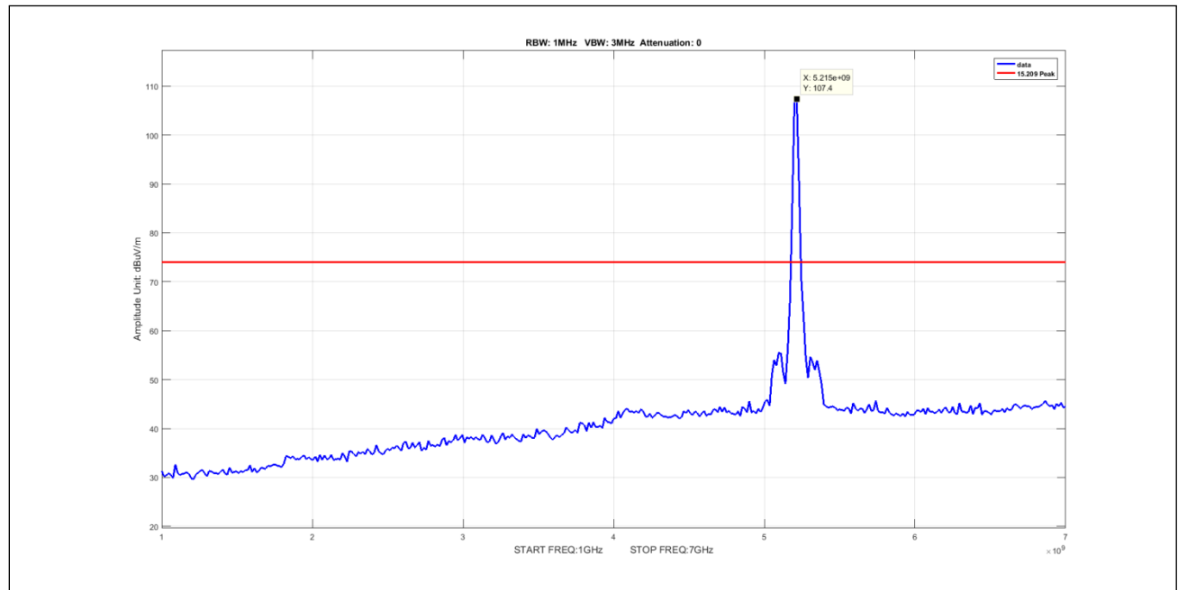
Plot 641. Undesirable Emissions, 90Sector Peak 1-7GHz 20M 5210 pow12
