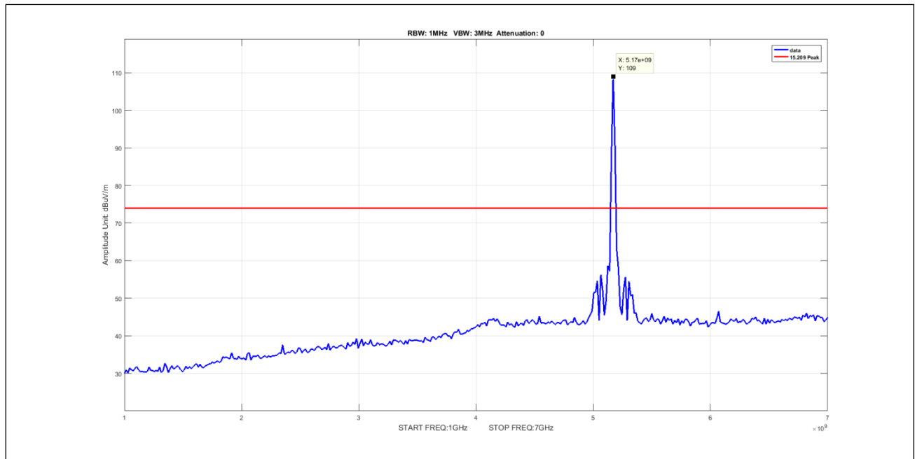
Plot 637. Undesirable Emissions, 90Sector Peak 1-7GHz 10M 5170 pow10
