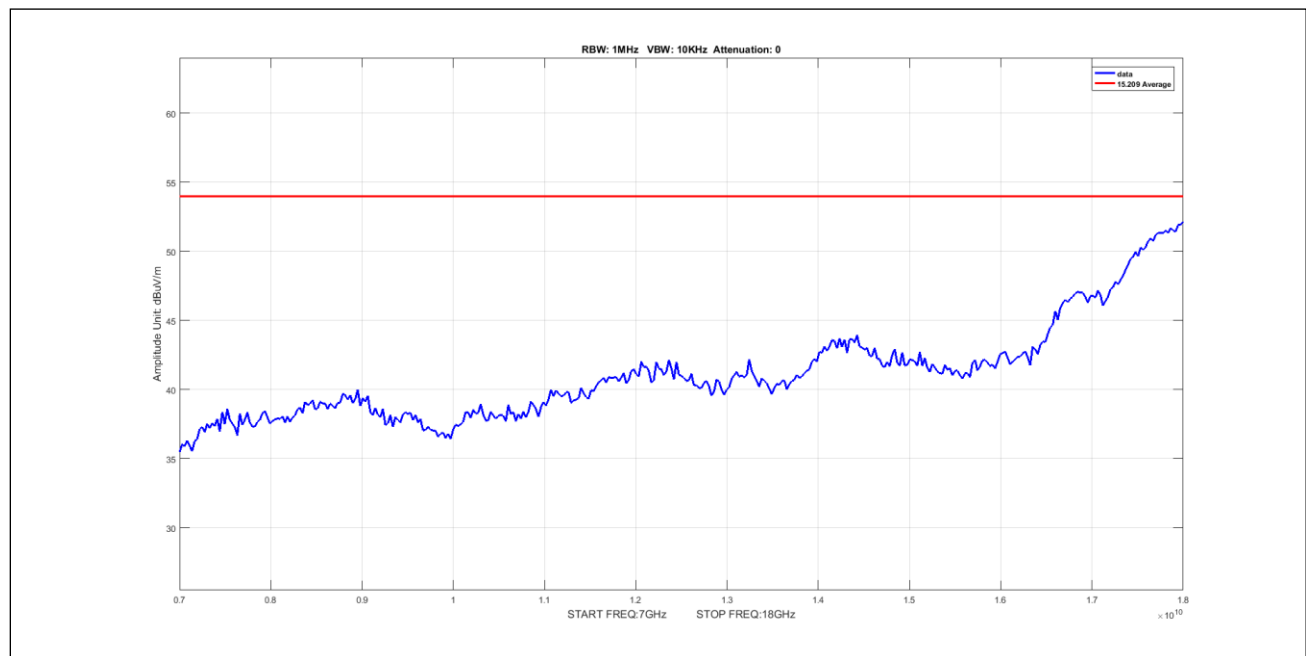
Plot 572. Undesirable Emissions, 8Omni Avg 7-18GHz 5M 5170 pow12
