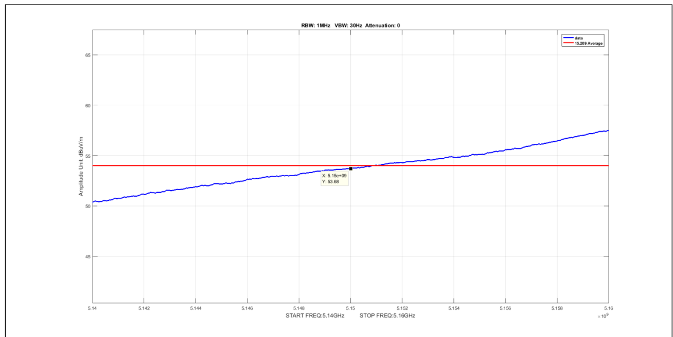
Plot 620. Undesirable Emissions, 90Sector Avg 1-7GHz 40M 5210 pow16 zoom
