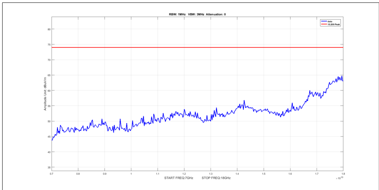
Plot 606. Undesirable Emissions, 8Omni Peak 7-18GHz 40M 5170 pow4
