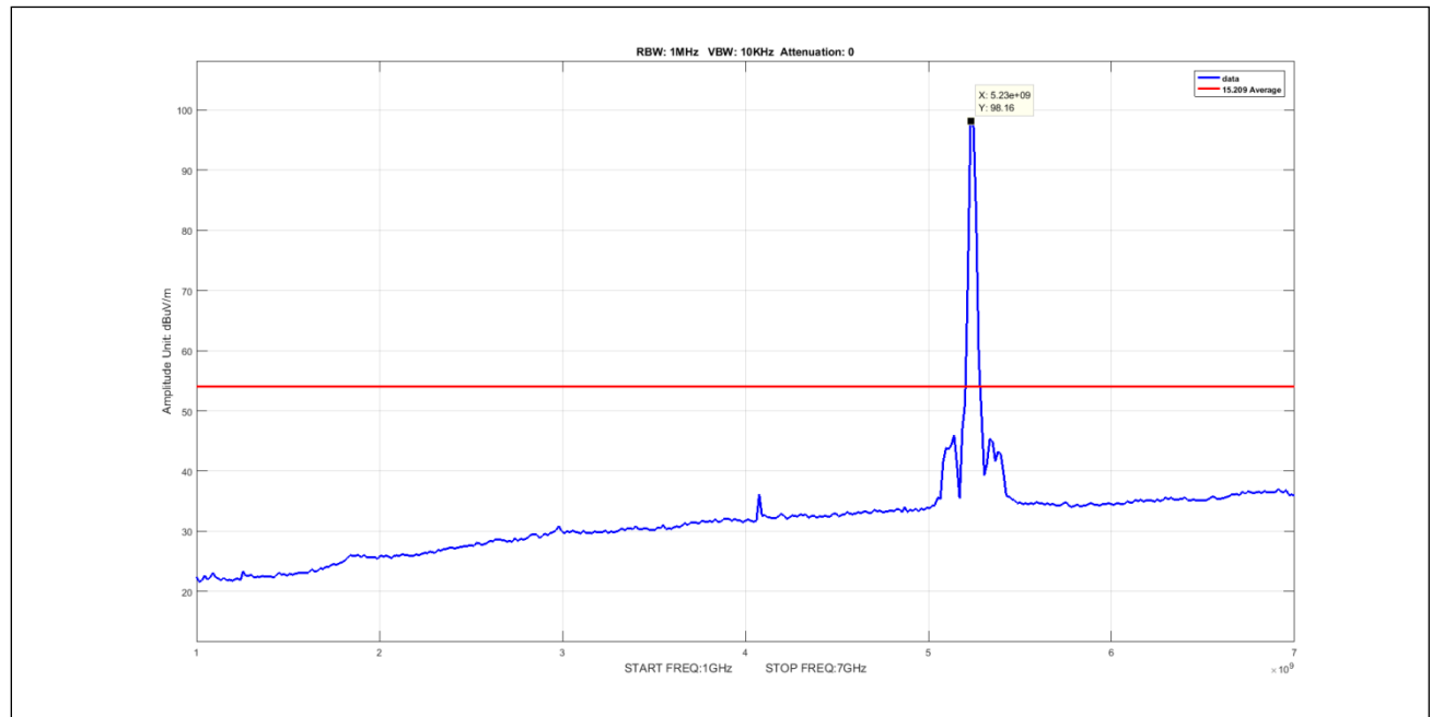
Plot 567. Undesirable Emissions, 8Omni Avg 1-7GHz 20M 5240 pow18
