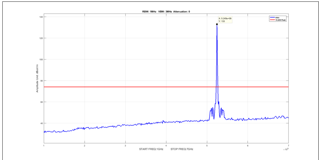
Plot 589. Undesirable Emissions, 8Omni Peak 1-7GHz 10M 5245 pow15
