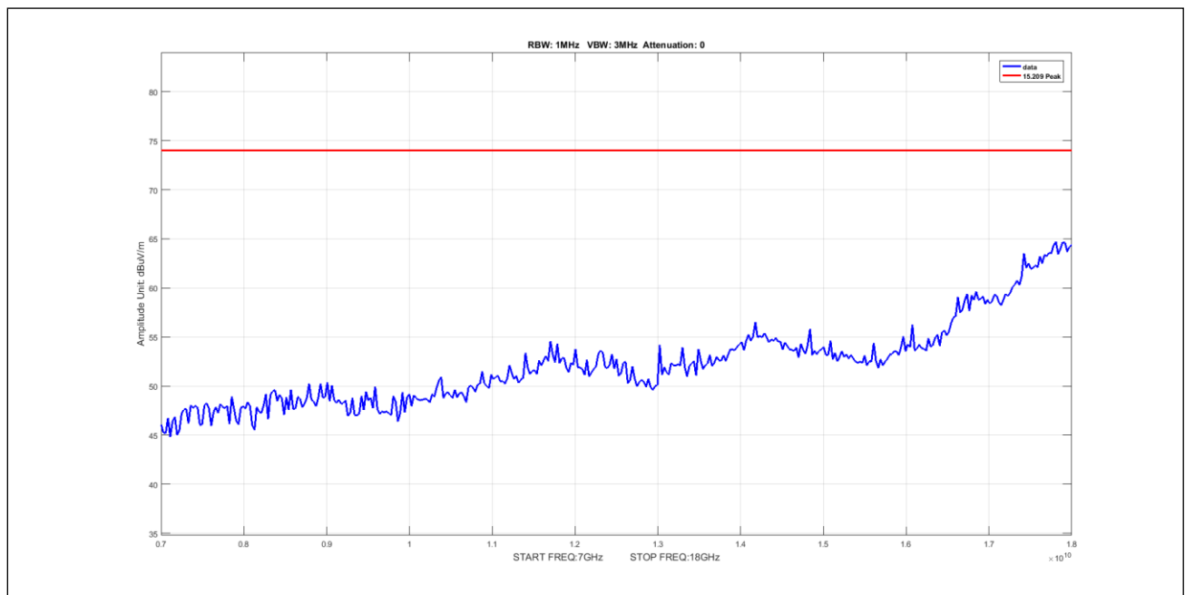
Plot 602. Undesirable Emissions, 8Omni Peak 7-18GHz 10M 5245 pow15
