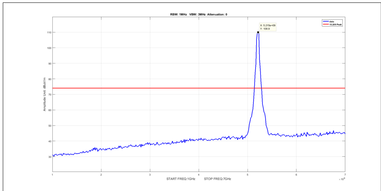
Plot 594. Undesirable Emissions, 8Omni Peak 1-7GHz 40M 5210 pow22
