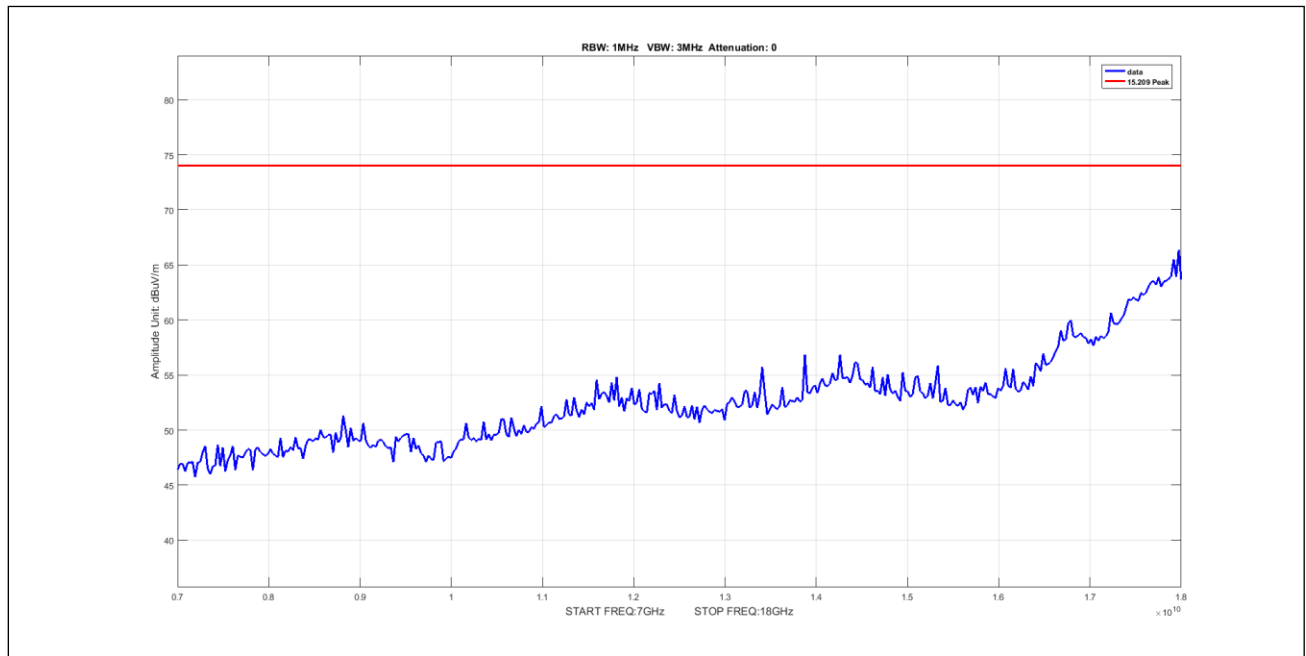
Plot 549. Undesirable Emissions, 5Omni Peak 7-18GHz 5M 5247.5 pow14
