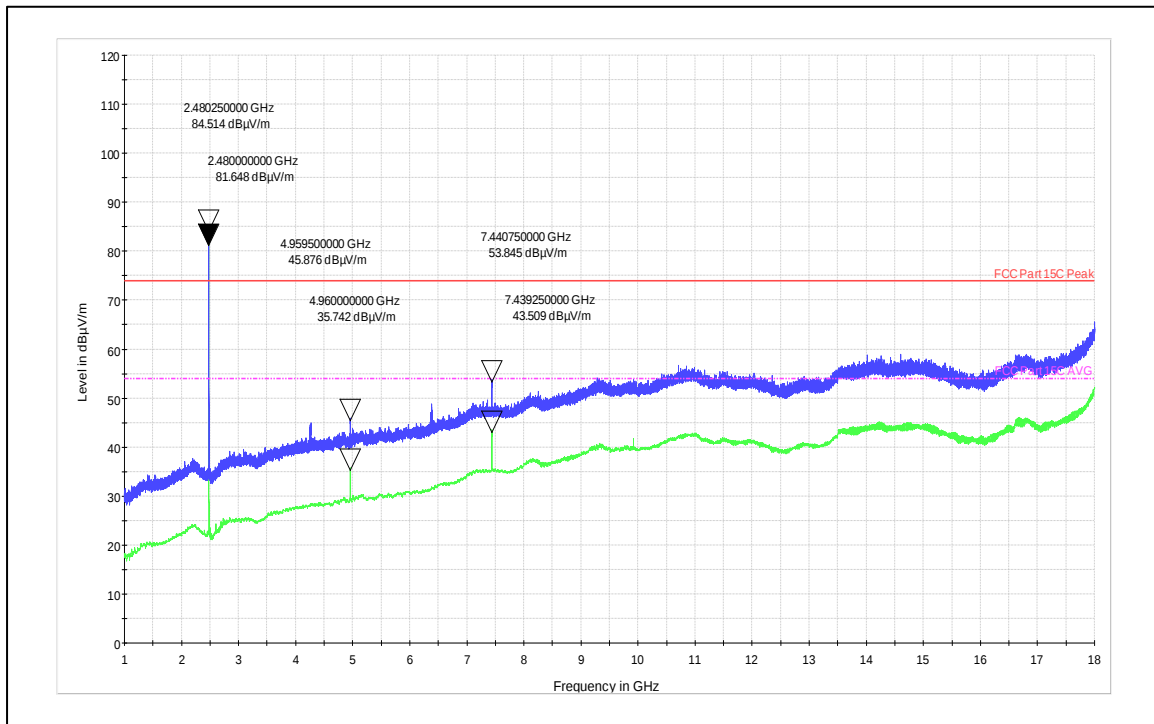
Channel Frequency 2480MHz Vertical Polarization
