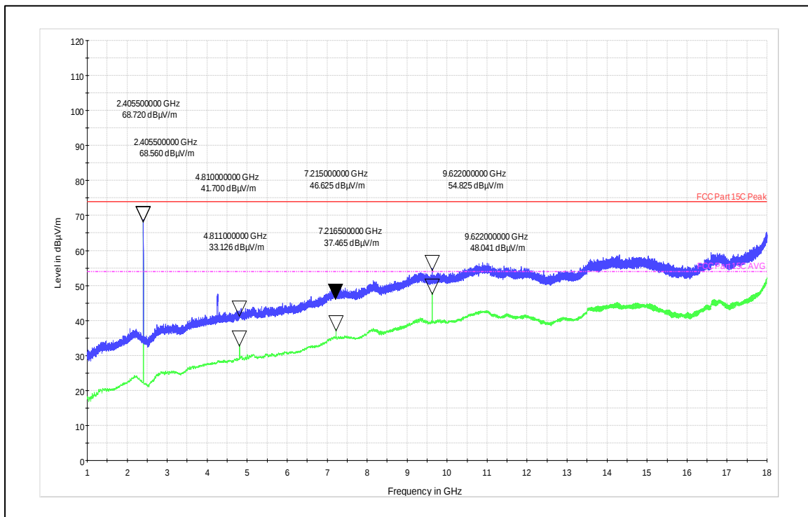
Channel Frequency 2405MHz Vertical Polarization
