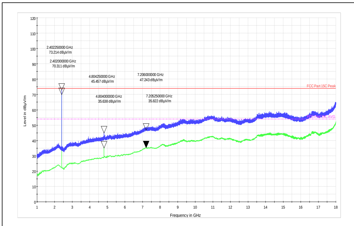
Channel Frequency 2402MHz Horizontal Polarization
