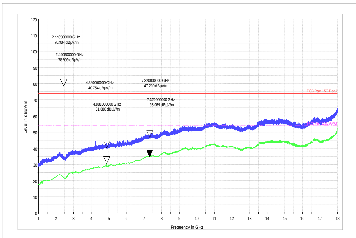
Channel Frequency 2440MHz Horizontal Polarization
