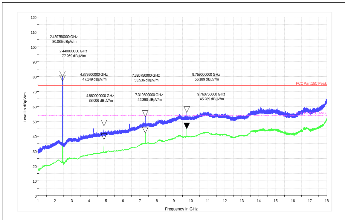
Channel Frequency 2440MHz Vertical Polarization
