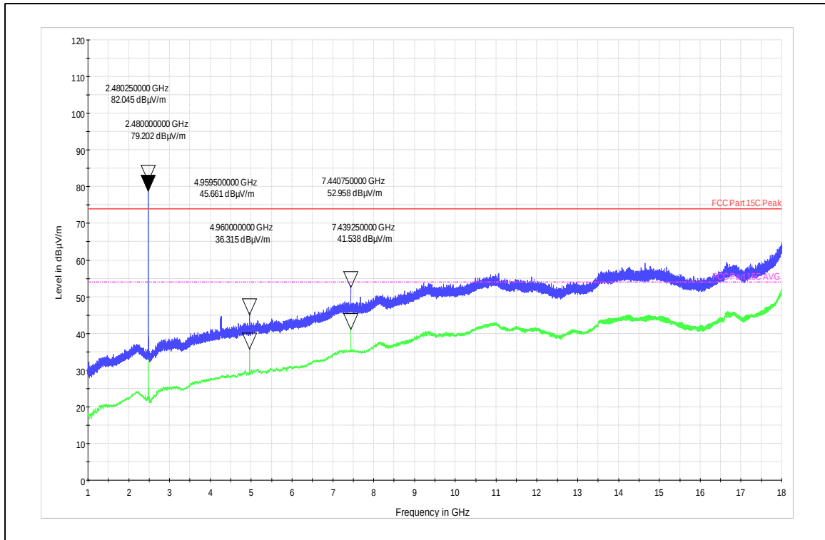
Channel Frequency 2480MHz Vertical Polarization
