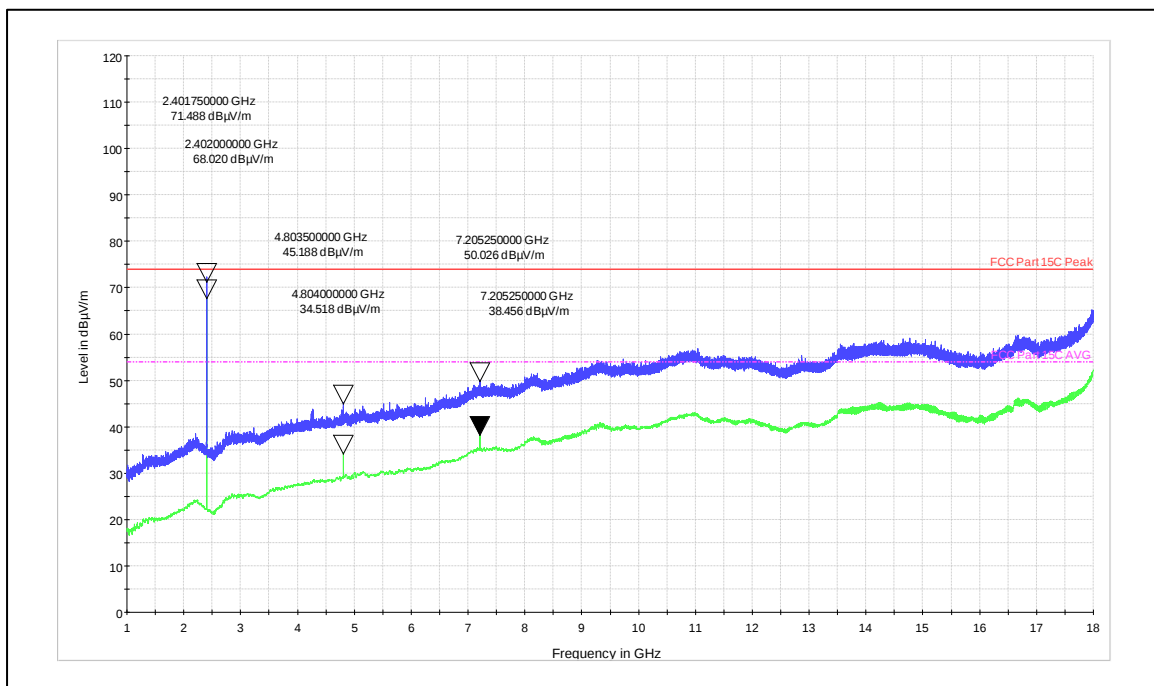
Channel Frequency 2402MHz Horizontal Polarization
