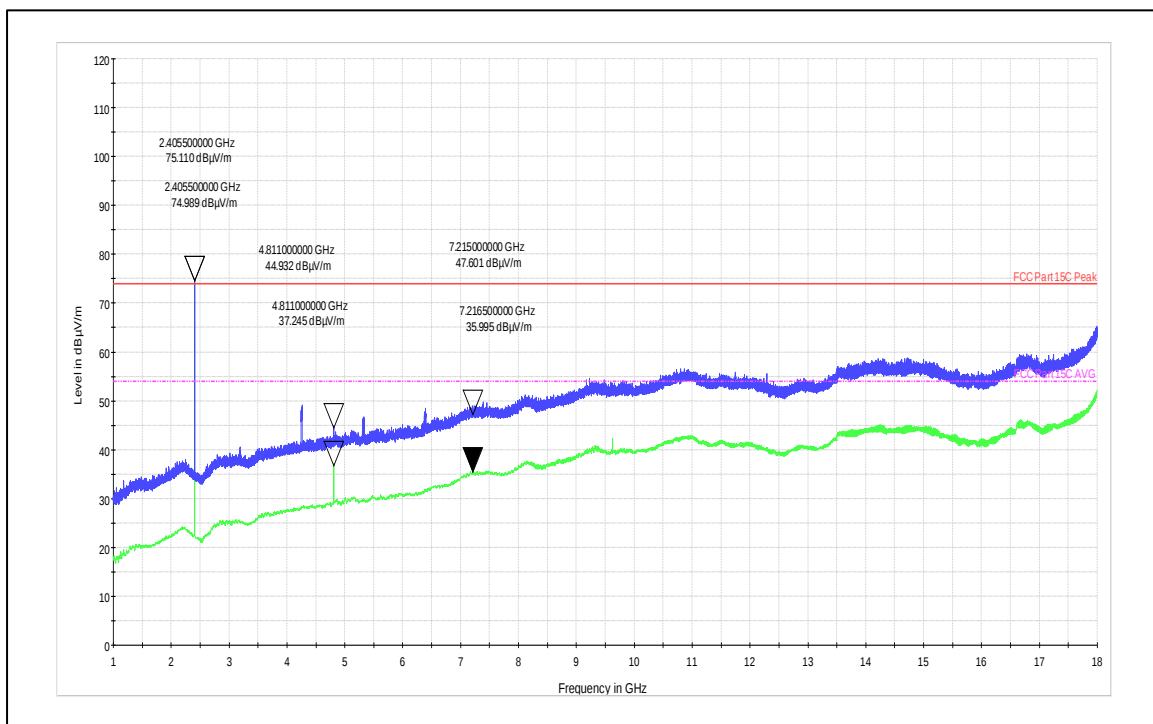
Channel Frequency 2405MHz Vertical Polarization
