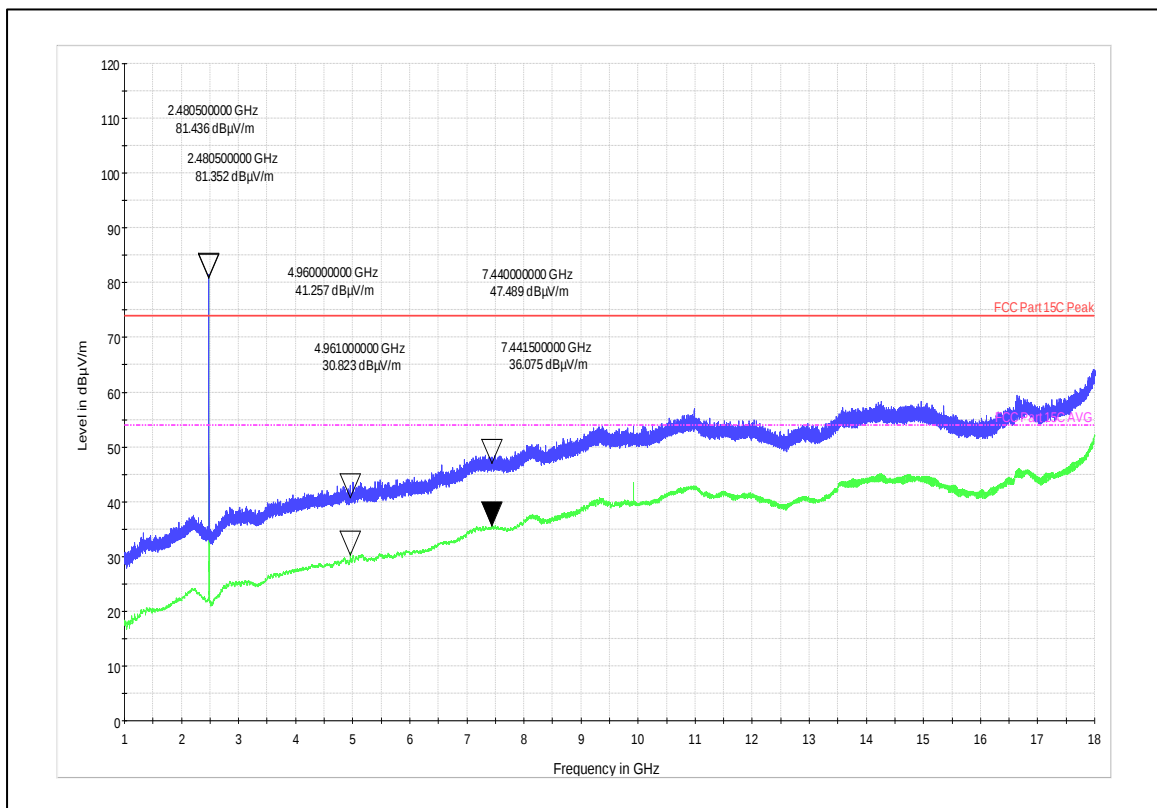
Channel Frequency 2480MHz Horizontal Polarization
