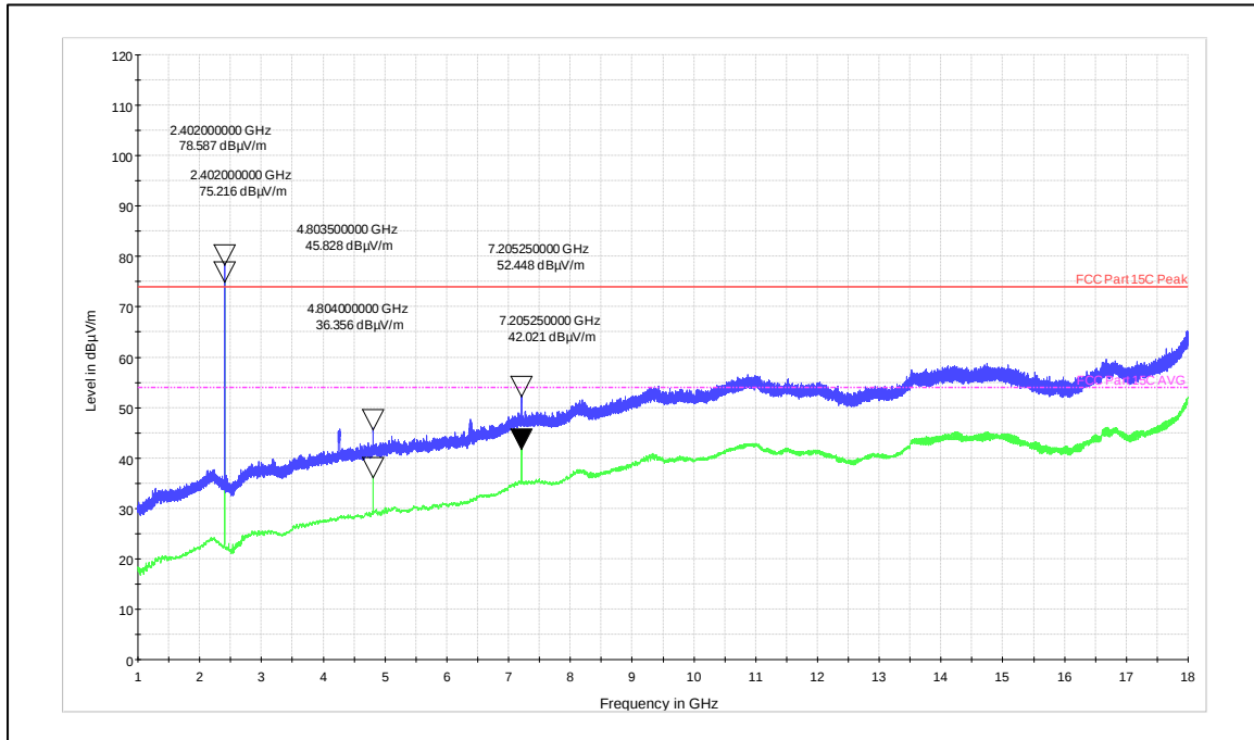
Channel Frequency 2402MHz Vertical Polarization
