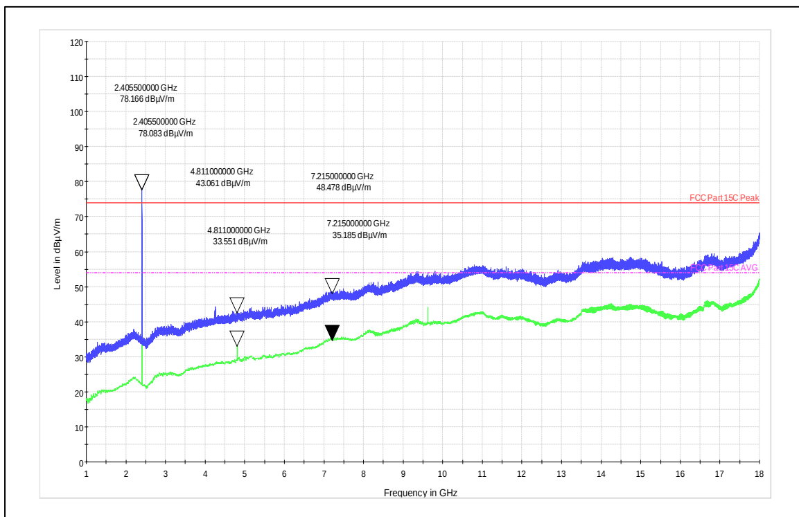
Channel Frequency 2405MHz Horizontal Polarization
