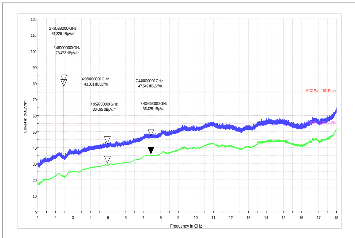
Channel Frequency 2480MHz Horizontal Polarization
