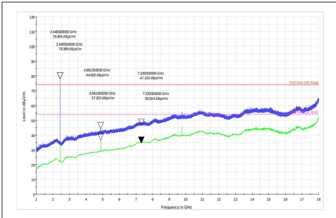
Channel Frequency 2440MHz Horizontal Polarization
