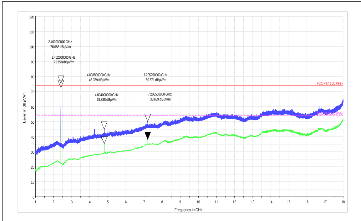
Channel Frequency 2402MHz Vertical Polarization
