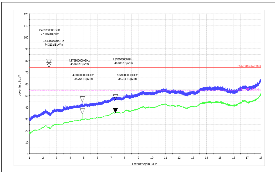
Channel Frequency 2440MHz Horizontal Polarization
