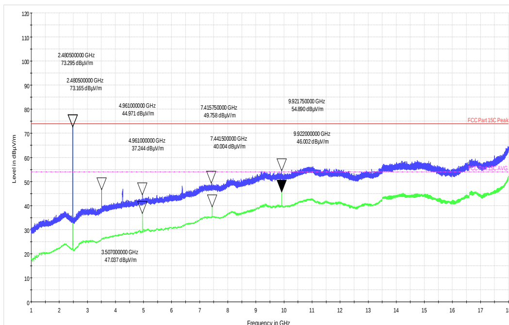
Channel Frequency 2480MHz Vertical Polarization
