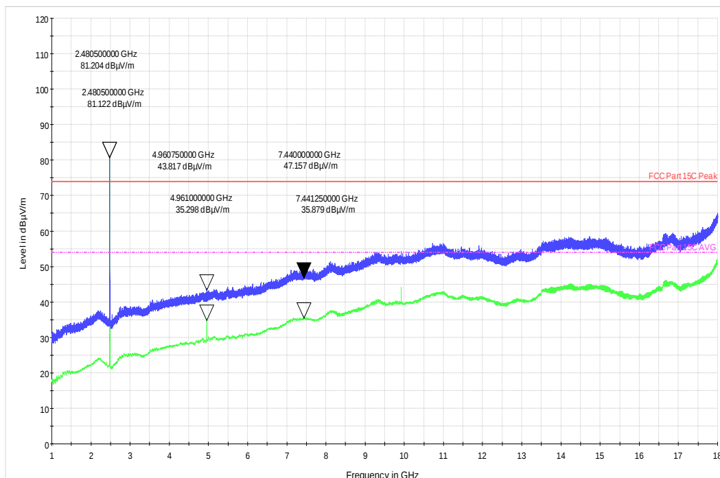
Channel Frequency 2480MHz Horizontal Polarization
