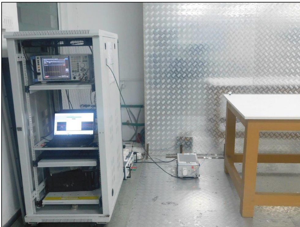
Test Setup of Conducted Emission on AC Power lines
