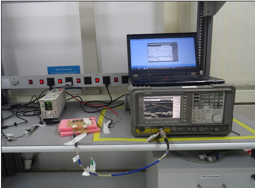
Conducted Test Setup
