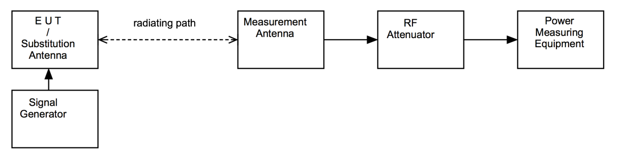
Figure vii Test Setup
