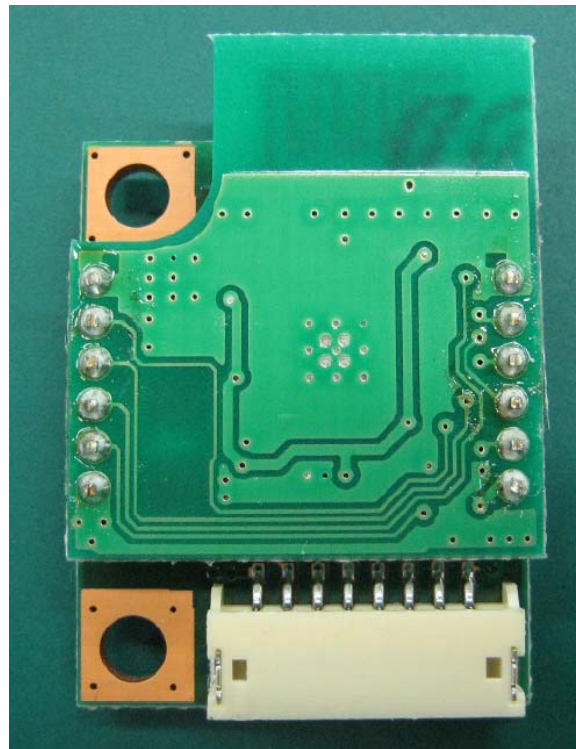
Receiver Bottom view
