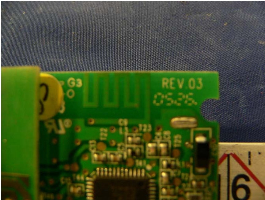
EUT – Antenna Close View
