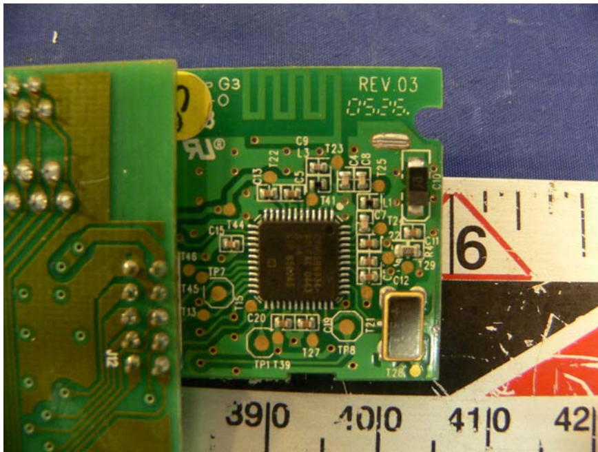
EUT – Transmitter Cover off, Component and Antenna View
