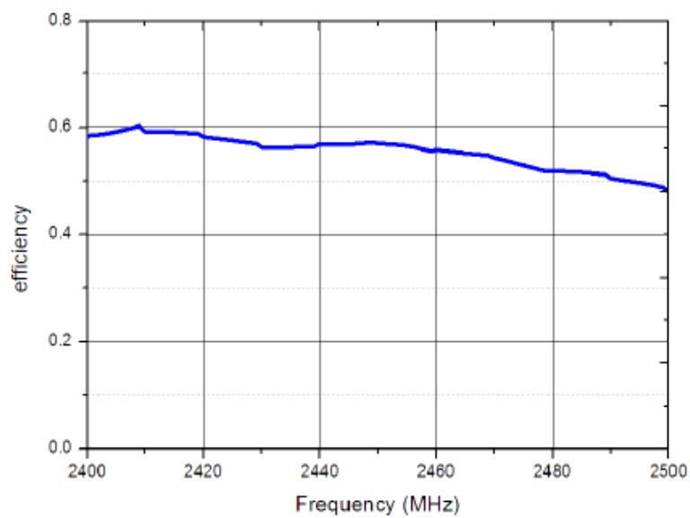
效率-频率 Efficiency-Frequency
