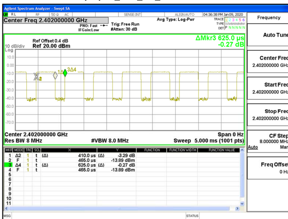
Duty Cycle_BLE_1M_LowCH00-2402
