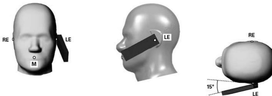
Fig-5.3 Illustration for Tilted Position
