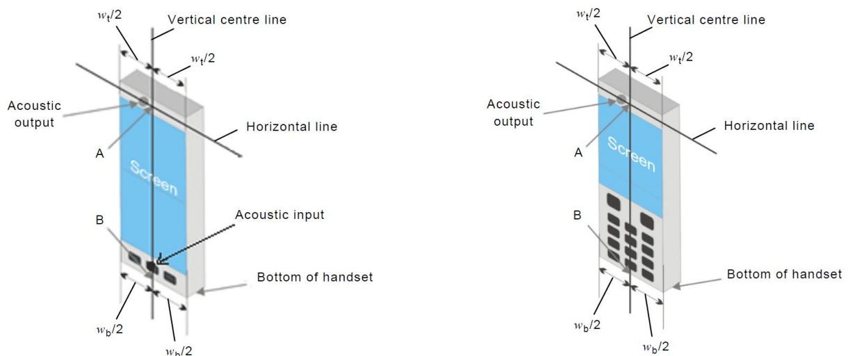
Fig-5.1 Illustration for Handset Vertical and Horizontal Reference Lines
