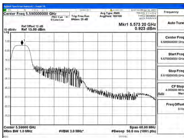
Mode:802.11be EHT40 Tone:26T Frequency:5590MHz Ant:Ant4
