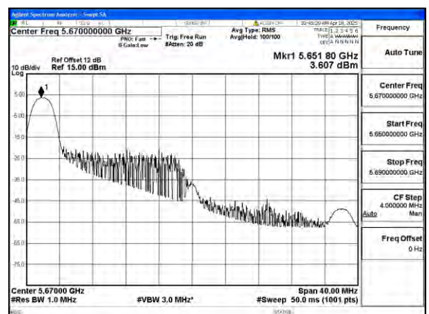
Mode:802.11ax HE40 Tone:26T Frequency:5670MHz Ant:Ant4
