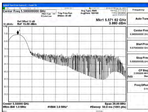
Mode:802.11be EHT20 Tone:26T Frequency:5580MHz Ant:Ant4
