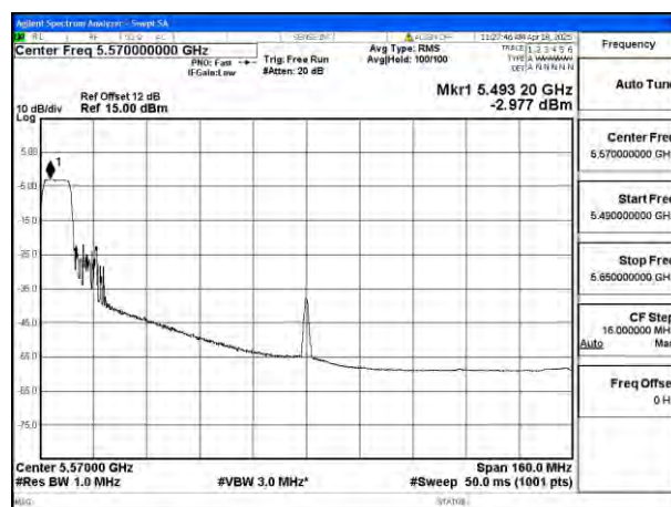
Mode:802.11ax HE160 Tone:106T Frequency:5570MHz Ant:Ant4
