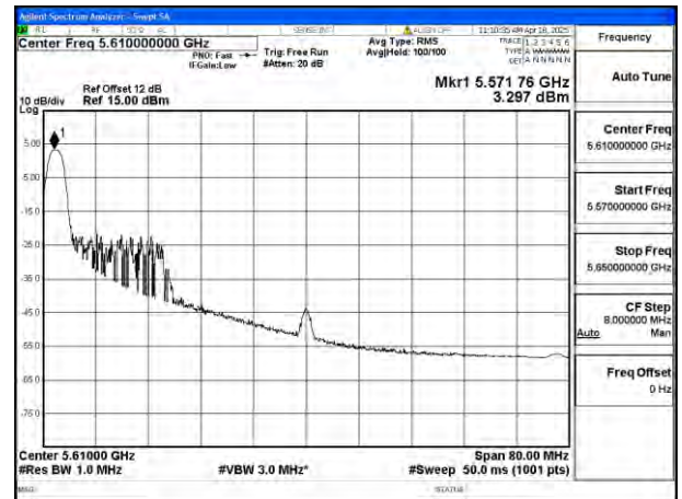
Mode:802.11ax HE80 Tone:26T Frequency:5610MHz Ant:Ant8
