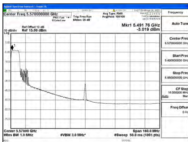
Mode:802.11ax HE160 Tone:106T Frequency:5570MHz Ant:Ant8
