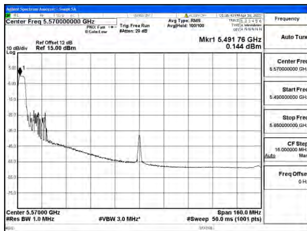
Mode:802.11be EHT160 Tone:52T Frequency:5570MHz Ant:Ant8
