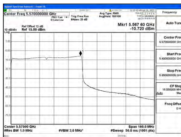
Mode:802.11ax HE160 Tone:996T Frequency:5570MHz Ant:Ant4
