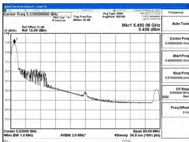
Mode:802.11be EHT80 Tone:26T Frequency:5530MHz Ant:Ant4
