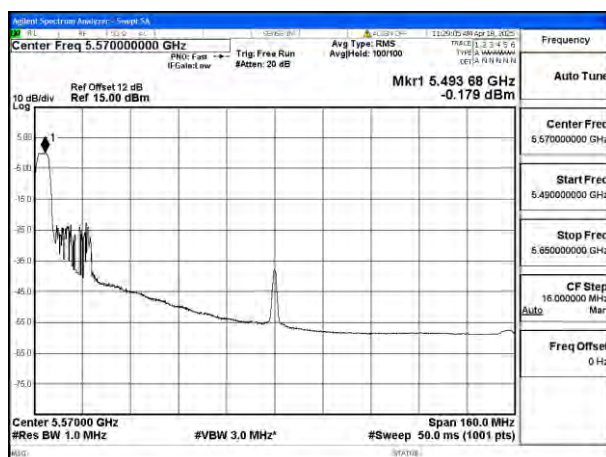
Mode:802.11ax HE160 Tone:52T Frequency:5570MHz Ant:Ant8
