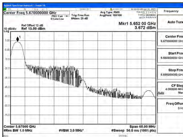
Mode:802.11ax HE40 Tone:26T Frequency:5670MHz Ant:Ant8
