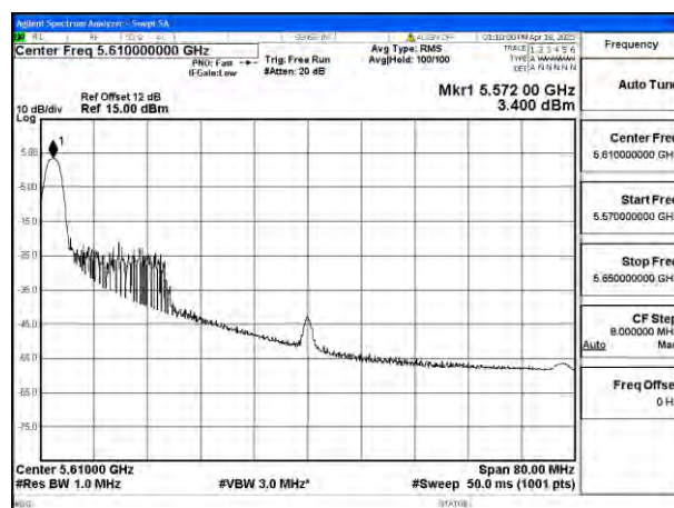
Mode:802.11be EHT80 Tone:26T Frequency:5610MHz Ant:Ant4
