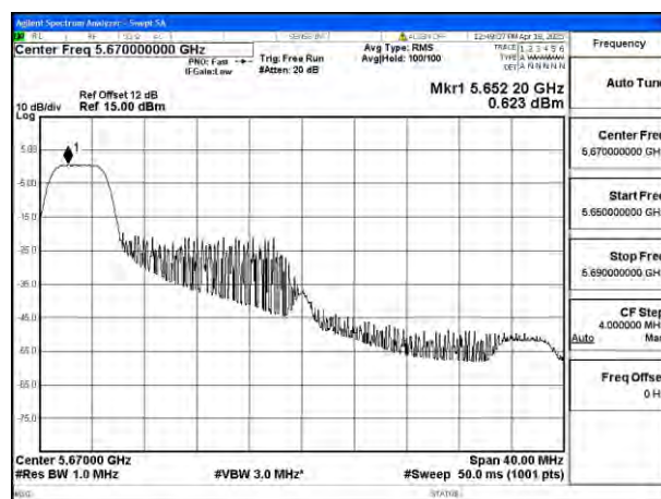
Mode:802.11be EHT40 Tone:26T Frequency:5670MHz Ant:Ant4
