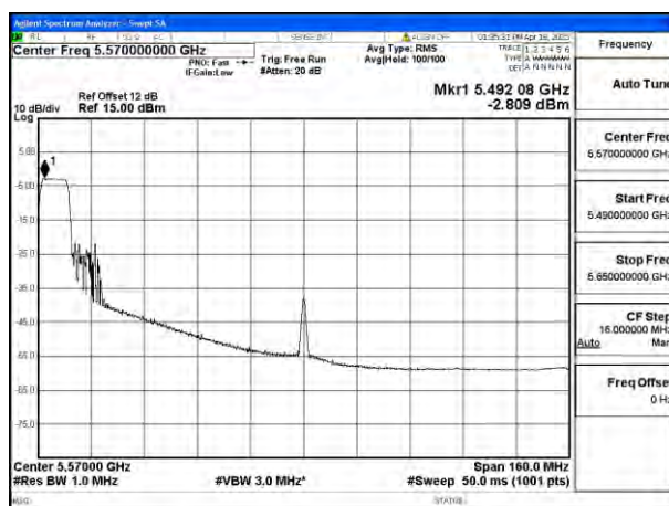
Mode:802.11be EHT160 Tone:106T Frequency:5570MHz Ant:Ant8
