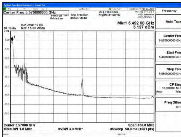
Mode:802.11be EHT160 Tone:26T Frequency:5570MHz Ant:Ant8
