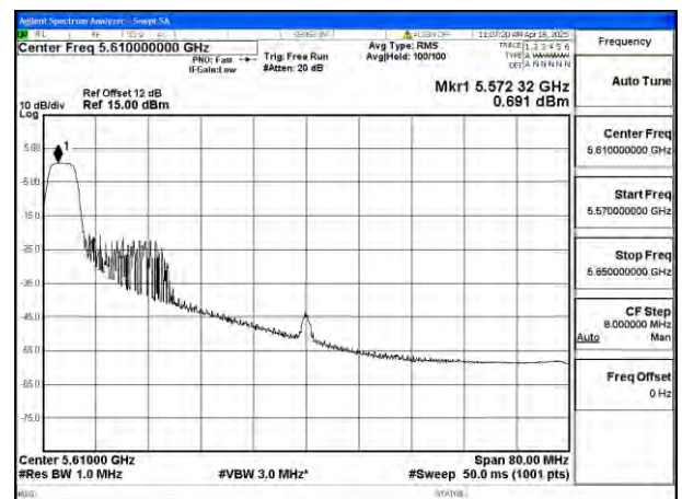
Mode:802.11ax HE80 Tone:52T Frequency:5610MHz Ant:Ant8
