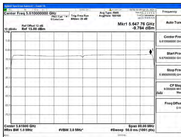
Mode:802.11be EHT80 Tone:996T Frequency:5610MHz Ant:Ant4
