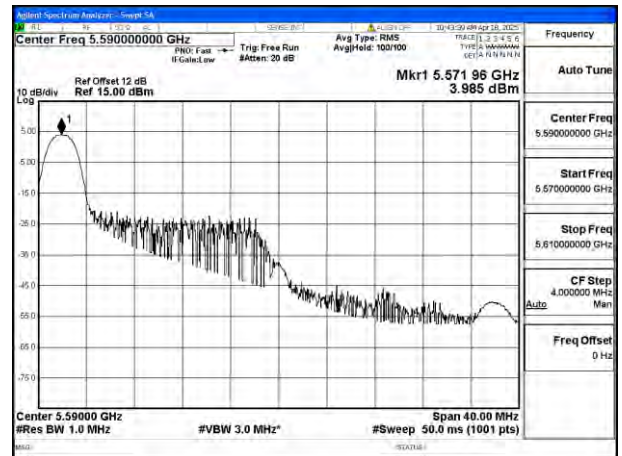
Mode:802.11ax HE40 Tone:26T Frequency:5590MHz Ant:Ant8
