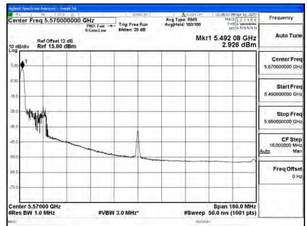
Mode:802.11be EHT160 Tone:26T Frequency:5570MHz Ant:Ant4
