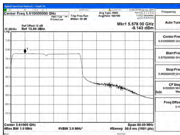
Mode:802.11be EHT80 Tone:484T Frequency:5610MHz Ant:Ant4
