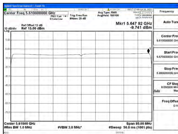
Mode:802.11be EHT80 Tone:996T Frequency:5610MHz Ant:Ant8
