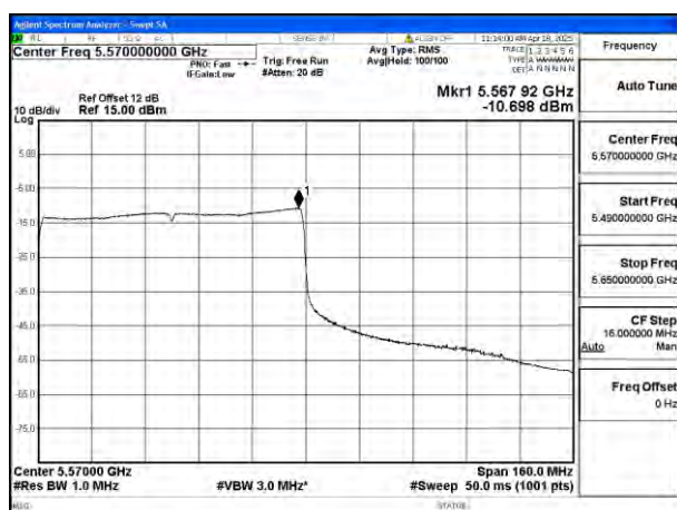
Mode:802.11ax HE160 Tone:996T Frequency:5570MHz Ant:Ant8
