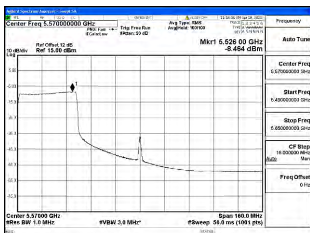
Mode:802.11ax HE160 Tone:484T Frequency:5570MHz Ant:Ant8
