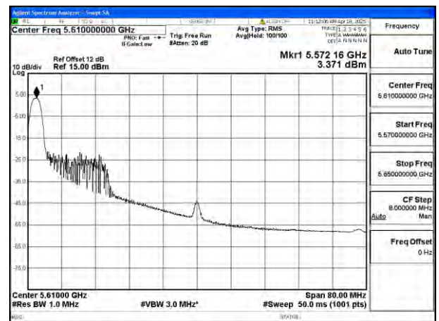
Mode:802.11ax HE80 Tone:26T Frequency:5610MHz Ant:Ant4
