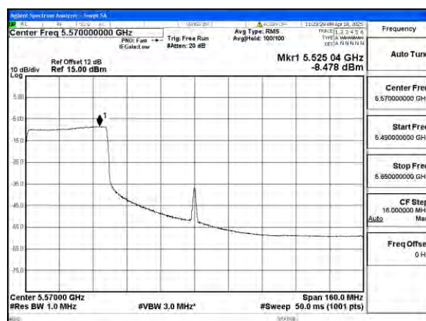
Mode:802.11ax HE160 Tone:484T Frequency:5570MHz Ant:Ant4
