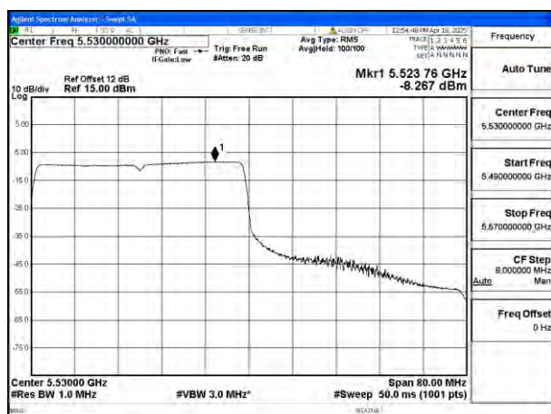
Mode:802.11be EHT80 Tone:484T Frequency:5530MHz Ant:Ant4
