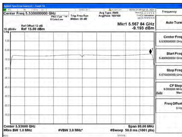
Mode:802.11be EHT80 Tone:996T Frequency:5530MHz Ant:Ant8
