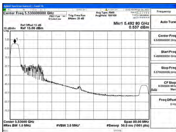
Mode:802.11be EHT80 Tone:52T Frequency:5530MHz Ant:Ant8
