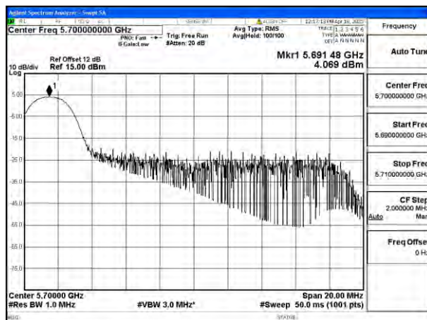
Mode:802.11be EHT20 Tone:26T Frequency:5700MHz Ant:Ant8
