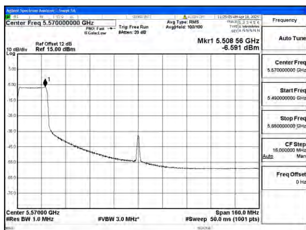
Mode:802.11ax HE160 Tone:242T Frequency:5570MHz Ant:Ant8
