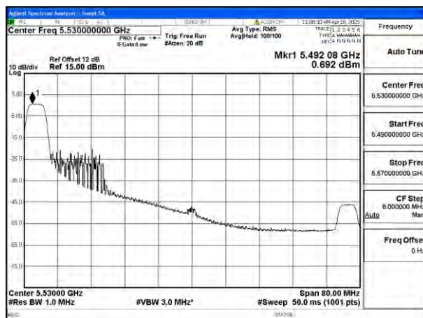
Mode:802.11ax HE80 Tone:52T Frequency:5530MHz Ant:Ant8
