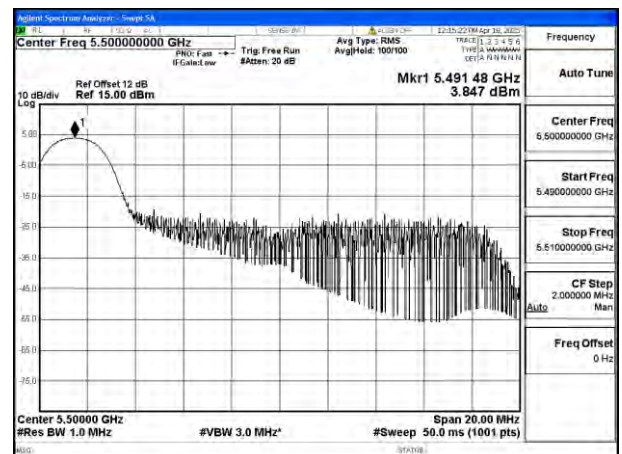
Mode:802.11be EHT20 Tone:26T Frequency:5500MHz Ant:Ant4
