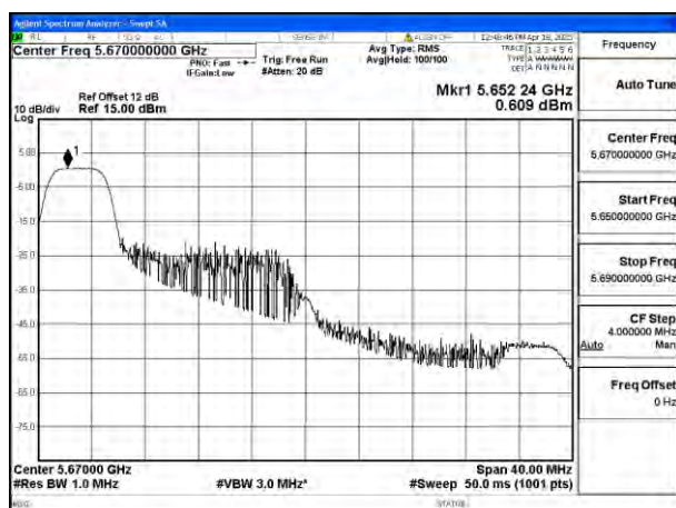
Mode:802.11be EHT40 Tone:26T Frequency:5670MHz Ant:Ant8
