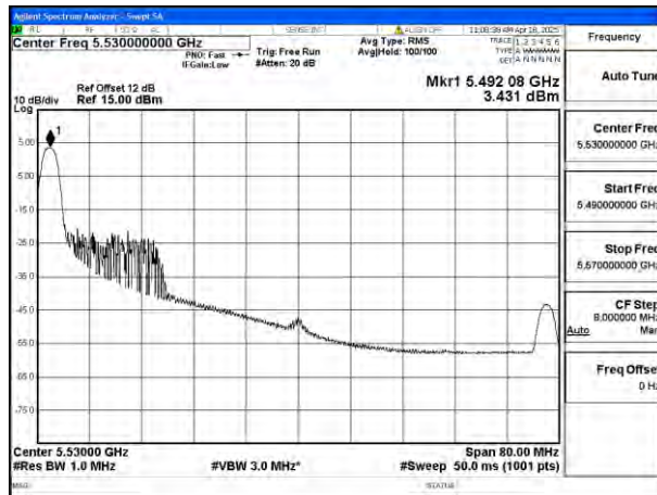
Mode:802.11ax HE80 Tone:26T Frequency:5530MHz Ant:Ant8
