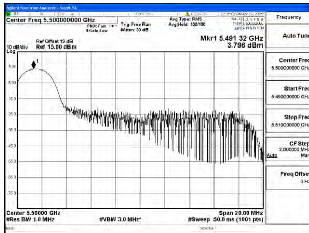
Mode:802.11be EHT20 Tone:26T Frequency:5500MHz Ant:Ant8
