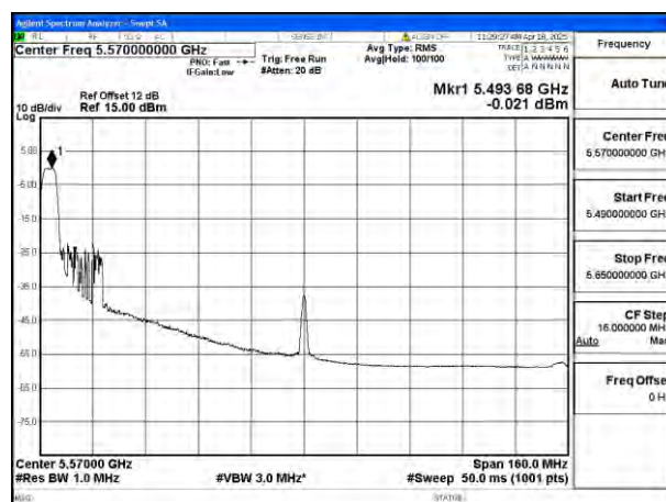
Mode:802.11ax HE160 Tone:52T Frequency:5570MHz Ant:Ant4
