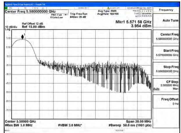
Mode:802.11be EHT20 Tone:26T Frequency:5580MHz Ant:Ant8
