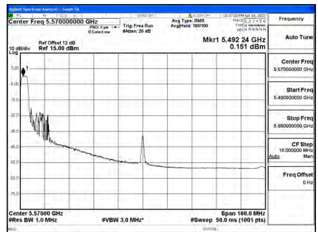
Mode:802.11be EHT160 Tone:52T Frequency:5570MHz Ant:Ant4
