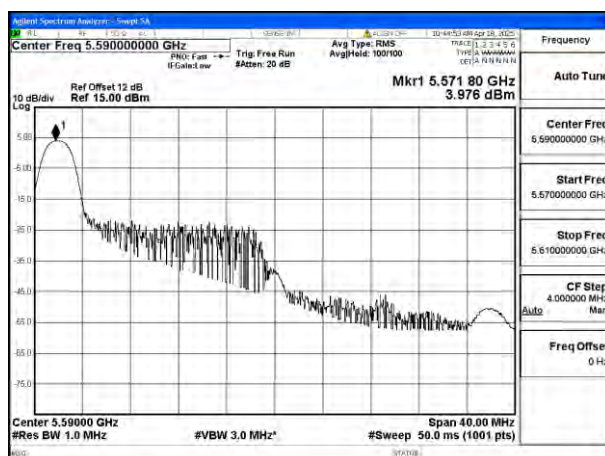
Mode:802.11ax HE40 Tone:26T Frequency:5590MHz Ant:Ant4
