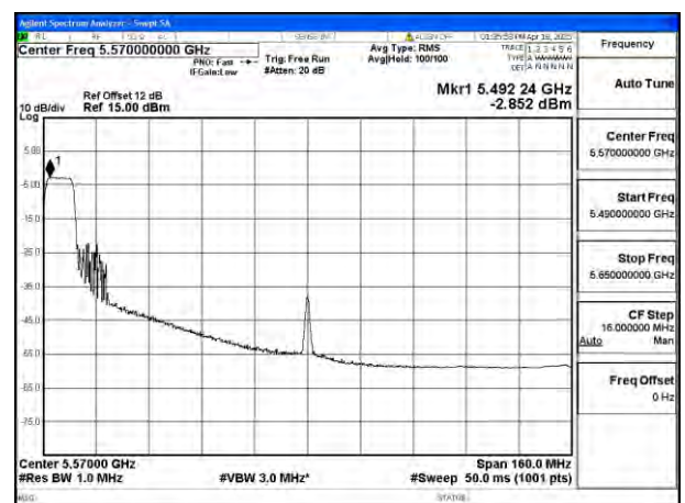
Mode:802.11be EHT160 Tone:106T Frequency:5570MHz Ant:Ant4
