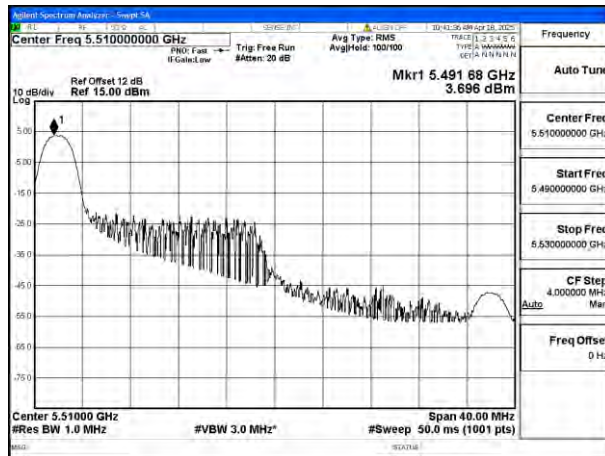
Mode:802.11ax HE40 Tone:26T Frequency:5510MHz Ant:Ant8
