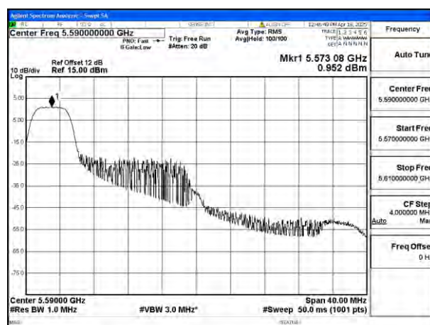
Mode:802.11be EHT40 Tone:26T Frequency:5590MHz Ant:Ant8
