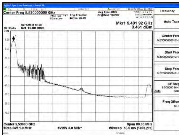
Mode:802.11ax HE80 Tone:26T Frequency:5530MHz Ant:Ant4
