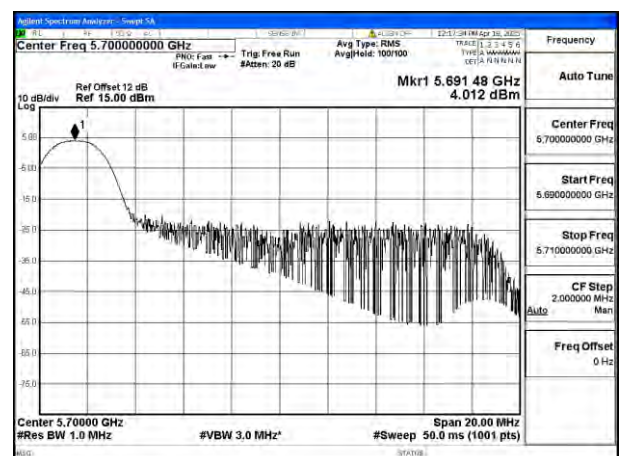
Mode:802.11be EHT20 Tone:26T Frequency:5700MHz Ant:Ant4
