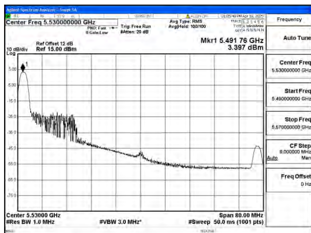
Mode:802.11be EHT80 Tone:26T Frequency:5530MHz Ant:Ant8
