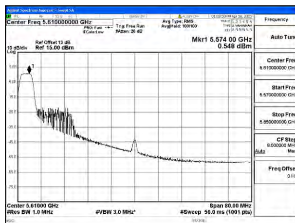
Mode:802.11be EHT80 Tone:52T Frequency:5610MHz Ant:Ant8
