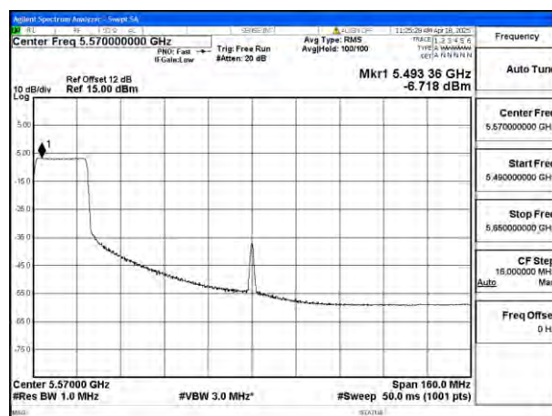
Mode:802.11ax HE160 Tone:242T Frequency:5570MHz Ant:Ant4
