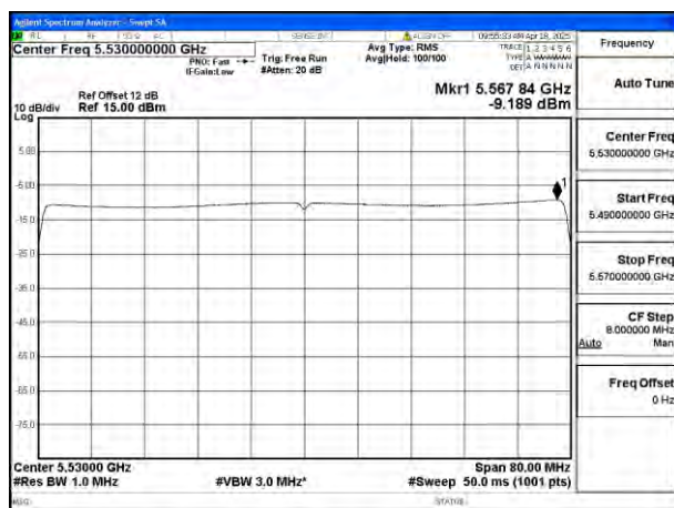
Mode:802.11be EHT80 Tone:996T Frequency:5530MHz Ant:Ant4
