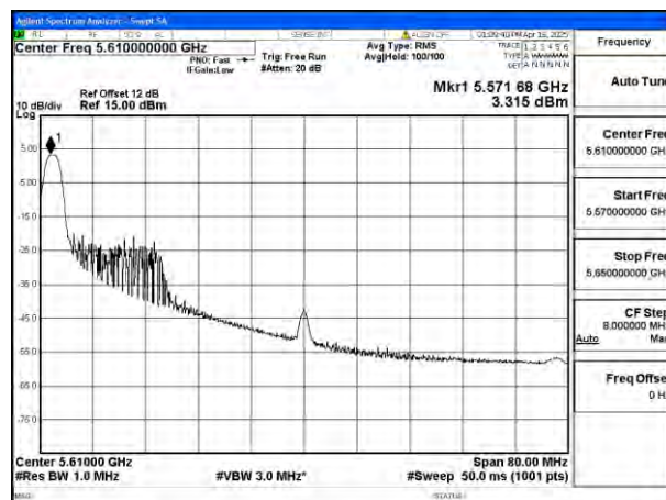
Mode:802.11be EHT80 Tone:26T Frequency:5610MHz Ant:Ant8
