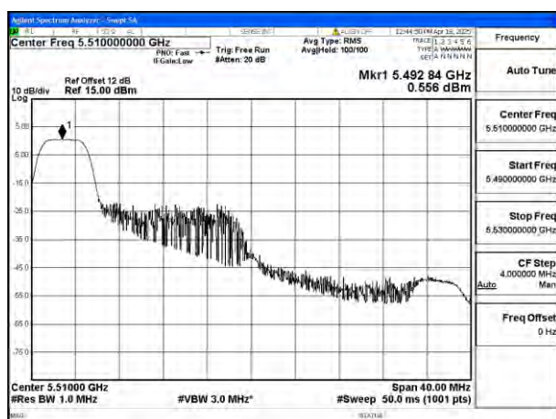
Mode:802.11be EHT40 Tone:26T Frequency:5510MHz Ant:Ant8
