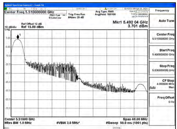
Mode:802.11ax HE40 Tone:26T Frequency:5510MHz Ant:Ant4
