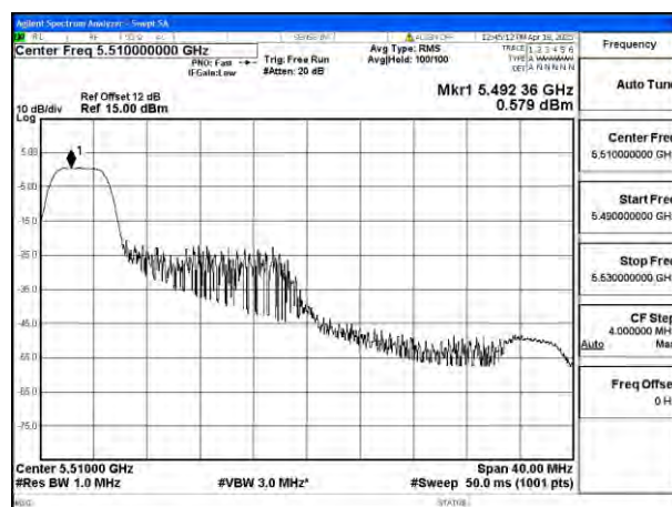
Mode:802.11be EHT40 Tone:26T Frequency:5510MHz Ant:Ant4
