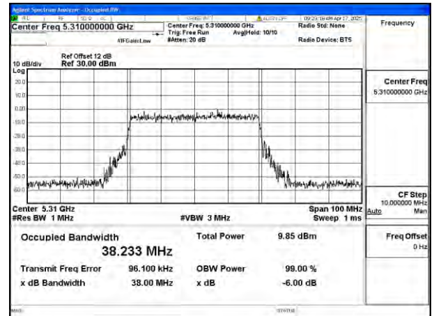
Mode:802.11be EHT40 Frequency:5310MHz Ant:Ant8
