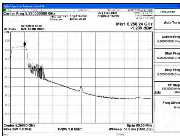
Mode:802.11ax HE80 Tone:106T Frequency:5290MHz Ant:Ant8
