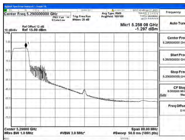
Mode:802.11ax HE80 Tone:106T Frequency:5290MHz Ant:Ant4
