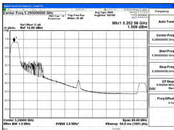
Mode:802.11ax HE80 Tone:52T Frequency:5290MHz Ant:Ant8
