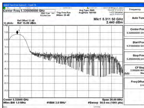
Mode:802.11ax HE20 Tone:26T Frequency:5320MHz Ant:Ant4
