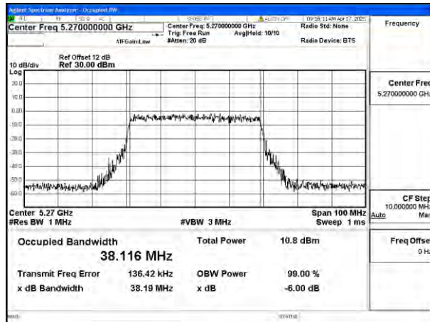
Mode:802.11be EHT40 Frequency:5270MHz Ant:Ant8
