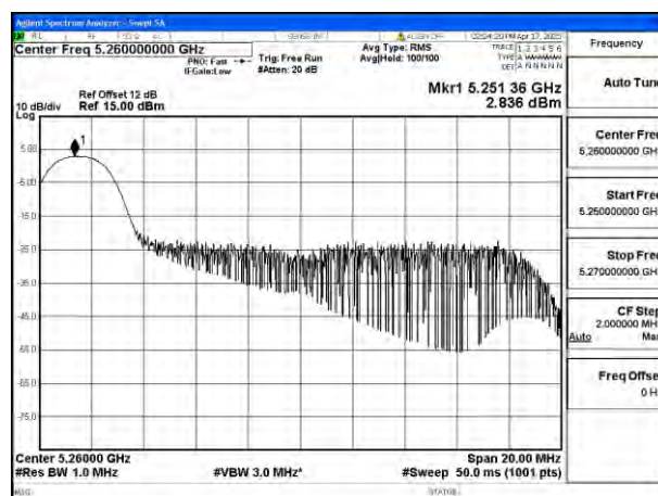
Mode:802.11ax HE20 Tone:26T Frequency:5260MHz Ant:Ant4
