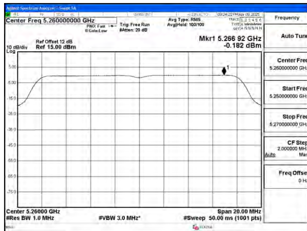
Mode:802.11a Frequency:5260MHz Ant:Ant8
