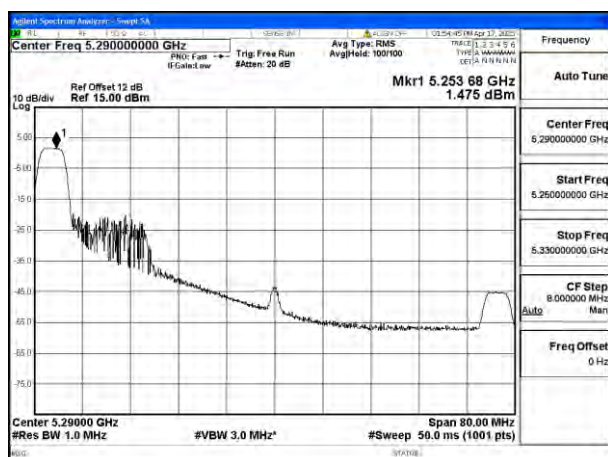
Mode:802.11be EHT80 Tone:52T Frequency:5290MHz Ant:Ant8
