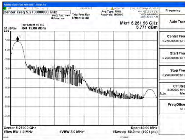
Mode:802.11be EHT40 Tone:26T Frequency:5270MHz Ant:Ant8
