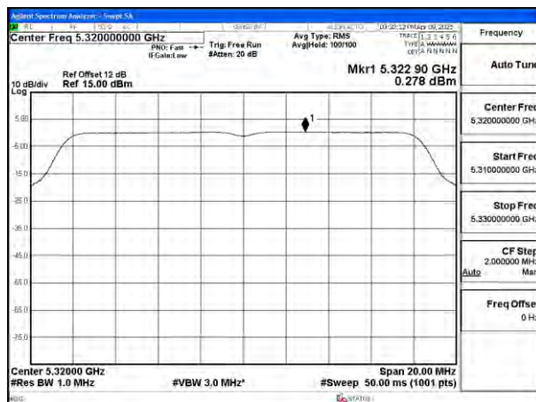
Mode:802.11a Frequency:5320MHz Ant:Ant8
