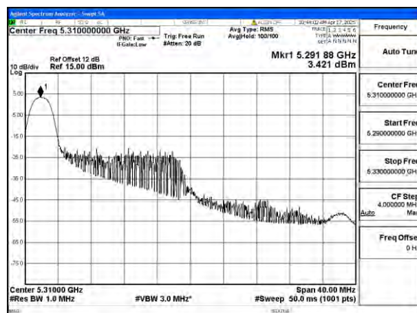
Mode:802.11ax HE40 Tone:26T Frequency:5310MHz Ant:Ant8
