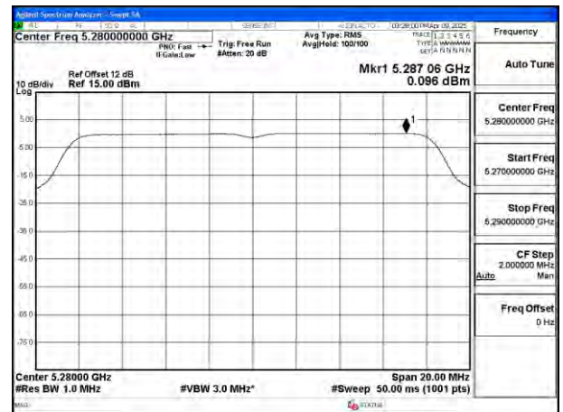
Mode:802.11a Frequency:5280MHz Ant:Ant8
