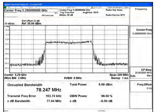
Mode:802.11ax HE80 Frequency:5290MHz Ant:Ant4
