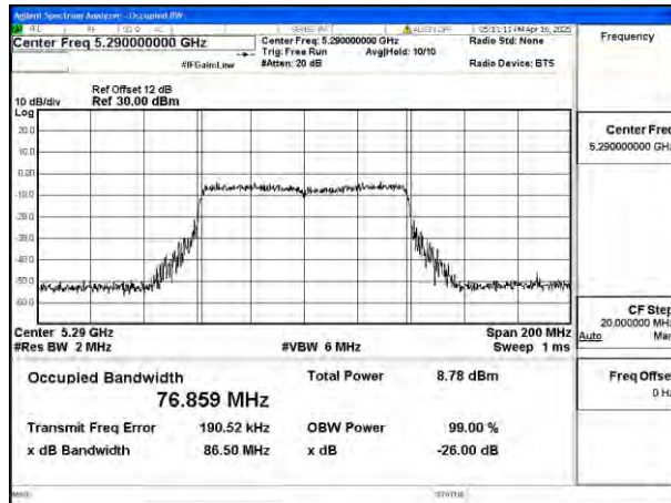
Mode:802.11ac VHT80 Frequency:5290MHz Ant:Ant8
