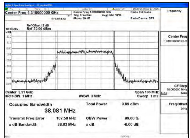
Mode:802.11be EHT40 Frequency:5310MHz Ant:Ant4
