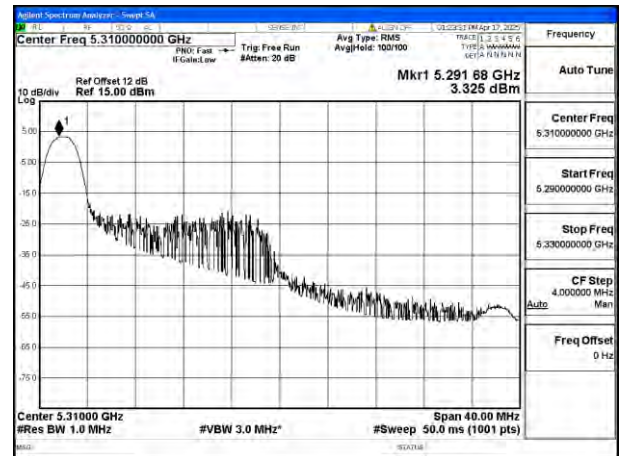
Mode:802.11be EHT40 Tone:26T Frequency:5310MHz Ant:Ant8
