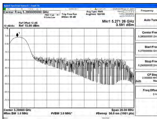
Mode:802.11ax HE20 Tone:26T Frequency:5280MHz Ant:Ant8
