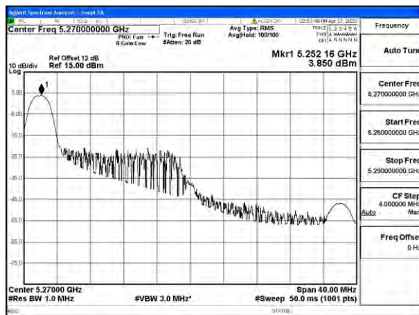
Mode:802.11be EHT40 Tone:26T Frequency:5270MHz Ant:Ant4
