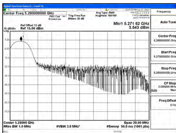
Mode:802.11ax HE20 Tone:26T Frequency:5280MHz Ant:Ant4
