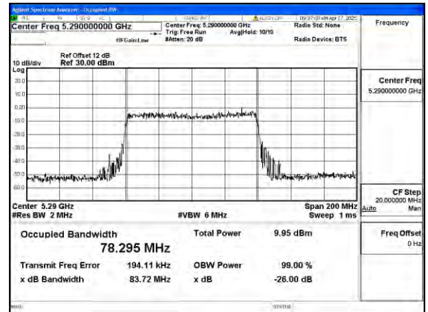
Mode:802.11be EHT80 Frequency:5290MHz Ant:Ant4
