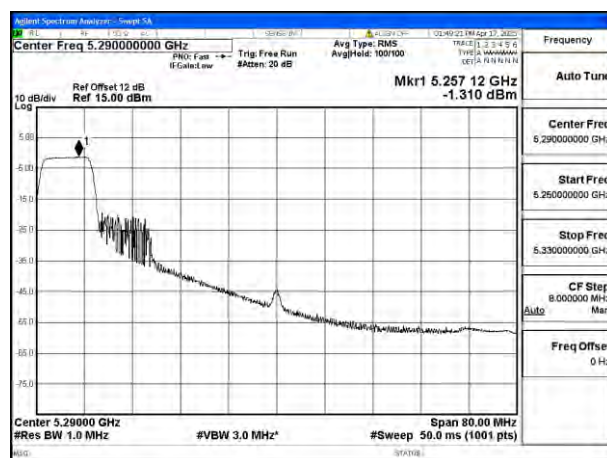
Mode:802.11be EHT80 Tone:106T Frequency:5290MHz Ant:Ant4
