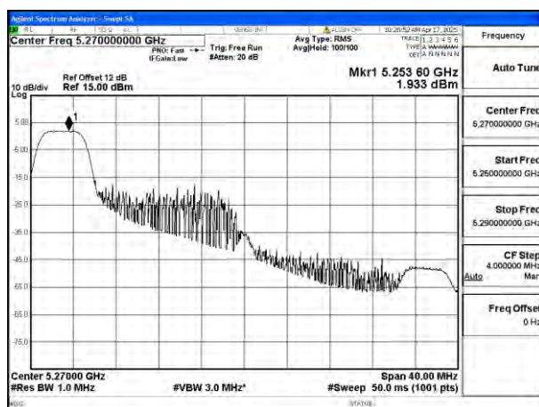
Mode:802.11ax HE40 Tone:52T
