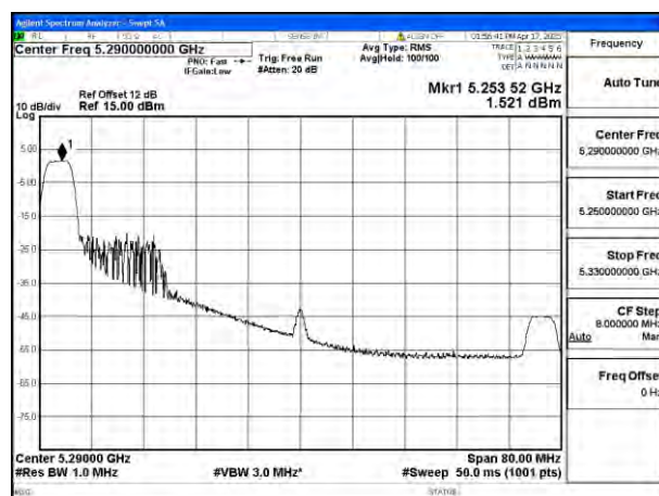
Mode:802.11be EHT80 Tone:52T Frequency:5290MHz Ant:Ant4
