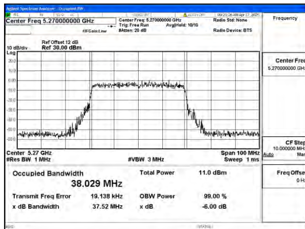
Mode:802.11be EHT40 Frequency:5270MHz Ant:Ant4
