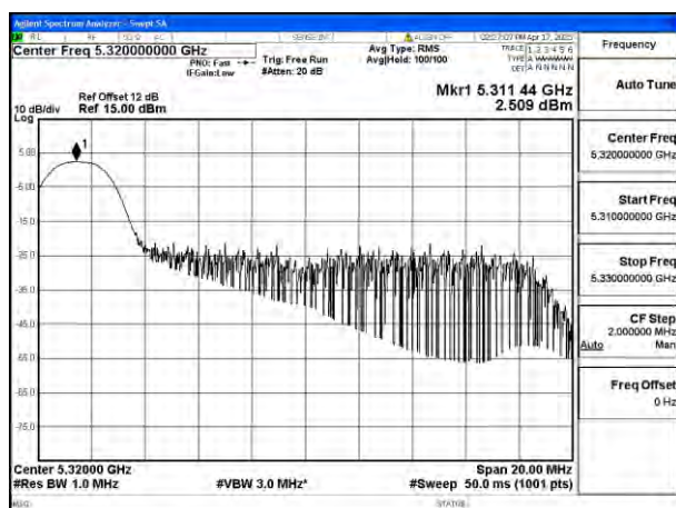
Mode:802.11ax HE20 Tone:26T Frequency:5320MHz Ant:Ant8
