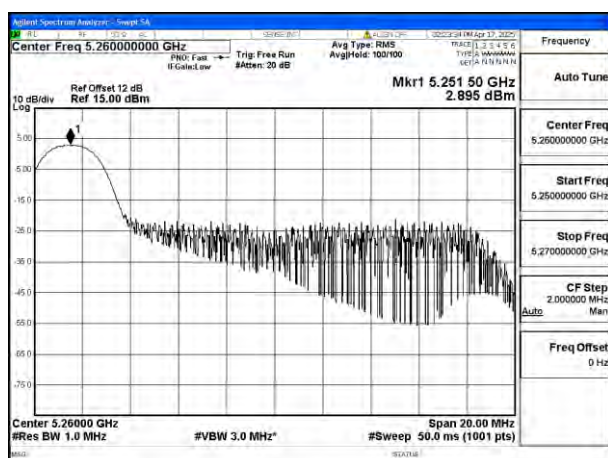
Mode:802.11ax HE20 Tone:26T Frequency:5260MHz Ant:Ant8
