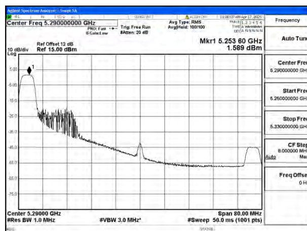
Mode:802.11ax HE80 Tone:52T Frequency:5290MHz Ant:Ant4
