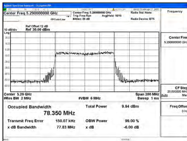
Mode:802.11ax HE80 Frequency:5290MHz Ant:Ant8
