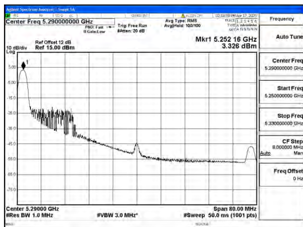
Mode:802.11be EHT80 Tone:26T Frequency:5290MHz Ant:Ant8
