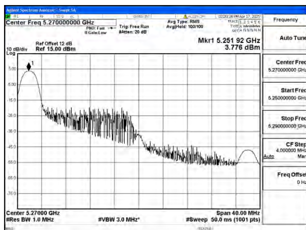
Mode:802.11ax HE40 Tone:26T Frequency:5270MHz Ant:Ant8
