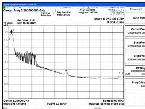
Mode:802.11ax HE80 Tone:26T Frequency:5290MHz Ant:Ant4
