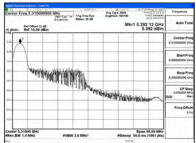
Mode:802.11be EHT40 Tone:26T Frequency:5310MHz Ant:Ant4
