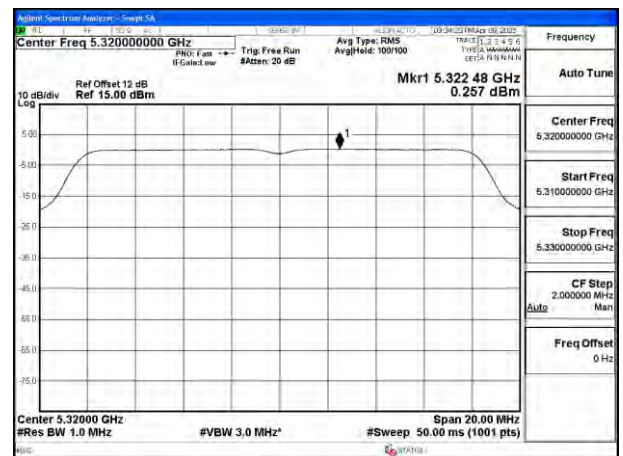
Mode:802.11a Frequency:5320MHz Ant:Ant4
