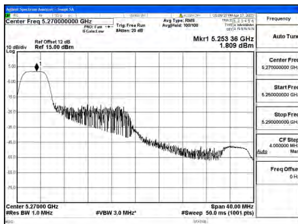
Mode:802.11be EHT40 Tone:52T Frequency:5270MHz Ant:Ant8
