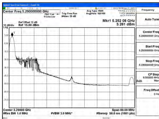
Mode:802.11ax HE80 Tone:26T Frequency:5290MHz Ant:Ant8
