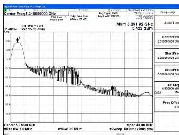
Mode:802.11ax HE40 Tone:26T Frequency:5310MHz Ant:Ant4
