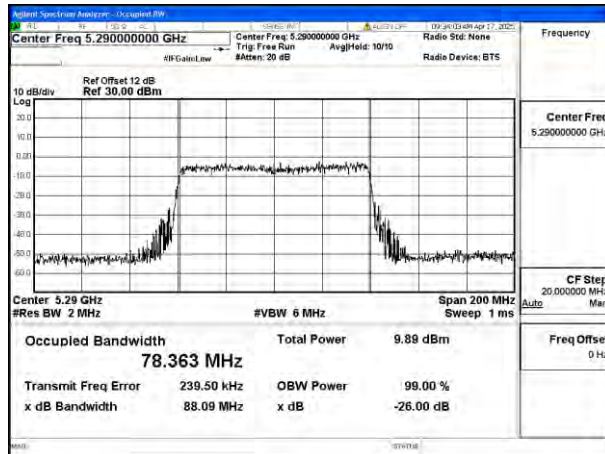
Mode:802.11be EHT80 Frequency:5290MHz Ant:Ant8
