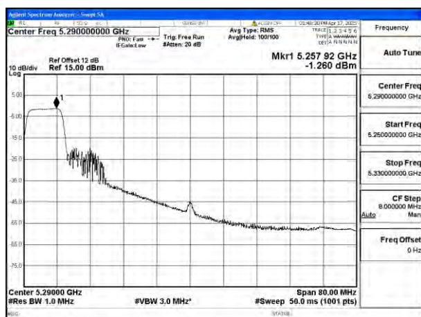
Mode:802.11be EHT80 Tone:106T Frequency:5290MHz Ant:Ant8
