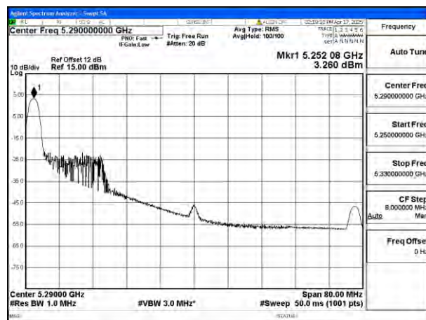
Mode:802.11be EHT80 Tone:26T Frequency:5290MHz Ant:Ant4
