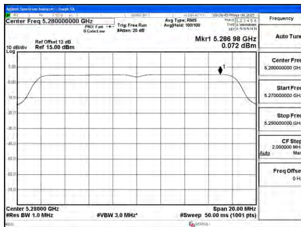
Mode:802.11a Frequency:5280MHz Ant:Ant4
