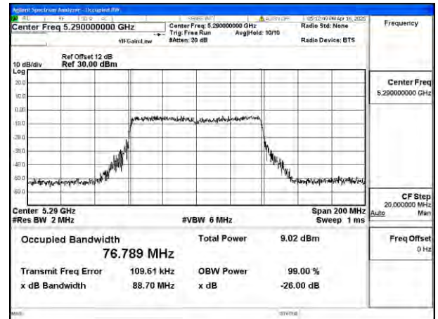
Mode:802.11ac VHT80 Frequency:5290MHz Ant:Ant4
