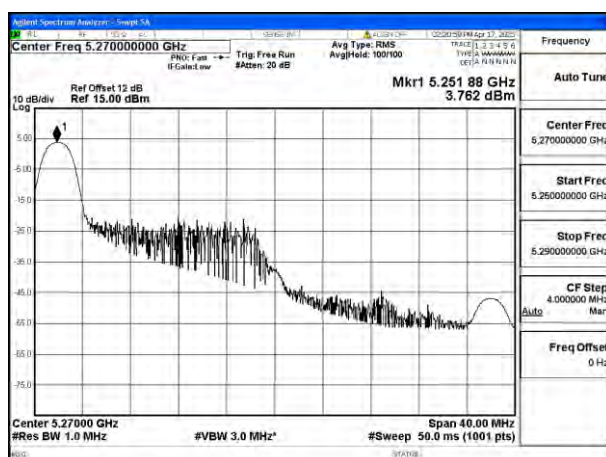
Mode:802.11ax HE40 Tone:26T Frequency:5270MHz Ant:Ant4
