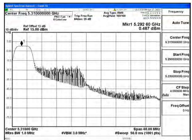
Mode:802.11be EHT40 Tone:52T Frequency:5310MHz Ant:Ant8
