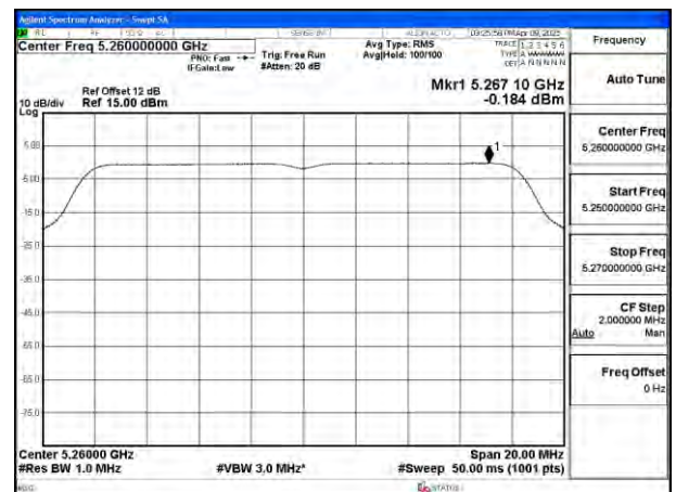
Mode:802.11a Frequency:5260MHz Ant:Ant4
