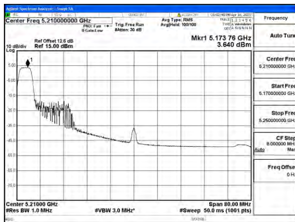
Mode:802.11ax HE80 Tone:52T Frequency:5210MHz Ant:Ant8
