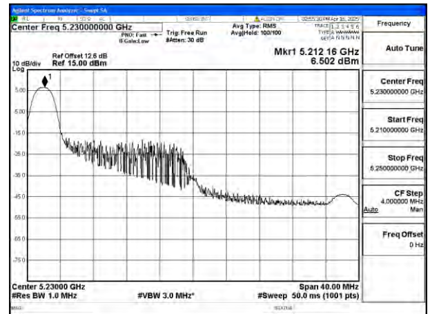
Mode:802.11be EHT40 Tone:26T Frequency:5230MHz Ant:Ant8
