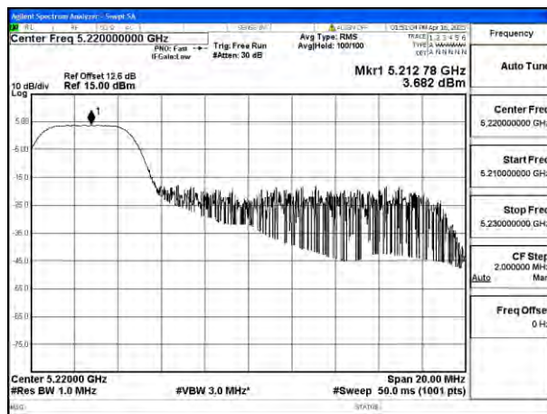
Mode:802.11be EHT20 Tone:52T Frequency:5220MHz Ant:Ant4
