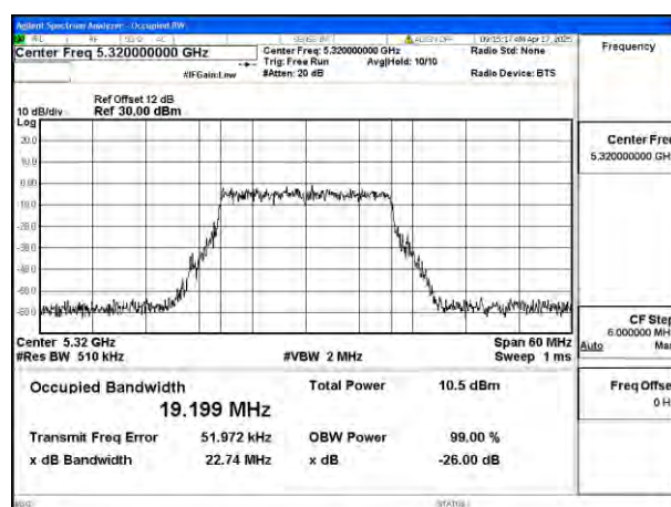
Mode:802.11be EHT20 Frequency:5320MHz Ant:Ant4
