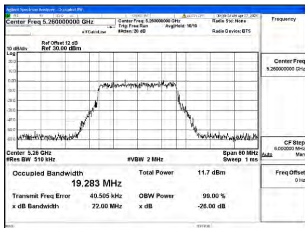
Mode:802.11ax HE20 Frequency:5260MHz Ant:Ant8
