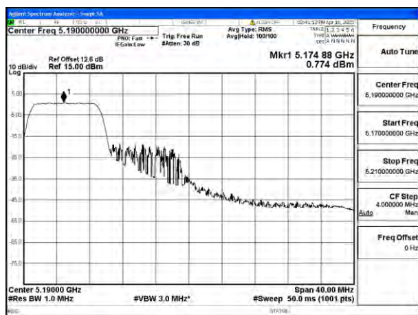
Mode:802.11be EHT40 Tone:106T Frequency:5190MHz Ant:Ant4
