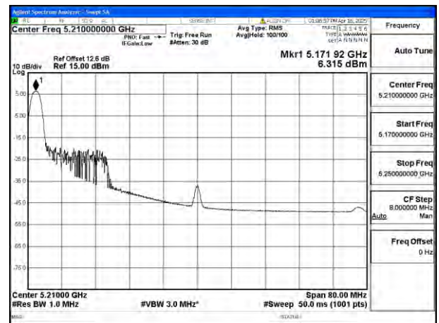
Mode:802.11ax HE80 Tone:26T Frequency:5210MHz Ant:Ant4
