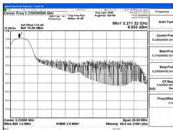
Mode:802.11be EHT20 Tone:26T Frequency:5220MHz Ant:Ant8
