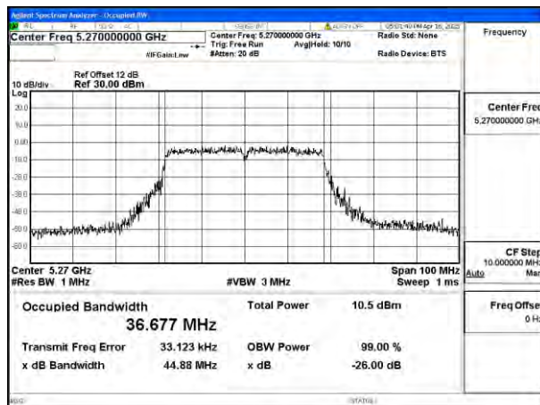
Mode:802.11ac VHT40 Frequency:5270MHz Ant:Ant4
