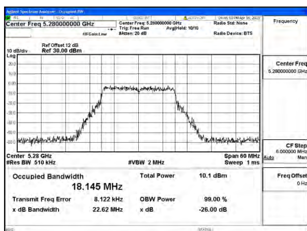
Mode:802.11ac VHT20 Frequency:5280MHz Ant:Ant4
