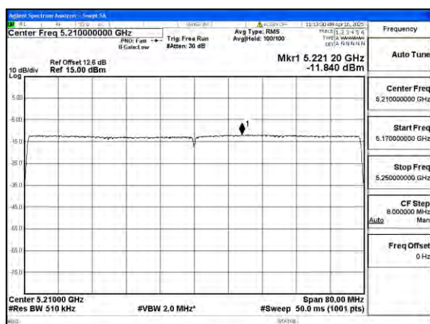
Mode:802.11be EHT80 Tone:996T Frequency:5210MHz Ant:Ant8
