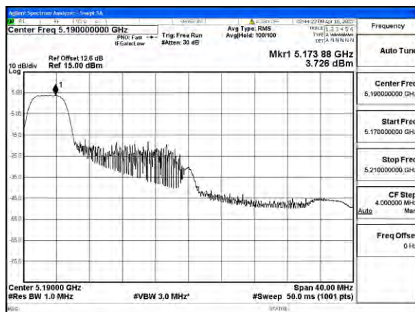
Mode:802.11be EHT40 Tone:52T Frequency:5190MHz Ant:Ant8
