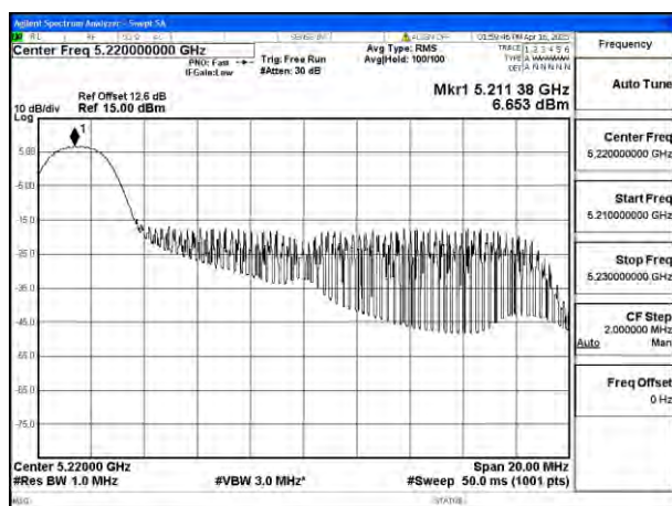
Mode:802.11be EHT20 Tone:26T Frequency:5220MHz Ant:Ant4
