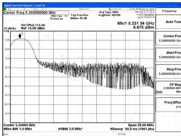
Mode:802.11ax HE20 Tone:26T Frequency:5240MHz Ant:Ant8
