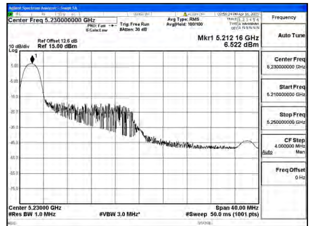
Mode:802.11be EHT40 Tone:26T Frequency:5230MHz Ant:Ant4
