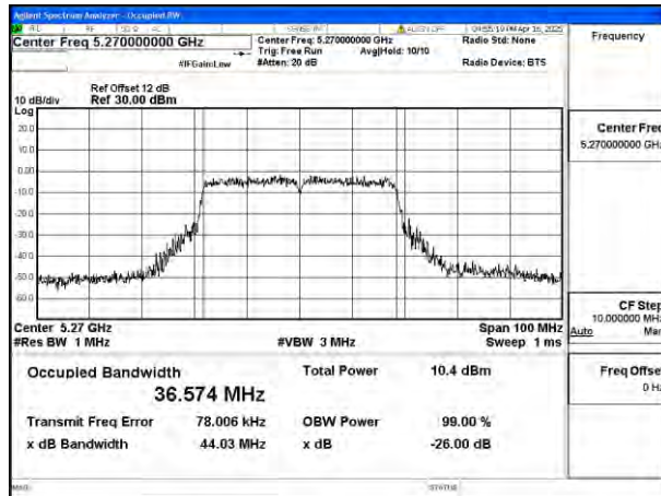
Mode:802.11ac VHT40 Frequency:5270MHz Ant:Ant8
