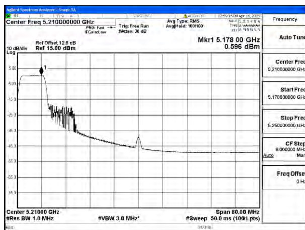
Mode:802.11ax HE80 Tone:106T Frequency:5210MHz Ant:Ant8
