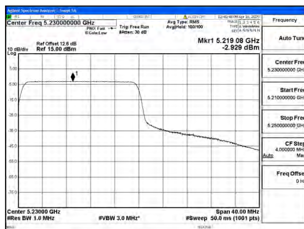
Mode:802.11ax HE40 Tone:242T Frequency:5230MHz Ant:Ant8
