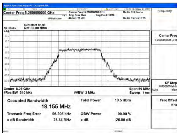
Mode:802.11ac VHT20 Frequency:5260MHz Ant:Ant8
