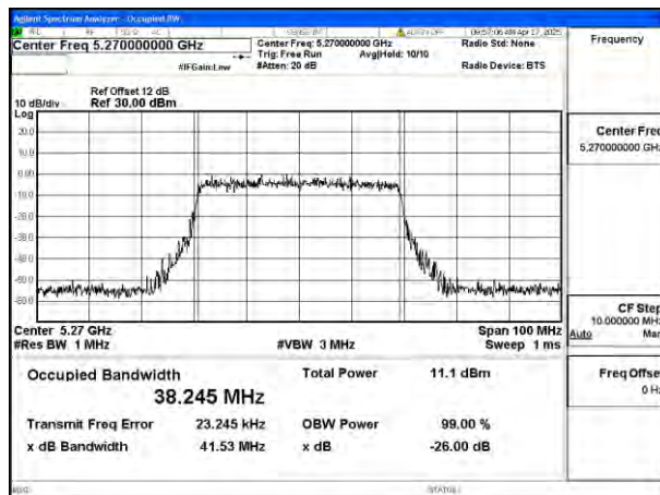
Mode:802.11ax HE40 Frequency:5270MHz Ant:Ant4
