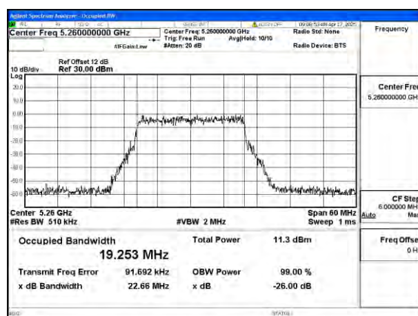
Mode:802.11be EHT20 Frequency:5260MHz Ant:Ant4
