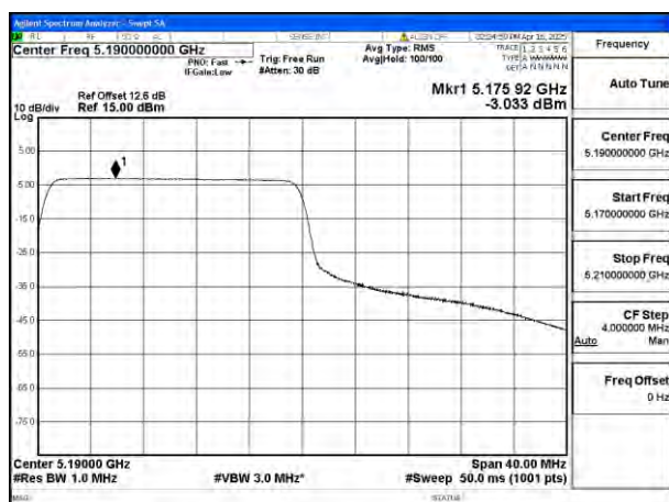
Mode:802.11be EHT40 Tone:242T Frequency:5190MHz Ant:Ant8
