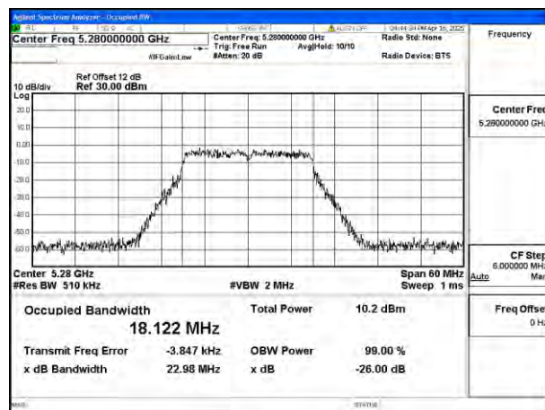
Mode:802.11ac VHT20 Frequency:5280MHz Ant:Ant8
