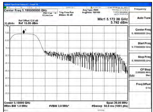
Mode:802.11be EHT20 Tone:52T Frequency:5180MHz Ant:Ant4
