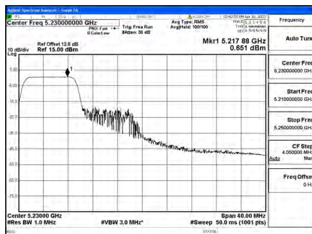
Mode:802.11be EHT40 Tone:106T Frequency:5230MHz Ant:Ant8
