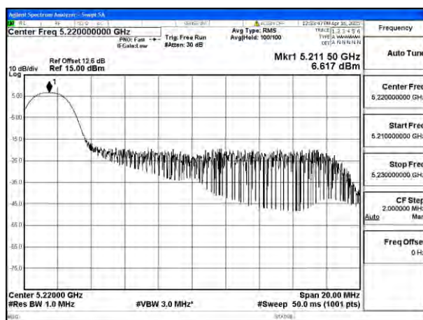
Mode:802.11ax HE20 Tone:26T Frequency:5220MHz Ant:Ant4
