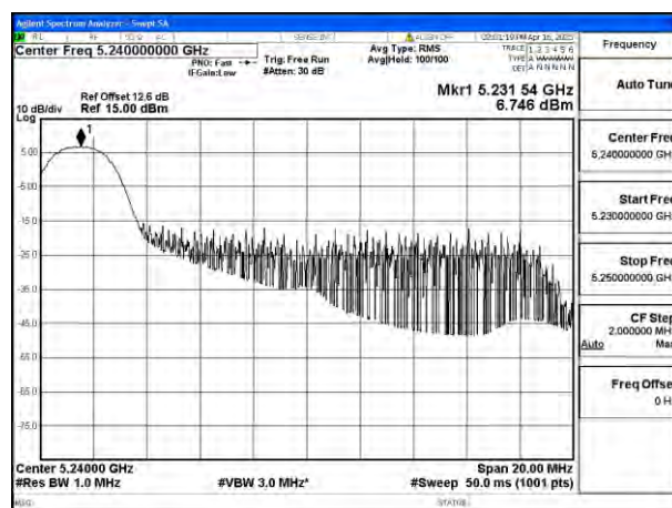
Mode:802.11be EHT20 Tone:26T Frequency:5240MHz Ant:Ant4
