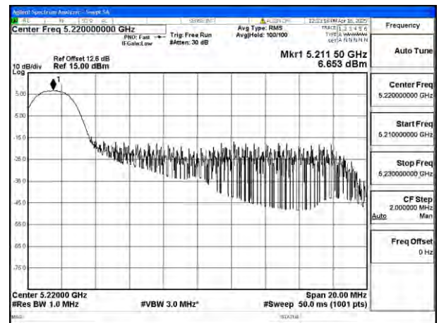
Mode:802.11ax HE20 Tone:26T Frequency:5220MHz Ant:Ant8
