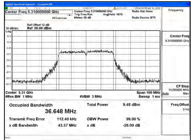
Mode:802.11ac VHT40 Frequency:5310MHz Ant:Ant8
