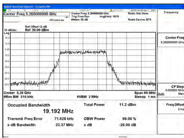
Mode:802.11be EHT20 Frequency:5260MHz Ant:Ant8
