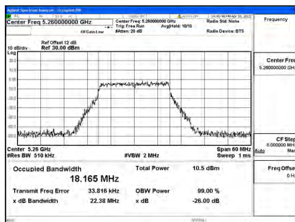
Mode:802.11ac VHT20 Frequency:5260MHz Ant:Ant4
