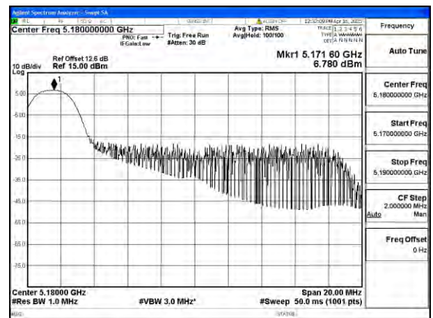
Mode:802.11ax HE20 Tone:26T Frequency:5180MHz Ant:Ant4
