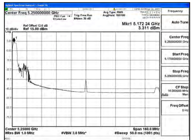
Mode:802.11be EHT160 Tone:52T Frequency:5250MHz Ant:Ant4
