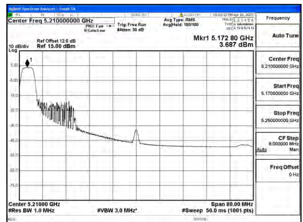
Mode:802.11ax HE80 Tone:52T Frequency:5210MHz Ant:Ant4
