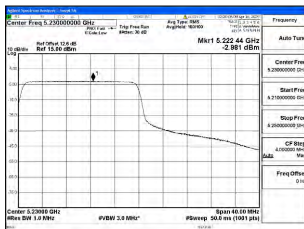
Mode:802.11be EHT40 Tone:242T Frequency:5230MHz Ant:Ant8
