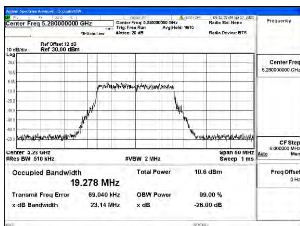
Mode:802.11be EHT20 Frequency:5280MHz Ant:Ant4
