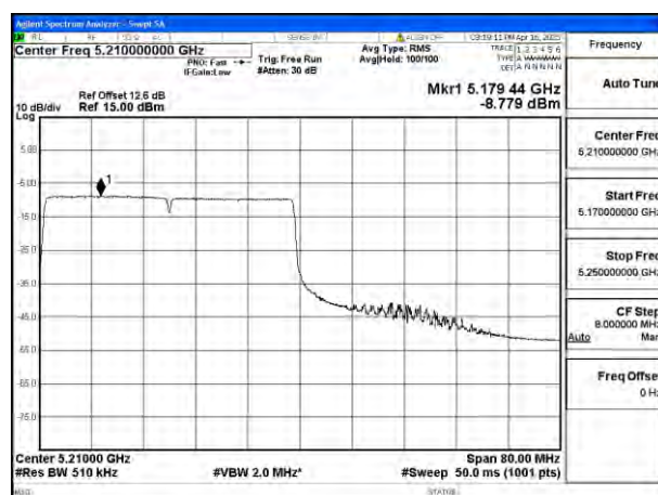
Mode:802.11be EHT80 Tone:484T Frequency:5210MHz Ant:Ant4
