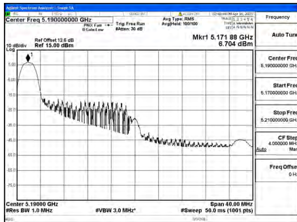
Mode:802.11be EHT40 Tone:26T Frequency:5190MHz Ant:Ant4
