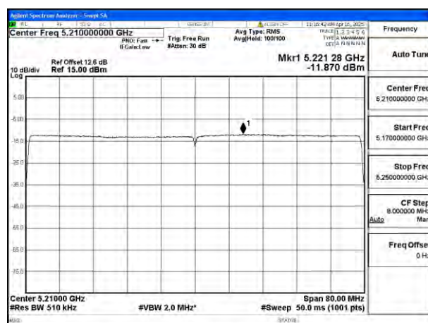
Mode:802.11be EHT80 Tone:996T Frequency:5210MHz Ant:Ant4
