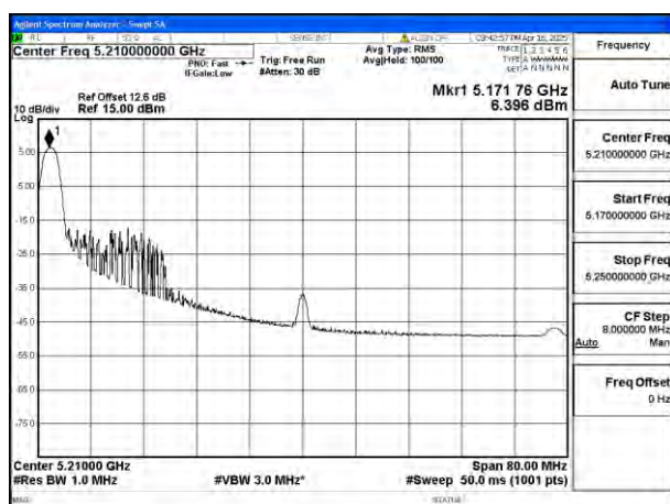
Mode:802.11be EHT80 Tone:26T Frequency:5210MHz Ant:Ant8
