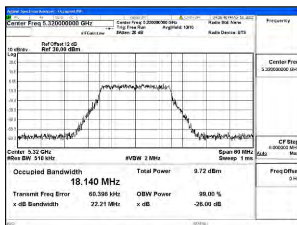
Mode:802.11n HT20 Frequency:5320MHz Ant:Ant4
