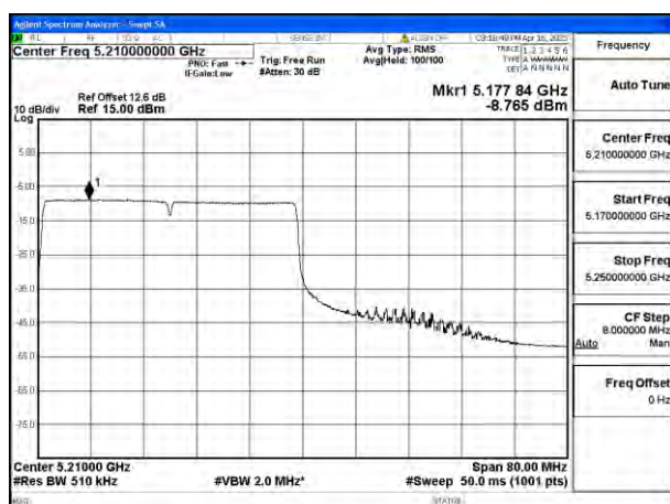
Mode:802.11be EHT80 Tone:484T Frequency:5210MHz Ant:Ant8
