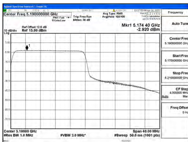
Mode:802.11ax HE40 Tone:242T Frequency:5190MHz Ant:Ant8
