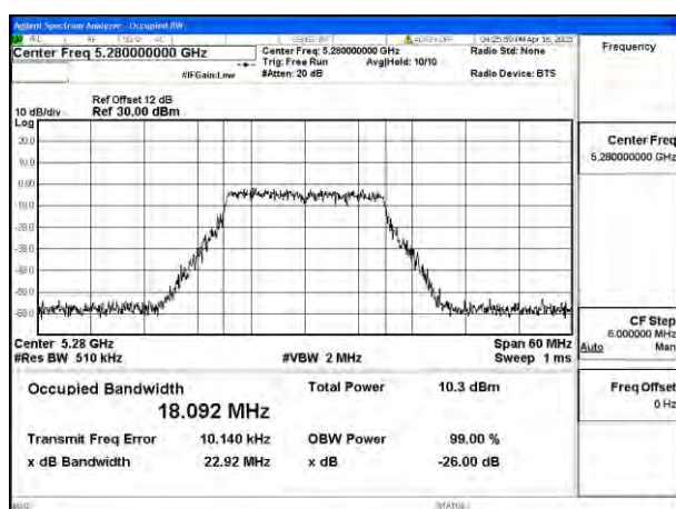
Mode:802.11n HT20 Frequency:5280MHz Ant:Ant4
