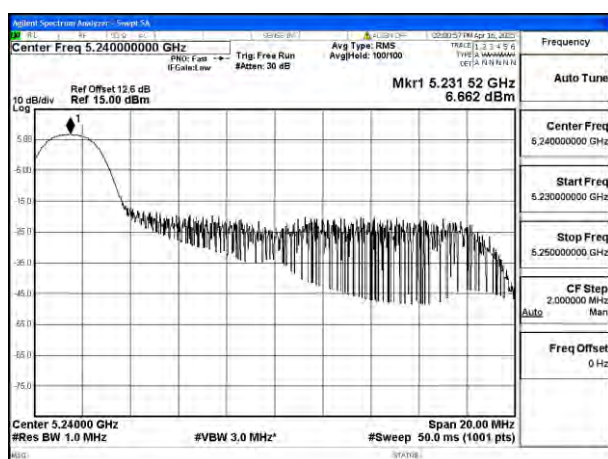
Mode:802.11be EHT20 Tone:26T Frequency:5240MHz Ant:Ant8
