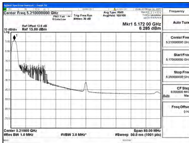
Mode:802.11ax HE80 Tone:26T Frequency:5210MHz Ant:Ant8
