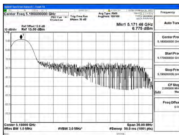
Mode:802.11be EHT20 Tone:26T Frequency:5180MHz Ant:Ant4
