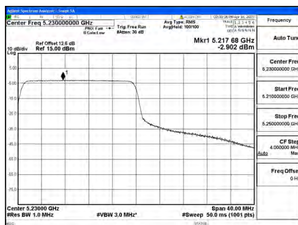
Mode:802.11be EHT40 Tone:242T Frequency:5230MHz Ant:Ant4
