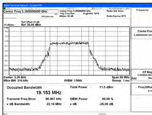
Mode:802.11ax HE20 Frequency:5260MHz Ant:Ant4
