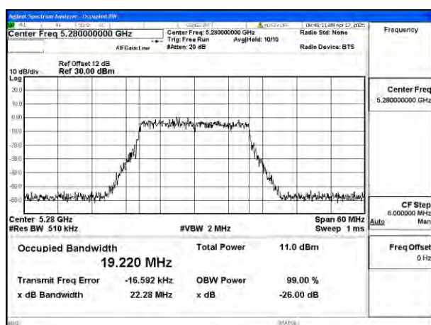
Mode:802.11ax HE20 Frequency:5280MHz Ant:Ant4
