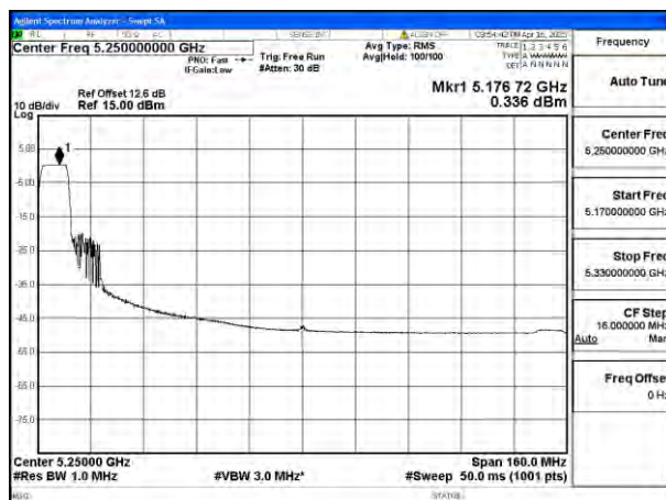
Mode:802.11be EHT160 Tone:106T
