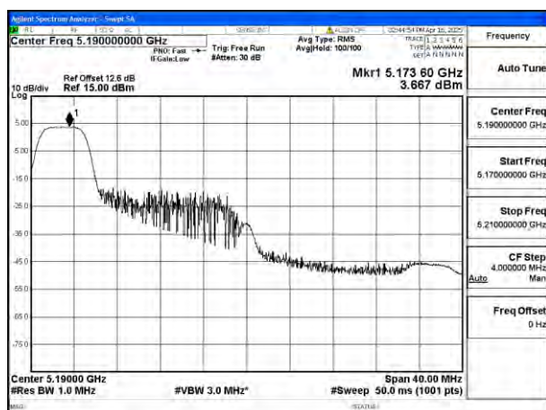
Mode:802.11be EHT40 Tone:52T Frequency:5190MHz Ant:Ant4
