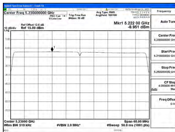
Mode:802.11ax HE40 Tone:484T Frequency:5230MHz Ant:Ant8
