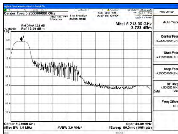
Mode:802.11be EHT40 Tone:52T Frequency:5230MHz Ant:Ant4
