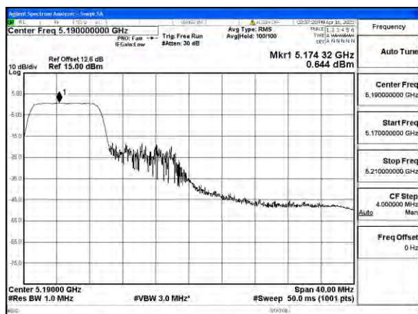
Mode:802.11be EHT40 Tone:106T Frequency:5190MHz Ant:Ant8
