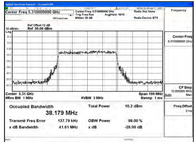
Mode:802.11ax HE40 Frequency:5310MHz Ant:Ant8
