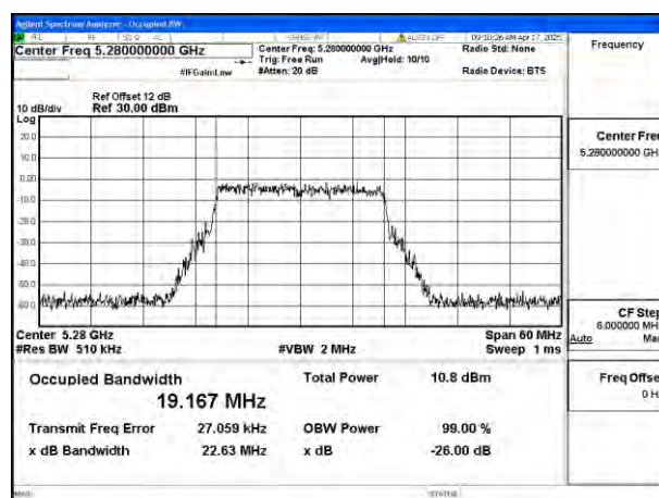
Mode:802.11be EHT20 Frequency:5280MHz Ant:Ant8
