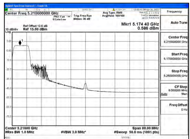
Mode:802.11ax HE80 Tone:106T Frequency:5210MHz Ant:Ant4
