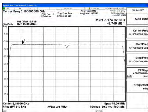
Mode:802.11be EHT40 Tone:484T Frequency:5190MHz Ant:Ant8
