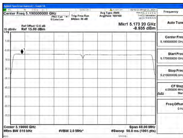
Mode:802.11ax HE40 Tone:484T Frequency:5190MHz Ant:Ant8
