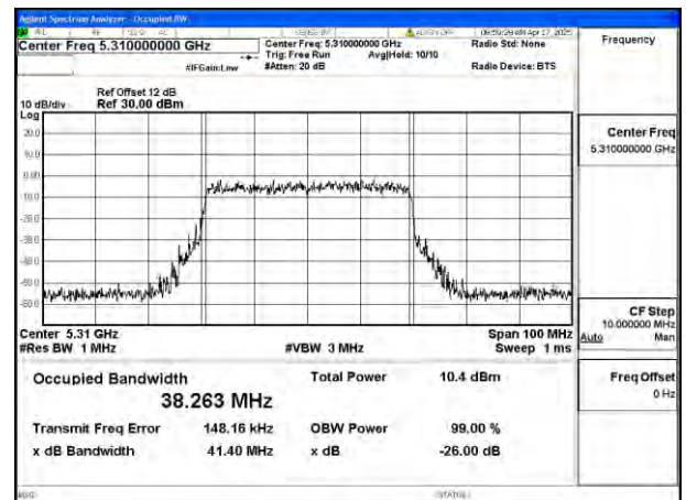
Mode:802.11ax HE40 Frequency:5310MHz Ant:Ant4
