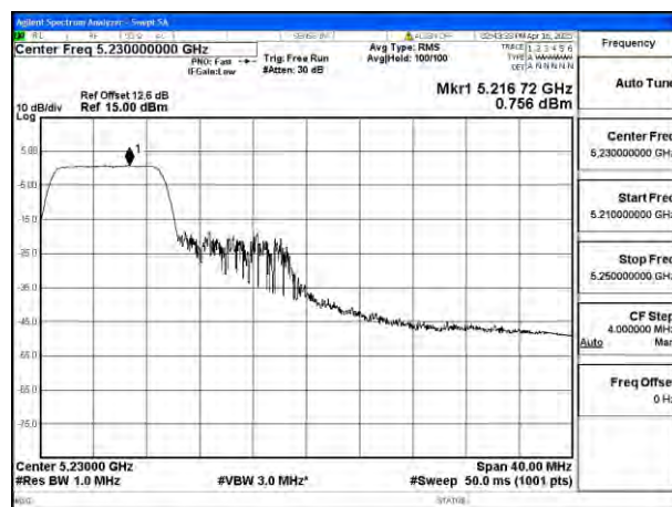
Mode:802.11be EHT40 Tone:106T Frequency:5230MHz Ant:Ant4
