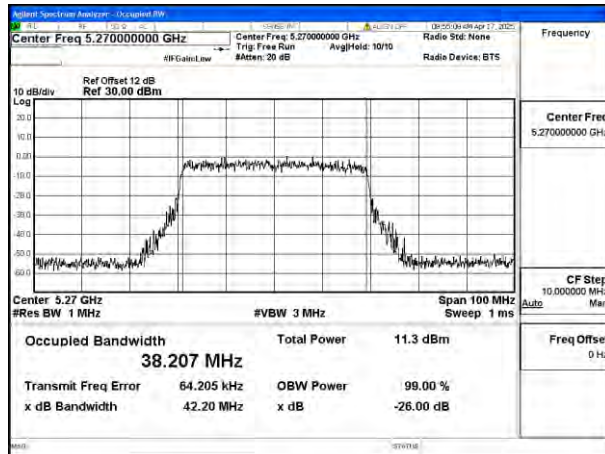
Mode:802.11ax HE40 Frequency:5270MHz Ant:Ant8
