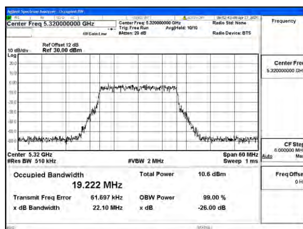
Mode:802.11ax HE20 Frequency:5320MHz Ant:Ant4
