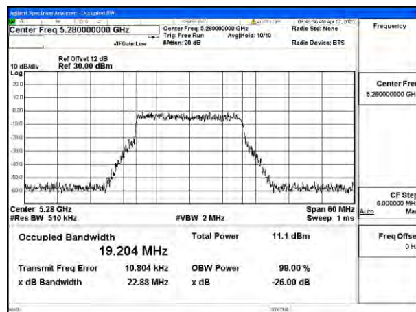
Mode:802.11ax HE20 Frequency:5280MHz Ant:Ant8
