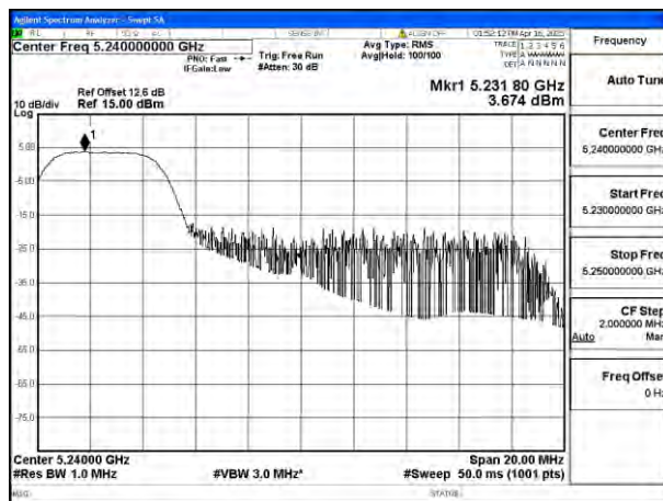
Mode:802.11be EHT20 Tone:52T Frequency:5240MHz Ant:Ant8
