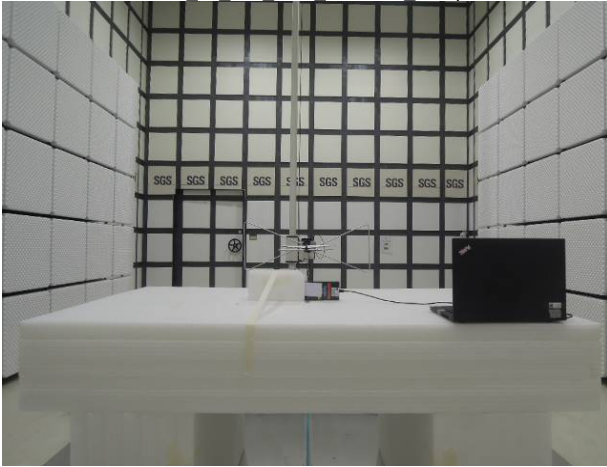
FCC 15 225 NFC Radiated Setup
