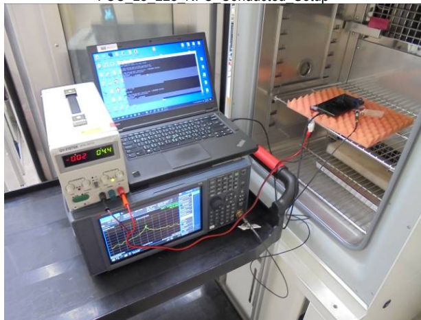
FCC 15 247 BLE Conducted setup
