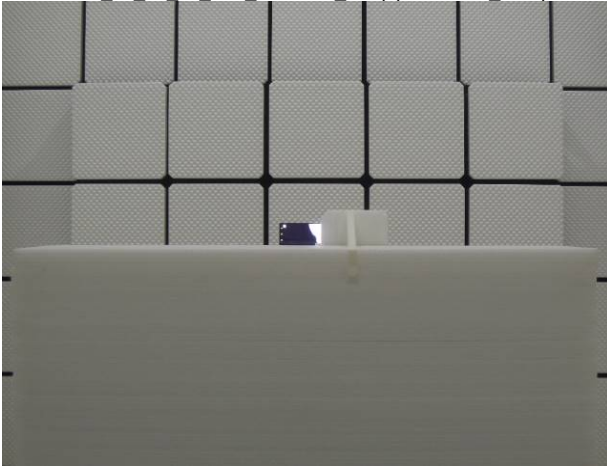
FCC 22 24 27 LTE Radiated 966(1)-H Plane Setup
