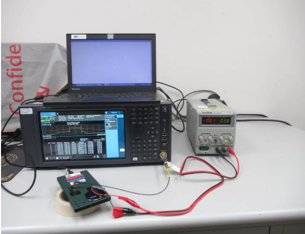
FCC 22 24 27 FR1 Conducted setup2
