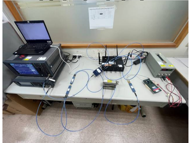
FCC 15 407 WLAN Normal DFS Slave SETUP
