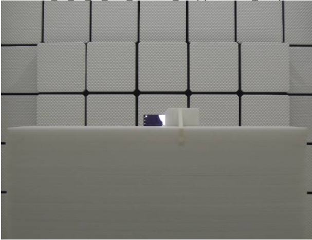
FCC 22 24 27 FR1 Radiated 966(1)-H Plane Setup
