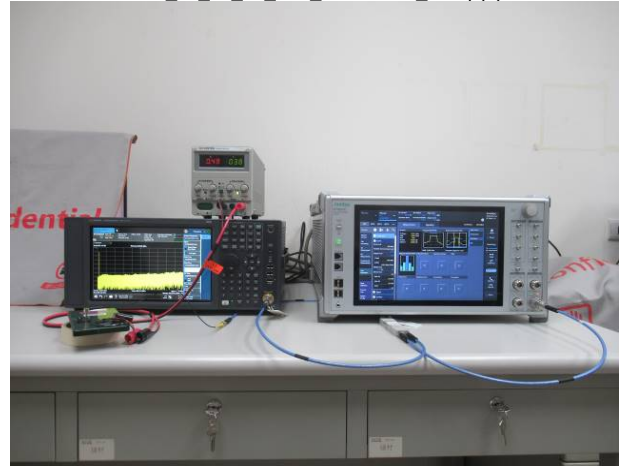
FCC 22 24 27 LTE Conducted Setup(2)
