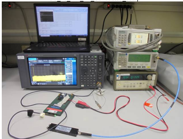
FCC 15 247 BT Conducted setup
