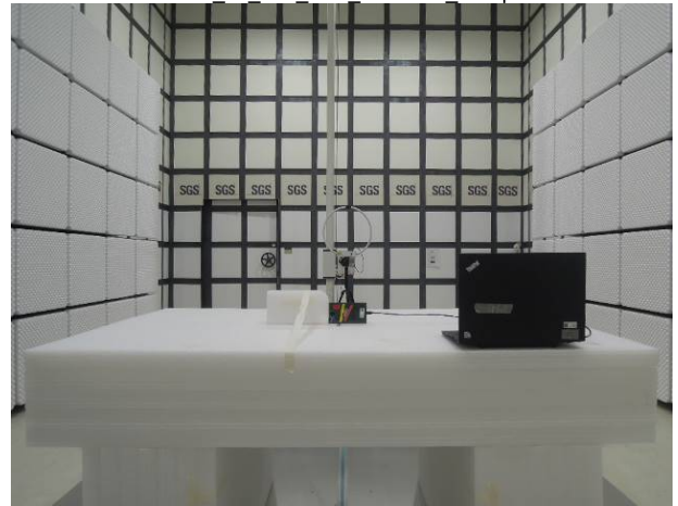
FCC 15 247 BLE Radiated Setup
