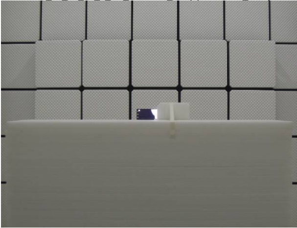
FCC 22 24 27 2 3G Radiated 966(1)-H Plane Setup
