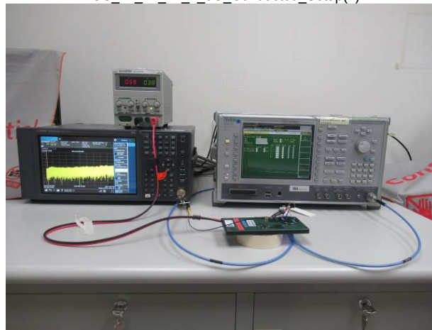
FCC 22 24 27 2 3G Conducted_Setup(1)
