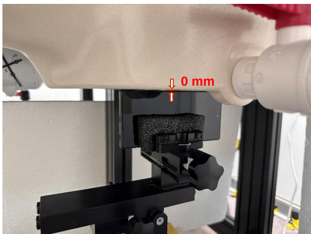
Photograph 23. Limb, Left Edge, 0mm
