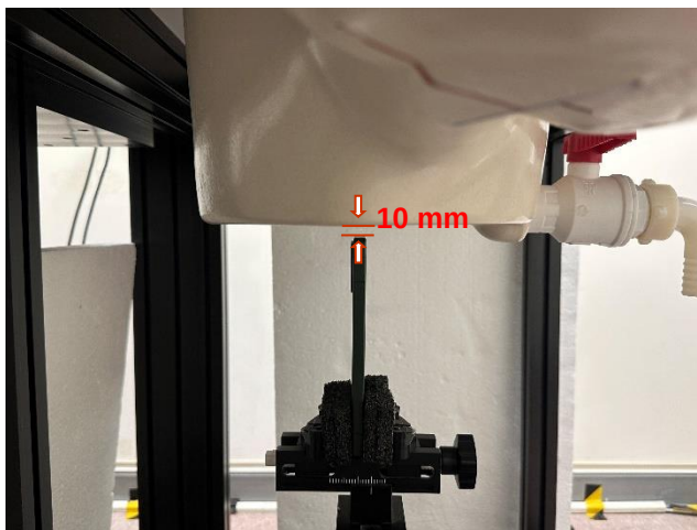
Photograph 30. Hotspot, Top Edge, 10mm
