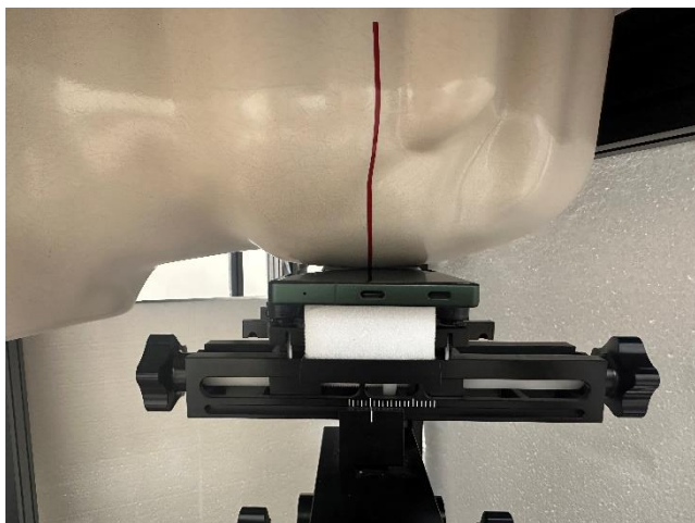
Photograph 5. Head, Left Touch, 0mm
