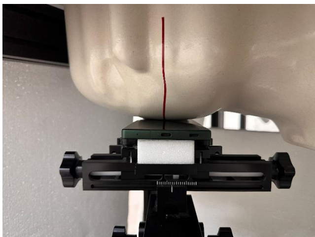
Photograph 1. Head, Right Touch, 0mm
