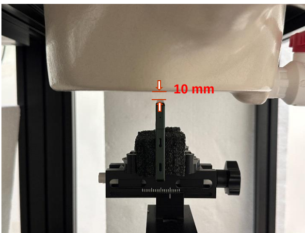
Photograph 36. Hotspot, Left Edge, 10mm
