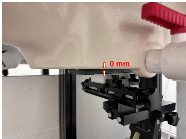
Photograph 15. Limb, Back Surface, 0mm
