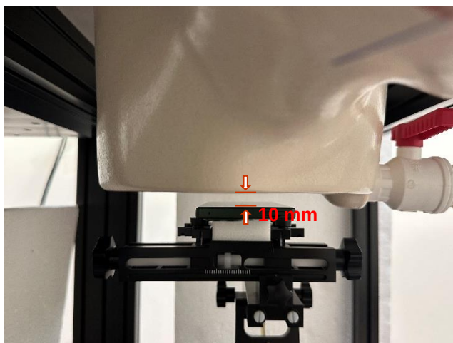
Photograph 10. Body, Front Surface, 10mm
