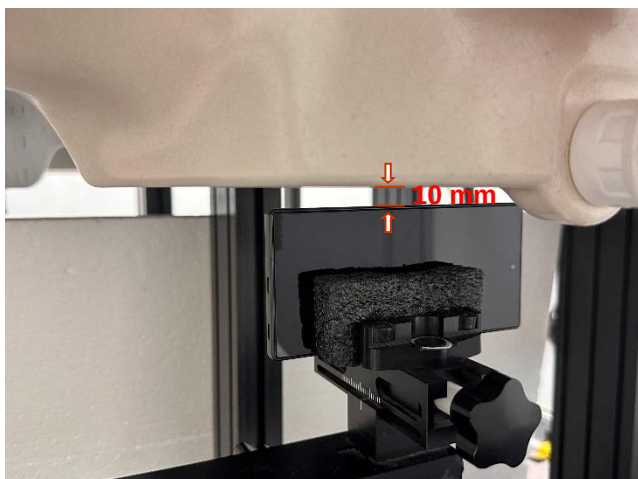
Photograph 35. Hotspot, Left Edge, 10mm
