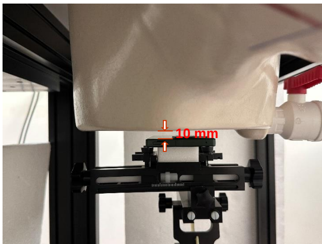
Photograph 28. Hotspot, Back Surface, 10mm
