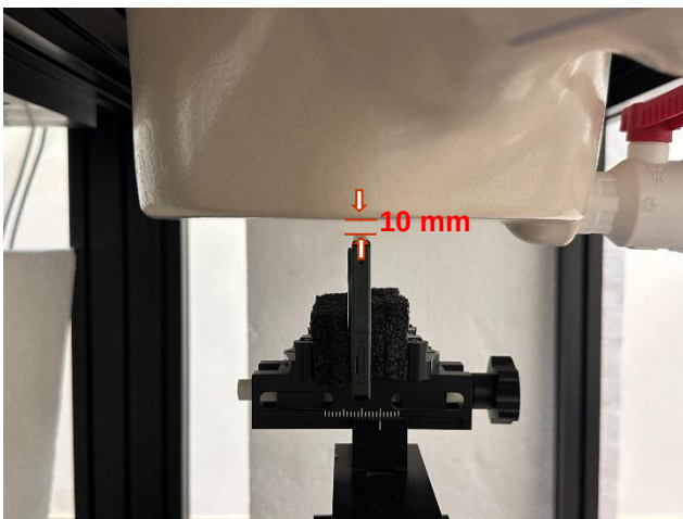
Photograph 34. Hotspot, Right Edge, 10mm
