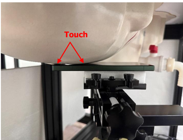
Photograph 2. Head, Right Touch, 0mm
