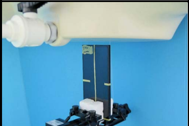
Bottom Side of EUT Tested at 10 mm
