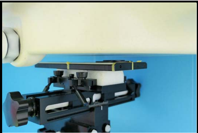
Rear Face of EUT Tested at 10 mm
