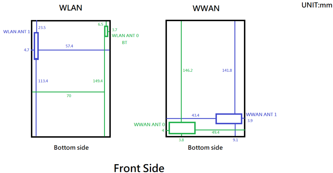
Fig.23 Antenna position of EUT
