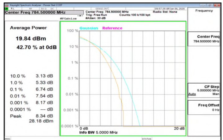
LTE_Band13_5MHz_64QAM_25_0_HighCH23255-784.5
