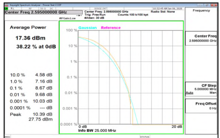
LTE_Band38_20MHz_64QAM_100_0_MidCH38000-2595
