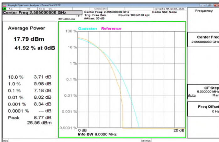
LTE_Band38_15MHz_64QAM_75_0_MidCH38000-2595
