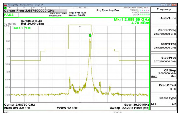
Band41_5MHz_QPSK_1_24_CH41565
