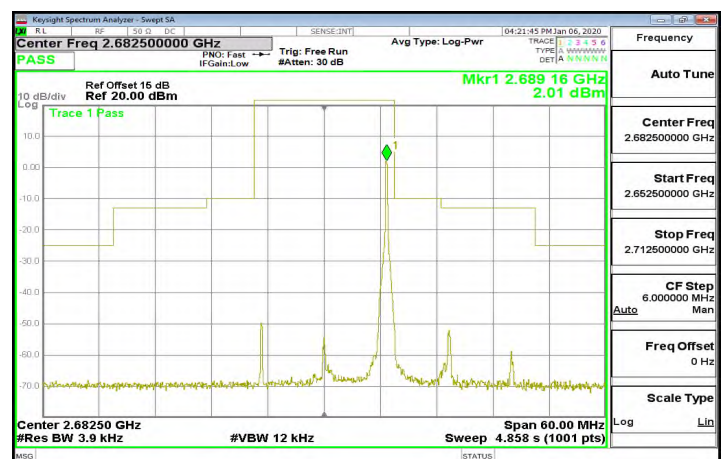
Band41_15MHz_64QAM_1_74_CH41515
