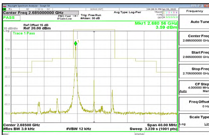
Band41_10MHz_16QAM_1_0_CH41540
