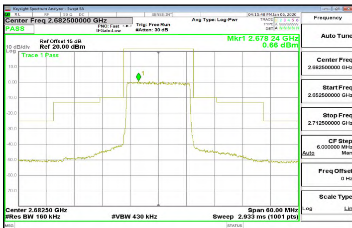
Band41_15MHz_QPSK_75_0_CH41515
