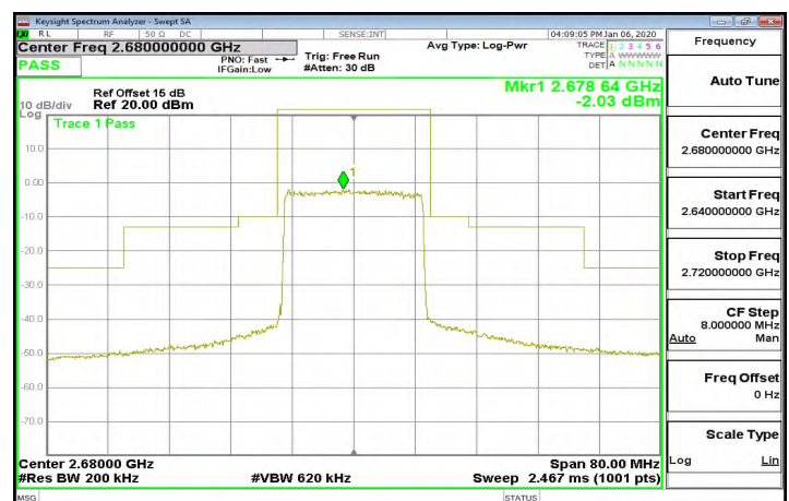
Band41_20MHz_64QAM_100_0_CH41490
