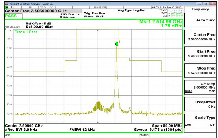
Band41_20MHz_16QAM_1_99_CH40620
