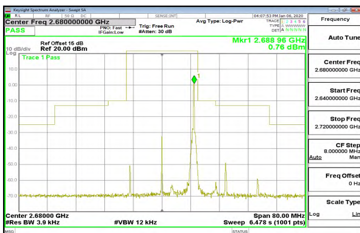
Band41_20MHz_64QAM_1_99_CH41490
