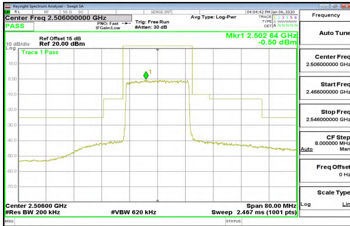
Band41_20MHz_16QAM_100_0_CH40620
