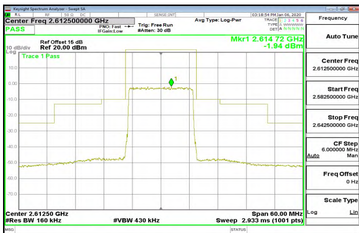
Band38_15MHz_64QAM_75_0_CH38175
