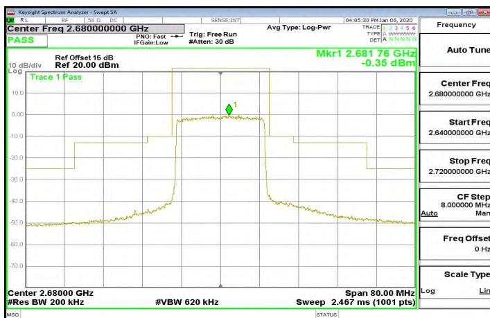
Band41_20MHz_16QAM_100_0_CH41490
