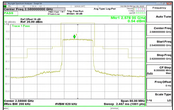
Band38_20MHz_QPSK_100_0_CH38000
