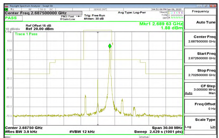
Band41_5MHz_64QAM_1_24_CH41565
