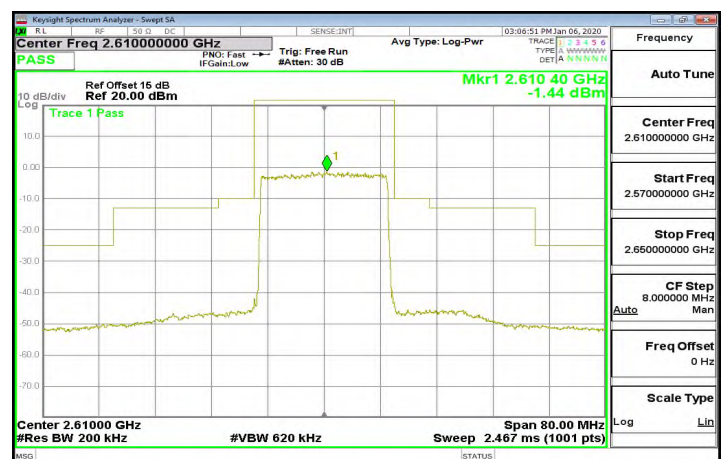
Band38_20MHz_64QAM_100_0_CH38150
