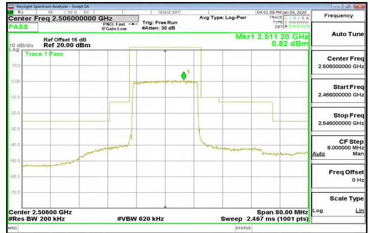
Band41_20MHz_QPSK_100_0_CH40620
