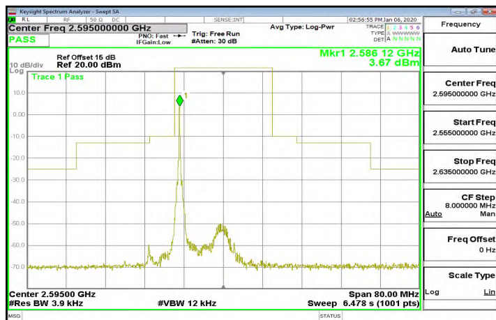
Band38_20MHz_QPSK_1_0_CH38150
