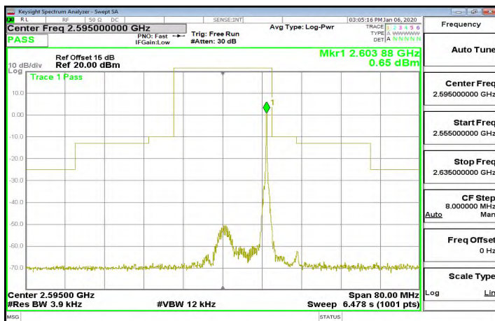
Band38_20MHz_64QAM_1_99_CH38150
