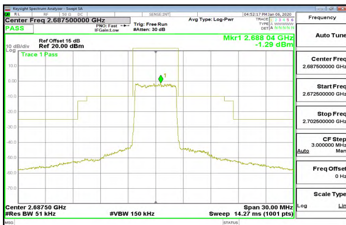
Band41_5MHz_64QAM_25_0_CH41565
