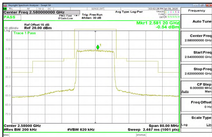
Band38_20MHz_16QAM_100_0_CH38000
