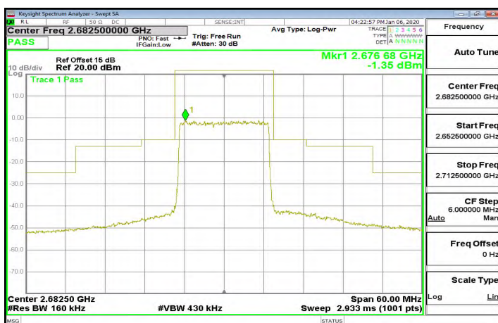
Band41_15MHz_64QAM_75_0_CH41515
