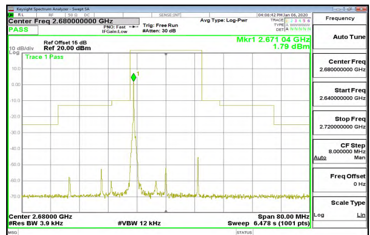
Band41_20MHz_64QAM_1_0_CH41490
