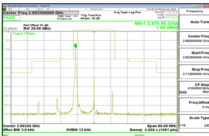
Band41_15MHz_64QAM_1_0_CH41515
