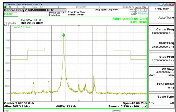
Band41_10MHz_QPSK_1_0_CH41540
