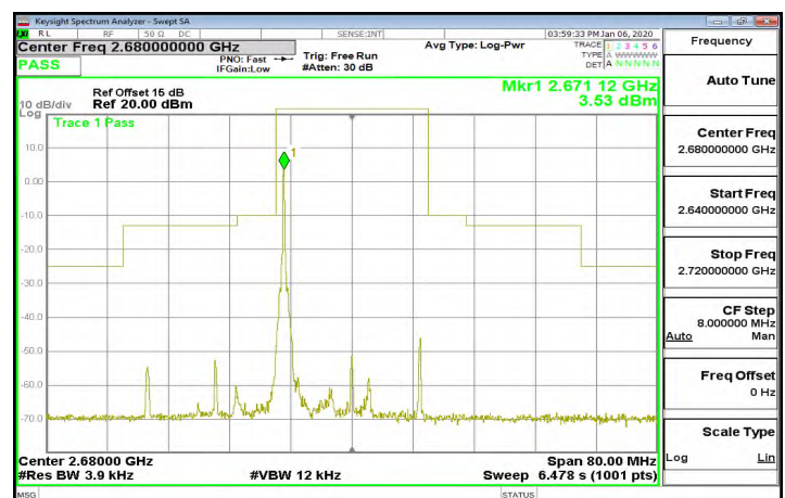
Band41_20MHz_QPSK_1_0_CH41490
