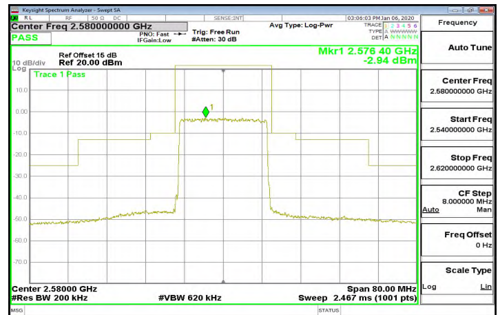
Band38_20MHz_64QAM_100_0_CH38000
