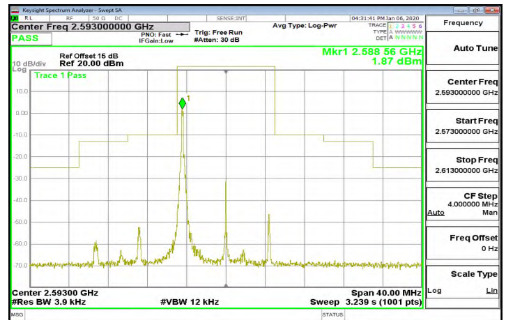
Band41_10MHz_64QAM_1_0_CH41540
