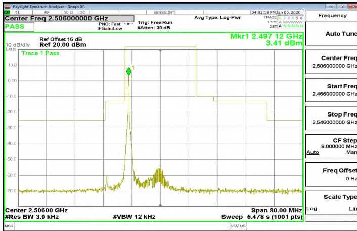
Band41_20MHz_16QAM_1_0_CH40620
