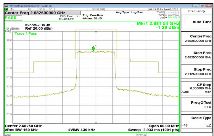
Band41_15MHz_16QAM_75_0_CH41515
