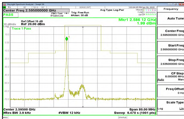
Band38_20MHz_64QAM_1_0_CH38150
