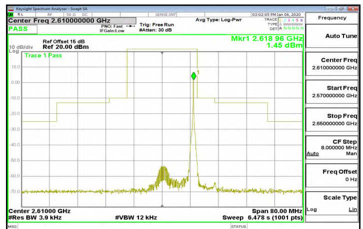
Band38_20MHz_16QAM_1_99_CH38150
