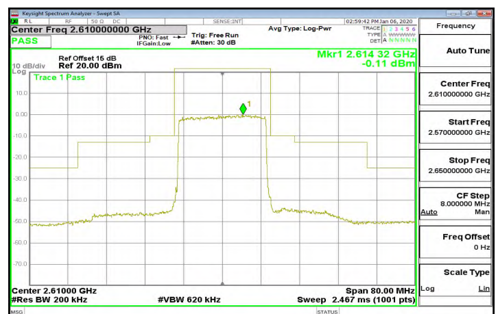
Band38_20MHz_QPSK_100_0_CH38150
