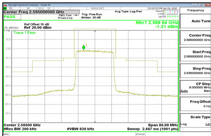
Band38_20MHz_16QAM_100_0_CH38150
