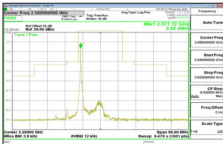
Band38_20MHz_QPSK_1_0_CH38000
