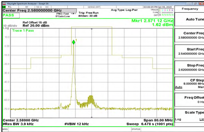
Band38_20MHz_16QAM_1_0_CH38000
