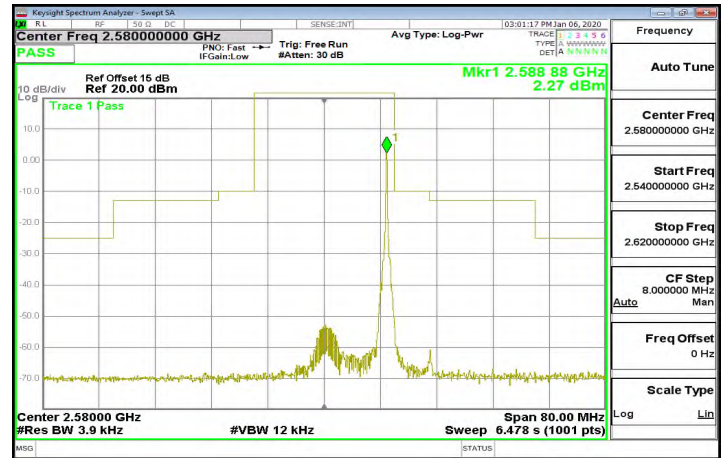
Band38_20MHz_16QAM_1_99_CH38000
