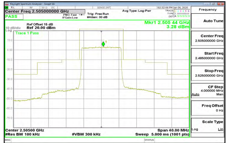
Band7_10MHz_QPSK_50_0_CH21100
