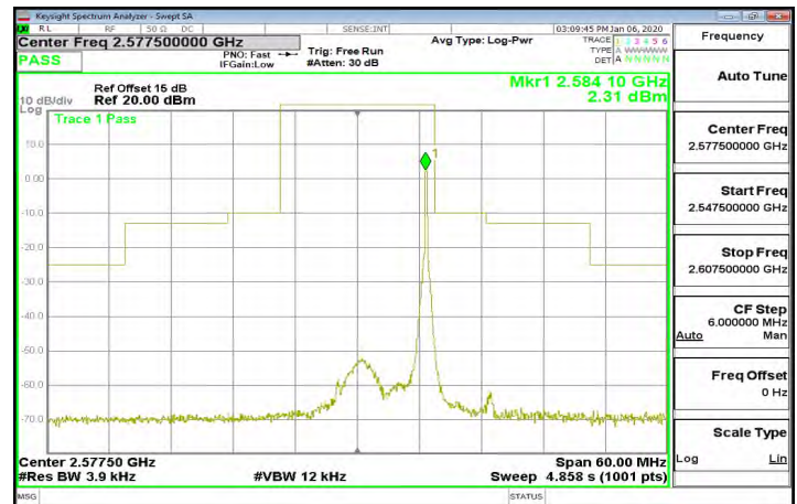
Band38_15MHz_QPSK_1_74_CH38000
