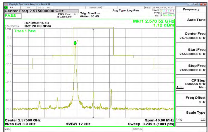
Band38_10MHz_64QAM_1_0_CH38000
