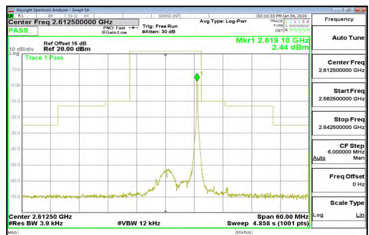
Band38_15MHz_QPSK_1_74_CH38175
