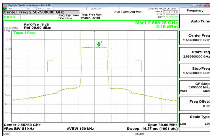
Band7_5MHz_16QAM_25_0_CH21425
