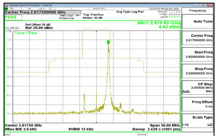
Band38_5MHz_64QAM_1_24_CH38225
