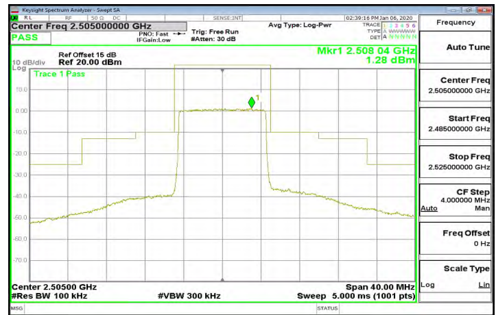
Band7_10MHz_64QAM_50_0_CH21100
