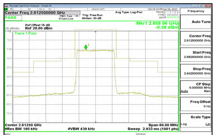
Band38_15MHz_16QAM_75_0_CH38175
