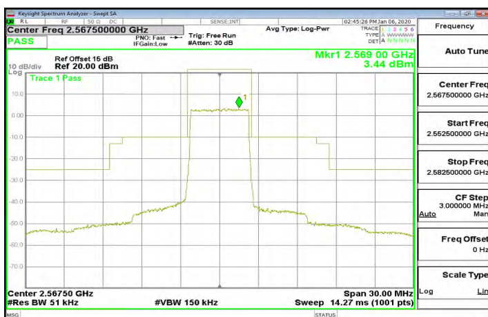
Band7_5MHz_QPSK_25_0_CH21425
