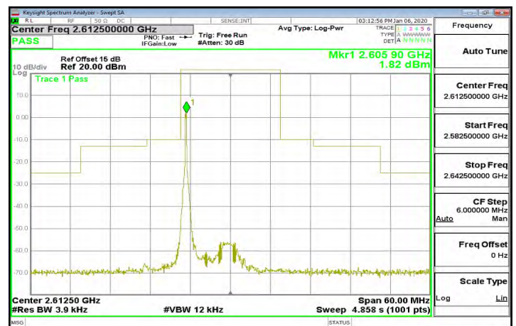
Band38_15MHz_16QAM_1_0_CH38175
