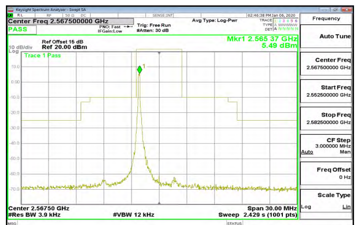
Band7_5MHz_16QAM_1_0_CH21425
