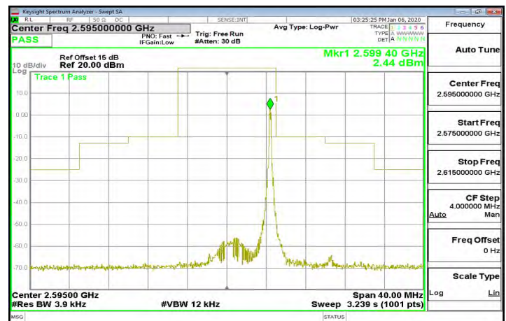
Band38_10MHz_16QAM_1_49_CH38200
