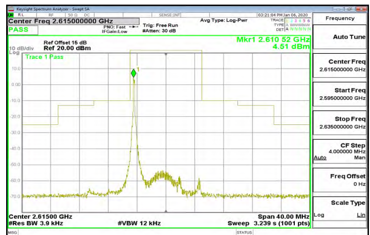
Band38_10MHz_QPSK_1_0_CH38200
