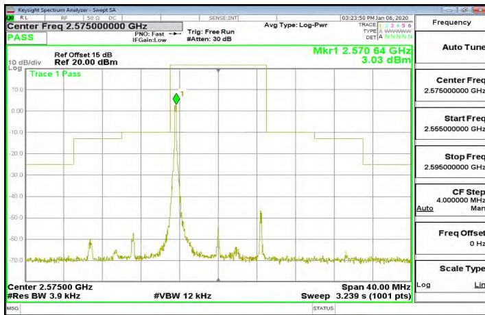
Band38_10MHz_16QAM_1_0_CH38000
