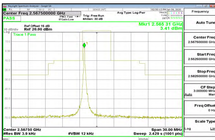
Band7_5MHz_64QAM_1_0_CH21425
