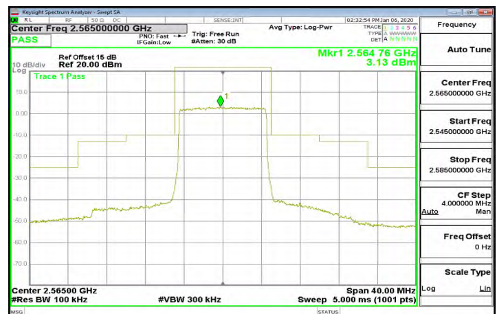
Band7_10MHz_QPSK_50_0_CH21400
