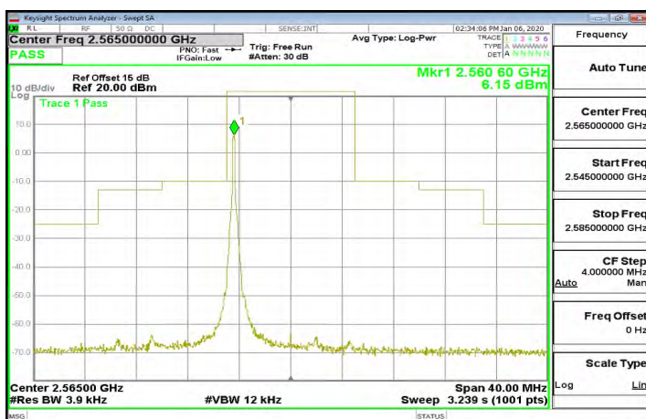
Band7_10MHz_16QAM_1_0_CH21400
