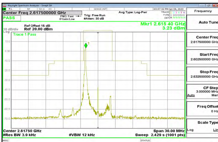
Band38_5MHz_QPSK_1_0_CH38225
