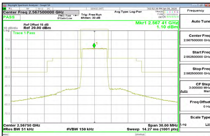
Band7_5MHz_64QAM_25_0_CH21425
