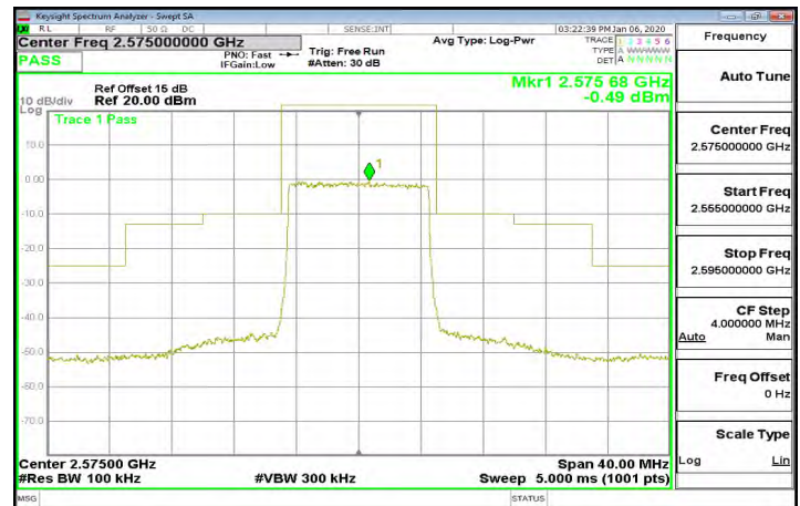
Band38_10MHz_QPSK_50_0_CH38000
