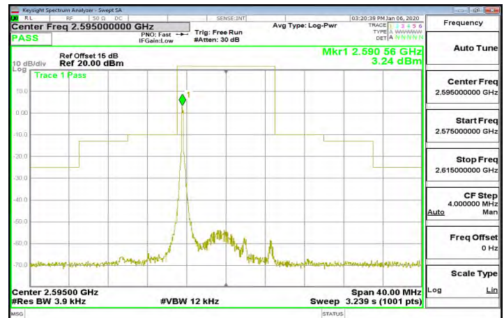
Band38_10MHz_QPSK_1_0_CH38200
