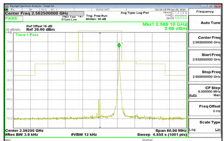
Band7_15MHz_64QAM_1_74_CH21375
