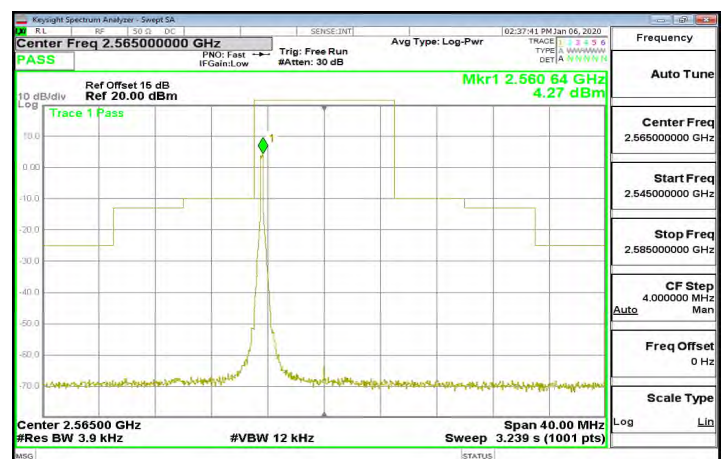
Band7_10MHz_64QAM_1_0_CH21400
