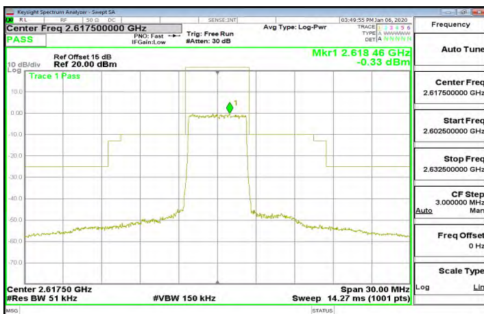
Band38_5MHz_QPSK_25_0_CH38225
