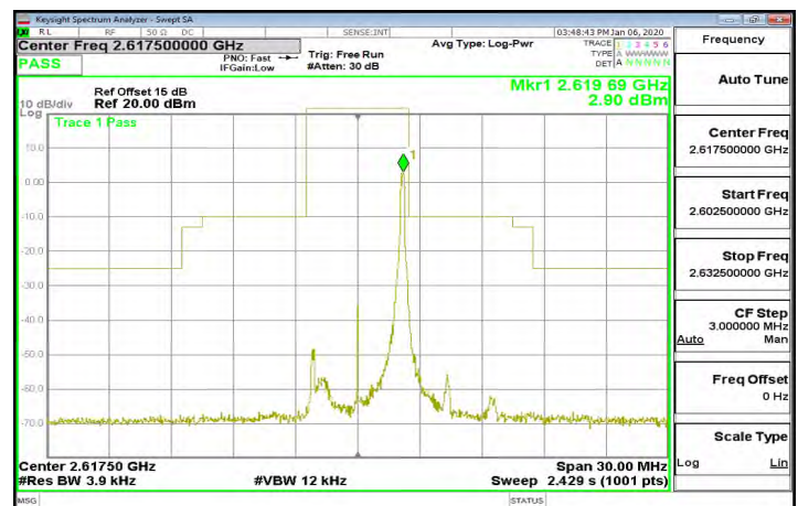
Band38_5MHz_QPSK_1_24_CH38225
