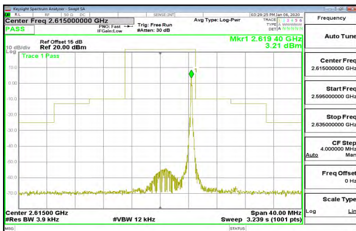
Band38_10MHz_64QAM_1_49_CH38200
