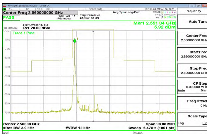
Band7_20MHz_16QAM_1_0_CH21350
