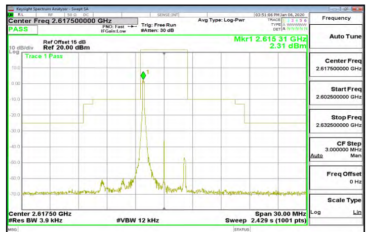
Band38_5MHz_16QAM_1_0_CH38225
