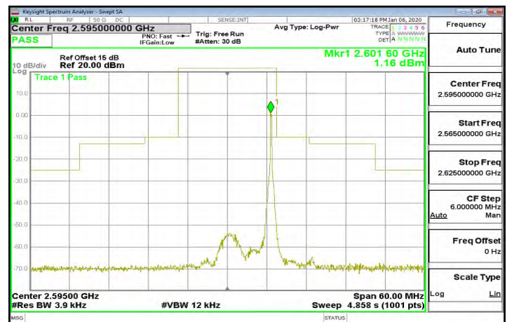
Band38_15MHz_64QAM_1_74_CH38175
