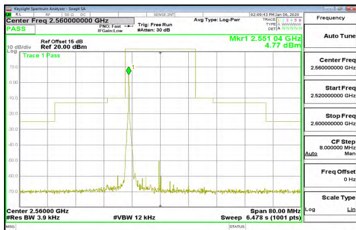
Band7_20MHz_64QAM_1_0_CH21350
