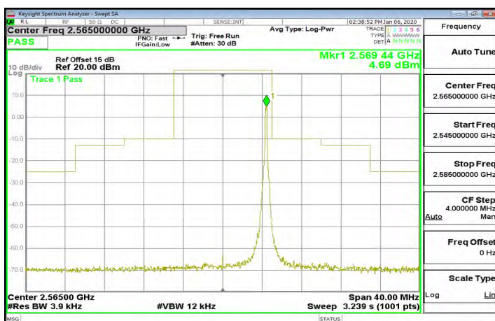
Band7_10MHz_64QAM_1_49_CH21400
