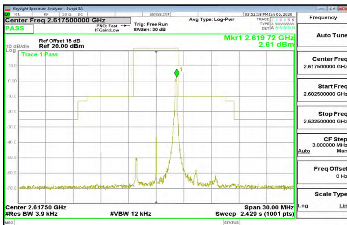
Band38_5MHz_16QAM_1_24_CH38225
