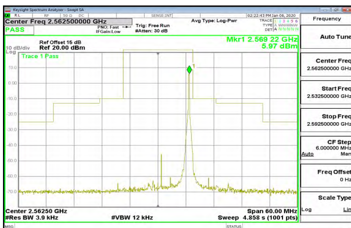
Band7_15MHz_16QAM_1_74_CH21375
