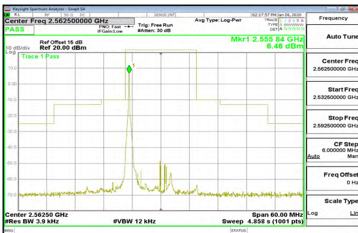
Band7_15MHz_QPSK_1_0_CH21375
