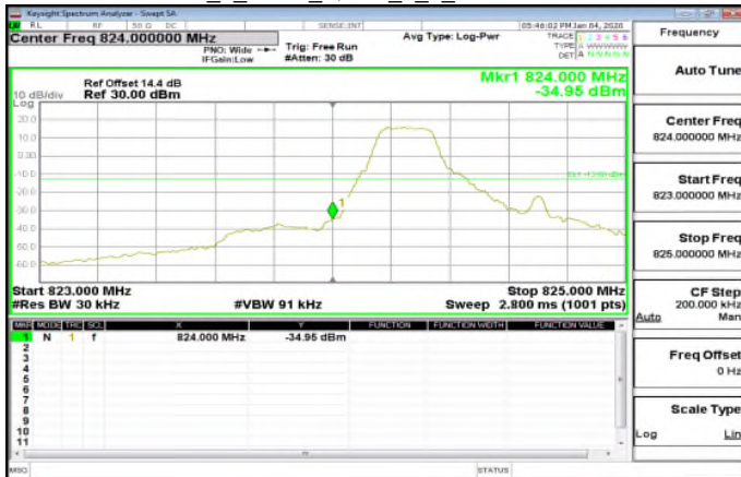
LTE\Band5_1_4MHz_QPSK_1_0_LowCH20407-824.7
