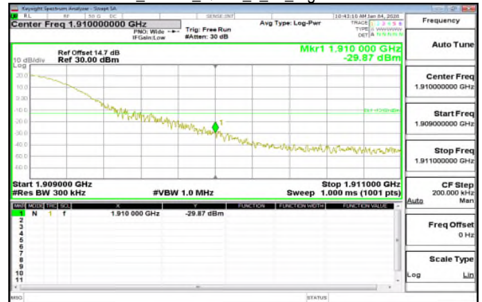
LTE\Band2_20MHz_QPSK_1_99_HighCH19100-1900
