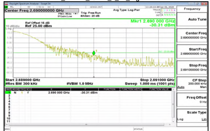
LTE\Band41_20MHz_QPSK_1_99_HighCH41490-2680
