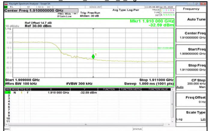
LTE\Band2_10MHz_QPSK_50_0_HighCH19150-1905
