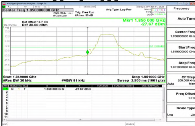
LTE\Band2_1_4MHz_QPSK_1_0_LowCH18607-1850.7
