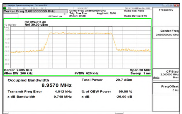
Band41_10MHz_16QAM_50_0_Main_HighCH41540-2685
