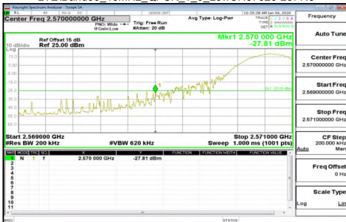
LTE\Band38_15MHz_QPSK_1_0_LowCH37825-2577.5
