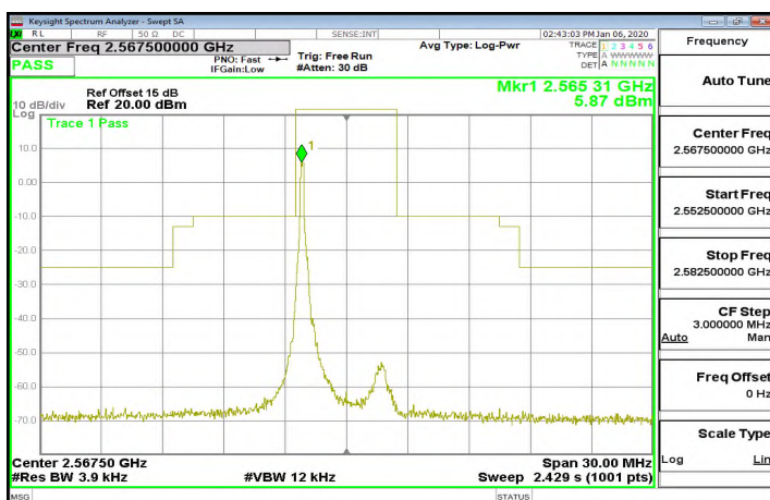
Band7_5MHz_QPSK_1_0_CH21425
