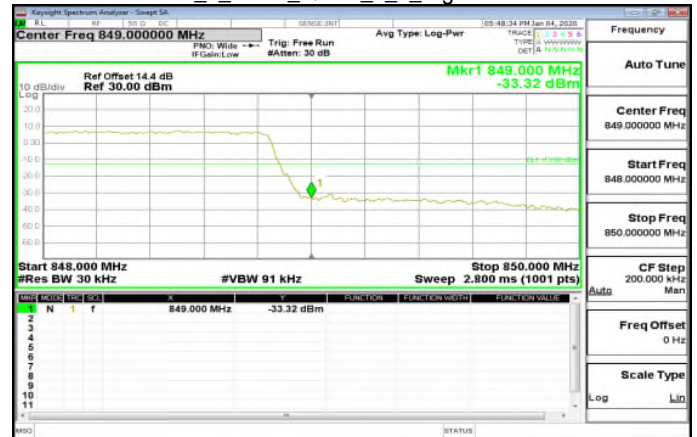
LTE\Band5_1_4MHz_QPSK_6_0_HighCH20643-848.3
