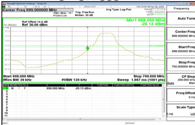
LTE\Band12_3MHz_QPSK_1_0_LowCH23025-700.5
