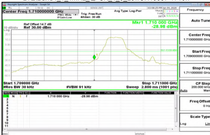
LTE\Band4_1_4MHz_QPSK_1_0_LowCH19957-1710.7
