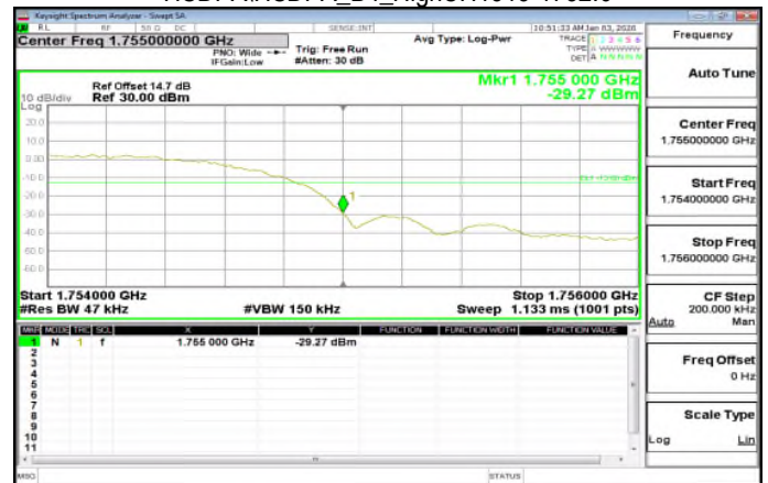
HSDPA\HSDPA_B4_HighCH1513-1752.6
