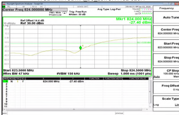
WCDMA\WCDMA_B5_LowCH4132-826.4
