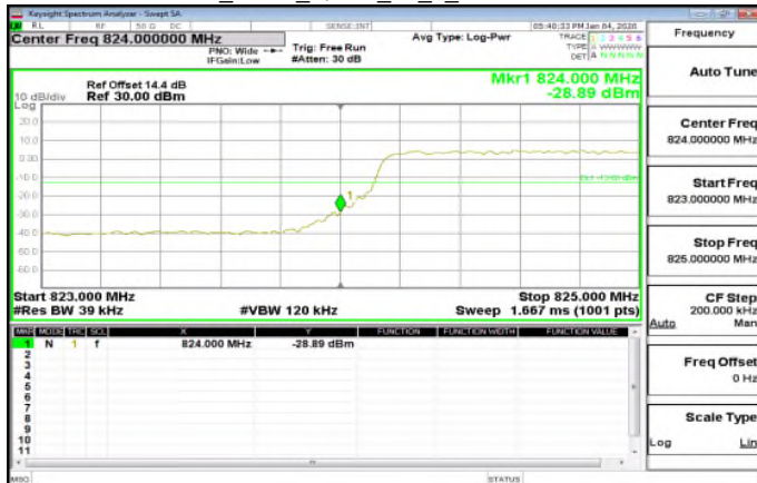
LTE\Band5_3MHz_QPSK_15_0_LowCH20415-825.5
