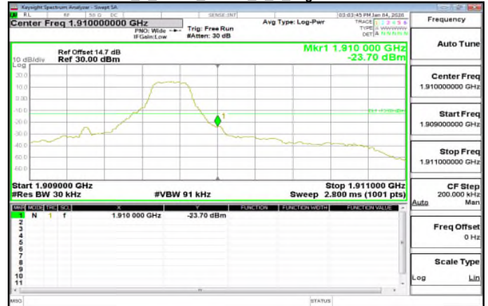
LTE\Band2_1_4MHz_QPSK_6_0_LowCH18607-1850.7
