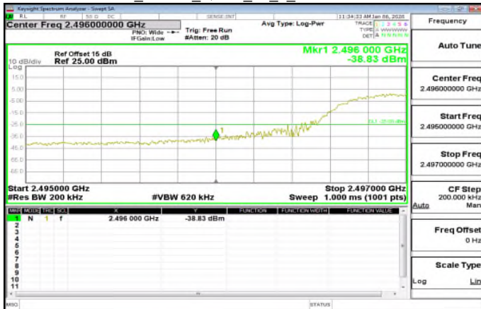
LTE\Band41_15MHz_QPSK_75_0_LowCH39725-2503.5
