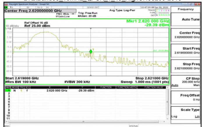
LTE\Band38_10MHz_QPSK_1_49_HighCH38200-2615
