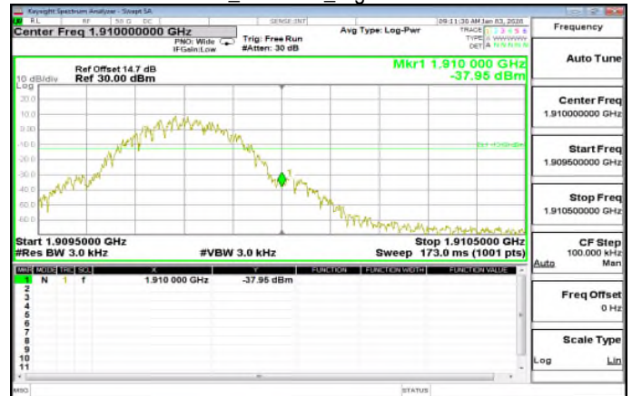
GSM\GSM_1900MHz_HighCH810-1909.8
