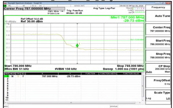
LTE\Band13_5MHz_QPSK_25_0_HighCH23255-784.5
