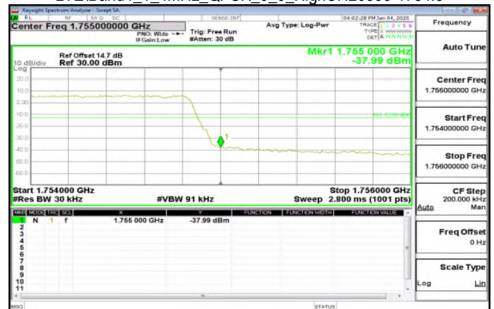
LTE\Band4_1_4MHz_QPSK_6_0_HighCH20393-1754.3
