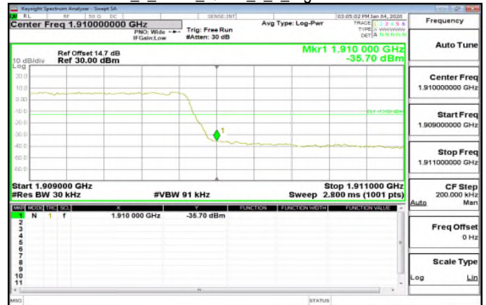
LTE\Band2_1_4MHz_QPSK_6_0_HighCH19193-1909.3
