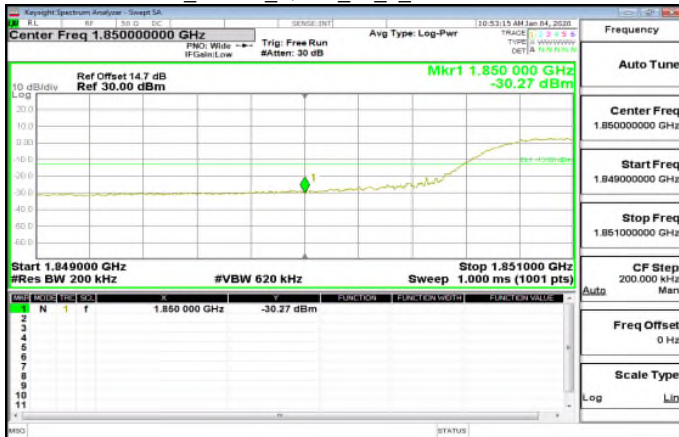
LTE\Band2_15MHz_QPSK_75_0_LowCH18675-1857.5
