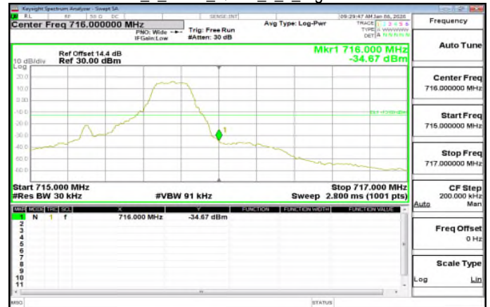
LTE/Band12_1_4MHz_QPSK_1_5_HighCH23173-715.3
