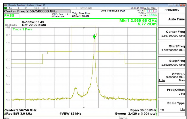
Band7_5MHz_QPSK_1_24_CH21425
