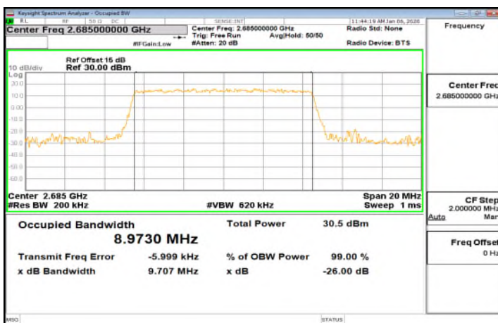
Band41_10MHz_QPSK_50_0_Main_HighCH41540-2685
