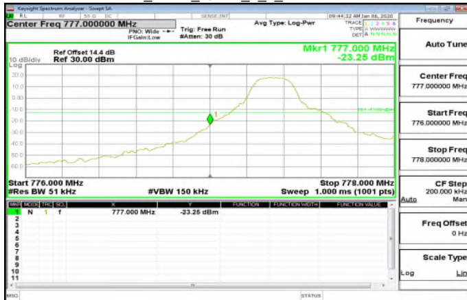
LTE\Band13_5MHz_QPSK_1_0_LowCH23205-779.5
