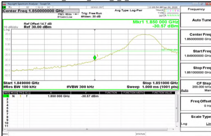
LTE\Band2_10MHz_QPSK_1_0_LowCH18650-1855
