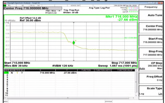
LTE\Band12_3MHz_QPSK_15_0_HighCH23165-714.5
