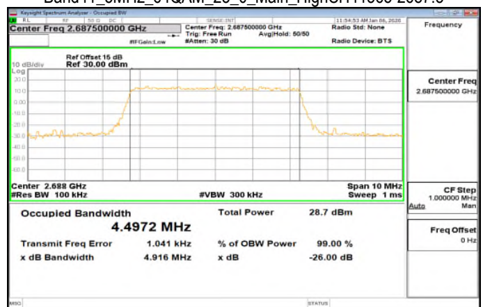
Band41_5MHz_64QAM_25_0_Main_HighCH41565-2687.5
