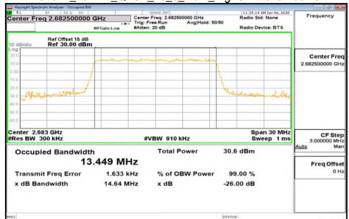
Band41_15MHz_QPSK_75_0_Main_HighCH41515-2682.5
