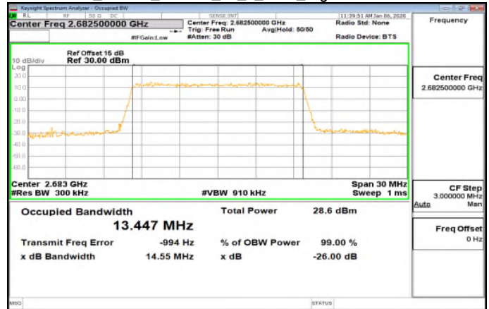
Band41_15MHz_64QAM_75_0_Main_HighCH41515-2682.5
