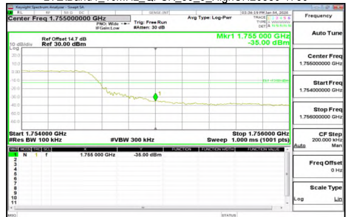
LTE\Band4_10MHz_QPSK_50_0_HighCH20350-1750
