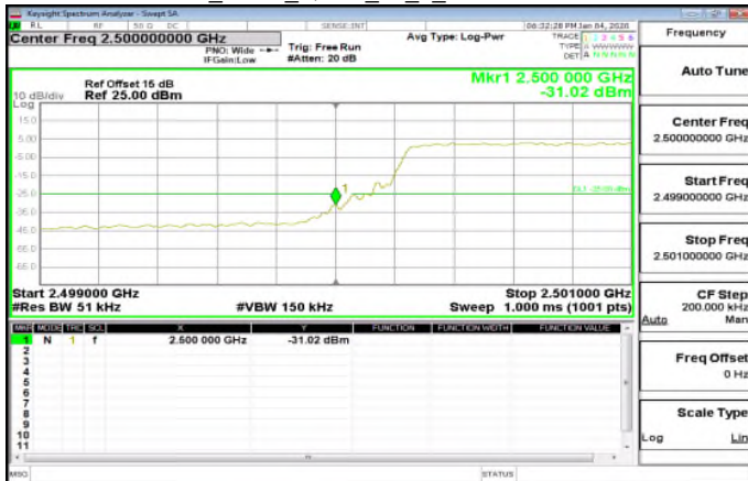
LTE\Band7_5MHz_QPSK_25_0_LowCH20775-2502.5
