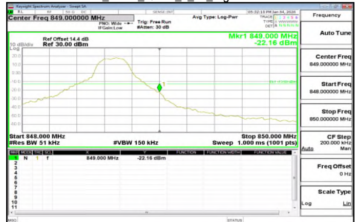
LTE\Band5_5MHz_QPSK_1_24_HighCH20625-846.5
