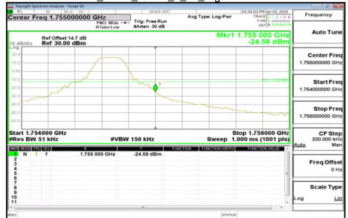
LTE\Band4_5MHz_QPSK_1_24_HighCH20375-1752.5
