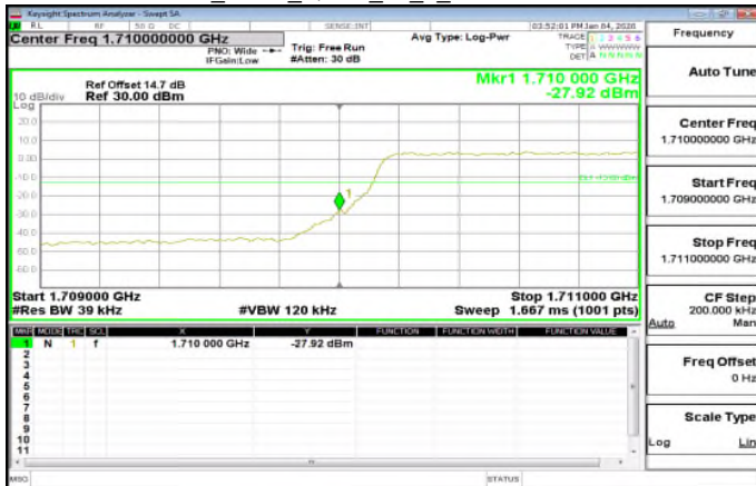
LTE\Band4_3MHz_QPSK_15_0_LowCH19965-1711.5
