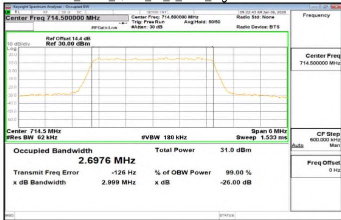
Band12_3MHz_QPSK_15_0_Main_HighCH23165-714.5
