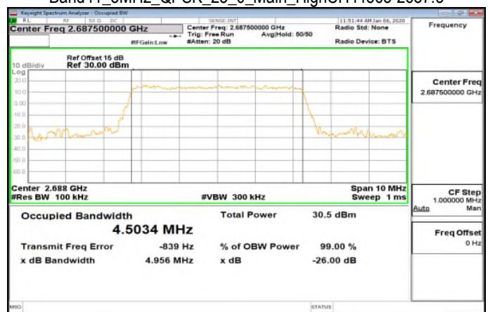
Band41_5MHz_QPSK_25_0_Main_HighCH41565-2687.5
