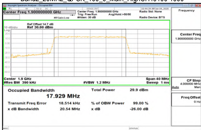
Band2_20MHz_QPSK_100_0_Main_HighCH19100-1900
