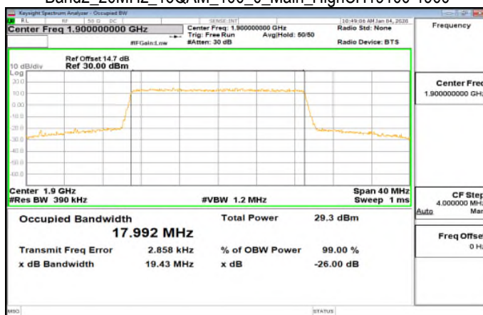
Band2_20MHz_16QAM_100_0_Main_HighCH19100-1900
