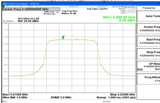
Full RU_802.11ax_20MHz_5500MHz
