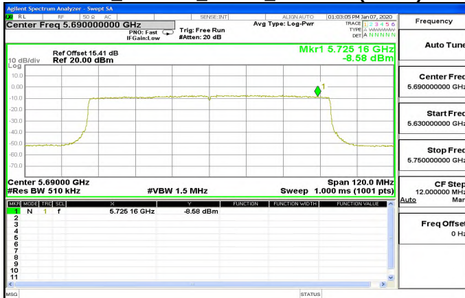
Full RU_802.11ax_80MHz_5690MHz (UNII 3)
