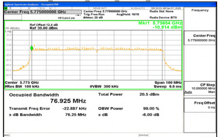
FCC 802.11ax 80MHz_Chain0_5775MHz
