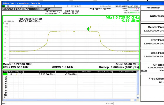
Full RU_802.11ax_20MHz_5720MHz (UNII 3)
