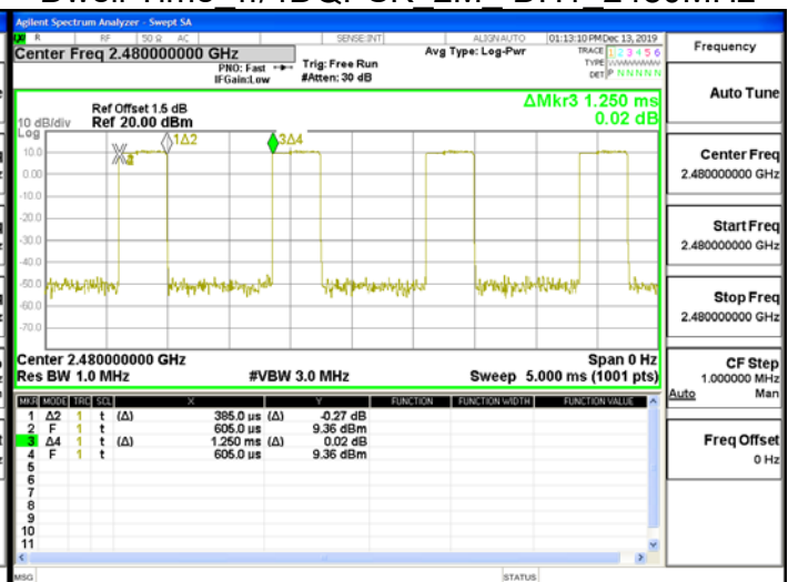
Dwell Time \pi/4 DQPSK 2M DH1 2480MHz
