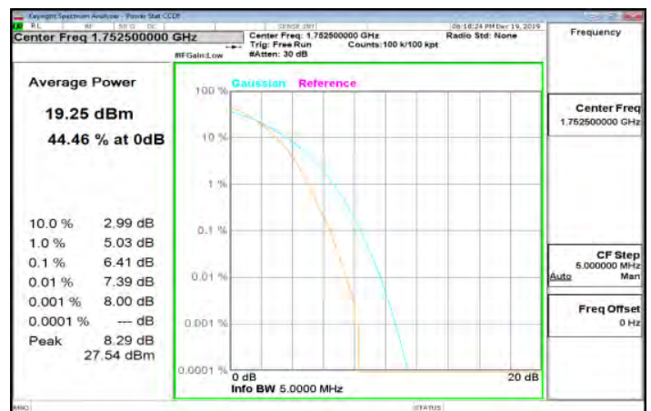
LTE_Band4_5MHz_64QAM_25_0_HighCH20375-1752.5
