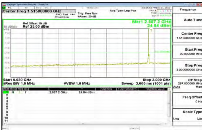
30MHz~3GHz_Band38_15MHz_QPSK_1_0_MidCH38000-2595
