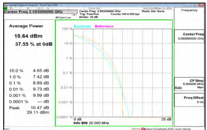
LTE_Band41_20MHz_64QAM_100_0_MidCH40620-2593
