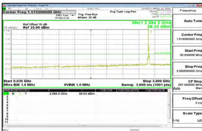
30MHz~3GHz_Band41_20MHz_QPSK_1_0_MidCH40620-2593
