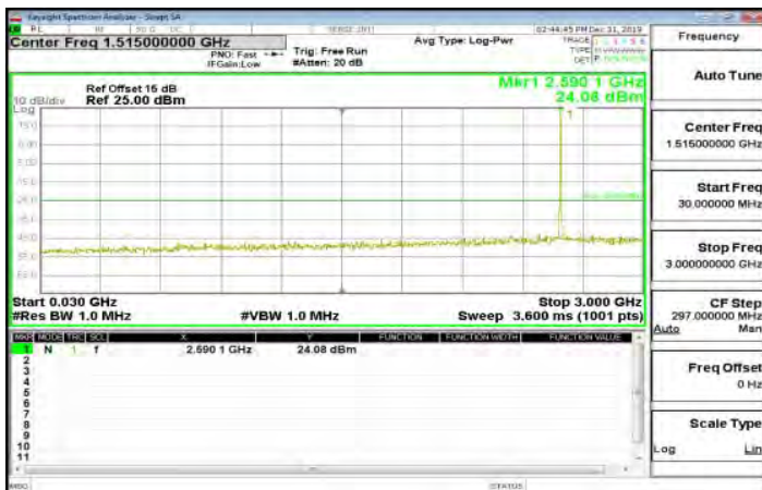
30MHz~3GHz_Band38_10MHz_QPSK_1_0_MidCH38000-2595
