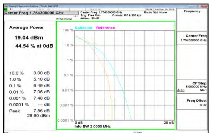
LTE_Band4_1_4MHz_64QAM_6_0_HighCH20393-1754.3
