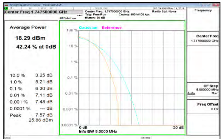
LTE_Band4_15MHz_64QAM_75_0_HighCH20325-1747.5
