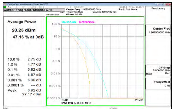
LTE_Band2_5MHz_64QAM_25_0_HighCH19175-1907.5
