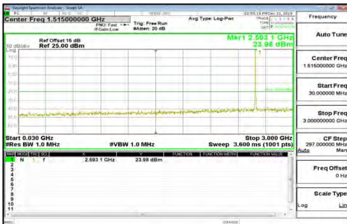
30MHz~3GHz_Band38_5MHz_QPSK_1_0_MidCH38000-2595
