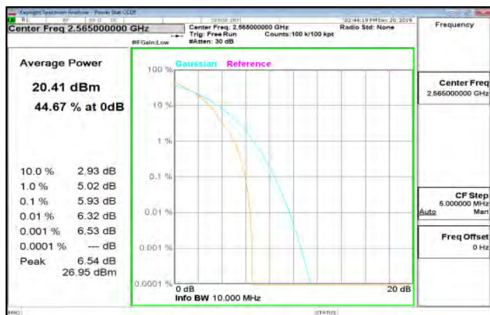
LTE_Band7_10MHz_64QAM_50_0_HighCH21400-2565
