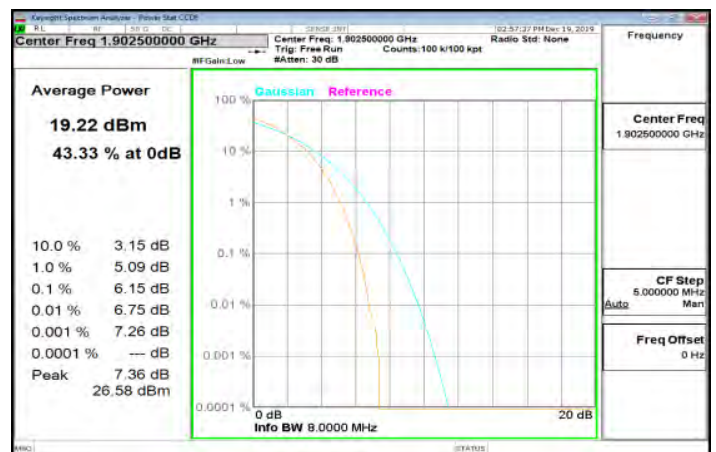
LTE_Band2_15MHz_64QAM_75_0_HighCH19125-1902.5
