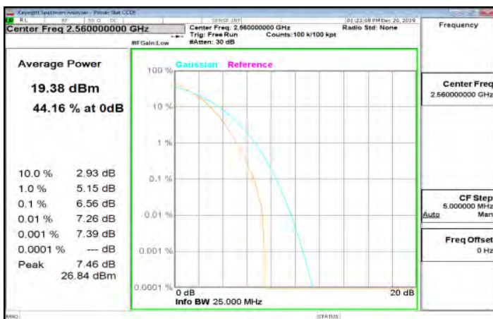
LTE_Band7_20MHz_64QAM_100_0_HighCH21350-2560
