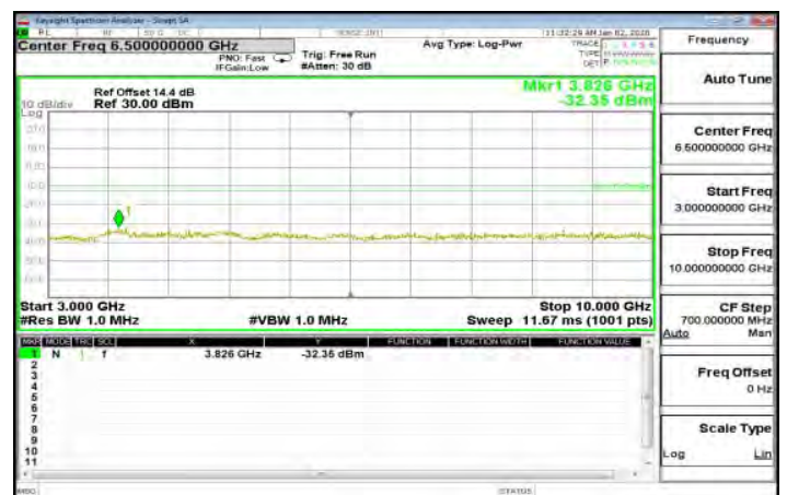
3GHz~10GHz_HSUPA_B5_MidCH4183-836.6
