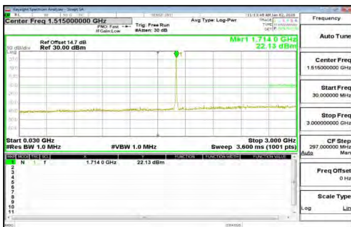
30MHz~3GHz_HSDPA_B4_LowCH1312-1712.4
