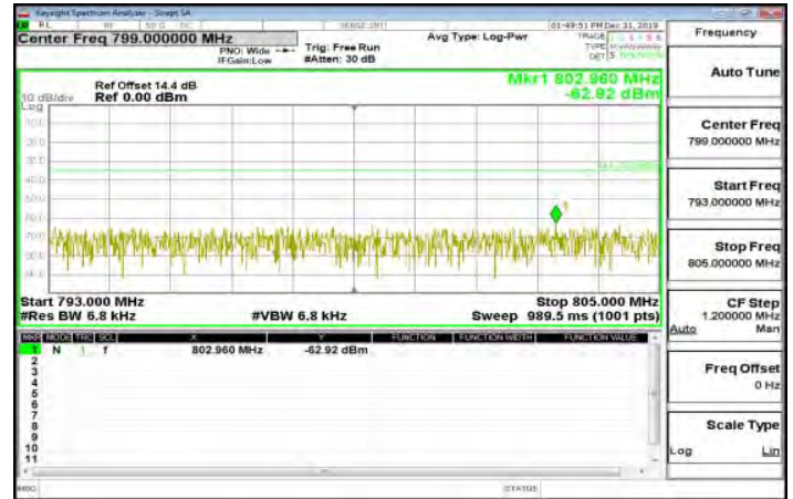
Inband-1_Band13_10MHz_QPSK_1_0_MidCH23230-782
