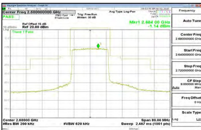
Band41_20MHz_16QAM_100_0_CH41490
