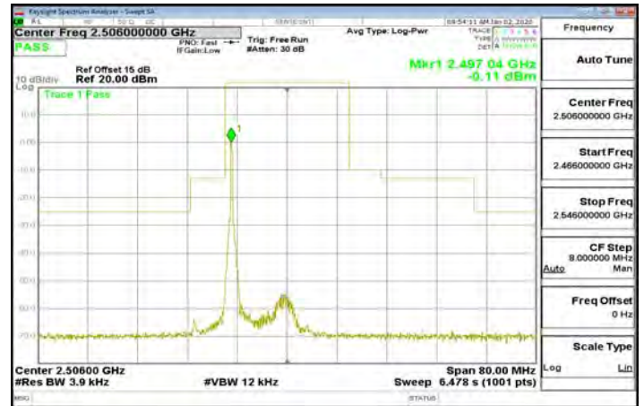
Band41_20MHz_64QAM_1_0_CH40620
