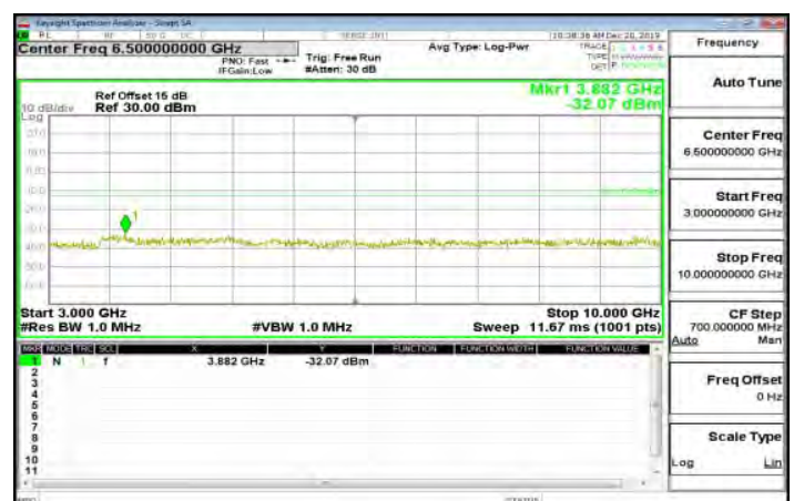
3GHz~10GHz_Band5_5MHz_QPSK_1_0_MidCH20525-836.5
