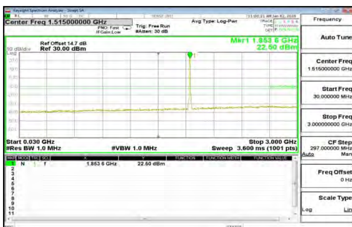
30MHz~3GHz_WCDMA_B2_LowCH9262-1852.4
