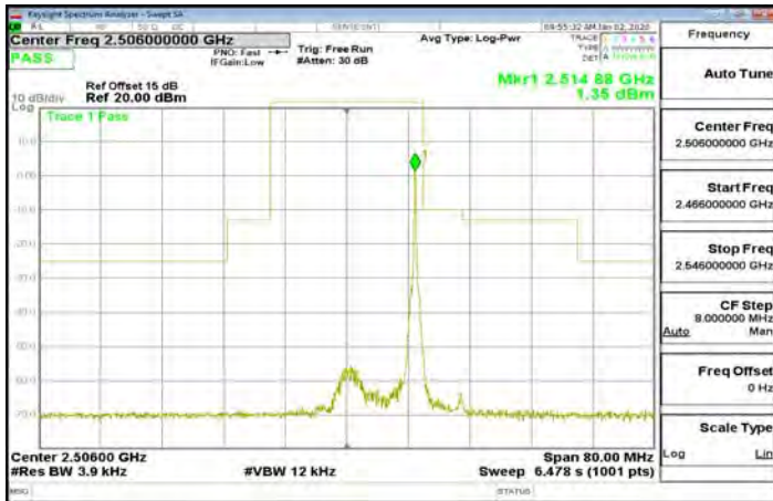
Band41_20MHz_64QAM_1_99_CH40620
