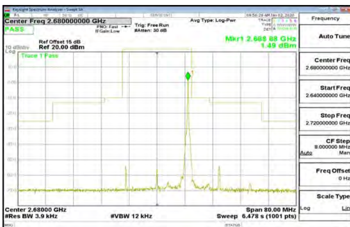
Band41_20MHz_64QAM_1_99_CH41490
