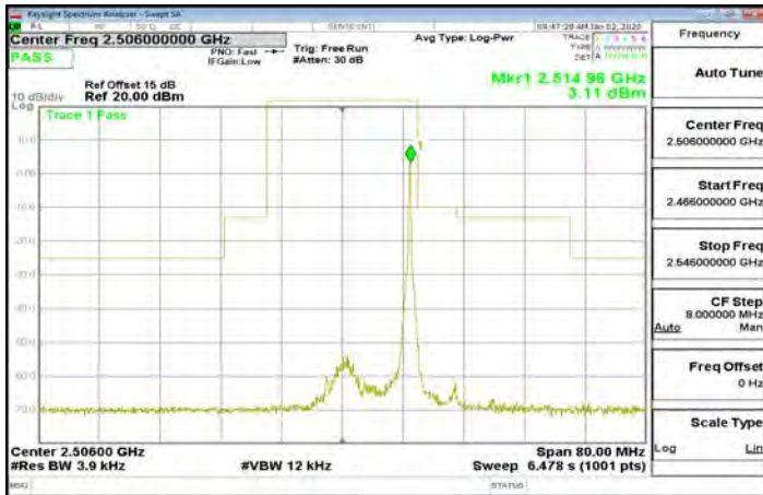
Band41_20MHz_QPSK_1_99_CH40620
