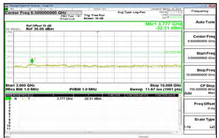
3GHz~10GHz_Band5_10MHz_QPSK_1_0_MidCH20525-836.5
