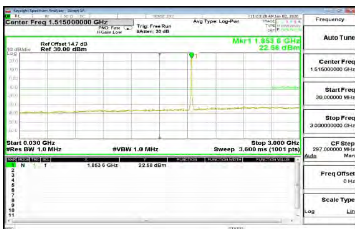
30MHz~3GHz_HSUPA_B2_LowCH9262-1852.4
