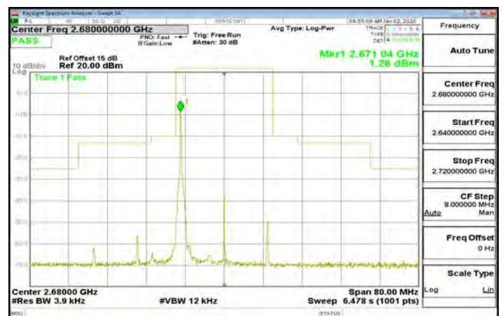
Band41_20MHz_64QAM_1_0_CH41490
