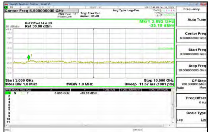
Inband-1_Band13_5MHz_QPSK_1_0_LowCH23205-779.5
