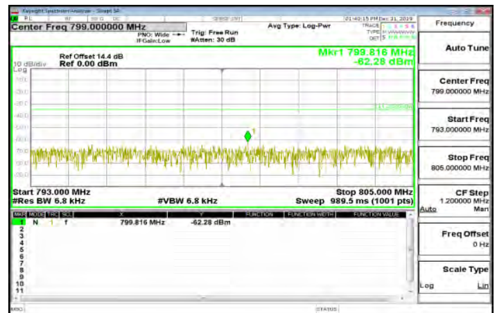
Inband-2_Band13_10MHz_QPSK_1_0_MidCH23230-782
