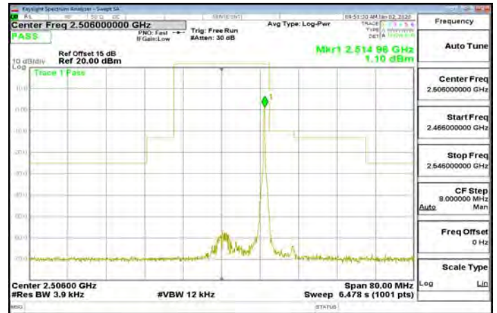
Band41_20MHz_16QAM_1_99_CH40620
