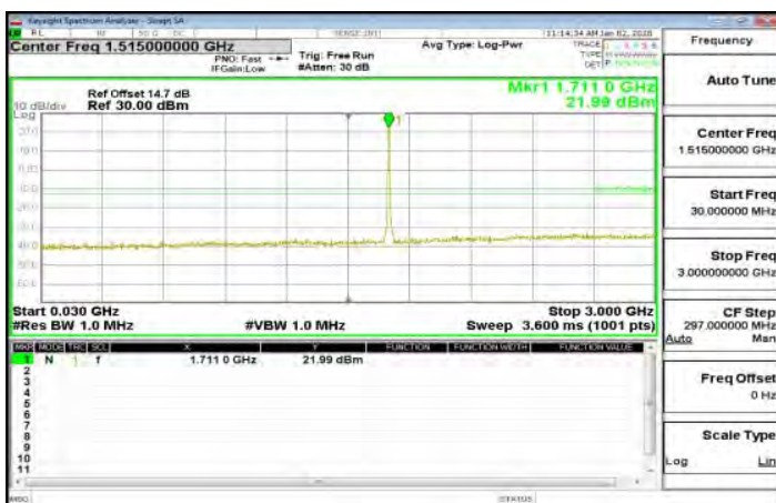
30MHz~3GHz_HSUPA_B4_LowCH1312-1712.4
