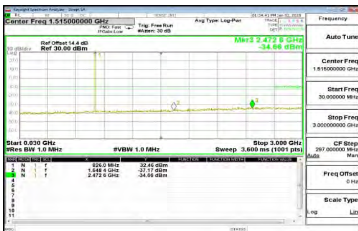
30MHz~3GHz_GPRS_850MHz_LowCH128-824.2
