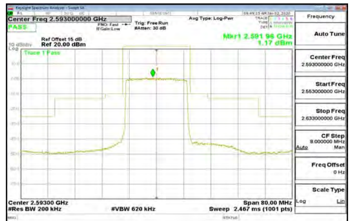
Band41_20MHz_QPSK_100_0_CH41490
