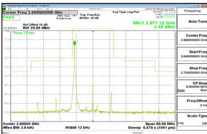
Band41_20MHz_16QAM_1_0_CH41490
