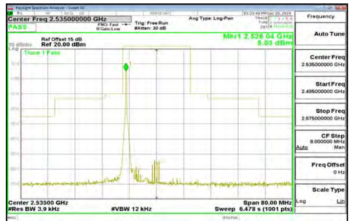
Band7_20MHz_64QAM_1_0_CH21350
