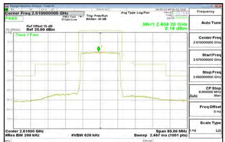
Band38_20MHz_QPSK_100_0_CH38150
