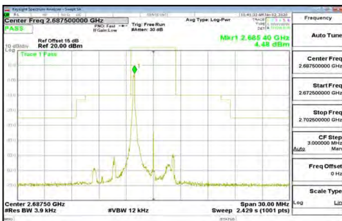
Band41_5MHz_QPSK_1_0_CH41565
