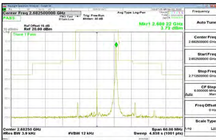
Band41_15MHz_16QAM_1_74_CH41515
