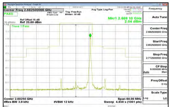
Band41_15MHz_64QAM_1_74_CH41515
