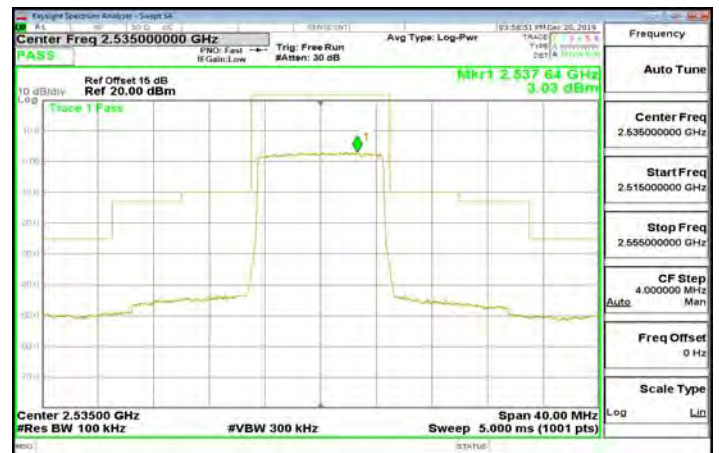
Band7_10MHz_QPSK_50_0_CH21400
