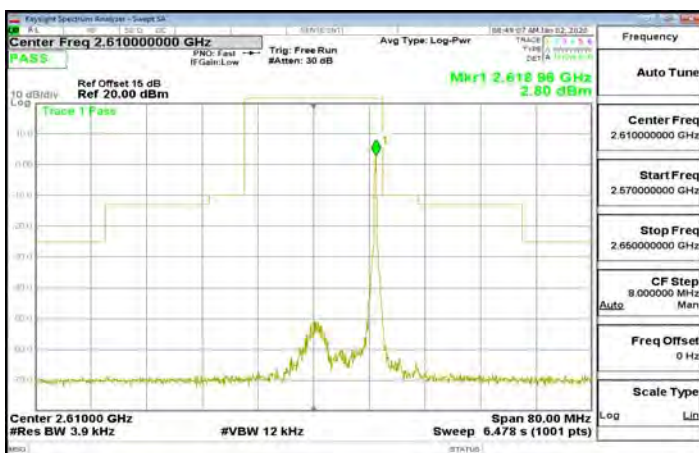
Band38_20MHz_QPSK_1_99_CH38150
