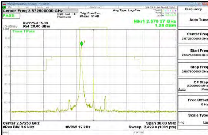
Band38_5MHz_64QAM_1_0_CH38000
