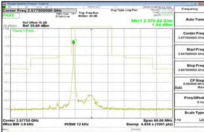
Band38_15MHz_QPSK_1_0_CH38000
