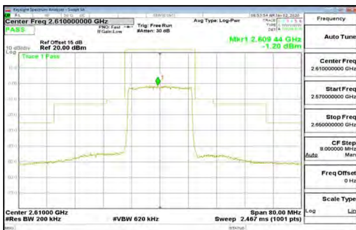
Band38_20MHz_16QAM_100_0_CH38150
