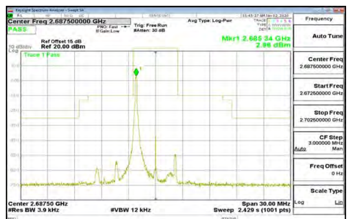
Band41_5MHz_16QAM_1_0_CH41565
