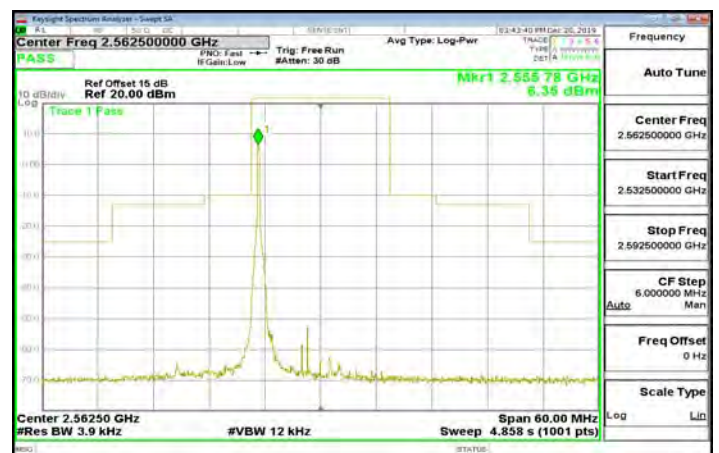
Band7_15MHz_16QAM_1_0_CH21375
