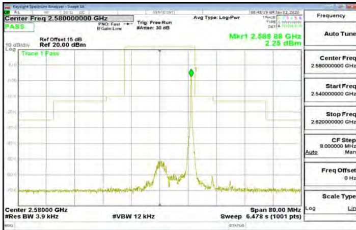
Band38_20MHz_QPSK_1_99_CH38000
