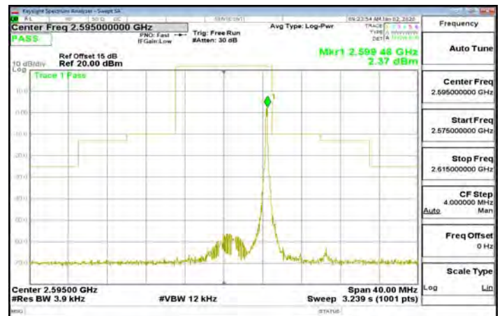
Band38_10MHz_16QAM_1_49_CH38200
