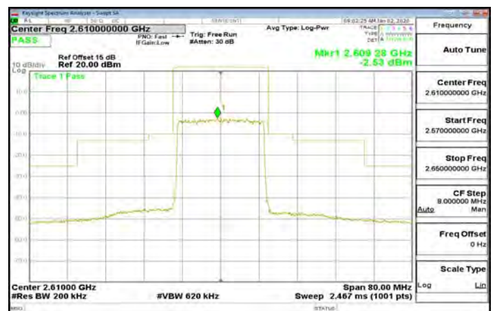
Band38_20MHz_64QAM_100_0_CH38150
