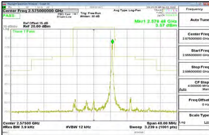
Band38_10MHz_QPSK_1_49_CH38000
