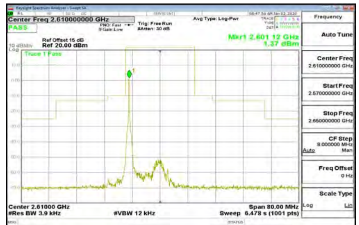
Band38_20MHz_QPSK_1_0_CH38150
