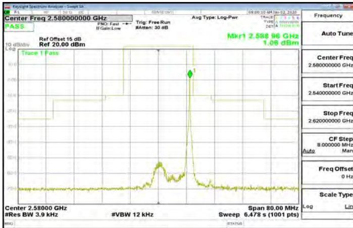
Band38_20MHz_64QAM_1_99_CH38000
