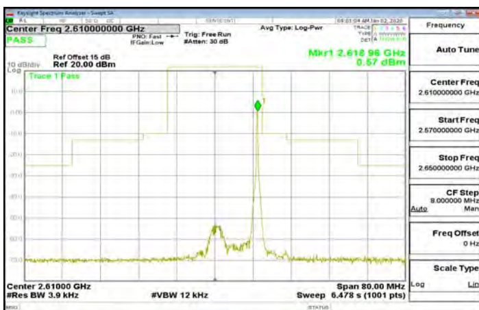
Band38_20MHz_64QAM_1_99_CH38150
