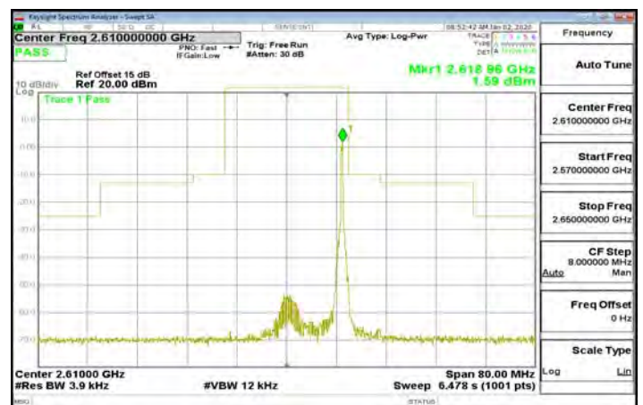
Band38_20MHz_16QAM_1_99_CH38150
