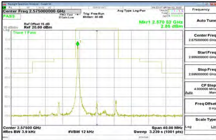
Band38_10MHz_16QAM_1_0_CH38000
