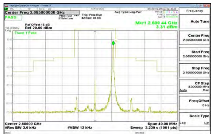
Band41_10MHz_16QAM_1_49_CH41540
