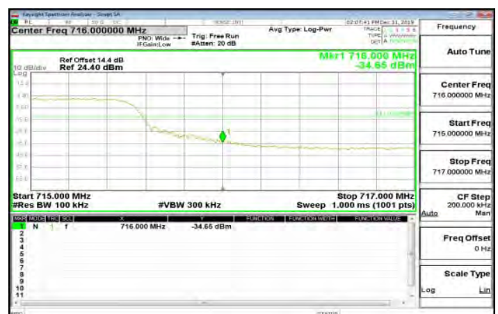
LTE\Band17_10MHz_QPSK_50_0_HighCH23800-711
