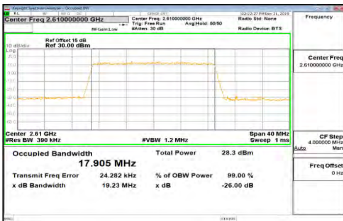
Band38_20MHz_64QAM_100_0_Main_HighCH38150-2610
