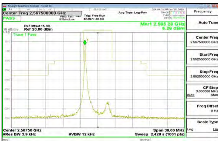
Band7_5MHz_QPSK_1_0_CH21425
