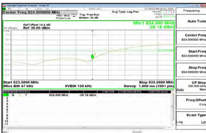
WCDMA\WCDMA_B5_LowCH4132-826.4
