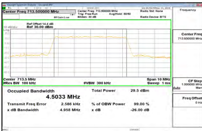
Band17_5MHz_16QAM_25_0_Main_HighCH23825-713.5
