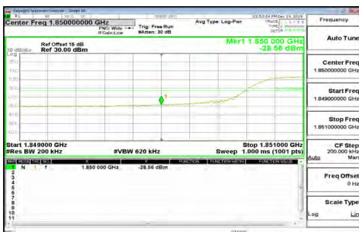
LTE\Band2_15MHz_QPSK_75_0_LowCH18675-1857.5
