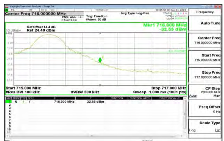
LTE\Band12_10MHz_QPSK_1_49_HighCH23130-711
