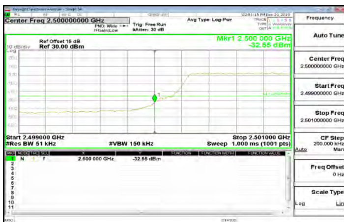
LTE\Band7_5MHz_QPSK_25_0_LowCH20775-2502.5
