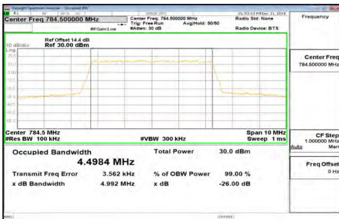
Band13_5MHz_16QAM_25_0_Main_HighCH23255-784.5
