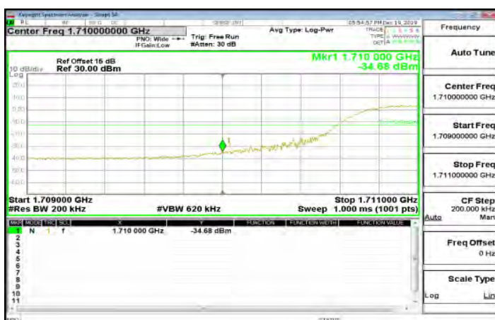
LTE\Band4_15MHz_QPSK_75_0_LowCH20025-1717.5
