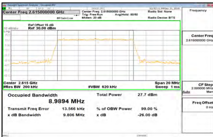
Band38_10MHz_64QAM_50_0_Main_HighCH38200-2615
