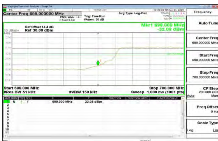
LTE\Band12_5MHz_QPSK_25_0_LowCH23035-701.5
