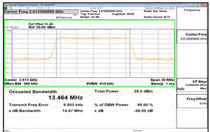
Band38_15MHz_64QAM_75_0_Main_HighCH38175-2612.5
