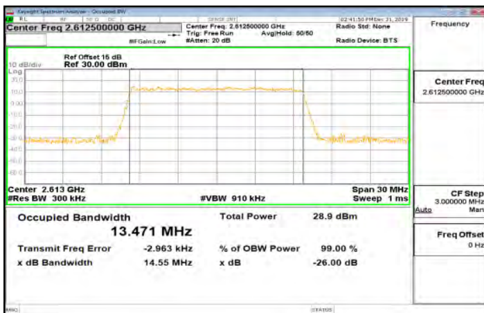
Band38_15MHz_16QAM_75_0_Main_HighCH38175-2612.5
