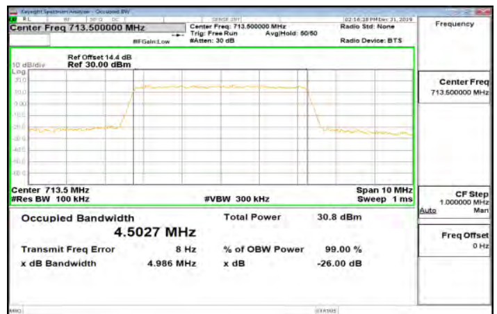
Band17_5MHz_QPSK_25_0_Main_HighCH23825-713.5
