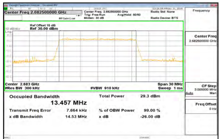
Band41_15MHz_64QAM_75_0_Main_HighCH41515-2682.5
