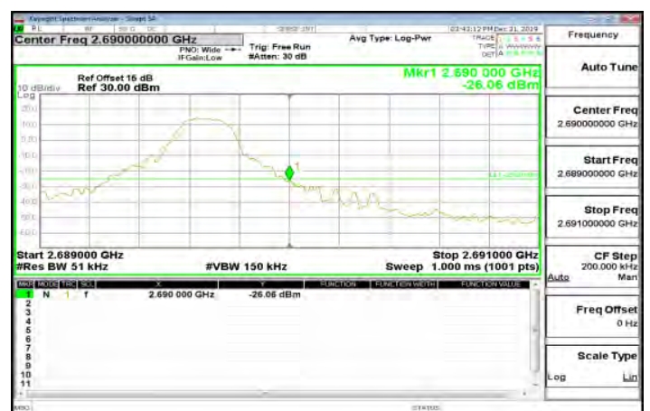
LTE\Band41_5MHz_QPSK_1_24_HighCH41565-2687.5
