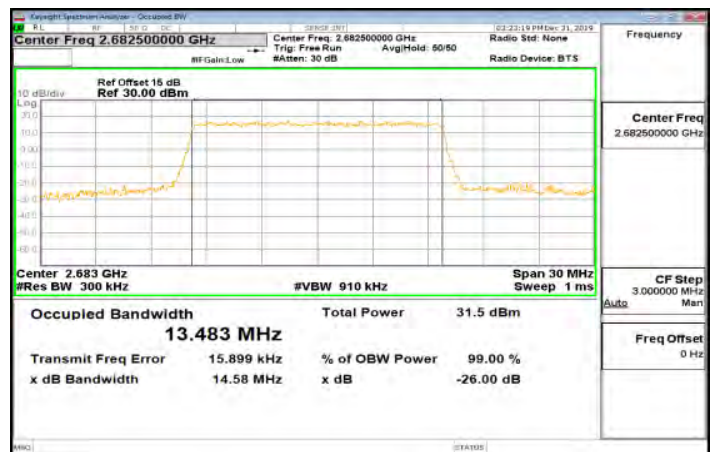
Band41_15MHz_QPSK_75_0_Main_HighCH41515-2682.5
