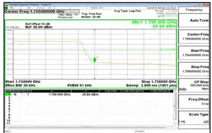
LTE\Band4_1_4MHz_QPSK_6_0_HighCH20393-1754.3
