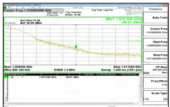
LTE\Band2_20MHz_QPSK_1_99_HighCH19100-1900
