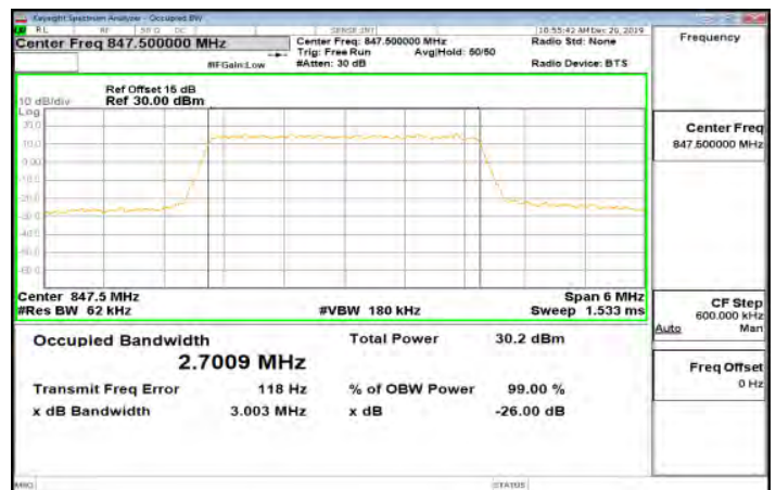
Band5_3MHz_16QAM_15_0_Main_HighCH20635-847.5
