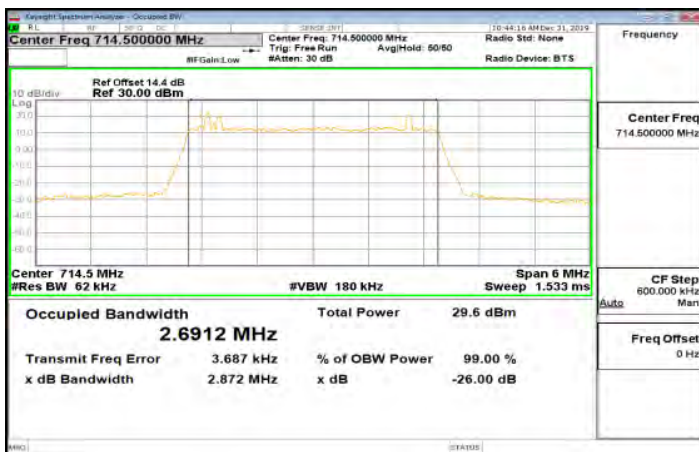
Band12_3MHz_64QAM_15_0_Main_HighCH23165-714.5
