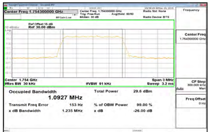
Band4_1_4MHz_QPSK_6_0_Main_HighCH20393-1754.3
