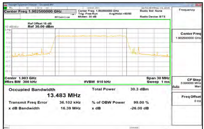
Band2_15MHz_QPSK_75_0_Main_HighCH19125-1902.5
