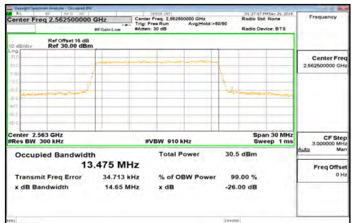
Band7_15MHz_QPSK_75_0_Main_HighCH21375-2562.5
