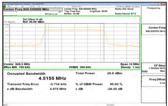
Band5_5MHz_64QAM_25_0_Main_HighCH20625-846.5
