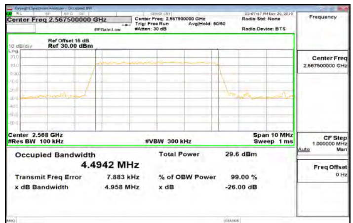
Band7_5MHz_64QAM_25_0_Main_HighCH21425-2567.5
