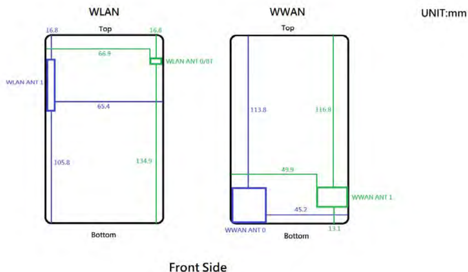
Fig.23 Antenna position of EUT
