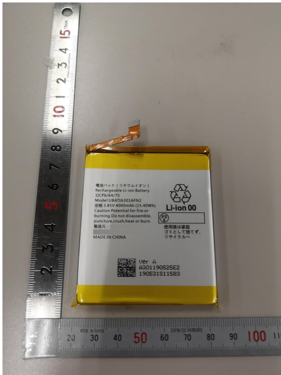
Battery 1
