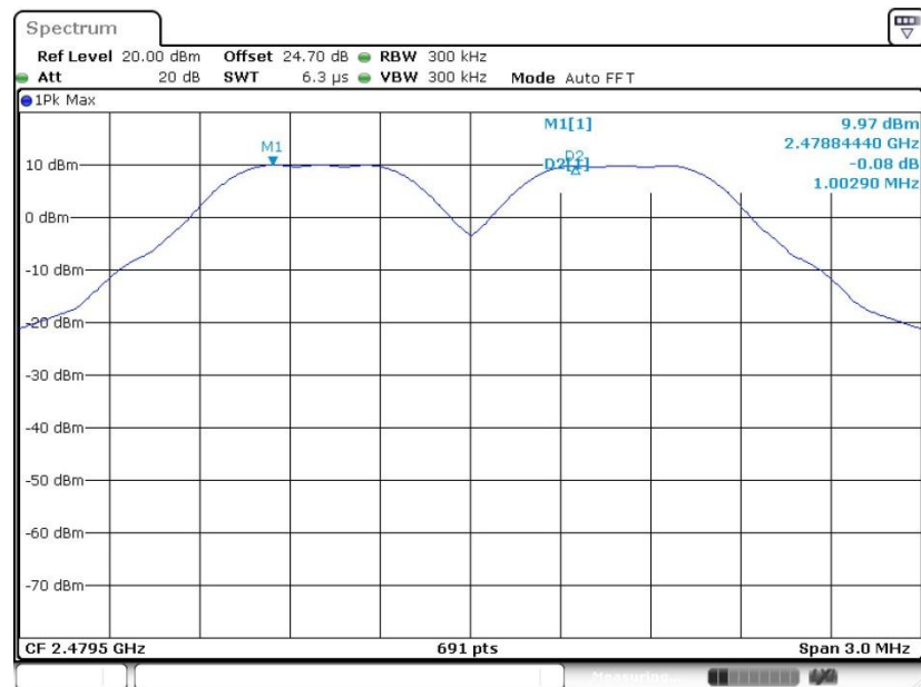
Channel Separation Plot on Channel 77 - 78
