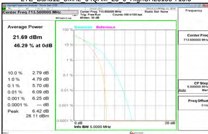
LTE Band12 5MHz 64QAM 25 0 HighCH23155-713.5
