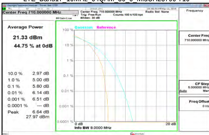
LTE Band17 10MHz 64QAM 50 0 MidCH23790-710
