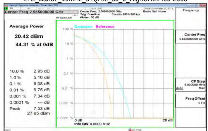
LTE Band7 10MHz 64QAM 50 0 HighCH21400-2565
