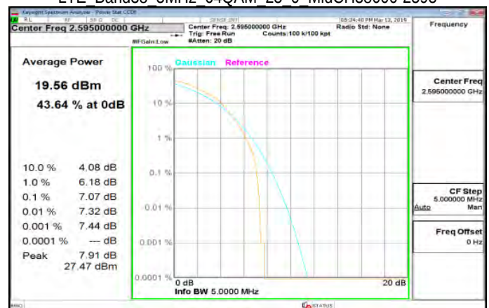
LTE Band38 5MHz 64QAM 25 0 MidCH38000-2595
