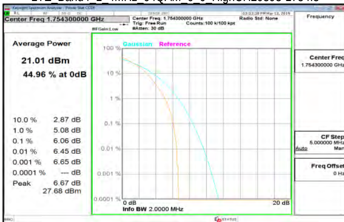
LTE Band4 1 4MHz 64QAM 6 0 HighCH20393-1754.3
