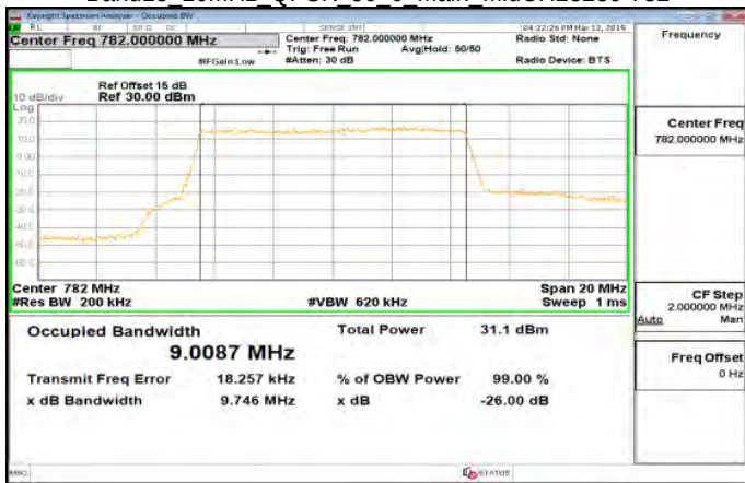
Band13 10MHz QPSK 50 0 Main HighCH23230-782
