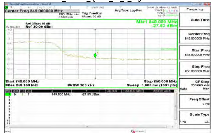
LTE\Band5 10MHz QPSK 50 0 HighCH20600-844
