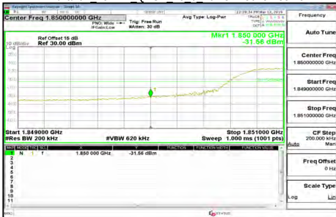
LTE\Band2 15MHz QPSK 75 0 LowCH18675-1857.5
