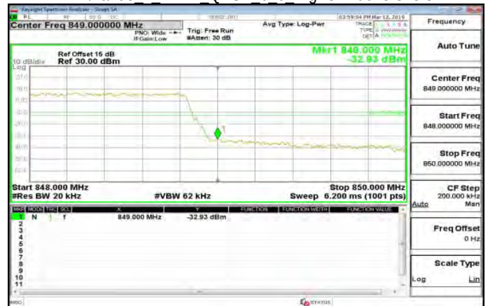
LTE\Band5 1 4MHz QPSK 6 0 HighCH20643-848.3
