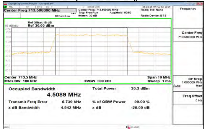
Band17 5MHz 64QAM 25 0 Main HighCH23825-713.5
