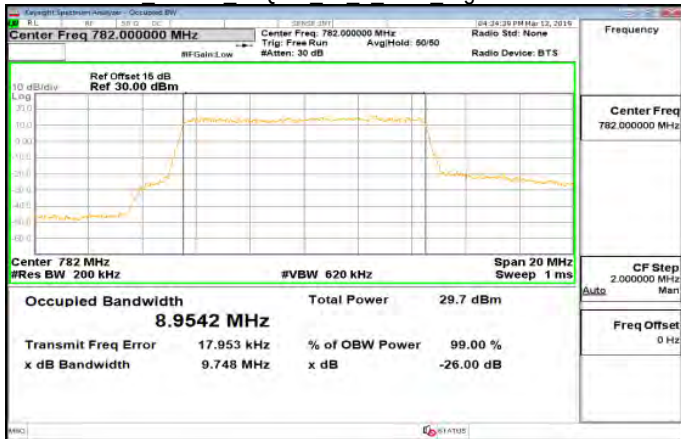
Band13 10MHz 64QAM 50 0 Main HighCH23230-782
