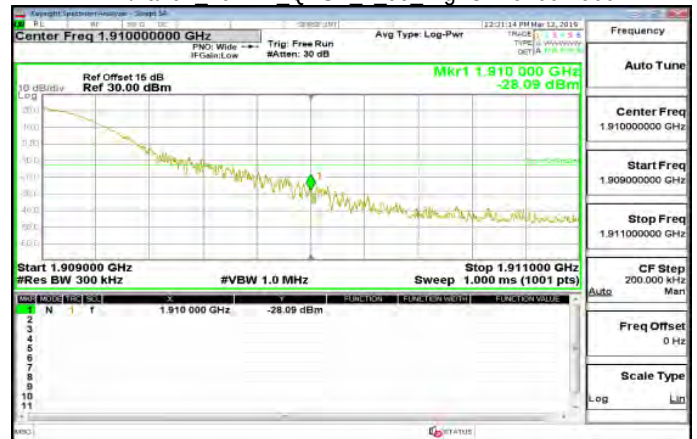
LTE\Band2 20MHz QPSK 1 99 HighCH19100-1900
