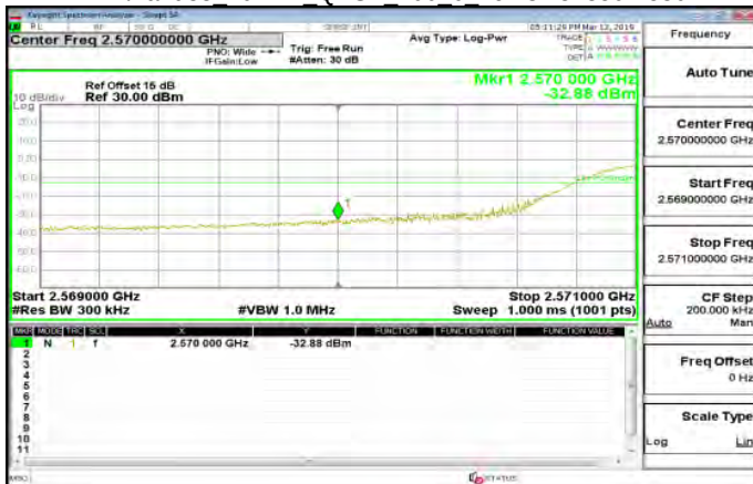
LTE\Band38 20MHz QPSK 100 0 LowCH37850-2580
