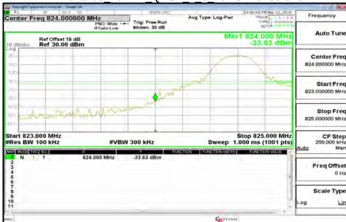
LTE\Band5 10MHz QPSK 1 0 LowCH20450-829
