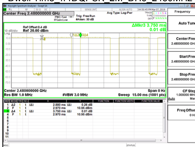
Dwell Time π4DQPSK 2M DH5 2480MHz
