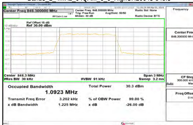
Band5 1 4MHz 64OAM 6 0 HighCH20643-848.3
