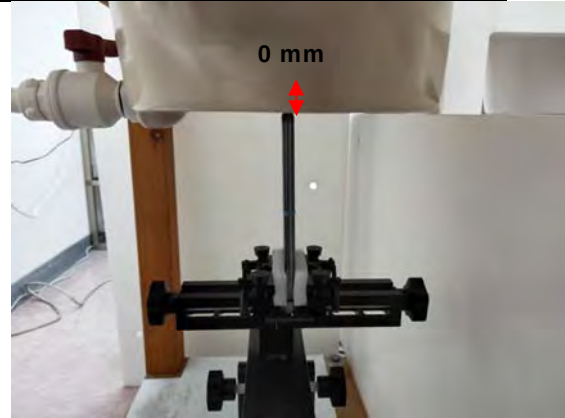
Fig.18 EUT Bottom side to flat phantom
