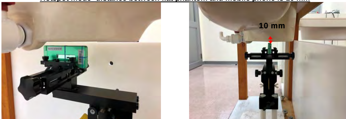
Fig.12 EUT Right side to flat phantom
