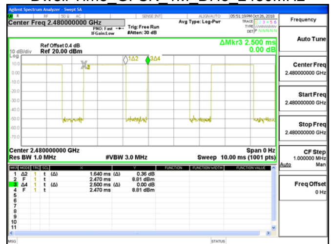
Dwell Time_GFSK_1M_DH3_2480MHz
