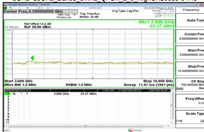
3GHz~10GHz Band5 3MHz OPSK 1 0 HighCH20635-847.5
