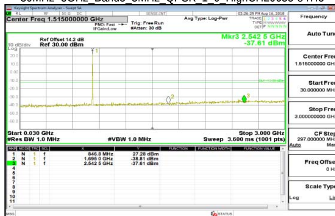
30MHz~3GHz Band5 3MHz OPSK 1 0 HighCH20635-847.5
