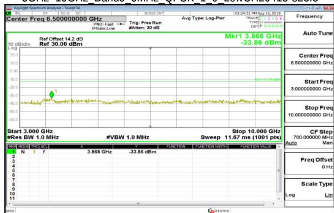
3GHz~10GHz Band5 3MHz OPSK 1 0 LowCH20415-825.5
