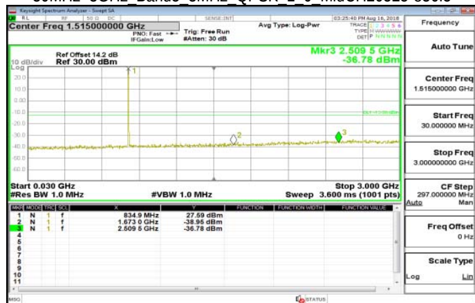
30MHz~3GHz Band5 3MHz OPSK 1 0 MidCH20525-836.5
