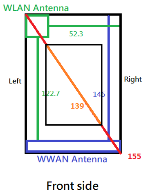
Fig.17 Antenna position of EUT
