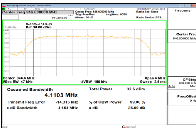
WCDMA_B5_HighCH4233-846.6
