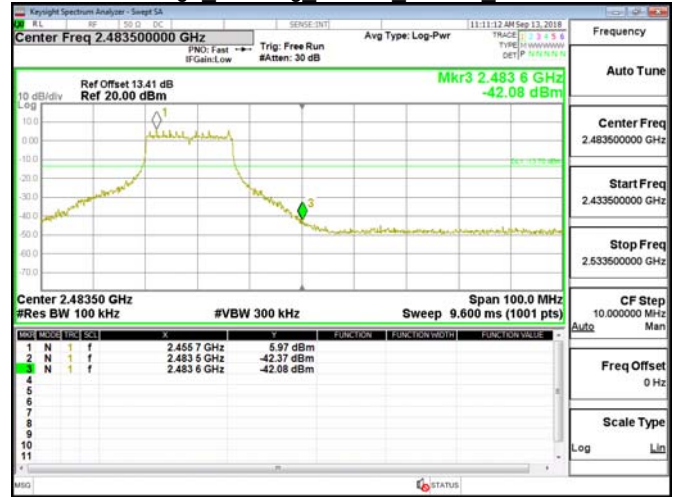
Band Edge 802.11g 20MHz Chain0 2462MHz
