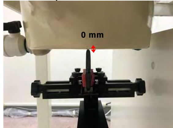
Fig.18 EUT Right side to flat phantom
